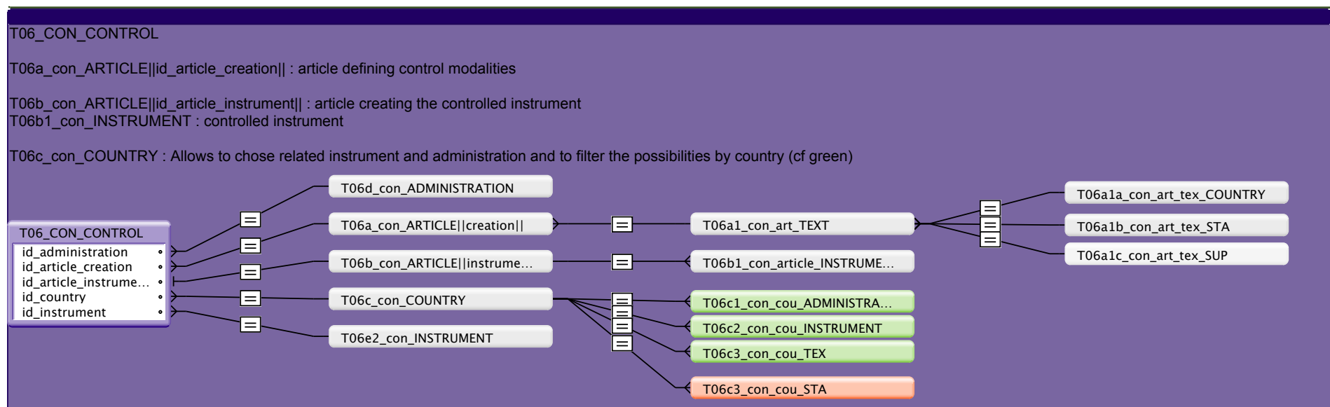
Anchor-buoy diagram n°5: CONTROL table
