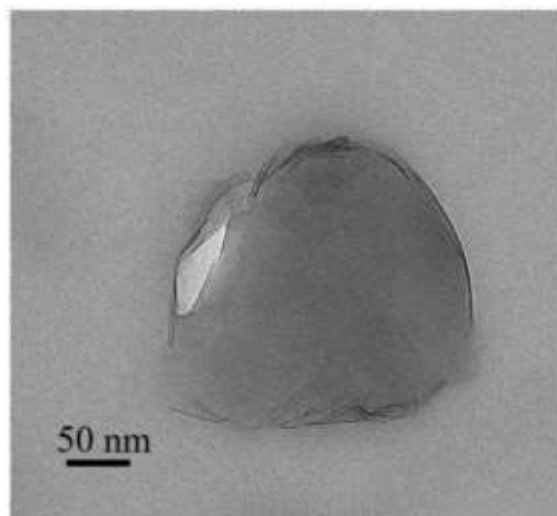
FIG. 3.11. Typical TEM of a PMMA/PS/Cloisite 20A droplet
