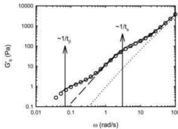
FIG. 1.10 Storage modulus of a PI/PDMS blend compatibilized with 0.1% of a bloc copolymer. The dashed line is the PI/PDMS blend without compatibilizer. [23]
