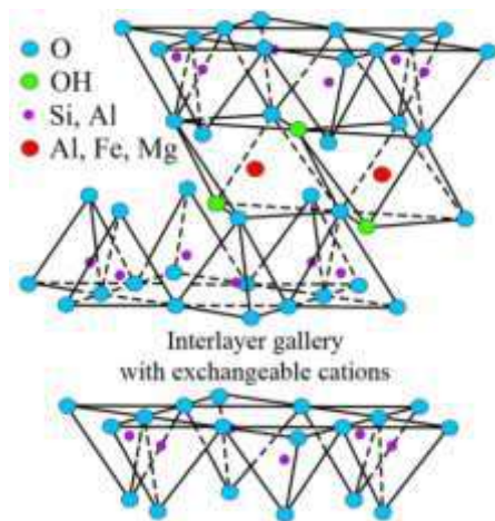
FIG. 1.7 Structure of montmorillonite
