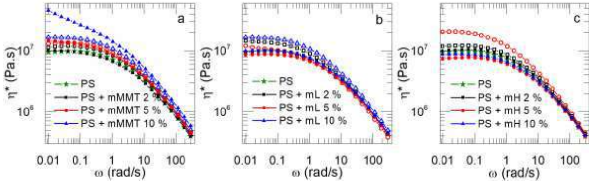
FIG. 6.3 Complex viscosities of PS with different concentration of (a) MMT and mMMT, (b) L and mL and (c) H and mH. Filled symbols correspond to the modified clays and open symbols to non-modified clays
