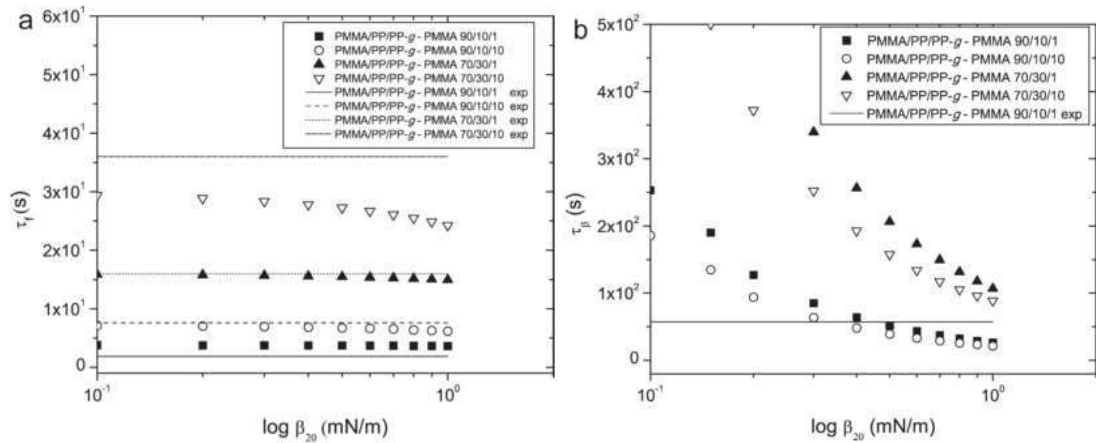
FIG. 1.13 (a) \tau_f values as a function of \beta_{20} estimated using eqs. ( 1.12 )-( 1.15 ), for PMMA/PP/PP-g-PMMA blends. (b) \tau\beta values as a function of b_{20} estimated using eqs. ( 1.12 )-( 1.15 ), for PMMA/PP/PP-g-PMMA blends[16]
