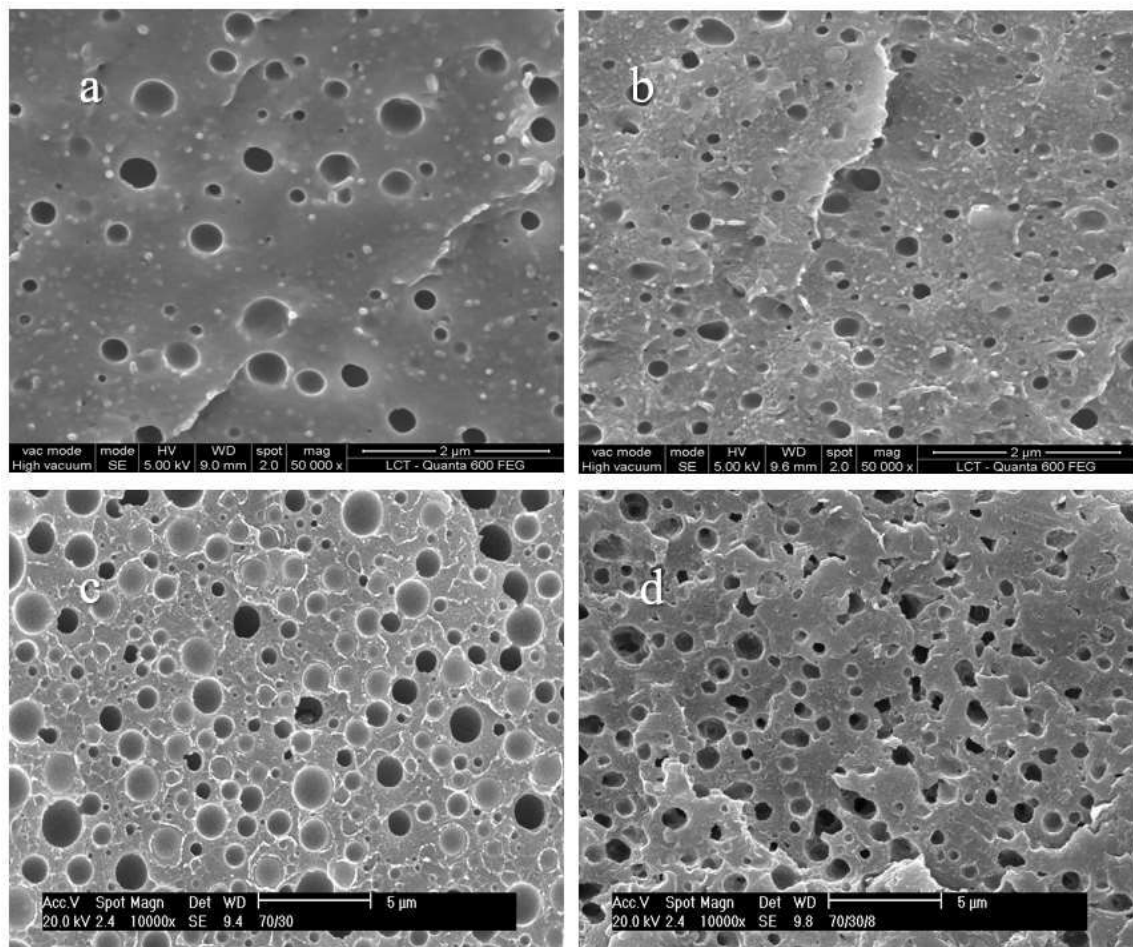
FIG. 3.3. Morphology of blends for a 90/10 composition (a) with and (b) without the addition of 8 % Cloisite 20A, and for a 70/30 composition (c) without and (d) with addition of 8 % of Cloisite 20A
