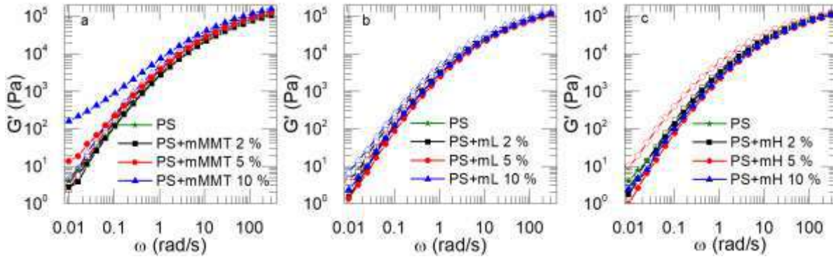
FIG. 5.4 Storage moduli as a function of frequency at 200 °C of PS with (a) MMT and mMMT, (b) L and mL and (c) H and mH. Filled symbols correspond to the modified clays and open symbols to non-modified clays
