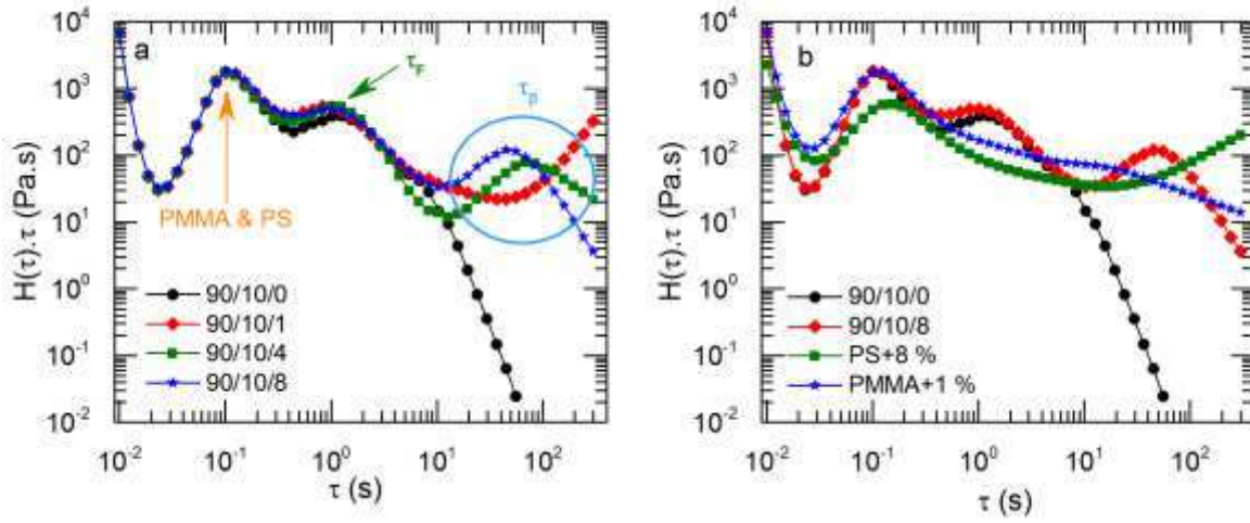
FIG. 3.15. Relaxation spectrum of PMMA+(PS+C) (90/10) (a) blends with different levels of Cloisite 20A at 220 °C, (b) comparison of 90/10/8 blends with PMMA+1 % and PS+8 %
