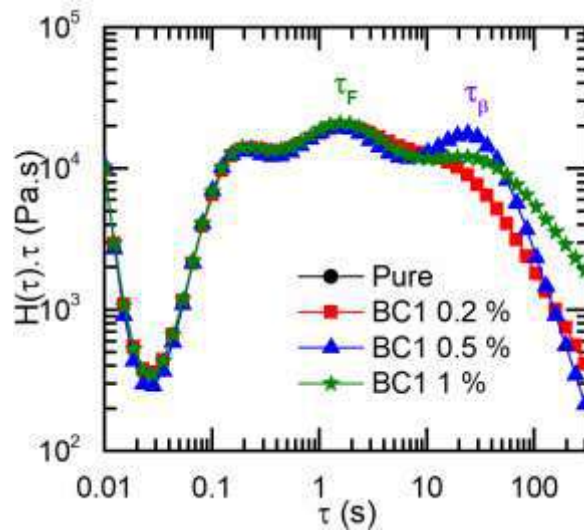
FIG. 4.6 Relaxation spectra of BC1 at 180 °C
