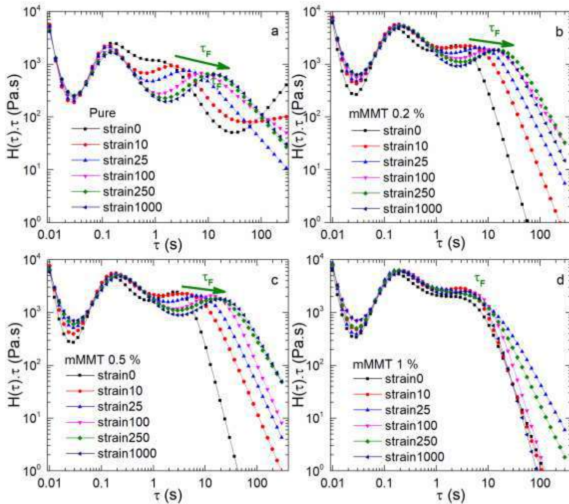
FIG. 5.10 Relaxation spectra of the blends containing (a) 0 %, (b) 0.2 %, (c) 0.5 % and (d) 1 % of mMMT during coalescence test
