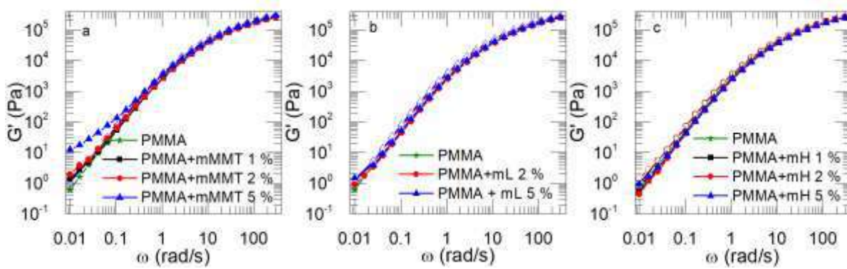
FIG. 5.5 Storage moduli as a function of frequency at 200 °C of PMMA with (a) MMT and mMMT, (b) L and mL and (c) H and mH. Filled symbols correspond to the modified clays and open symbols to non-modified clays
