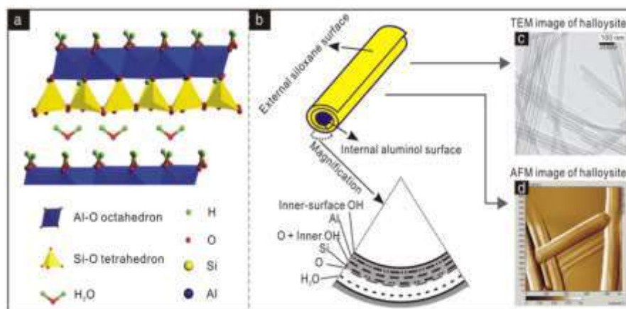
FIG. 1.8 Halloysite structure [43]
