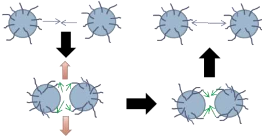
FIG. 3.1 Illustration of the Marangoni stress
