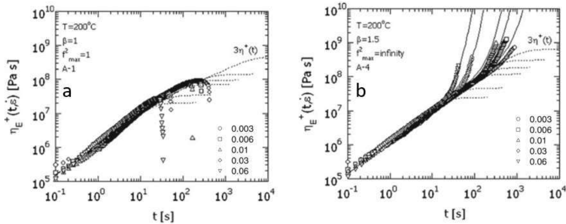
FIG. 1.15 Tensile stress growth coefficients of (a) linear PMMA, (b) cross-linked PMMA. The viscoelastic limit is indicated by 3\eta^+ , the other dotted lines and plain lines are the predictions of various models not described here. Extracted from [71]
