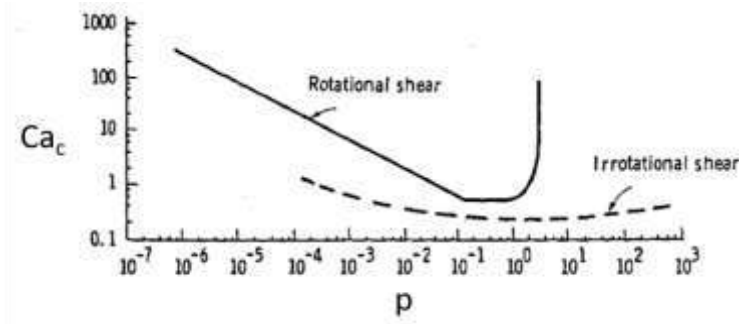
FIG. 4.1 Effect of the viscosity ratio on critical capillary number in rotational shear and irrotational shear fields [5]
