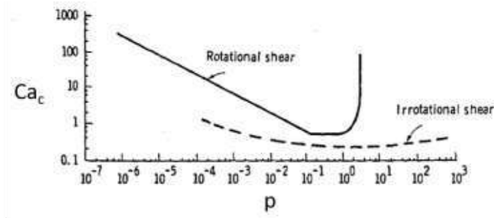
FIG. 1.2 Effect of the viscosity ratio on critical capillary number in rotational shear and irrotational shear fields [5]
