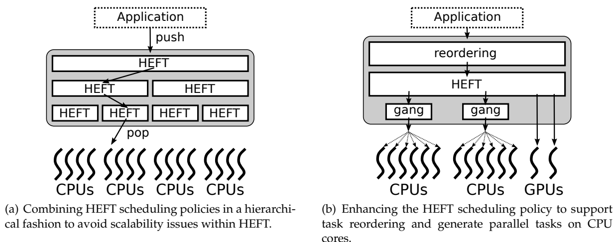
Figure 3.21: Composing scheduling policies.
