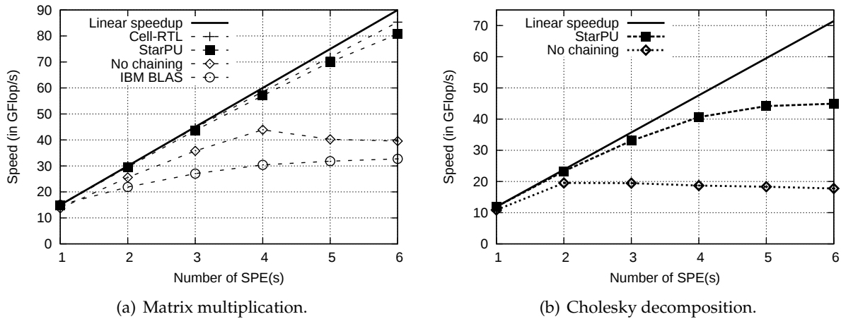
Figure 2.22: Scalability of StarPU on the Cell processor.
