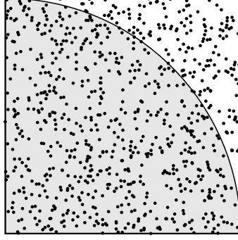
Figure 7.11: Computing \pi with Monte Carlo method. Points are randomly shot over a unit square. The shaded area delimits a quarter of circle with a unit radius, centered at (0,0). The probability that a point should hit the shaded is equal to \frac{\pi}{4} .
