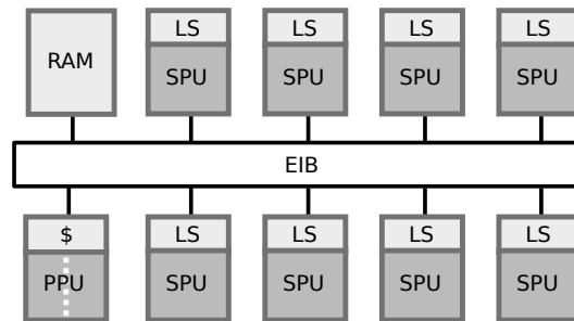
Figure 1.2: Architecture of the Cell Processor.
