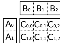
Figure 4.5: Product of two tiled matrices. The result is a 2 \times 3 tiled matrix which is computed with only 6 tasks. Each tile (e.g. A_1 or C_{0,2} ) is stored contiguously in memory.
