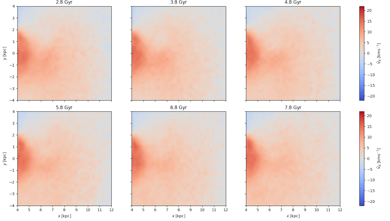
Figure 3.5: Bar-only model test-particle snapshots for constant pattern speed: frames from \tilde{V}_R(x, y) shown in the (x, y) plane defined on [4, 12] \text{ kpc} \times [-4, 4] \text{ kpc} , and binned with bins of size (250 \text{ pc})^2 , always with the same orientation of the bar, at different snapshots. The radial velocity field generated by a constant pattern-speed bar is remarkably stable with time.
