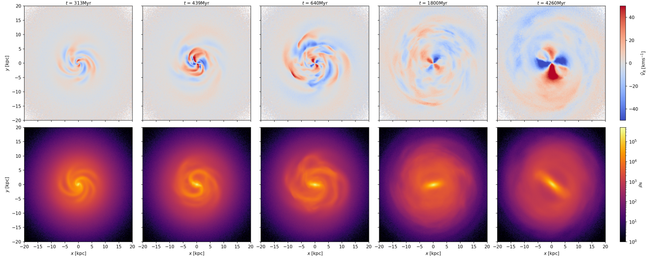
Figure 5.2: Snapshots for stellar particles from a N-body simulation initialized with our axisymmetric potential Table 2.1. The sampling of 835 million particles was done with AGAMA . The disk DFs are the same as in Eq. 1.27 with parameters described in Chapter 3. The DF for the bulge and dark matter halo were obtained using Eddington inversion implemented in AGAMA . For the gas particles we don't determine the DF, instead we sample the positions from density and assign velocities following the axisymmetric Jeans equation. The top panels show the median radial velocity. Bottom panels show the number density. The non-axisymmetric structures are visible in different snapshots from earlier (left panels) to later frames (right panels). Preliminary analysis shows that the bar formed in this self-consistent simulation has a similar length to the bar model presented in this thesis. The stellar disk, bulge, dark matter halo and gas disk has respectively, 150.3, 16.7, 626.25, 41.75 millions of particles,
