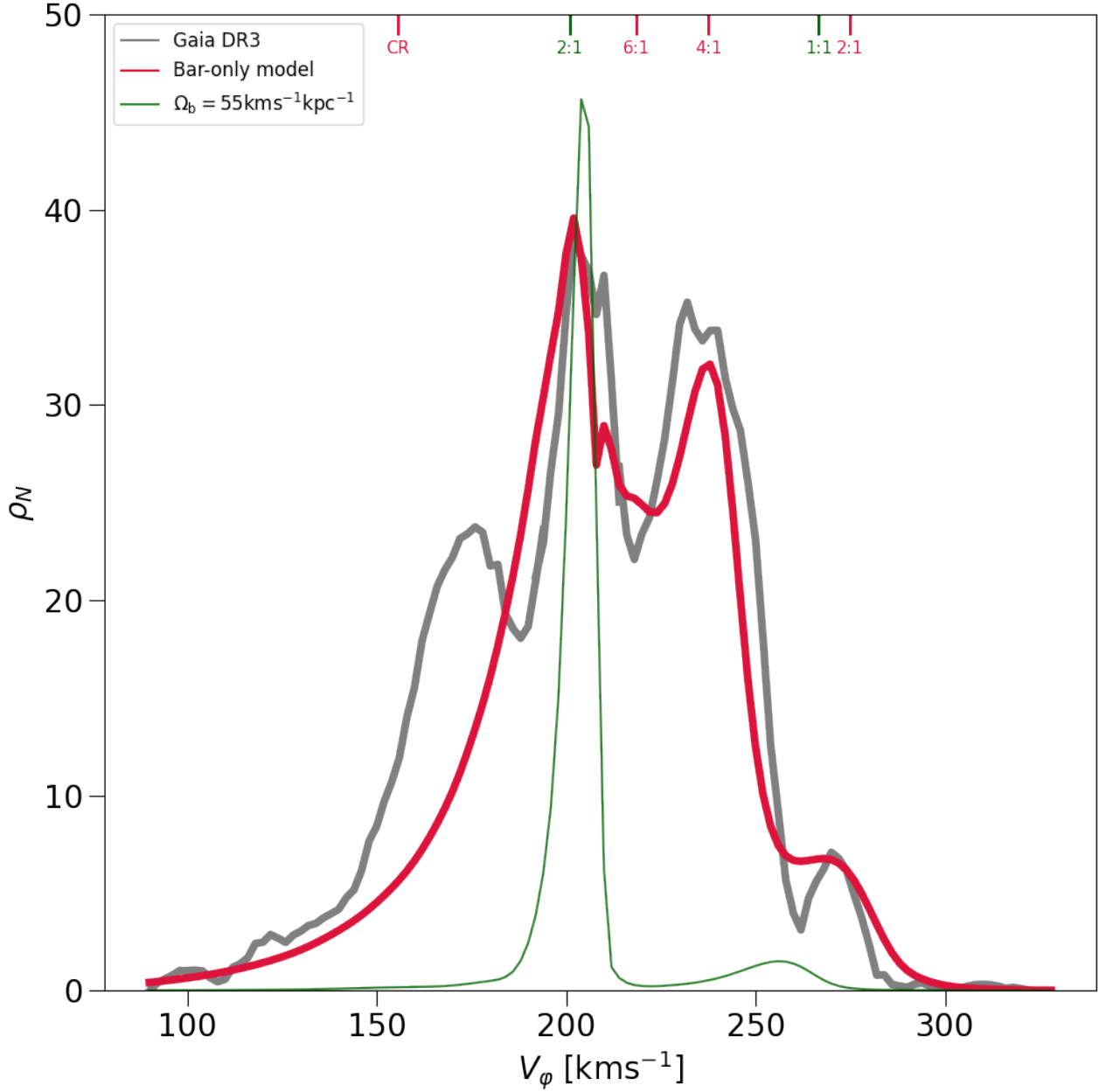
Figure 2.8: 1-Dimensional distribution of the azimuthal velocity of stars in the Solar neighborhood within 99 \text{ kms}^{-1} < V_R < 101 \text{ kms}^{-1} , a region of velocity space where the bar impact dominates the distribution (over potential spiral arms signatures). In grey, the stellar distribution from the Gaia RVS disk sample in the Solar neighborhood, smoothed with the Savitzky-Golay filter from the SciPy library. Red line: the renormalized best bar-only model at V_R = 100 \text{ kms}^{-1} , with pattern speed \Omega_b = 37 \text{ kms}^{-1}\text{kpc}^{-1} . For reference, we are providing the results for \Omega_b = 55 \text{ kms}^{-1}\text{kpc}^{-1} (green line), where only the 1:1 resonance leaves a small signature at higher V_\phi than the strong OLR peak. The approximate locations of the different resonances evaluated with Eq. A.5 (described in the Appendix A) represented as red ( \Omega_b = 37 \text{ kms}^{-1}\text{kpc}^{-1} ) and green ( \Omega_b = 55 \text{ kms}^{-1}\text{kpc}^{-1} ) dashes on top of the plot.
