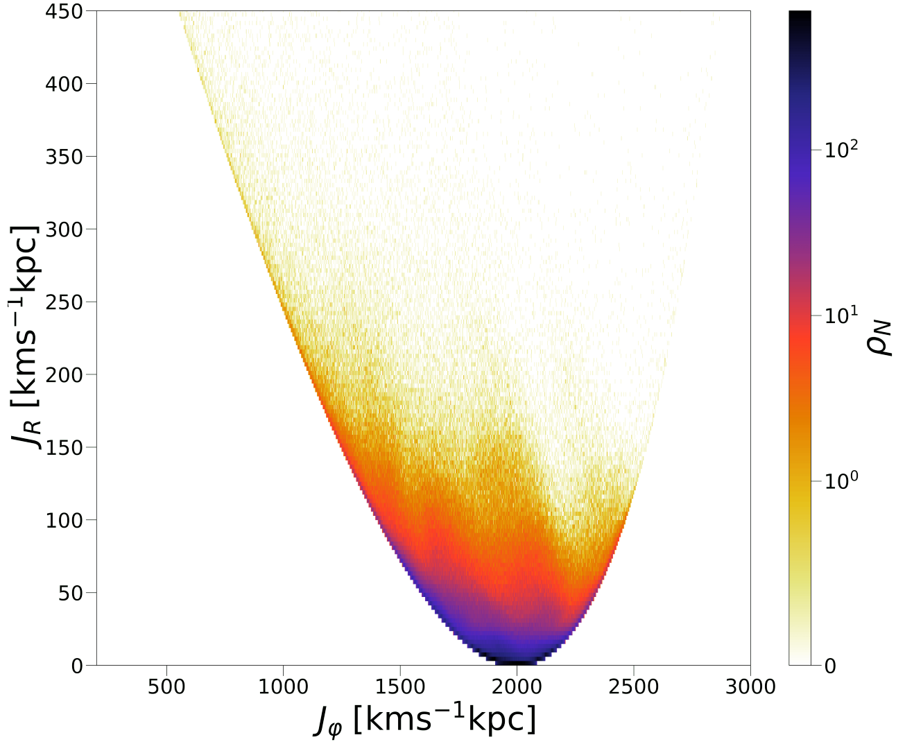
Figure 2.3: Same distribution as in Fig 2.2 on the actions (J_\phi, J_R) plane (computed with AGAMA in the axisymmetric potential of Table 2.1) defined on a [0, 600] \text{ kms}^{-1} \text{ kpc}^{-1} \times [200, 3000] \text{ kms}^{-1} \text{ kpc}^{-1} grid, binned with (3 \times 2 \text{ km}^2 \text{ s}^{-2} \text{ kpc}^{-2}) bins.
