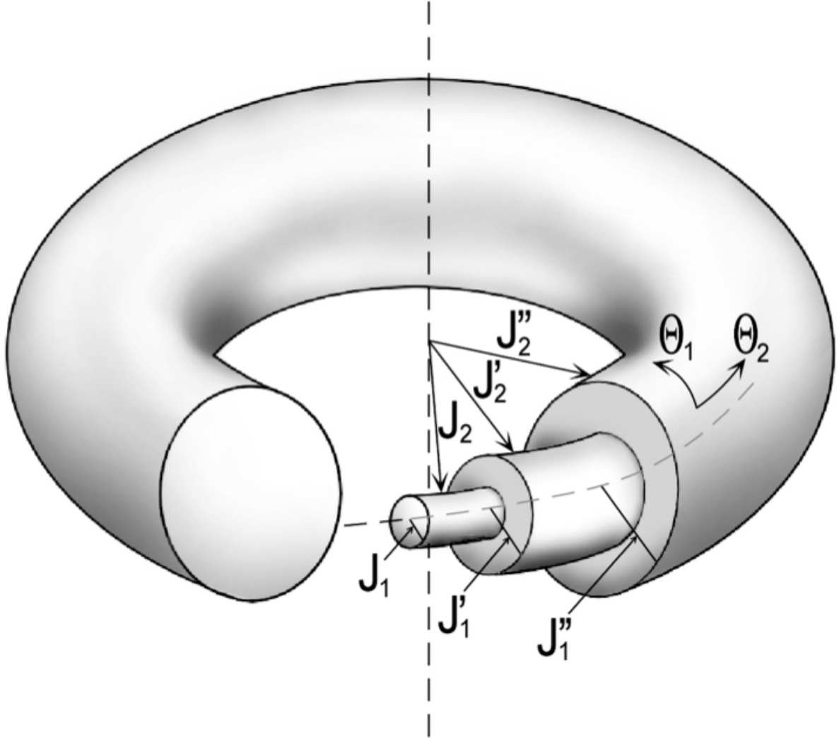
Figure 1.5: Figure extracted from (Masoliver and Ros, 2011). Illustration of a 2-dimensional orbital torus in action-angle variables within 4-dimensional phase-space (for instance, within a Galactic disk, neglecting the vertical direction). The nested torii represent different regular orbits, distinguished by their actions. The stellar trajectory lies on the torus surface and is mapped by the angles that evolve linearly in time.
