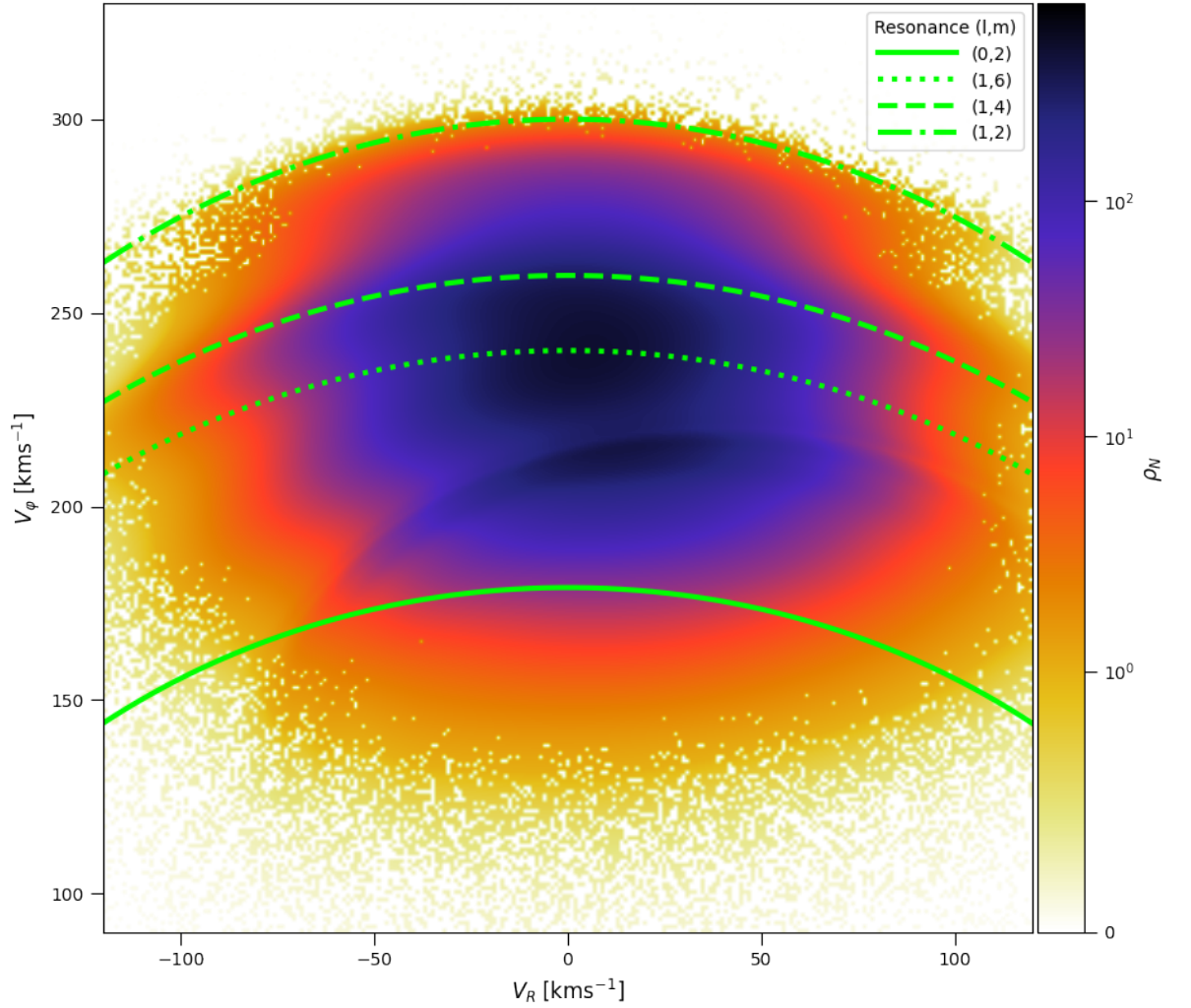
Figure A.1: Resonant lines V_\varphi^{\text{res}} as a function of V_R from Eq. A.5 at R = R_0 , computed with the potential of Table 2.1, for a bar pattern speed of 37 \text{ km s}^{-1} \text{ kpc}^{-1} . The lines are overlaid on top of the local velocity space density produced by our preferred bar-only model at the Sun's position.
