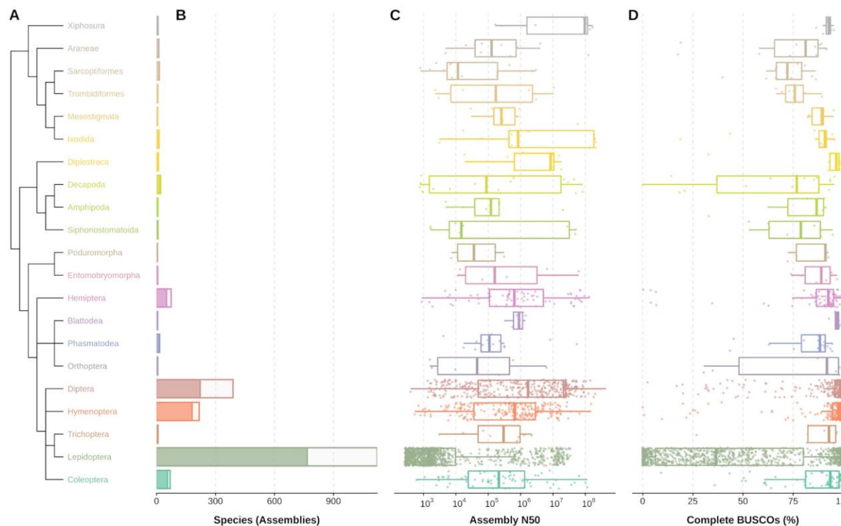
Figure 6-7: Assembly statistics for arthropod species. A: Phylogenetic tree. B: Number of assemblies for each group. C: Assembly N50 for each group. D: BUSCO completeness for each group. Figure from Feron and Waterhouse, 2022.
