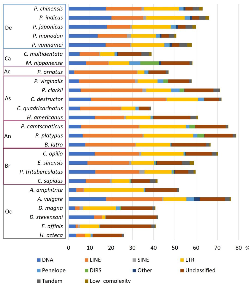
Figure 2. Proportion and content of repetitive elements in genomes. Percentage of repetitive elements in the genome by class of repetitive elements. De, Dendrobranchiata; Ca, Caridea; Ac, Achelata; As, Astacidea; An, Anomura; Br, Brachyura; Oc, other Crustacea.
