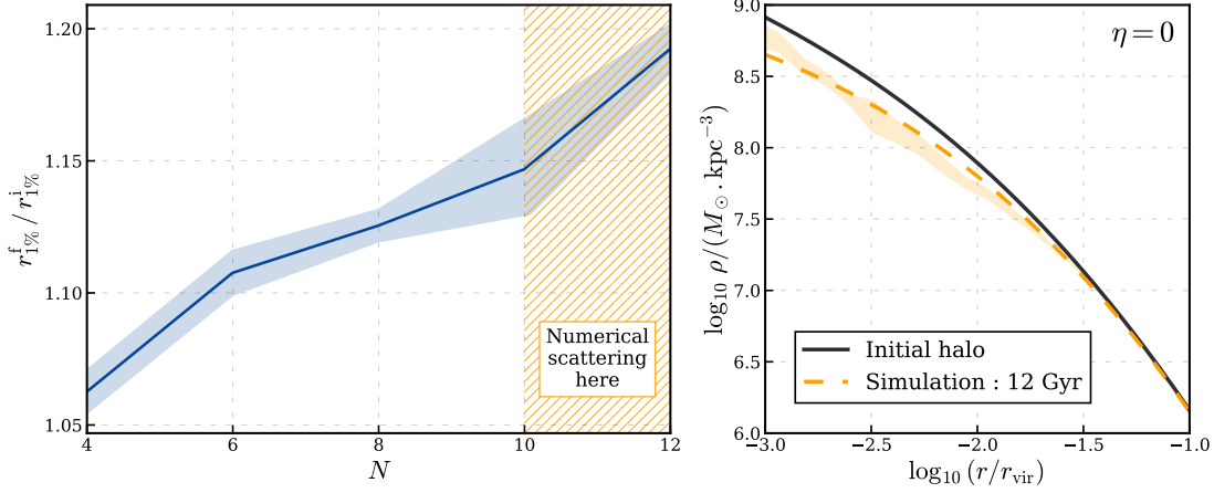
Figure 2.10: Left Panel: Magnitude of the core creation as a function of the number of alternating mass flows. Core creation is measured using the ratio r_{1\%}^f / r_{1\%}^i of the final to initial radius enclosing 1% of the virial mass of the halo. We simulated the cases with N = 4, 6, 8, 10 , and 12 even-numbered episodes, i.e., the moments when the central baryonic mass is the same as the initial mass. For each case, we conducted 5 simulations, and the scatter corresponds to the standard deviation of the 5 values of r_{1\%}^f / r_{1\%}^i obtained. The increase in this ratio with N indicates that core creation becomes more significant as the number of flow episodes increases. The region where N > 10 is hatched to indicate the presence of numerical scattering. An example of the effect of this scattering is shown in the right panel, where the artificial lowering of the density profile is observed when the simulation time is too long, despite the baryonic mass remaining constant.
