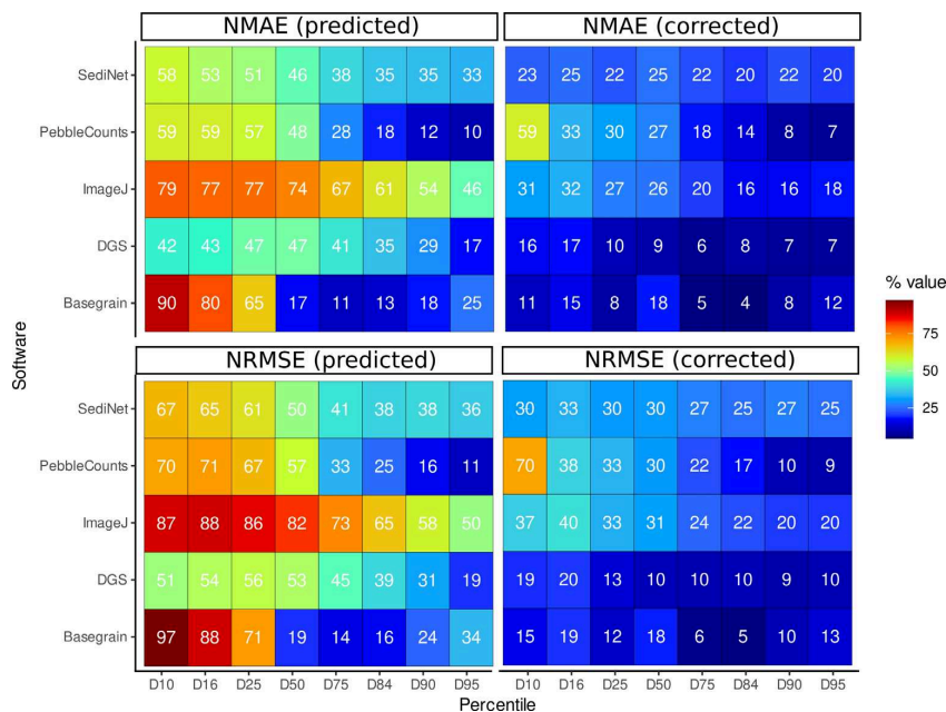
FIGURE 7 Values of normalized root mean square error (NRMSE) (predicted and corrected) and normalized mean absolute error (NMAE) (predicted and corrected) for each software packages. Predicted and corrected correspond respectively to no calibrated and calibrated results after linear regression application [Color figure can be viewed at wileyonlinelibrary.com ]
