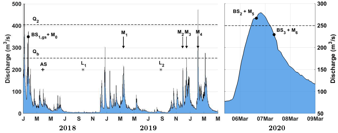
Figure 4.2: Monitoring framework related to the flow hydrograph of the Moselle river at the Châtel-sur-Moselle gauging station with a focus on the studied flood F . BS_n indicates the dates of bedload sampling with gs signifying that bedload samples were sieved, AS indicates the date of the installation of the acoustic monitoring station at the bridge, L_n indicates the dates of the LiDAR topo-bathymetric acquisition, M_n indicates the date of acoustic maps.
