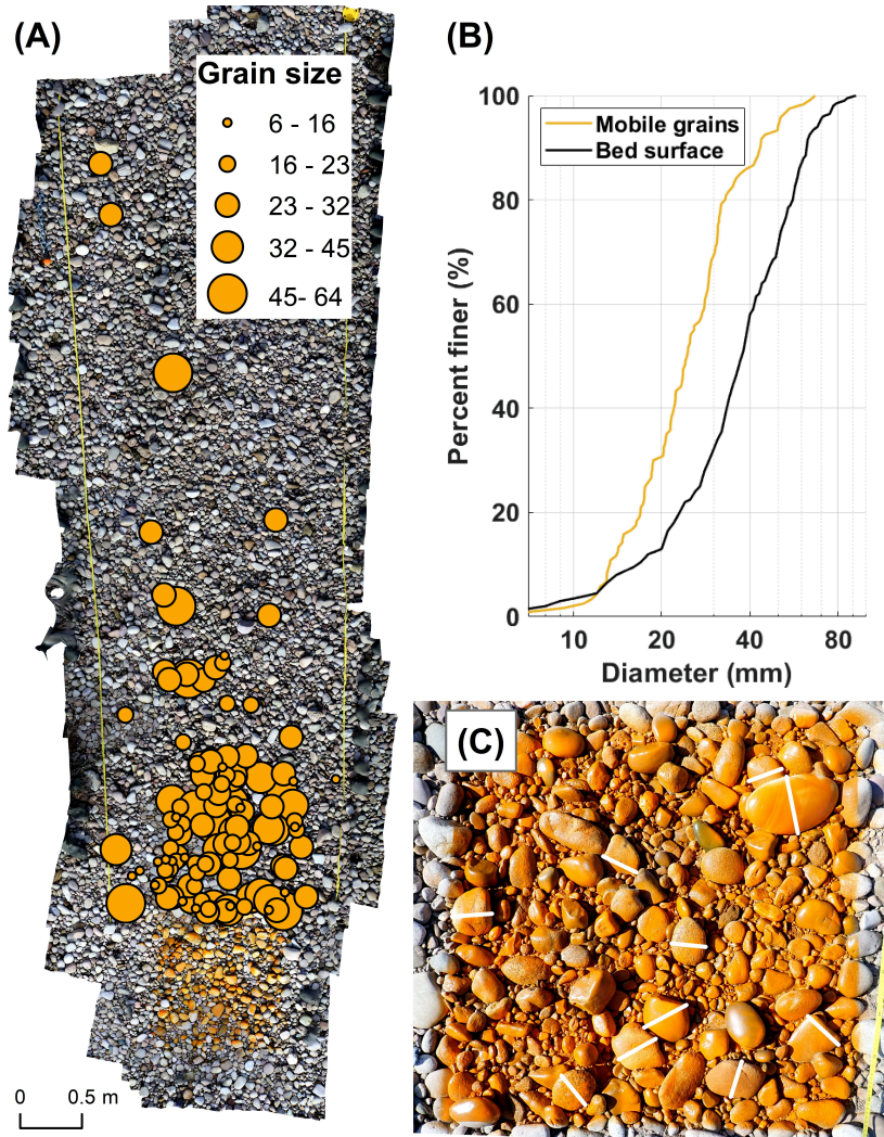
Figure 3.3: Example of (A) an orthophoto mosaic built from pictures taken at PP_6 during survey E_1 , when partial transport was observed. Orange circles indicate the diameters, measured on the orthophoto, of particles recovered out of the patch, (B) a cumulative frequency distribution of mobile particles size measured on the orthophoto and of particles measured in the field at riverbed surface, (C) picture showing a digitalization of the ten largest particle observed on the patch PP_1 set at PI .
