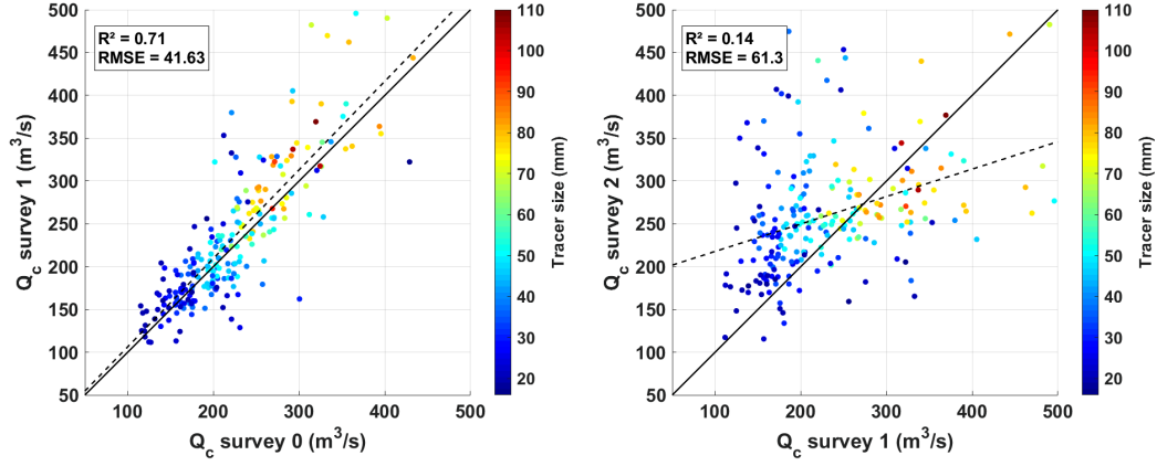
Figure 5.12: Comparison of the critical discharge for tracers motion between S_0 - S_1 (left plot) and S_1 - S_2 (right plot). The solid line corresponds to the 1:1 relationship and the dotted line represent the trendline based on our data.
