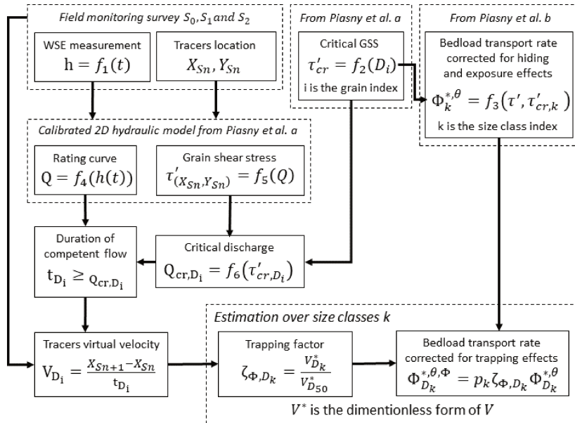
Figure 5.2: Flowchart of the main components of the method for calibrating the bedload transport composition for a 2D hydro-sedimentary model using complementary data on particle mobility and dynamics.
