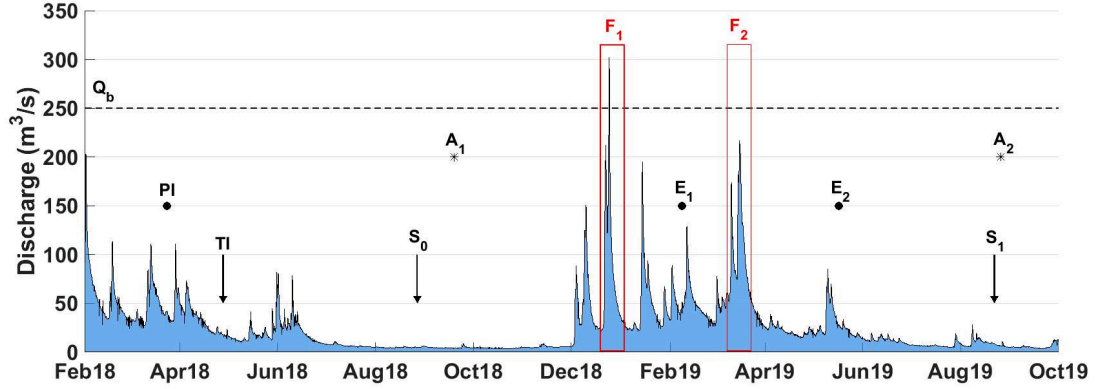
Figure 3.2: Monitoring framework related to the flow hydrograph of the Moselle river at the Châtel-sur-Moselle gauging station. A_n indicates the dates of the aerial topo-bathymetric acquisitions, E_n indicates the dates of the painted bed patches surveys, PI indicates the patches installation and TI the tracers injection, F_n indicates the floods for which the flow competence is estimated and S_n indicates the dates of the tracer surveys.
