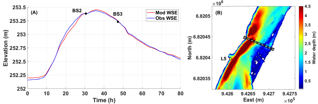
Figure 4.6: (A) Comparison between the WSE recorded by the limnimeter located upstream of the bridge (yellow point in B) and the WSE modeled during the studied flood F from unsteady simulations performed with the submodel \mathcal{M}_{f,s} (B) Map of the water depth predicted at steady state ( Q = 268m^3/s ) by the submodel \mathcal{M}_{f,s} during the bedload sampling campaign BS_2 .
