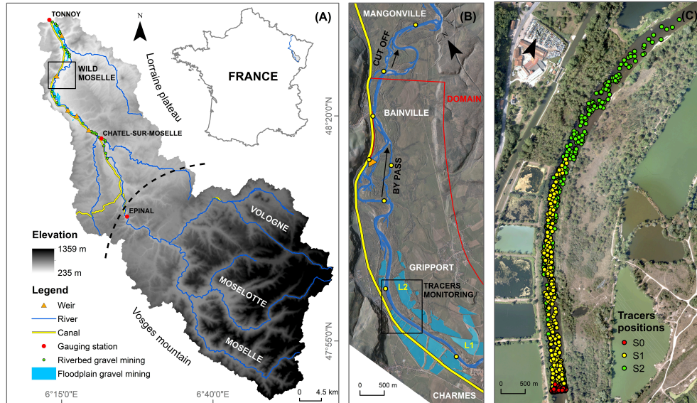
Figure 5.1: Study site (A) location of the “Wild Moselle river” in the Moselle Basin, (B) longitudinal extension of the 2D hydro-sedimentary model \mathcal{M}_{f,p} (C) position of tracers over time.
