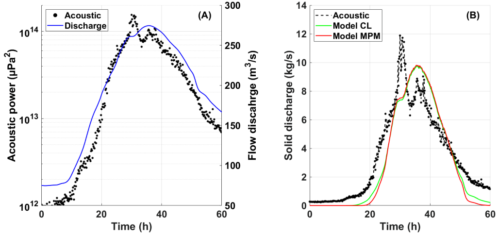
Figure 4.10: Comparison between chronicles of (A) acoustic power and flow discharge and (B) bedload fluxes estimated using acoustic measurements and numerical simulations during the studied flood F of March 2020.
