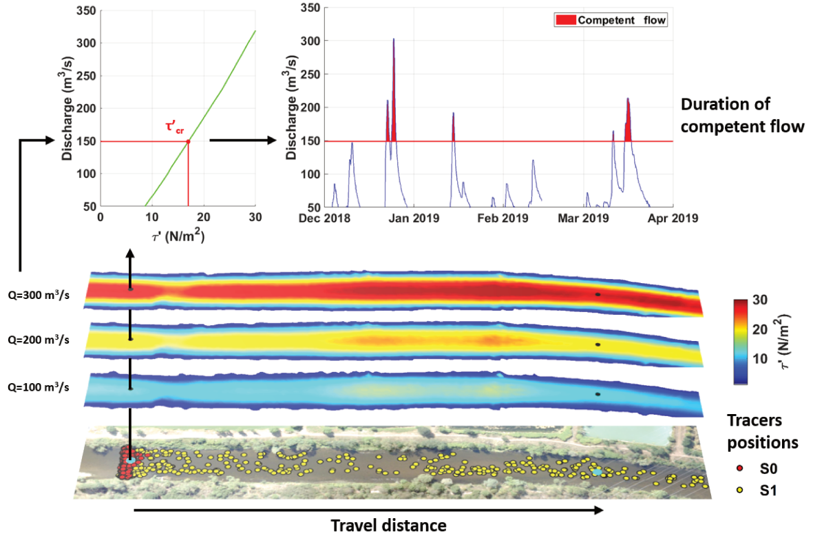
Figure 5.5: Flowchart of the methods employed to estimate the distances traveled by the tracers and the duration of the flow competent to transport these tracers. These methods are based on the results of field surveys ( S_n ) and of the catalog of 2D hydro-sedimentary model outputs for different inflow discharge.
