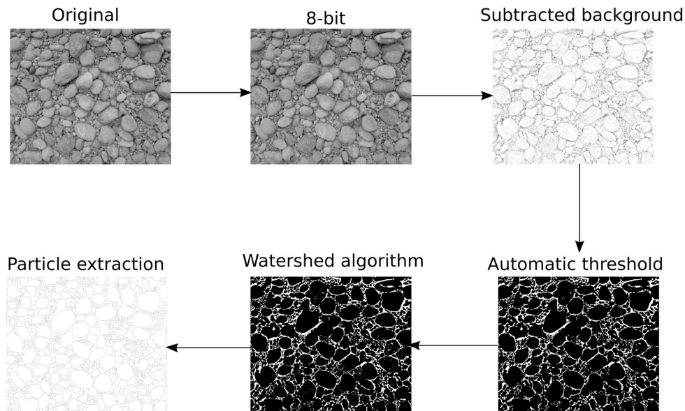
FIGURE 4 Example of image processing by the ImageJ software package, based on the protocol developed by Sulaiman et al. (2014)
