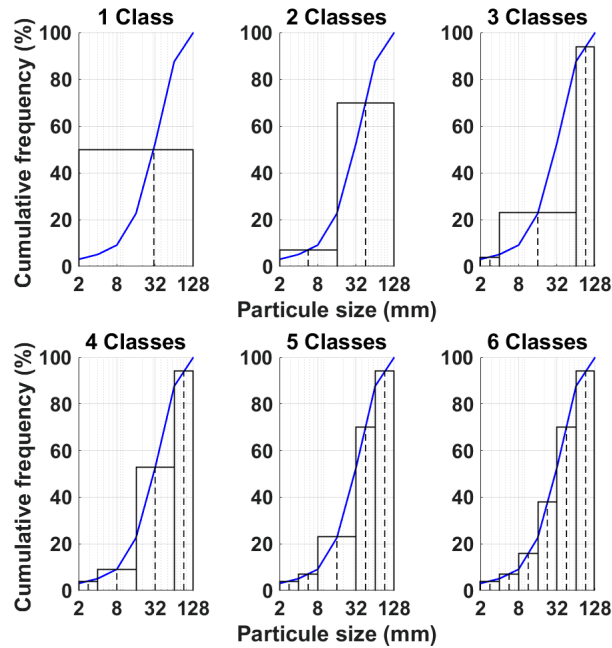
Figure 5.7: Discretization of the granulometric curve of the bed surface material into different numbers of size classes with corresponding representative diameters. This curve was determined from Wolman pebble counts performed along the injection reach.
