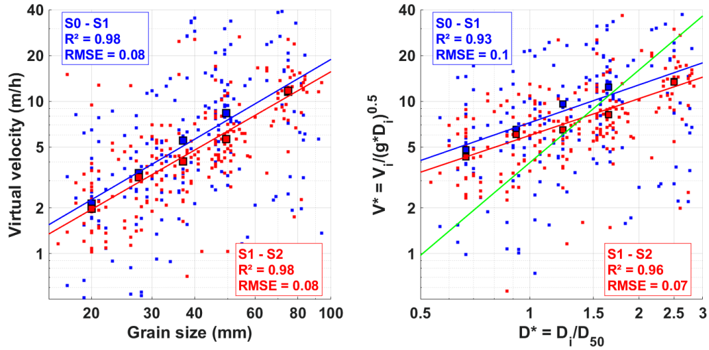
Figure 5.14: Virtual velocity of tracers as a function to their size during each period P_n (left plot) and dimensionless virtual velocity of tracers as a function to their relative size during each period P_n (right plot). Large squares indicates the median velocity as a function of the median size of tracers within each size class and green line represents the results obtained by Milan (2013).
