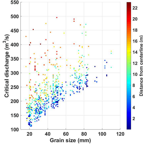
Figure 5.11: Critical discharge for tracers motion as a function to the tracers size and lateral position according to the river centerline.
