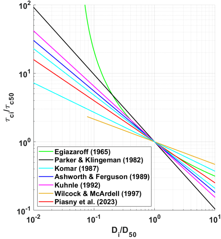
Figure 3.7: Comparison of different hiding functions : in all studies \theta_{ci} = \theta_{cr} \left( \frac{D_i}{D_r} \right)^{-b} with b \in [0.33; 0.98] except in Egiazaroff (1965) where \theta_{ci} = \left( \log(19) / \log(19 \frac{D_i}{D_r}) \right)^2 .
