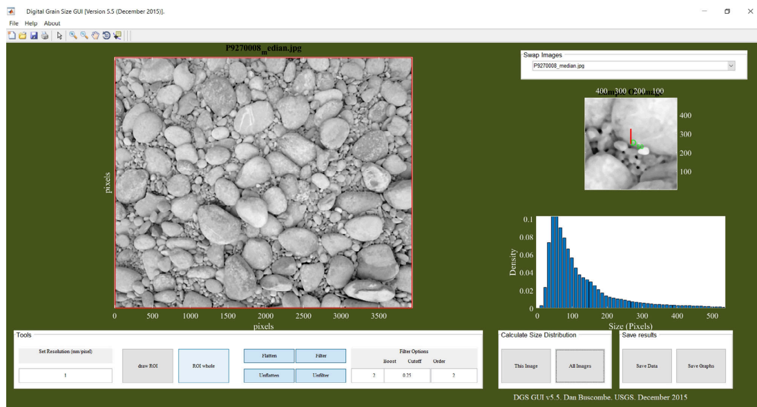
FIGURE 2 Example of image processing by the digital grain size (DGS) software package developed by Buscombe (2013) [Color figure can be viewed at wileyonlinelibrary.com ]
