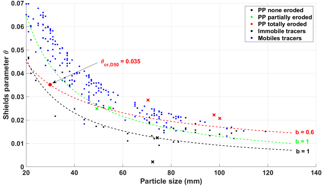
Figure 3.6: Shields parameter computed (equation 3.1) based on (i) the maximum grain shear stress modelled at each painted patch (denoted PP) or tracer location and to (ii) the size of the studied particles, whether they are mobile or immobile. The green dashed line represents an extrapolation of the critical Shields parameter estimated from partially eroded patches, assuming equal mobility ( b = 1 ). The black dashed line represents an extrapolation of the Shields parameter estimated from uneroded patches, assuming equal mobility ( b = 1 ). The red dashed line represents an extrapolation of the critical Shields parameter estimated from partially eroded patches, assuming size-selective transport ( b = 0.6 )
