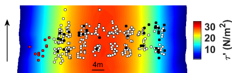
Figure 3.4: Grain shear stress \tau' modelled at the peak of the flood F_1 ( Q = 303m^3/s ) over tracers injection site. Points indicate mobile (white), immobile (black), and excluded (red) tracers.
