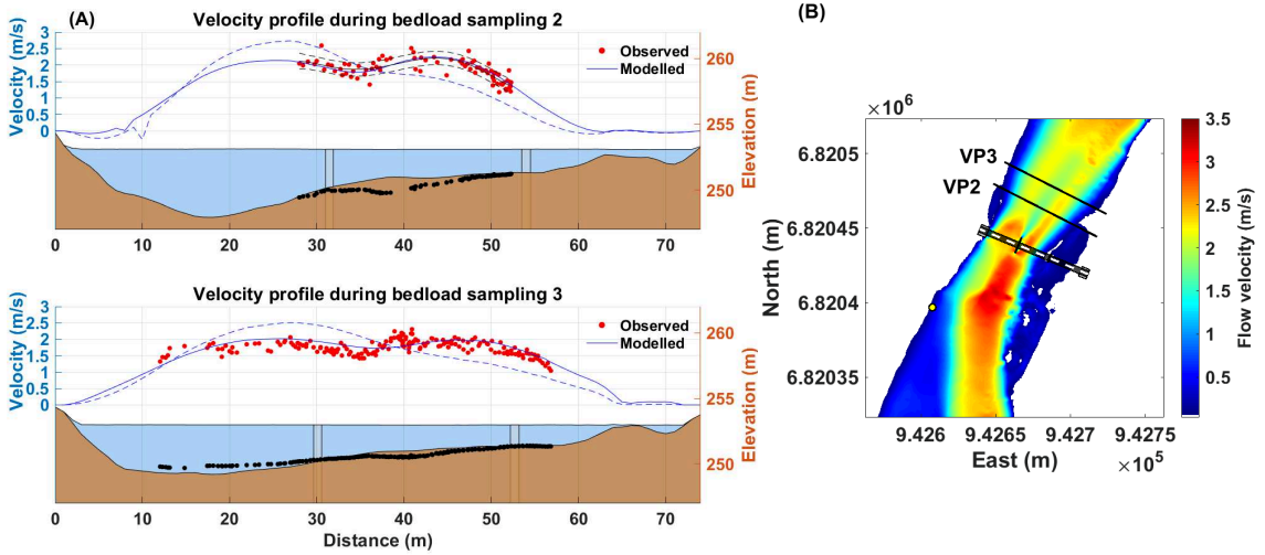
Figure 4.7: (A) Comparison between observed (red points) and modeled depth-averaged flow velocities, during the bedload sampling BS_2 ( Q = 268m^3/s ) and BS_3 ( Q = 233m^3/s ), before (solid blue line) and after (dashed blue line) calibration of the friction coefficient. (B) Map of the depth-averaged flow velocities predicted at steady state ( Q = 268m^3/s ) by the model \mathcal{M}_{f,s} during the bedload sampling campaign BS_2 .
