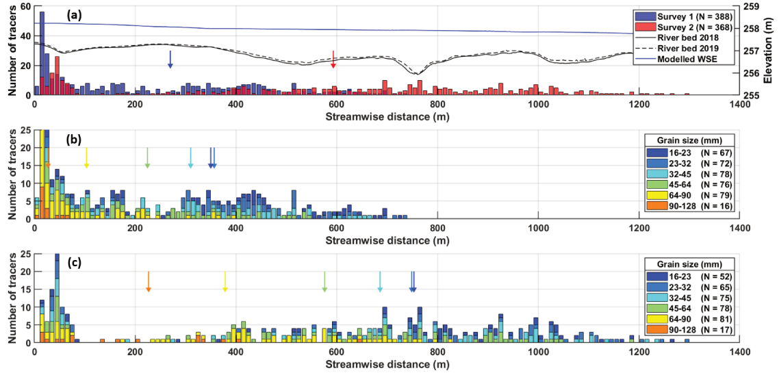
Figure 5.8: Longitudinal distribution of (a) all tracers recovered at S_n and the longitudinal profile of the river bed extracted at the centerline from the DEM of 2018 and 2019 with the water surface elevation modelled at Q = 40m^3/s using the DEM of 2018, (b) all tracers recovered at S_1 and (c) all tracers recovered at S_2 . Arrows indicate the mean distance traveled by all mobile tracers recovered at S_n - S_{n+1} in (a), the mean distance traveled by each size class k , based on mobile tracers recovered at S_0 - S_1 in (b) and at S_1 - S_2 in (c).
