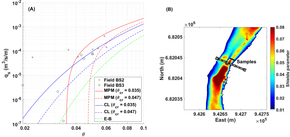
Figure 4.8: (A) Local bedload transport measured during sampling BS_2 and BS_3 as a function of the local Shields parameter modelled at steady state for the corresponding discharge using \mathcal{M}_{f,s} (MPM : Meyer-Peter & Müller laws, CL : Camenen & Larson laws, E-B : Einstein-Brown laws) (B) Map of the Shields parameter predicted at steady state ( Q = 268 \text{ m}^3/\text{s} ) by the model \mathcal{M}_{f,s} during the bedload sampling campaign BS_2 .
