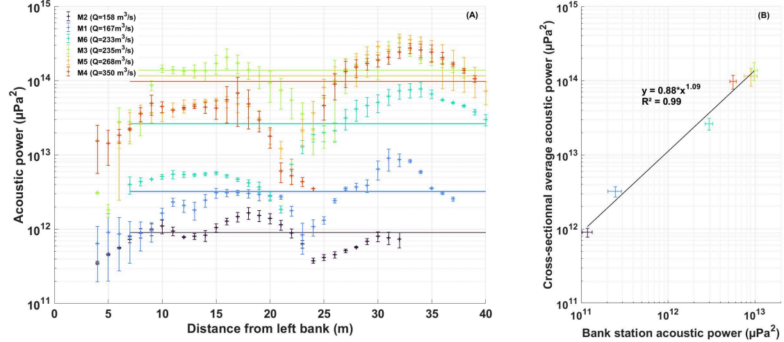
Figure 4.5: (A) Results of acoustics maps performed at different discharge and (B) relationship between bank and cross-section averaged measurements
