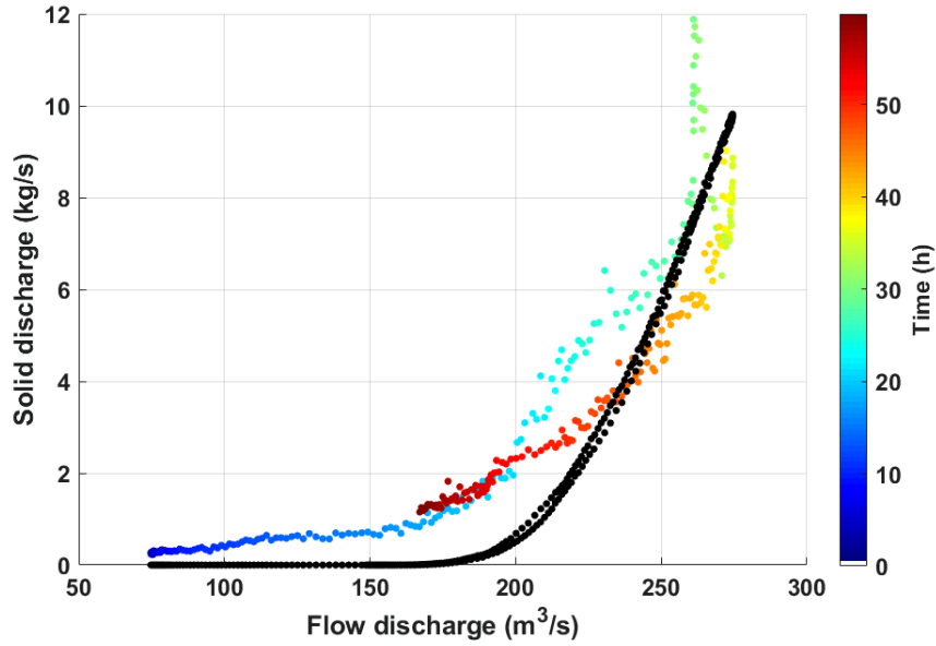
Figure 4.11: Comparison between observed (colored points) and modeled (black points using MPM law) bedload hysteresis during the studied flood F of March 2020.
