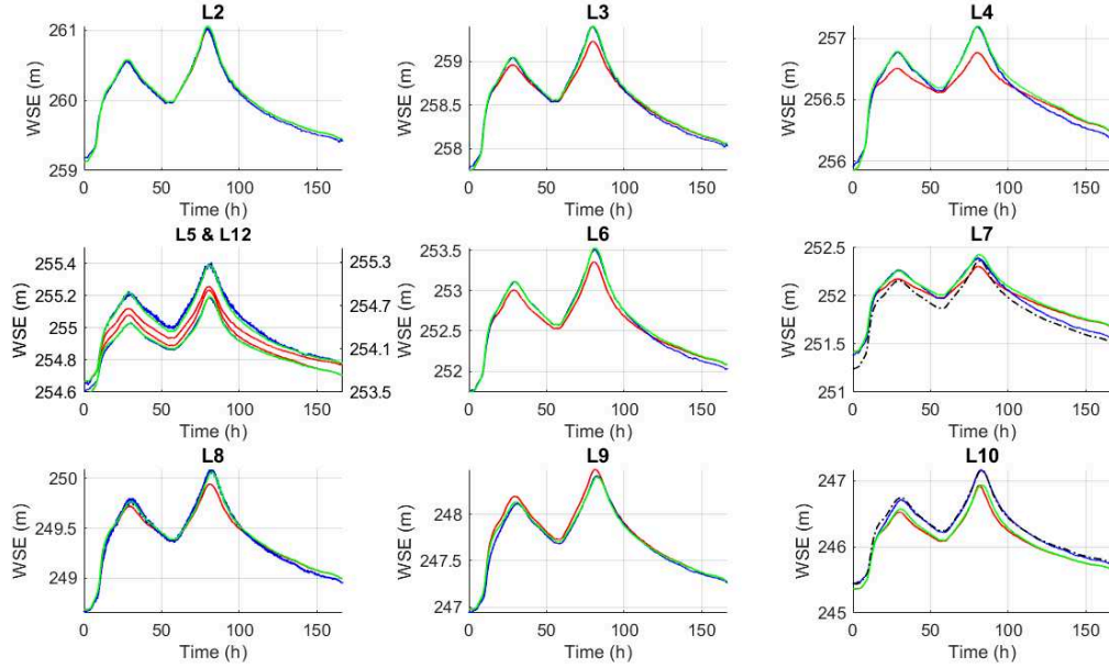
Figure 3.5: Comparison between observed and modelled WSE during the flood event F_1 (discharges ranging from 40 to 303\text{m}^3/\text{s} ). Blue solid line indicate the WSE recorded by the limnimeter L_n distributed along the Moselle river (Figure 3.1 D). Red and green solid line indicates the WSE modelled using the DEM of 2018, with a Strickler coefficient in the floodplain of 47\text{m}^{1/3}/\text{s} and 8\text{m}^{1/3}/\text{s} , respectively. Dashed black line indicates, at L7 and L10, the WSE modelled using the DEM of 2019 with a Strickler coefficient in the floodplain of 8\text{m}^{1/3}/\text{s} .
