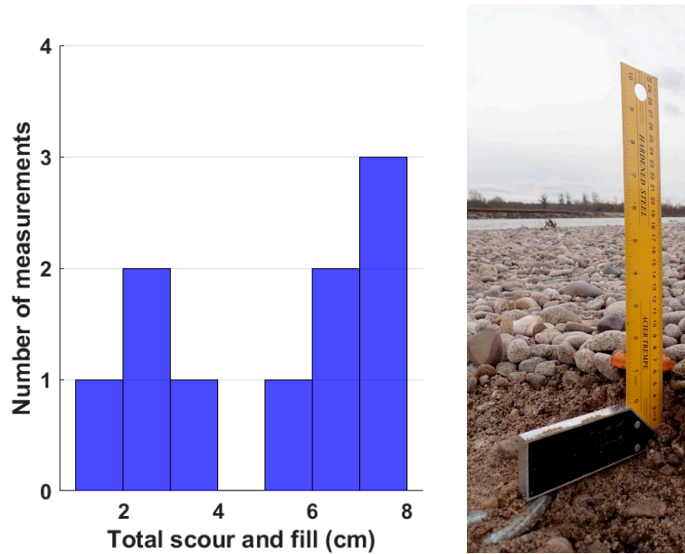
Figure 5.6: Distribution of total scour and fill measured during 3 flow events ( Q_{max} = 303m^3/s ; 214m^3/s and 254m^3/s ) by 20 chains ( n_{tot} = 60 ) installed across the river at 6 easily accessible emerged gravel bars of the Moselle river (left). Results excludes cases of (i) no morphological evolutions ( n = 29 ), (ii) river incision ( n = 3 ), (iii) lost chains ( n = 4 ) and (iv) stolen chains ( n = 14 ). Measurement of total scour and fill using a scour chain (right).
