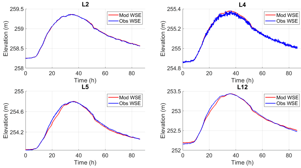
Figure 4.12: Comparison between the WSE recorded by limnimeter L_n and the WSE modeled during the studied flood F from unsteady simulations performed with the submodel \mathcal{M}_{f,h} .
