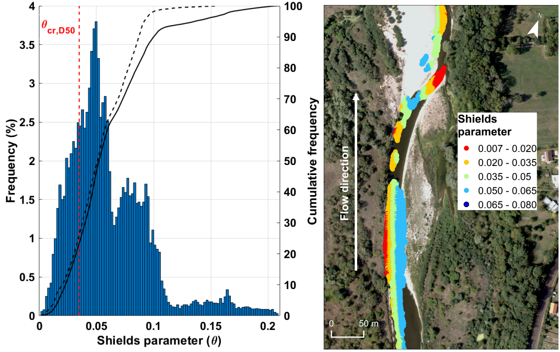
Figure 3.8: Statistical distribution of the Shields parameter computed over all areas eroded ( \Delta Z \leq -10cm ) between LiDAR surveys A_1 and A_2 , compared to the critical Shields parameter estimated in this study \theta_{cr} := 0.035 . An example of the spatial distribution of the maximum Shields parameter modeled over eroded areas distributed along a reach located at the downstream part of the study site.
