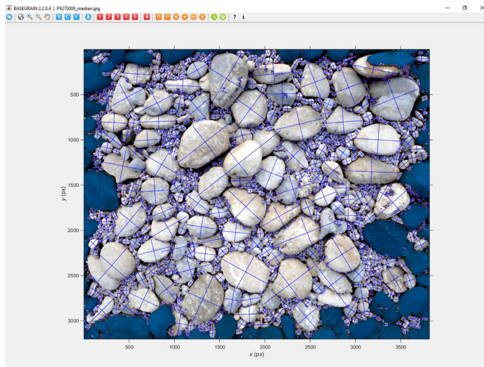
FIGURE 3 Example of image processing by the Basegrain software package developed by Detert and Weitbrecht (2012) [Color figure can be viewed at wileyonlinelibrary.com ]
