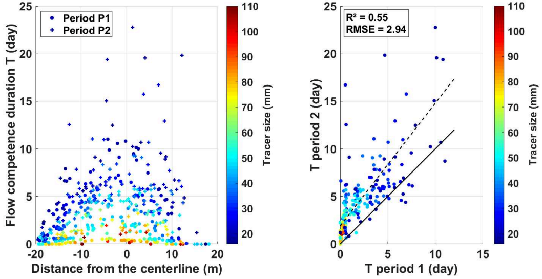
Figure 5.13: Duration of competent flow as a function to the tracer lateral position and size for each period P_n (left plot) and comparison of the flow competence duration between periods P_1 - P_2 (right plot). The solid line corresponds to the 1:1 relationship and the dotted line represents the trendline based on our data.
