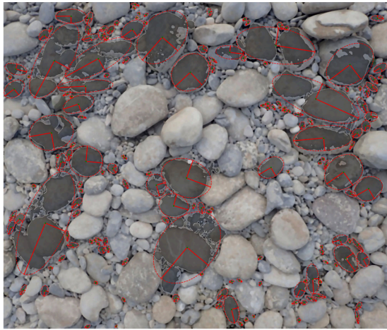
FIGURE 5 Example of image processing by the PebbleCounts software package developed by Purinton and Bookhagen (2019) [Color figure can be viewed at wileyonlinelibrary.com ]
