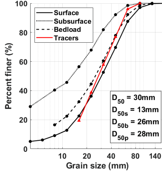
Figure 5.3: Cumulative grain size distribution of (i) the bed surface material, estimated from 6 samples collected along the reach of injection by grid-by-number pebble counts ( n_{tot} = 1200 ), (ii) the bed subsurface material, estimated from a volumetric sample collected on a bar located in the middle of the study area ( m_{tot} = 346\text{kg} ), (iii) the bedload material, estimated from bedload samples collected in the middle of the study area during a flood of bankfull discharge using a Helley-Smith sampler ( m_{tot} = 245\text{kg/s} ) and (iv) the injected pit-tags ( n = 450 ) with corresponding median diameter of the bed surface ( D_{50} ), the bed subsurface ( D_{50s} ), the bedload ( D_{50b} ), the pit-tags ( D_{50p} ).
