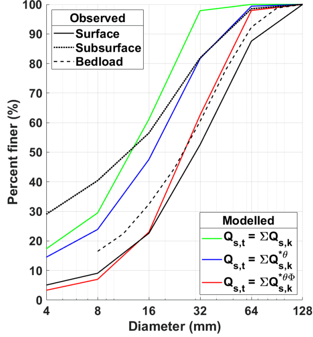
Figure 5.15: Comparison of the grain size distribution of the observed bedload and modelled bedload using 6 size classes, without a correction factor ( Q_{s,k} ), with a corrector factor \zeta_{\theta} for hiding-exposure effects ( Q_{s,k}^{\theta} ) and with a correction factor for hiding-exposure effects \zeta_{\theta} and a correction factor \zeta_{\Phi} for trapping effects ( Q_{s,k}^{\theta,\Phi} ).
