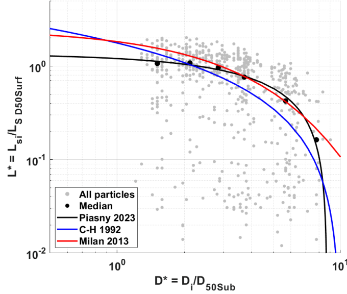
Figure 5.9: Relative travel distances of all tracers recovered during S_n - S_{n+1} as a function to their relative size and median relative travel distances of tracers contained in each size class as a function of the median relative size of those tracers contained in each size class. Polynomial curve fitted to our median value compared to the curve found by Church and Hassan (1992) (noted C-H) and Milan (2013).
