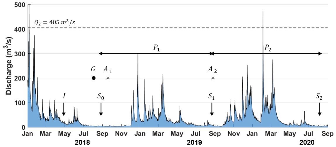
Figure 5.4: Monitoring framework related to the flow hydrograph of the Moselle river at the Châtel-sur-Moselle gauging station. A_n indicates the dates of aerial topo-bathymetric acquisitions, G indicates the date of surface and subsurface material grain size measurements, I indicates the date of tracer injection, S_n indicates the dates of tracer surveys and P_n is the monitoring periods between two tracer surveys.
