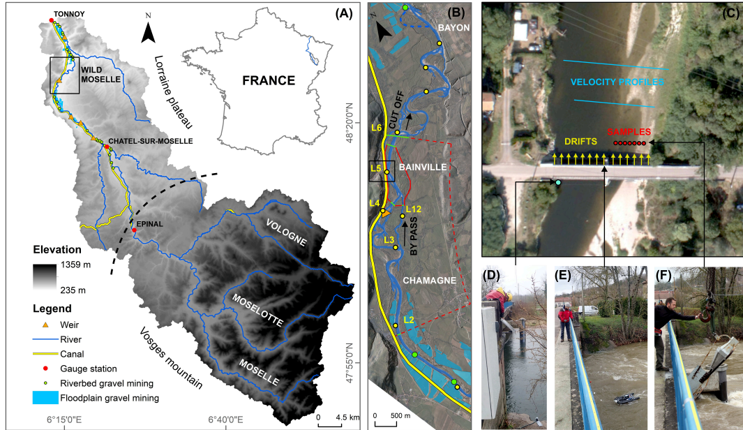
Figure 4.1: (A) location of the “Wild Moselle river” in the Moselle Basin, (B) longitudinal extension of the 2D hydraulic model \mathcal{M}_{f,h} (red dashed line) and the 2D hydro-sedimentary model \mathcal{M}_{f,s} (red solid line) into the natural regional reserve (C) area of bedload fluxes measurement and modelling, velocity and acoustic measurements, (D) hydrophone fixed at the left bank, (E) acoustic mapping, (F) bedload sampling.
