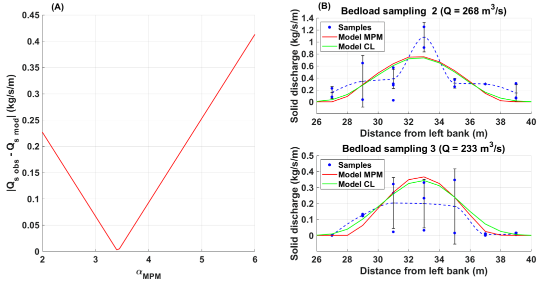
Figure 4.9: (A) Calibration of \alpha_{MPM} and (B) Comparison between observed and predicted cross-sectional bedload transport rates during bedload sampling campaigns BS_2 and BS_3 .
