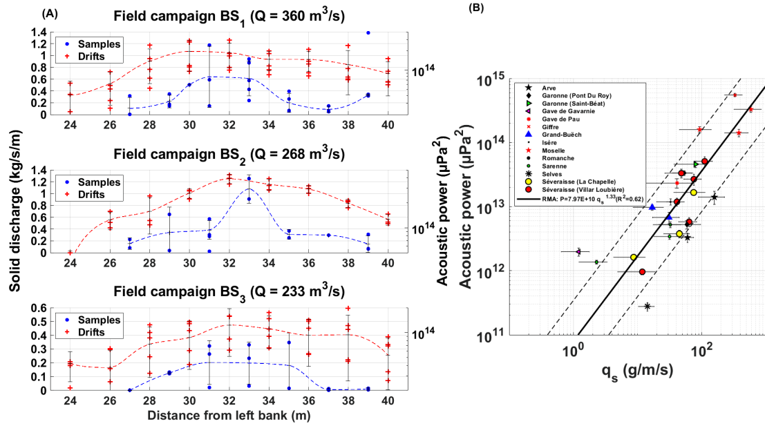
Figure 4.4: (A) Cross-sectional profiles of bedload flux (samples) and acoustic power (drifts) monitored at each field campaign. (B) Relationship between cross-sectional averaged values of acoustic power and specific bedload flux integrated into the model proposed by Geay et al. (2020)
