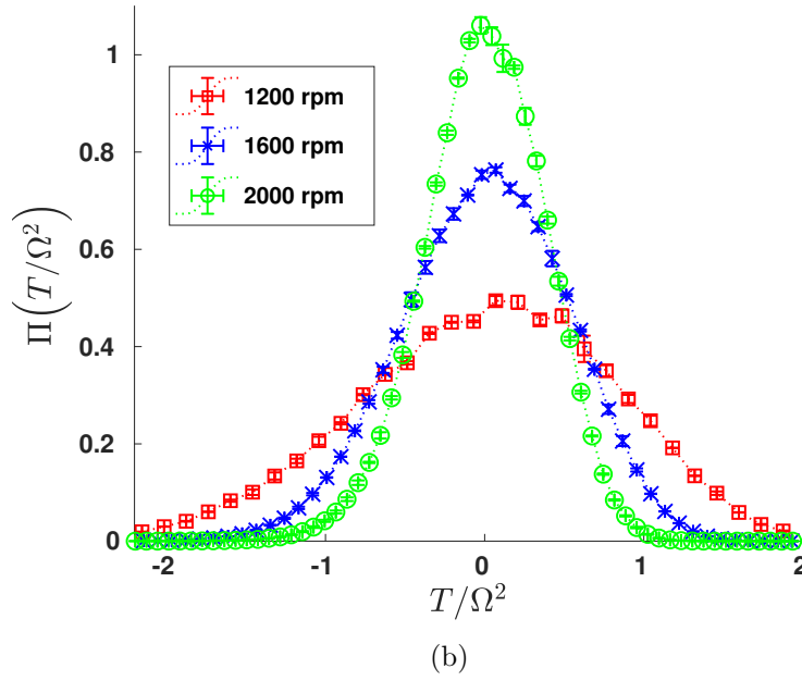
Fig. II.11 (a) PDF of temperature fluctuations normalized by T_{rms} . Exponential tails in PDF for negative fluctuations are observed. The negative exponential tails do not coincide on normalization. (b) PDF of temperature fluctuations normalized by large scale scaling \Omega^2 . Red squares: 1200 rpm; Blue crosses: 1600 rpm; Green circles: 2000 rpm.
