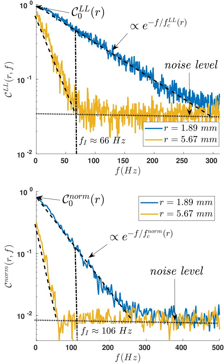
Fig. III.30 Coherence of velocity fluctuations when the rotation rate of the motors is \Omega = 3200 rpm (a) For longitudinal component, denoted by \mathcal{C}^{LL} . (b) For the norm, denoted by \mathcal{C}^{norm} .
