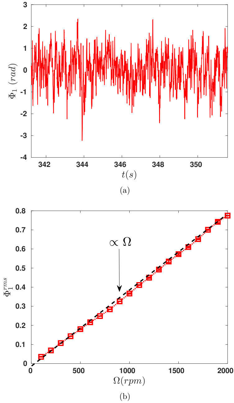
Fig. IV.8 (a) Time series of phase fluctuations for \Omega = 2000\text{rpm} . (b) Scaling of RMS of phase fluctuations \Phi_1^{rms} with the rotation rate \Omega . Dashed line shows the predicted linear scaling.
