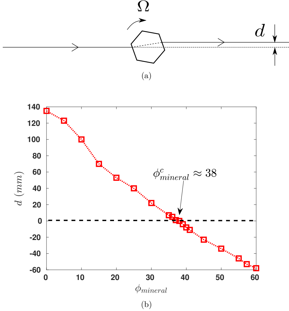
Fig. III.19 (a) Sketch showing the incident beam being deflected by a distance ' d ' by the rotating hexagonal axis. When the incident beam is perpendicular to the faces of the axis or when it falls on the vertices of the hexagonal axis, it is not deflected. (b) Plot showing the maximum distance of deflection ' d ' of the incident laser beam versus the volume fraction of mineral oil \phi_{mineral} . The volume fraction of mineral oil at which we obtain matching of refractive indices is denoted by \phi_{mineral}^c .
