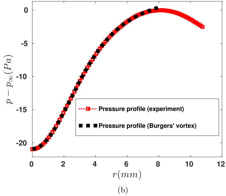
Fig. II.17 (a) Temperature profile obtained from coherent averaging (red) and a fit for the pressure profile of weakly compressible adiabatic Burgers vortex solution (dashed line) (eqn.(II.39)). (b) Pressure profile obtained from coherent averaging (red) and a fit for the pressure profile of weakly compressible adiabatic Burgers vortex solution (dashed line) (eqn.(II.37)). We have used r = u'_{rms}t to transform time to space co-ordinate. The rotation rate is \Omega = 2000 rpm.
