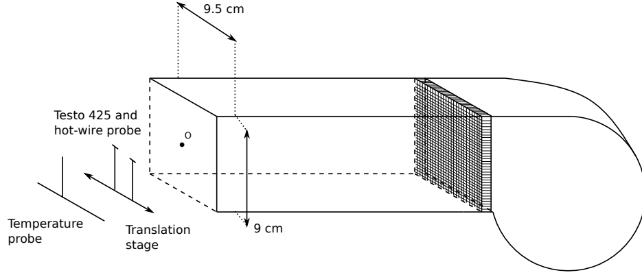
Fig. A.1 Sketch of the calibration setup.
