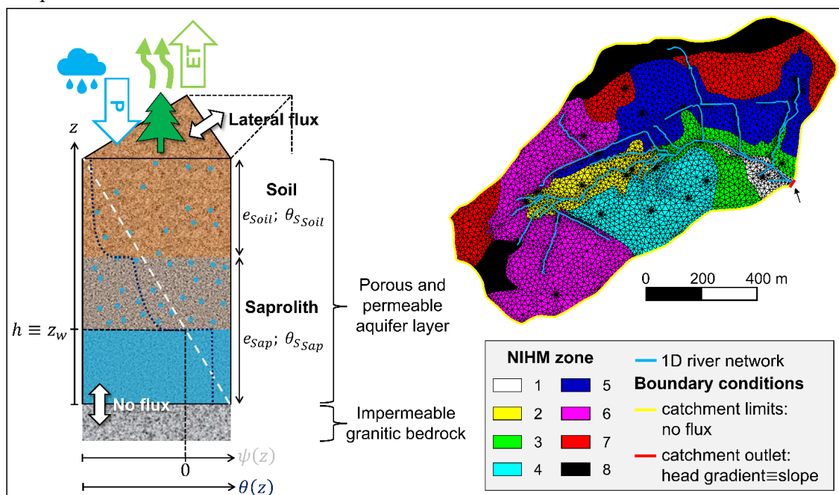
Figure 4.15. Schematic diagram of the NIHM hydrological model. Left: vertical view showing the vertical parameterization of the NIHM model and the water content distribution in a cell, z_w referring to the aquifer level. Right: Horizontal view showing the parametrization of NIHM in 8 hydrological zones.
