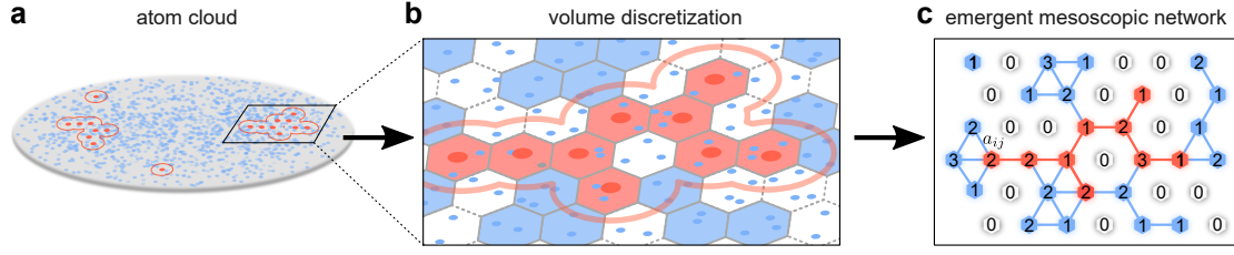
Fig. 5.3: Emergent heterogeneous Rydberg network. a To describe the excitation dynamics in the atom cloud a susceptible-infected-susceptible (SIS) model is developed on a heterogeneous network that emerges from the atom cloud. b Coarse graining of the system into hexagonal cells, which allows for the densest possible tiling in two dimensions. Each cell i contains either zero ( I_i = 0 , healthy, blue or white shading) or one ( I_i = 1 , infected, red shading) Rydberg excitations (red disks). Additionally, cells with at least one ground state atom (blue disks) that fulfills the facilitation conditions N_i \geq 1 can potentially be excited over time (susceptible, blue shading). Empty cells with N_i = 0 have zero excitation probability (white shading). c The coarse-grained cells are translated into network nodes, where the hexagonal cell structure with six nearest neighbors translates into a corresponding triangular network structure defined by the adjacency matrix a_{ij} . The infection probability of each node is weighted by the number of atoms in that cell that can undergo facilitated excitation N_i (shown in each node). Accordingly, vacant cells ( N_i = 0 ) translate into disconnected nodes that do not participate in the excitation dynamics. This results in a weighted, heterogeneous emergent network structure (see text for more details).
