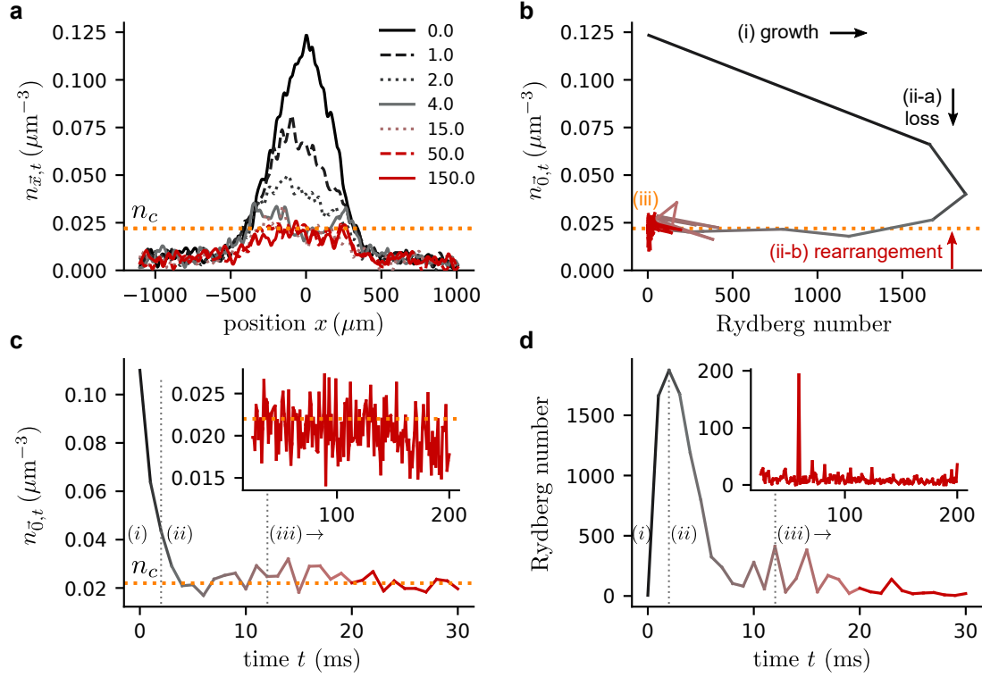
Fig. 4.7: Evolution of the spatial density profile during SOC dynamics in the dipole trap. a Atom density n_{x,t} cross section through the center of the cloud after Rydberg laser exposure times of 0, 1, 2, 4, 15, 50 and 150 ms (see labels). Initially at t = 0 ms (black line), we observe an approximately Gaussian density profile as expected for the thermal cloud in the dipole trap. Fast loss in the center of the cloud results in a dip after t = 4 ms (gray line). For later times, the density profile shows a flat top at the critical density n_c (orange dotted line) while at the same time the width of the cloud reduces. The three-dimensional density was reconstructed using an inverse Abel transformation on absorption images (see text for more details). b Atom density in the center of the cloud against the corresponding cloud-integrated Rydberg excitation number during the SOC dynamics up to 200 ms. Initially, we start with a density n_{0,t} \approx 0.125 \mu\text{m}^{-3} and zero Rydberg excitations. Subsequently, we observe a growth of the Rydberg number (i) which comes with a reduction in the atom density (ii-a). Around the critical density n_c , we observe overshoots below as well as above due to the rearrangement of atoms in the trapping potential (ii-b). This mechanism sustains the system close to the critical point (iii) for extended periods. c Central atom density as a function of the laser excitation time t . After a fast initial loss, within the first 5 ms, down towards the critical density, we observe an increase in the density due to refilling in the range 10 – 20 ms, before it drops back down again after around 30 ms. At later times, the atom density stays quite constant around n_c from 25 up to 200 ms (see inset with same axes dimensions). d Corresponding number of Rydberg excitations in the atom cloud as a function of the laser excitation time t . The excitation number quickly rises within the first 2 ms before it drops due to the simultaneous reduction in the atom density. This is followed by a range of larger activity fluctuations (10 – 20 ms) which we attribute to fast refilling of atoms. At later times from 25 – 200 ms, the activity is small, but generally non-zero with fluctuations to higher numbers (see inset with same axes dimensions). Note that each time point corresponds to an individual run of the experiment.
