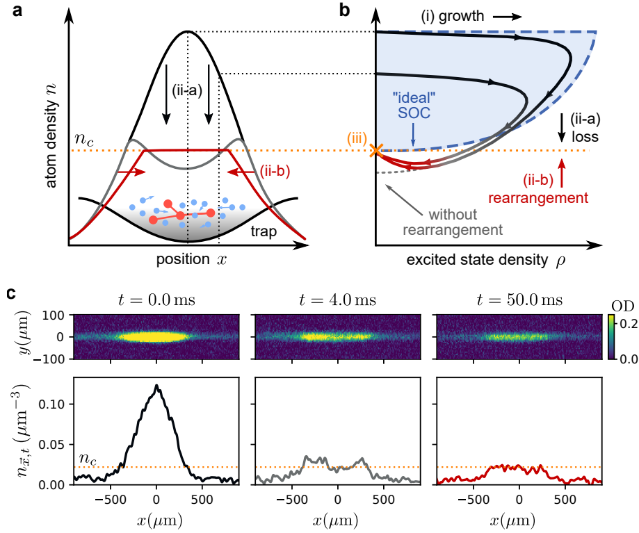
Fig. 4.6: Stabilization of the self-organized critical state induced by the trapping potential.
