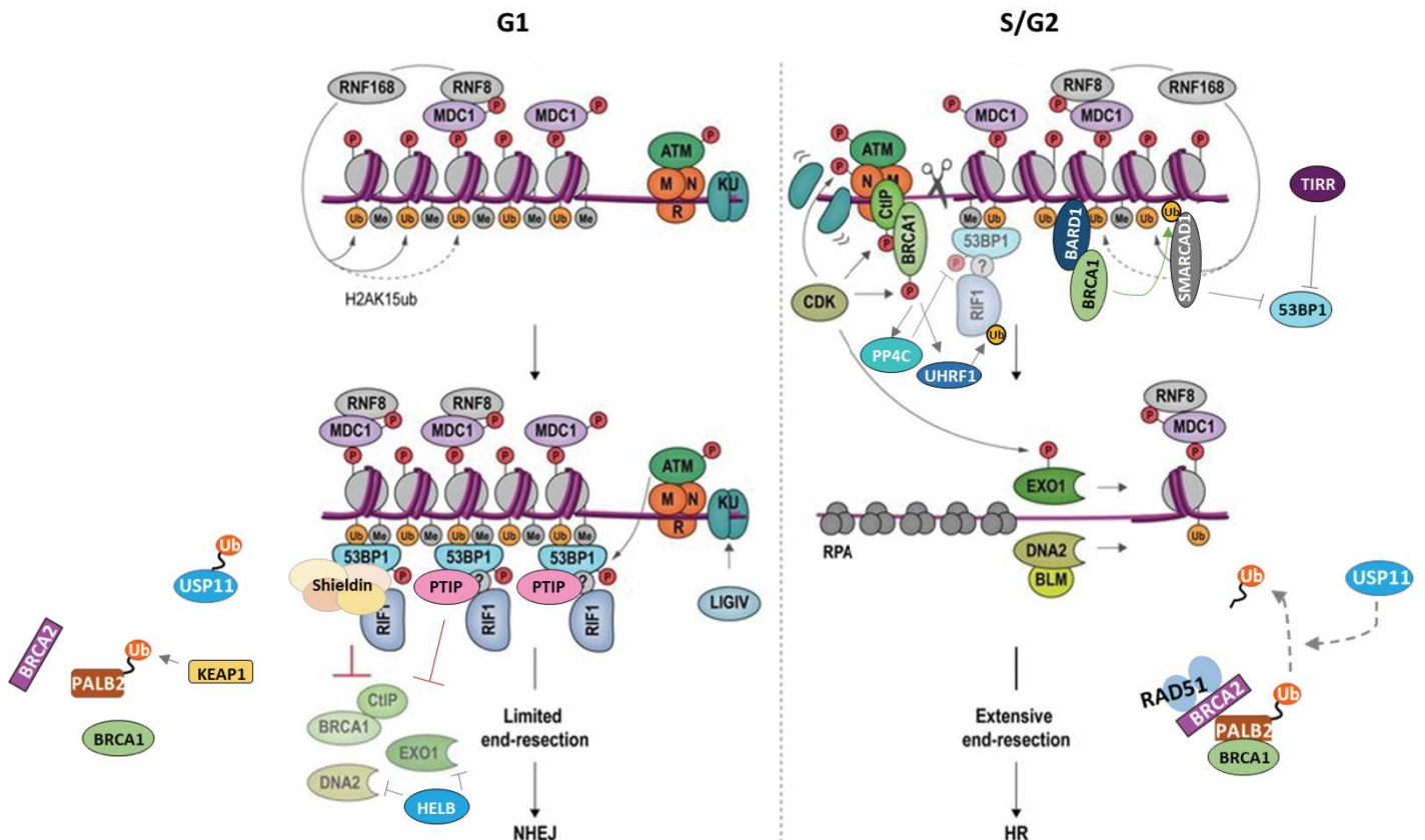
Figure 8: Role of BRCA1-53BP1 competition and cell cycle in regulating end resection
