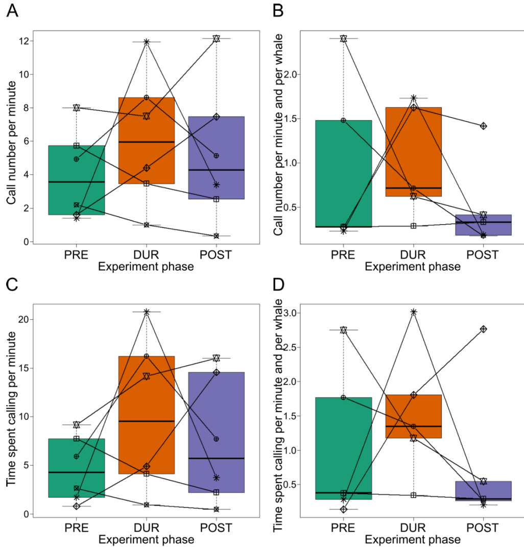
Figure 19: Vocal activity before, during, and after MEKW playbacks A and B) Number of annotated calling events C and D) Cumulative duration of annotated calling events. Left panels (A and C) were corrected for experiment phase duration. Right panels (B and D) were corrected for both experiment phase duration and average group size. Stars – gm13_137a; crossed diamonds – gm13_149a; + crossed circles – gm13_169a; double triangles – gm13_169b; crossed squares – gm14_180a; x crossed circles – gm14_180b
