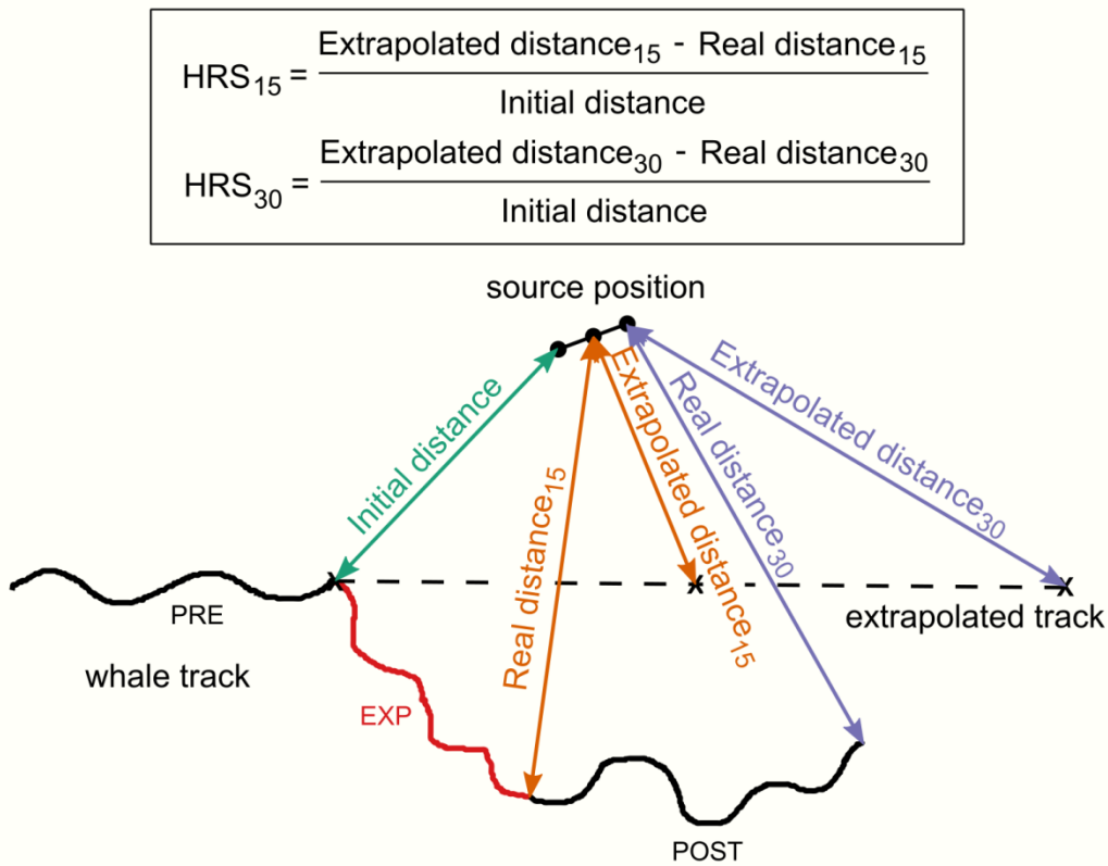
Figure 4: Horizontal reaction score (HRS) calculation. The HRS measures the difference in the distance between the whale and the sound source and the distance there would be between the whale and the sound source if the whale kept the same behaviour as right before the playback. We used the speed and heading of the whale during the pre-exposure phase to extrapolate its movement trajectory.
