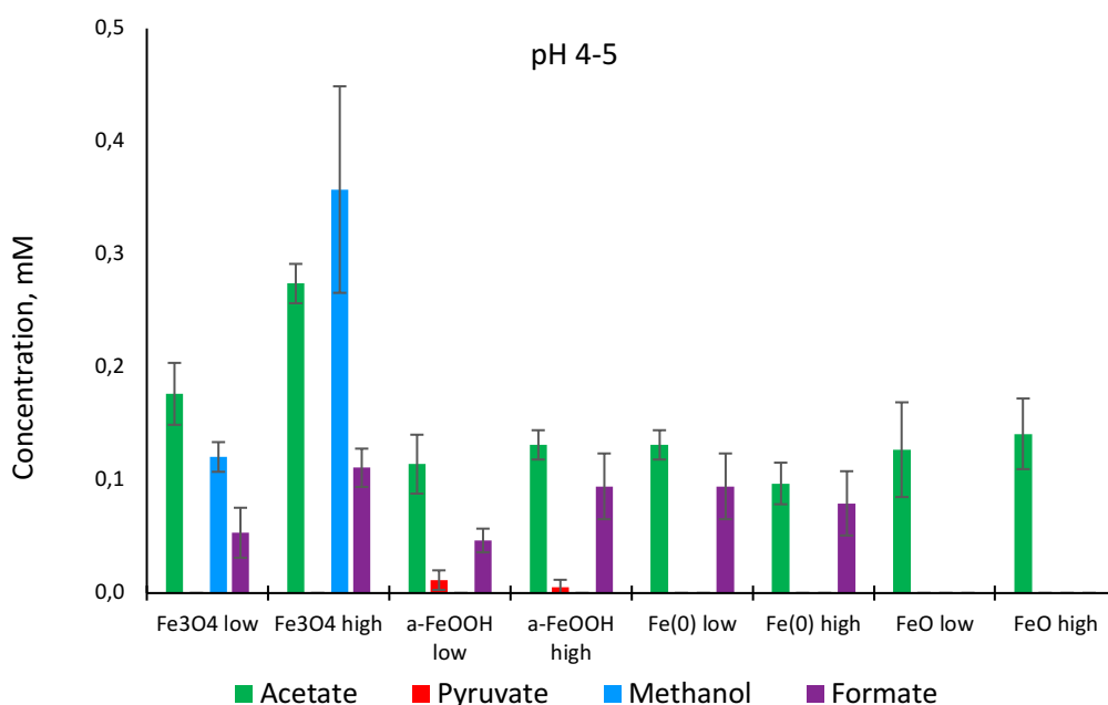
Fig 30. Concentrations of detected \text{CO}_2 reduction products obtained under \text{CO}_2/\text{H}_2 atmosphere (total pressure 25 bars) with iron oxide or metallic iron powder (low meaning 1 mmol of metal atoms, high meaning 3 mmol of metal atoms) in 1 mL \text{H}_2\text{O} each, at pH 4-5 at 100 °C for 16 hours.
