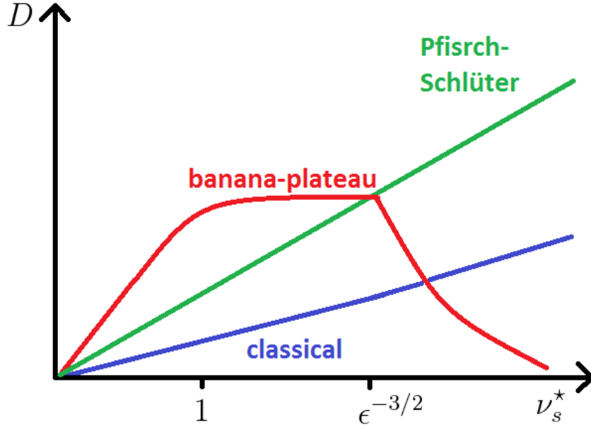
Figure 4.3.: Comparison between the classical prediction (blue), the banana-pateau contribution (red) and the Pfirsch-Schlüter contribution (green)
