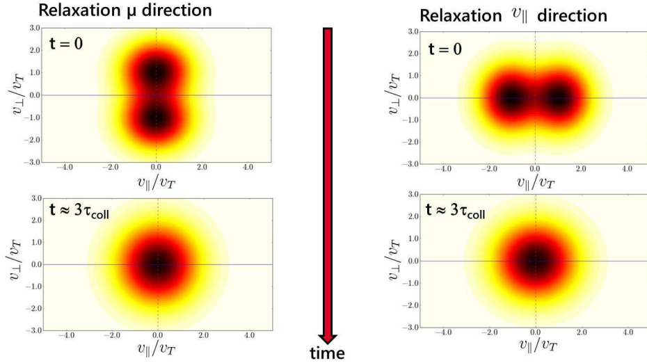
Figure 3.4.: Initial (top) and final (bottom) slices of the distribution function in velocity space are given. The initial distribution function is far from a Maxwellian in the v_{\perp} direction on the left and in the v_{\parallel} direction on the right. In both cases, the converged state is an isotropic Maxwellian.
