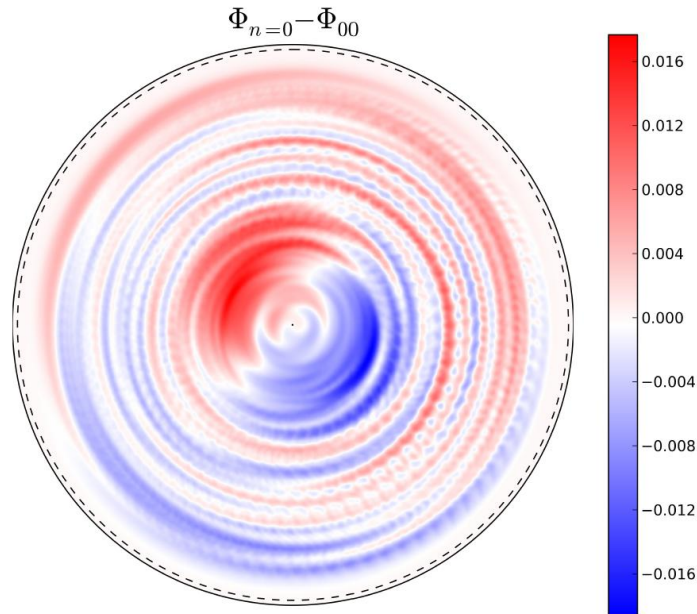
Figure 7.1.: Amplitude of the non zonal electric potential in the GYSELA simulation
