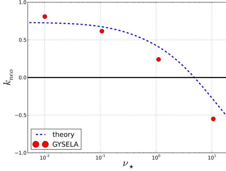
Figure 4.4.: k_{neo} = eB \frac{v_\theta}{\nabla T} versus \nu_\star predicted by theory (dashed line) compared with GYSELA results (red dots)
