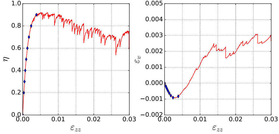
Figure 5.18 – Drained triaxial test response. The diamond points correspond to the mechanical states considered for the stability analysis.
