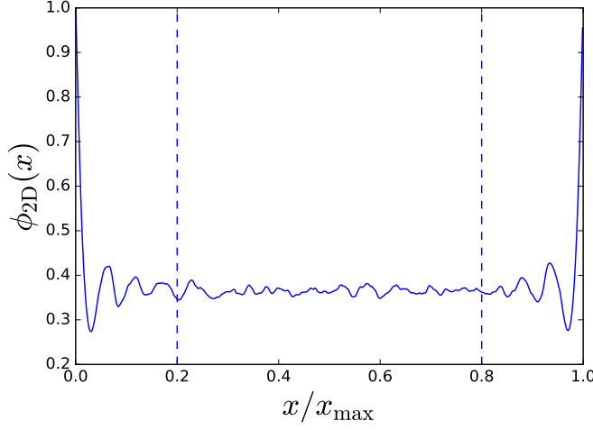
Figure 3.9 – 2D porosity \phi_{2D}(x) computed in the x direction for the dense sample in the initial isotropic state ( \varepsilon_{zz} = 0 ). The central zone of the sample used to compute spatial autocorrelation functions is shown by vertical dashed lines.
