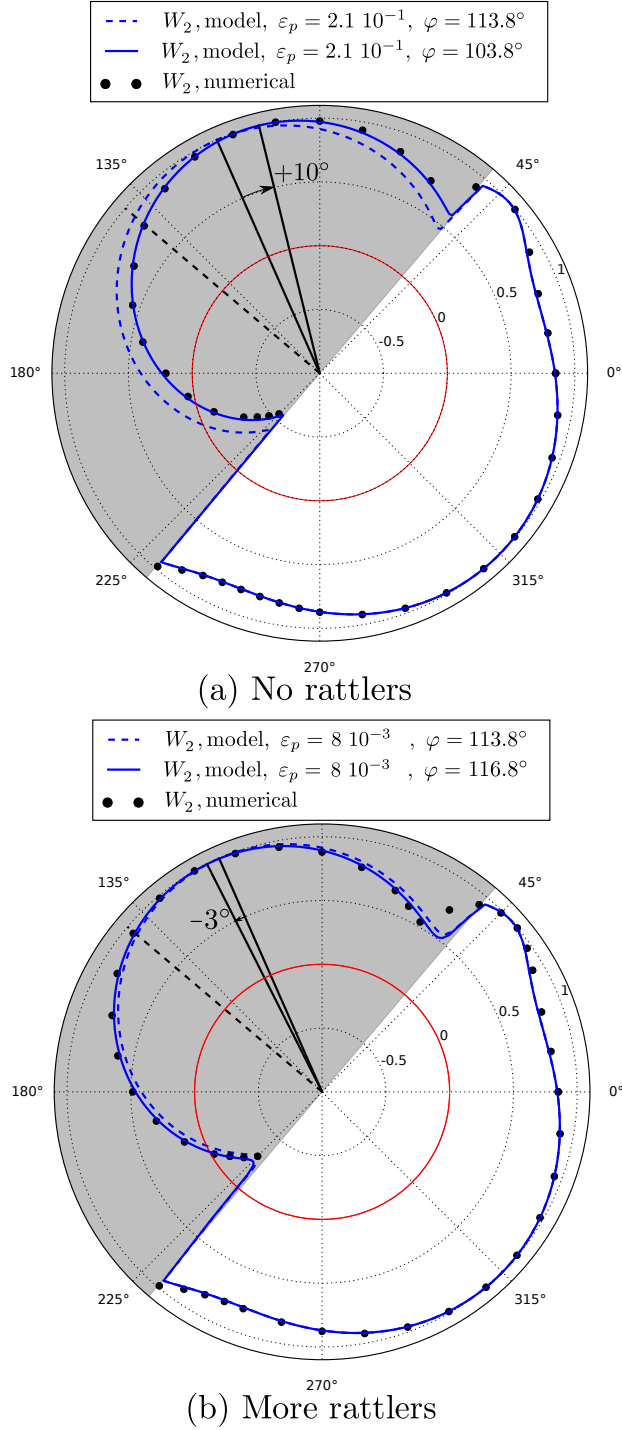
Figure 4.35 – Circular envelopes of normalized second-order work for \eta = 0.45 corresponding to the sample without rattlers (a) and in which additional rattlers are incorporated (b). The phenomenological fits coming from the elastoplastic model presented in Section 4.4.1 are shown with a dashed line with parameters from Table 4.1 and updated \varepsilon_p values, and as a solid line for the updated plastic parameters from Table 4.2. The maximum plastic intensity direction \varphi + \Delta\varphi (the black dashed line segment) and the plastic flow direction \varphi (two thick solid line) are also shown for both fits.
