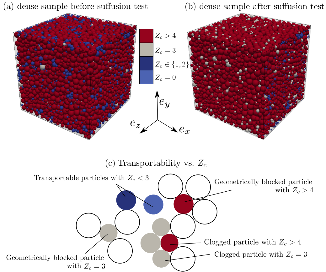
Figure 3.19 – Dense sample under isotropic confinement before (a) and after (b) the application of a hydraulic gradient I = 1 in direction \mathbf{e}_x . Particles are colored according to their coordination number Z_c in relation with their transportability (c).
