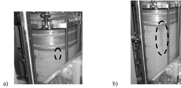
Figure 1.2 – Localization of erosion along the boundaries of erodimeter cells in laboratory tests (Sail et al., 2011).
