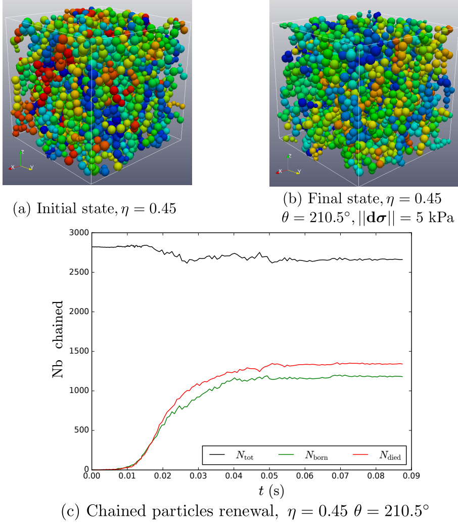
Figure 4.14 – Visualization of force chains identified in the initial (a) and final (b) configurations for a stress ratio \eta = 0.45 in an unstable direction \theta = 210.5^\circ for \|\mathbf{d}\boldsymbol{\sigma}\| = 5 \text{ kPa} . Force chains are composed of contacting particles of same color. (c) Time evolution of the number of chained particles (black), the number of new (green) and former (red) chained particles compared with the initial state.
