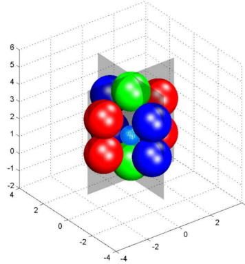
Figure 6.2 – A possible enriched version of the mesostructure of the 3D H-model (Xiong et al., 2017) with a central free particle.
