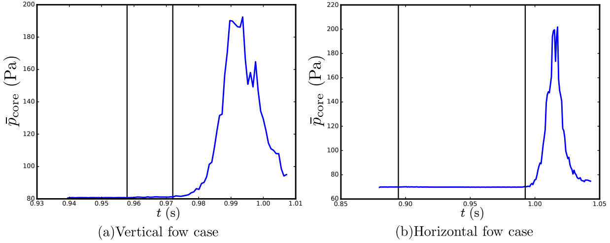
Figure 5.10 – Time evolution of the average pore pressure in the core of the sample for the two flow cases. The pore pressure is averaged over the domain [0.45\ell_x, 0.55\ell_x] \times [0.45\ell_y, 0.55\ell_y] \times [0.45\ell_z, 0.55\ell_z] where \ell_x , \ell_y and \ell_z are the sample dimensions. The onset of the two outbursts of kinetic energy visible in Figure 5.8 are shown with vertical solid lines.
