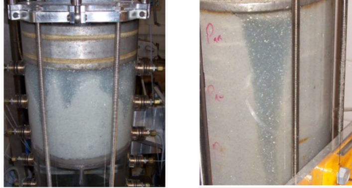
Figure 2.8 – Observation of microstructure heterogeneities in two experimental suffusion tests (Sibille et al., 2015b).
