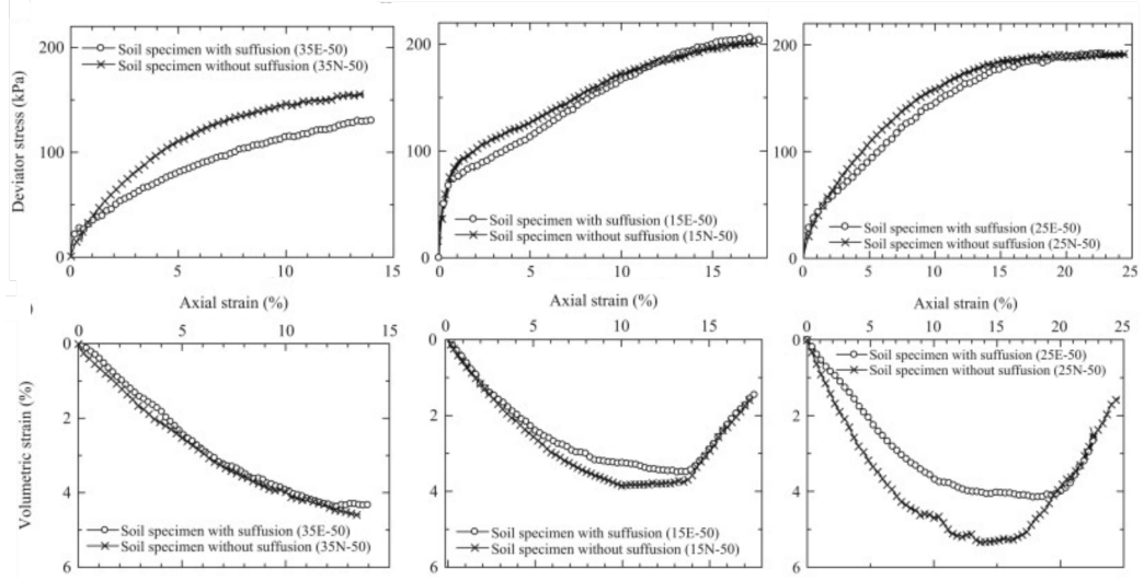
Figure 2.5 – Comparison of the drained triaxial responses of the three gap-graded specimens considered in Ke and Takahashi (2014a) with (circles) our without (crosses) suffusion. An effective confining pressure of 50 kPa is applied. The deviatoric stress (top) and the volumetric strain (bottom) evolutions with respect to the axial strain are shown.
