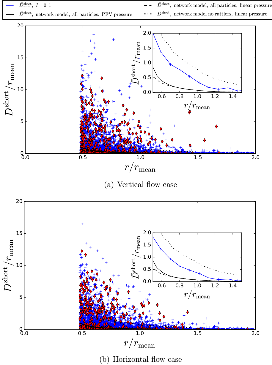
Figure 5.22 – Shortest travel distances of all the particles of the initially unstable sample corresponding to \eta = 0.9 subjected to a hydraulic gradient I = 0.1 in the vertical (a) or horizontal (b) directions. Extracted particles are identified by red diamonds. The mean transport distances \bar{D}_{\text{num}}^{\text{short}} are shown in blue solid lines. In black solid lines the numerical prediction corresponding the transport model of Section 3.3.3 are shown (pressure map computed thanks to the PFV scheme). Dashed and dot-dashed lines correspond to the predictions computed from the linear approximation of the macroscopic pressure gradient respectively on the pore network computed with all particles and on the pore network computed with only non-free particles.
