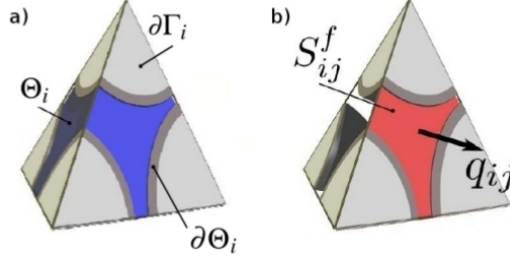
Figure 2.20 – Tetrahedron unit cell of the volume discretization (Chareyre et al., 2012). Pore volume (a) and constriction area (b).
