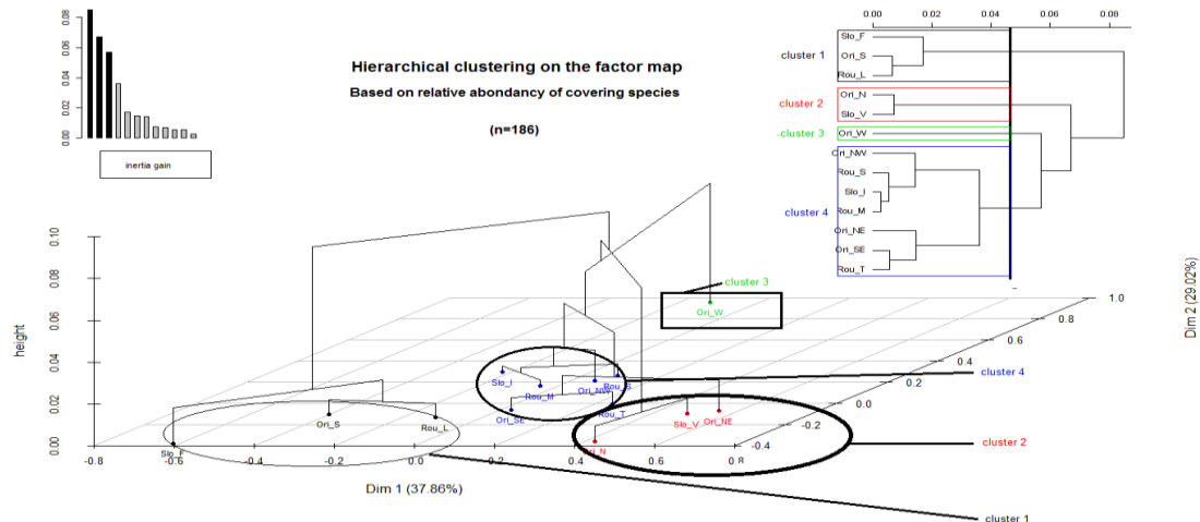
Fig.1: The two dimension HAC show a good repartition of species assemblages according to first gradient (37,86% of the variability explanation) with two opposite clusters (cluster 1 and cluster 2), the second one for intermediates values of each categories.
