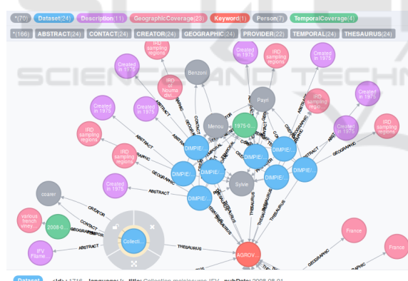
Figure 4: A zoom of different origins and scale matching with a hub node.
