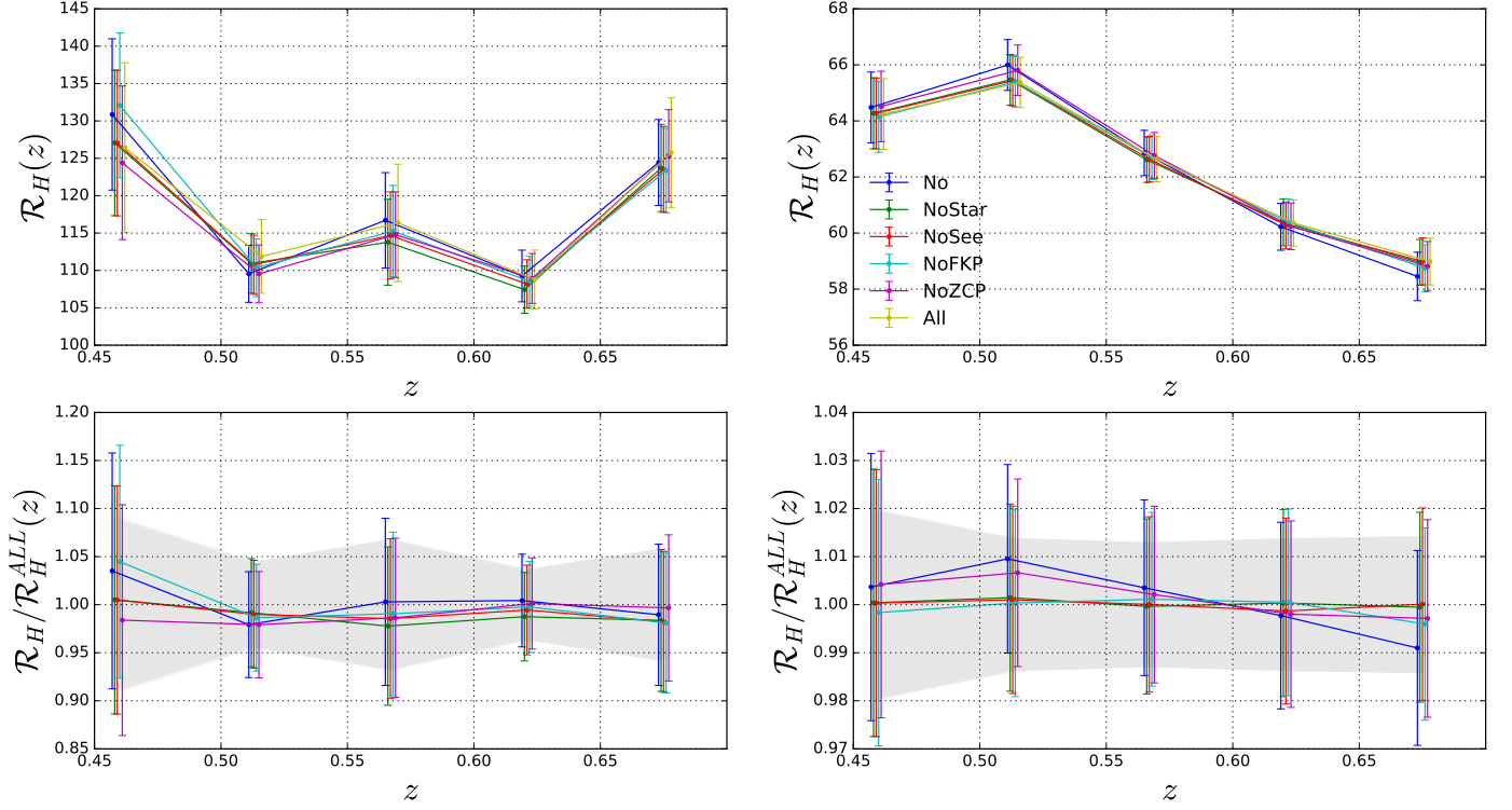
FIGURE 4.29: Systematic measurement for the homogeneity scale, \mathcal{R}_H , of the galaxy (left) and matter (right) distributions as a function of redshift, z , for the North galactic cap. Different colors correspond to different combination of the weighting scheme. Top figures show the measurement and bottom figures show the percentage ratio from the measurement applying all the weights. Shaded regions shows the 1\sigma error of the measurement applying all the weights.
