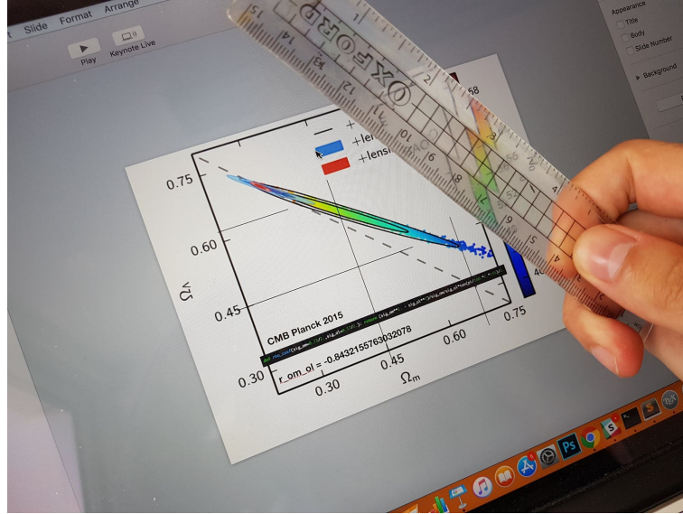
FIGURE 5.19: Illustration of extracting the (\Omega_m, \Omega_\Lambda) prior information from CMB. [Taken and remodified from Collaboration et al. [22]].
