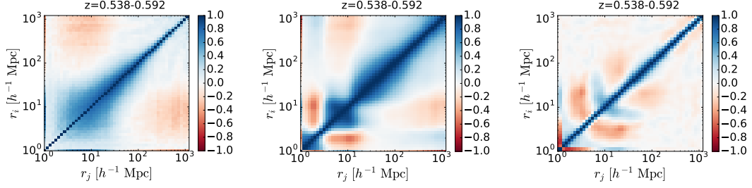
FIGURE 4.10: Correlation matrices for our estimators \xi(r) , \mathcal{N}(<r) and \mathcal{D}_2(r) for the total matter distribution estimators in the north galactic cap at the redshift slice 0.538 \leq z \leq 0.592 .
