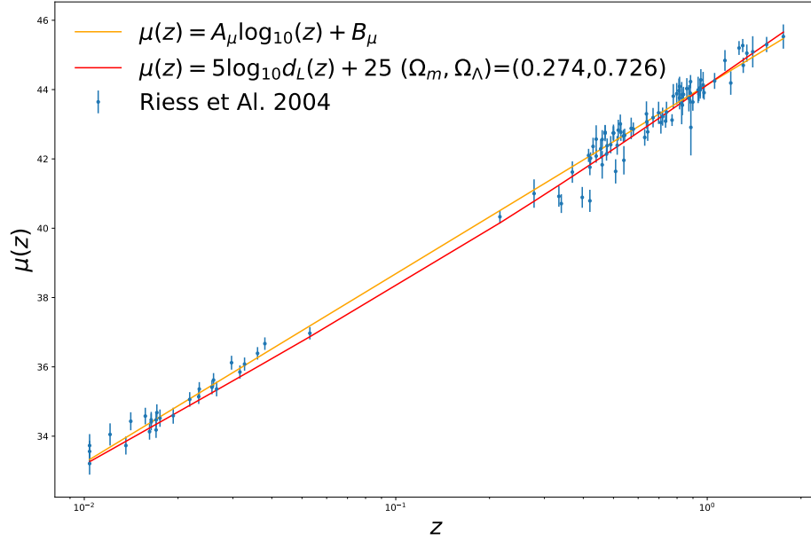
FIGURE 6.2: Supernovae distance module, \mu , as a function of redshift, z . Data points are denoted with blue, red line is the function of \Lambda CDM-model and orange is a simple relation between the distance module and the redshift.
