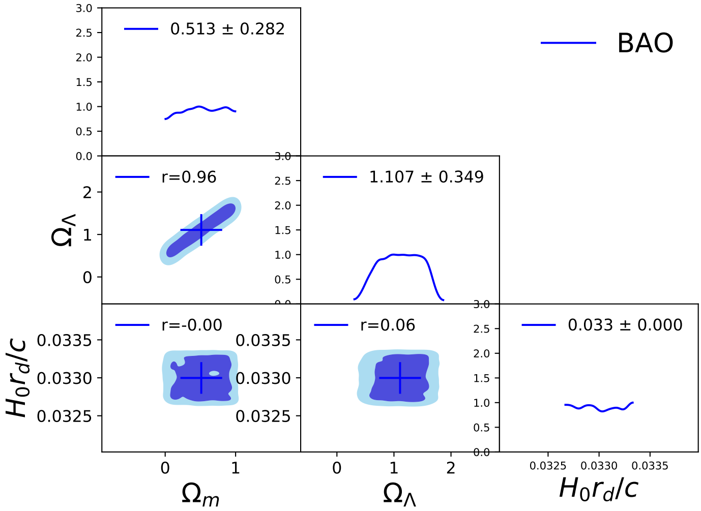
FIGURE 5.8: BAO results. see text for details.
