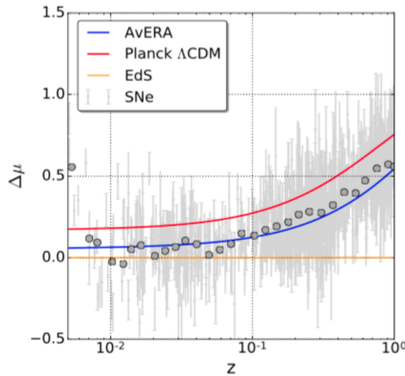
FIGURE 2.3: Relative Distance module measurement as a function of redshift of a compilation of Supernova, fitting separate isotropic universe (AvERA) better than homogeneous and isotropic universe (Planck best-fit model).[See text for details]
