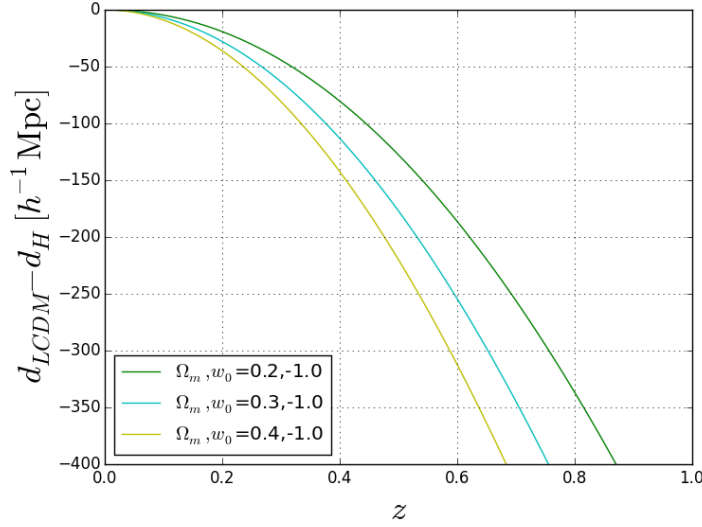
FIGURE A.3: \Lambda CDM-model Distance minus hubble distance as a function of redshift, z , for different fiducial cosmologies.
