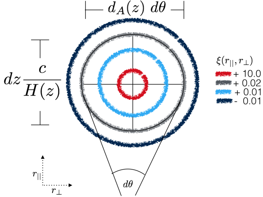
FIGURE 1.7: Illustration of the AP-test of large scale structure clustering. [See text for details]
