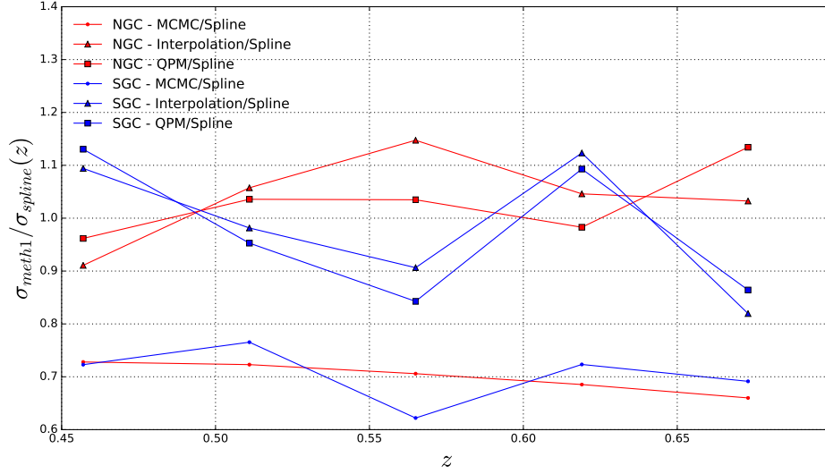
FIGURE 4.11: Ratio of the standard deviations of the homogeneity scale of the matter distribution using 3 methods over the standard deviation of the homogeneity scale using the spline method fit of our basis analysis for the different redshift bins for the NGC (red) and SGC (blue). The dot ('.') denotes the method of MCMC on the data, the ('□') square and ('^') wedge denote the standard deviation of the homogeneity scale on 1000 QPM mock catalogues with the interpolation method and the spline fit respectively.
