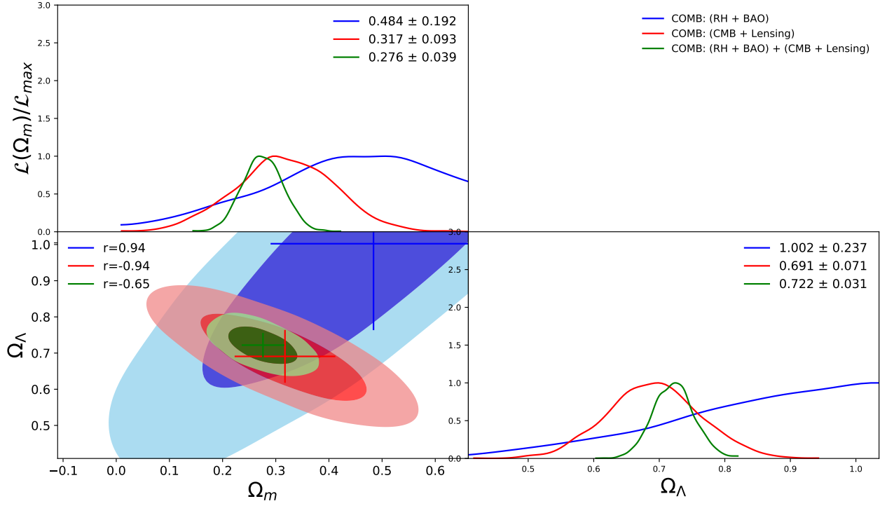
FIGURE 5.18: R_H + BAO combined with (CMB+Lensing). see text for details.
