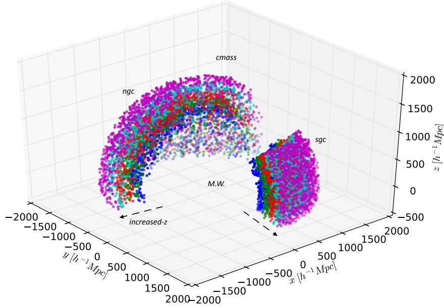
FIGURE 3.8: 3D representation of the CMASS sample. Different colors represent different redshift slices applied in homogeneity galaxy analysis[19].
