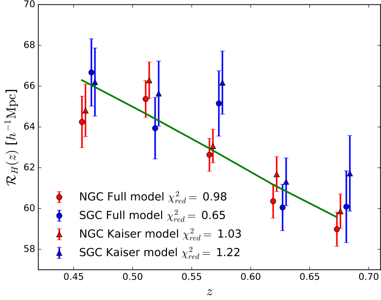
FIGURE 4.16: Measured homogeneity scale in different redshift bins, in the NGC and the SGC, with Kaiser (triangle) and full RSD model (circles).
