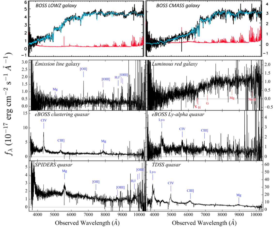
FIGURE 3.7: Sample of SDSS spectra. (Top) 2 SDSS-III targeted galaxies spectra (black) and the noise at each pixel (red) with the best redshift measurement (blue). (2nd row to Bottom) are 6 SDSS-IV targeted objects (black) with their identified emission lines (blue). [Image extracted by [18] and modified ]
