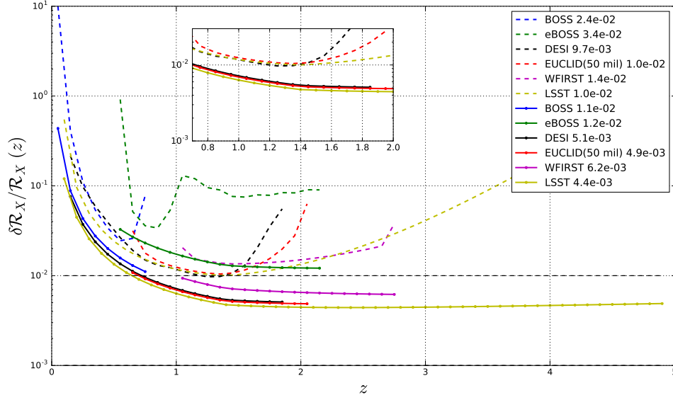
FIGURE 5.25: Precision of the scale, \mathcal{R}_X versus the redshift, z for the different experiments which are color-coded. The dash lines correspond to the BAO scale while the continues lines correspond to the homogeneity scale for the matter distribution. See text for details
