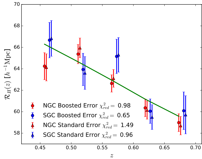
FIGURE 4.22: \mathcal{R}_H(z) with (circle) and without (triangle) boosting the errors, for NGC (red) and SGC (blue).
