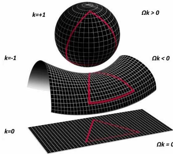
FIGURE 1.1: 2D Representation of possible variety of the curvature of our 3 dimensional spatial space.
