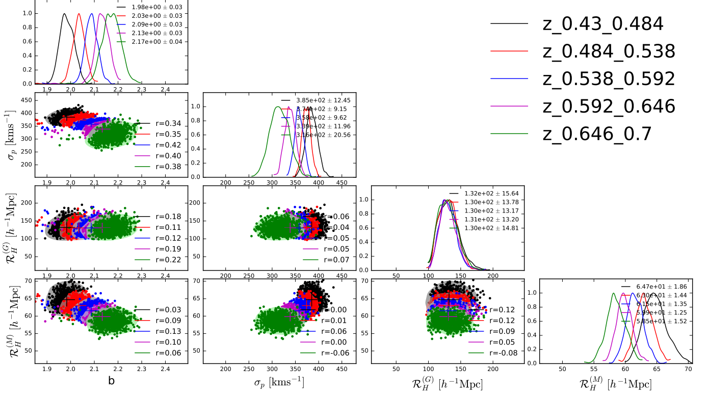
FIGURE 4.26: Same as Fig. 4.25 but for the South Galactic Cap.
