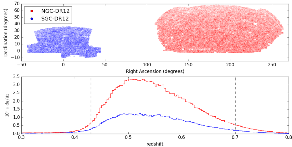
FIGURE 3.9: R.A. and Dec profiles (top) and redshift distribution (bottom) of the DR12 sample for the NGC and SGC. The vertical dashed lines define the redshift-cut used in the analysis [19].
