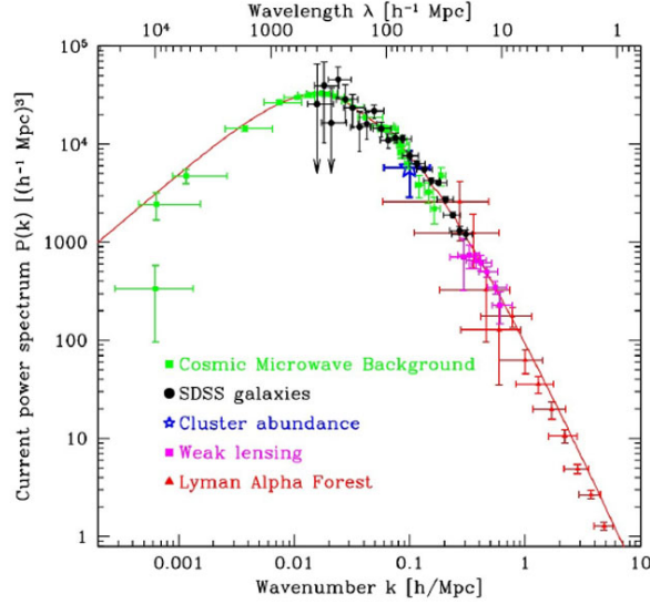
FIGURE 1.5: Measurement of the matter power spectrum observed by combination of different surveys[5].
