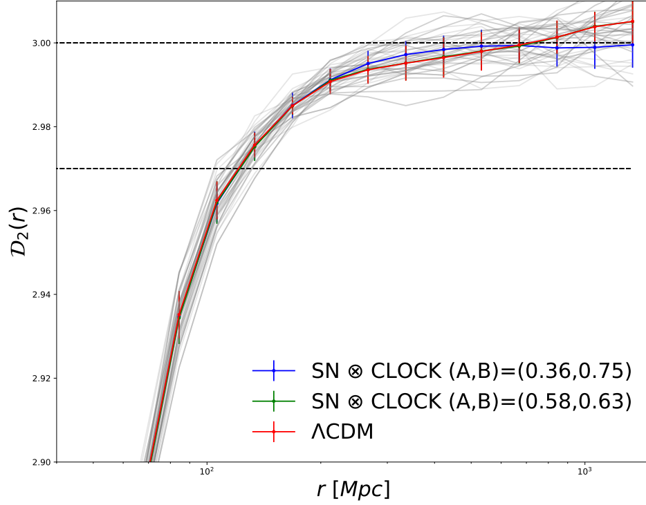
FIGURE 6.4: Fractal Correlation Dimension as a function of scales, D_2(r) , for the CMASS galaxy sample using a model independent distance measure and confirming the Cosmological Principle . [See text for details]
