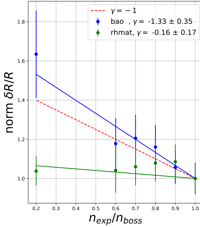
FIGURE 5.23: Normalized fractional error \delta R/R as a function of density, n , for the bao scale (blue) and the homogeneity scale (green) for the the galaxy distribution. [See text for details.]
