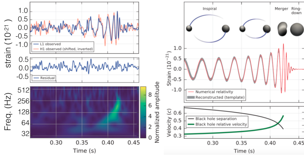
FIGURE A.2: Left: Gravitational Wave (GW) Signal as a function of time Right: Physical interpretation of the GW signal, which correspond to a coalescence of two Black Holes
