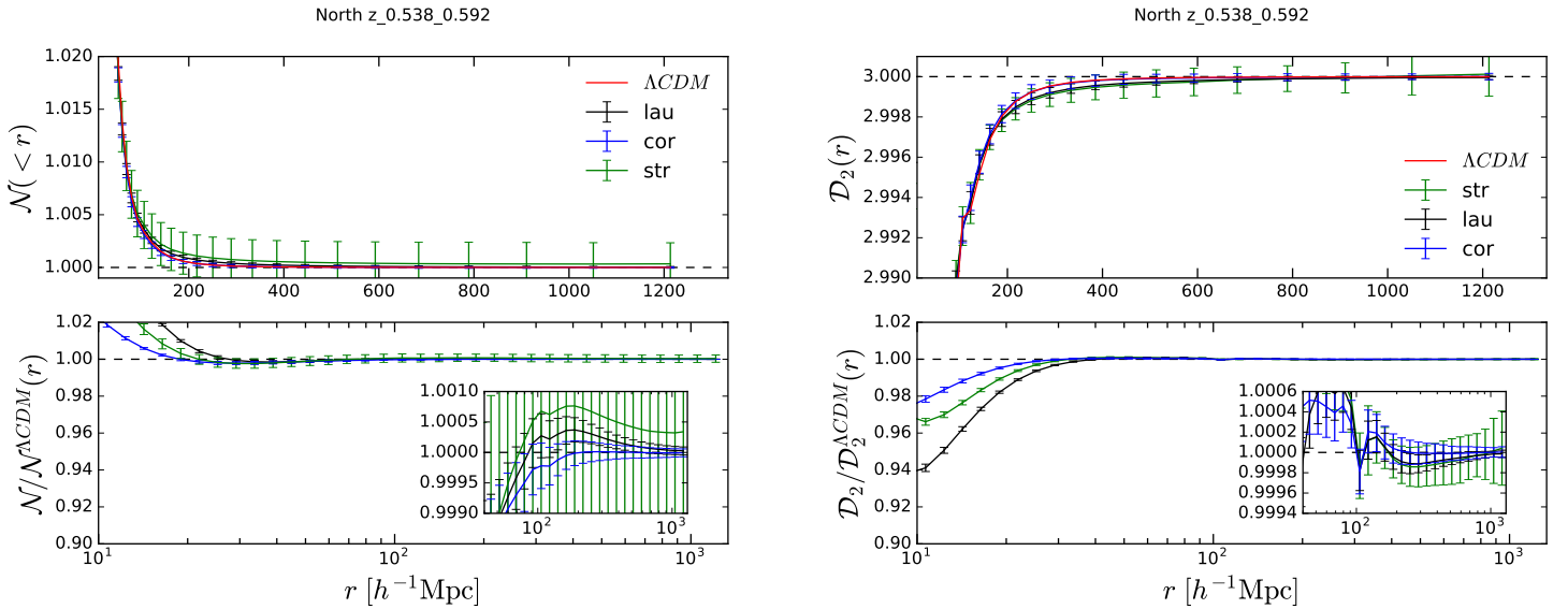
FIGURE 4.23: Top: the scaled counts-in-spheres, \mathcal{N}(< r) , (left) and the fractal correlation dimension, \mathcal{D}_2(r) , (right) for matter distribution, with str(green), lau (black) and cor (blue) estimators, compared to \Lambda\text{CDM} model (red). Bottom: the ratio to \Lambda\text{CDM} model for both estimator.
