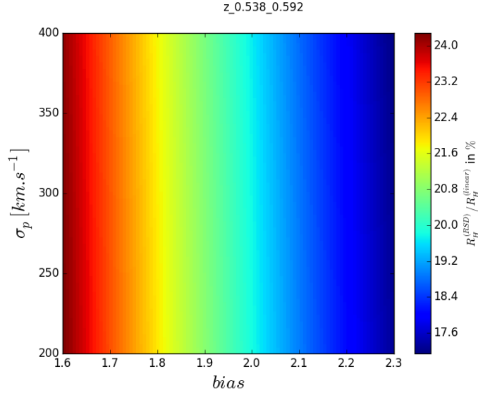
FIGURE 4.1: Test of necessity of RSD modelling: We show the percentage ratio of the predicted homogeneity scale defined in Eq. 4.7 with and without accounting redshift space distortions according to Eq.4.17. The effect ranges from 15 to 25% and varies according to the bias parameter and is therefore not negligible.
