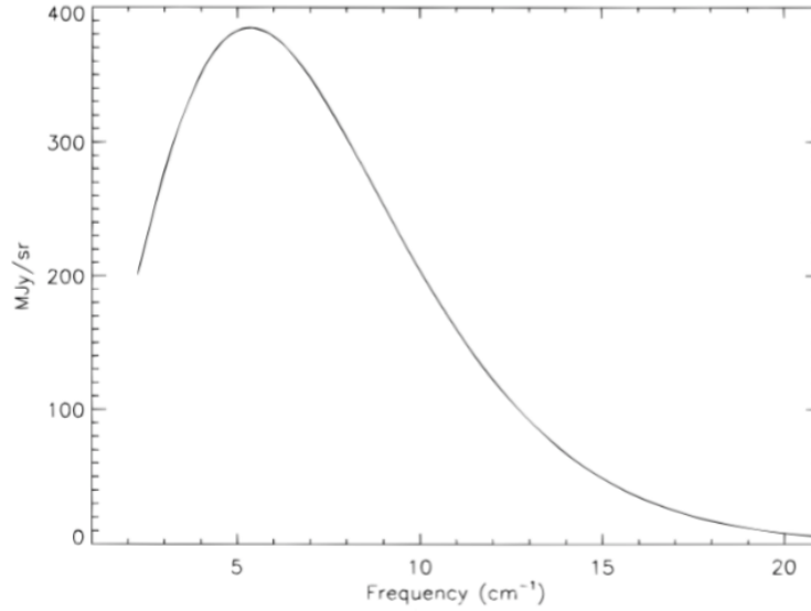
FIGURE 1.10: Uniform frequency spectrum (intensity vs frequency) fitted on the theoretical Planck Black Body curve. The errorbars are only a small fraction of the line thickness[9]. [See text for details]
