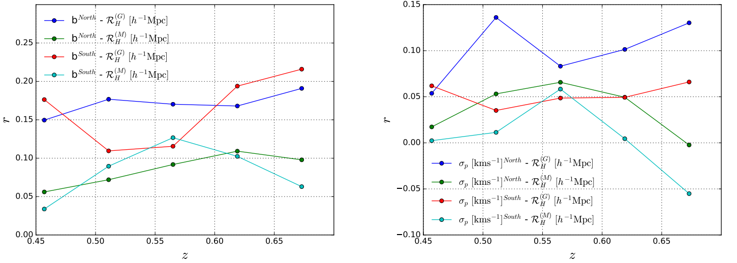
FIGURE 4.27: Correlation coefficient, r , as a function of redshift, z , between bias, b (left), or peculiar velocities, \sigma_p (right), and the homogeneity scale, \mathcal{R}_H for the North or South galactic caps for the matter (M) or galaxy (G) distribution, as measured for 1000 QPM mock catalogs.
