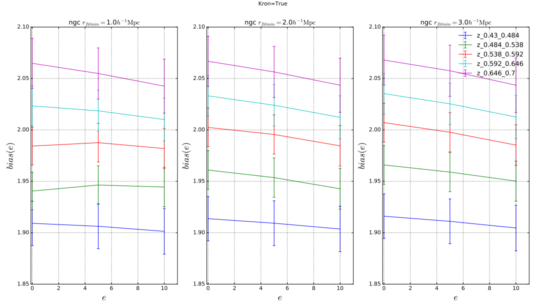
FIGURE 4.19: Cosmic bias parameter, b , as a function of boosting parameter e , for different fitting ranges from left to right and different redshift slices (different colors). See text for details]
