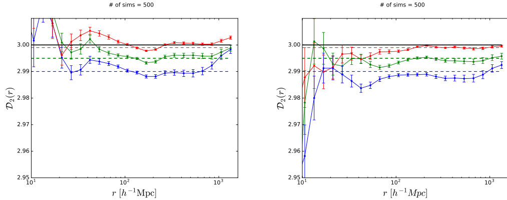
FIGURE 4.14: Reconstructed average value of \mathcal{D}_2 as a function of scales, r , with the estimators \mathcal{D}_2^{str}(r) (left) and \mathcal{D}_2^{cor}(r) (right), for 500 simulations. The errors are obtained with the standard deviation over 500 simulations. The dash line corresponds to the initial input value of \mathcal{D}_2
