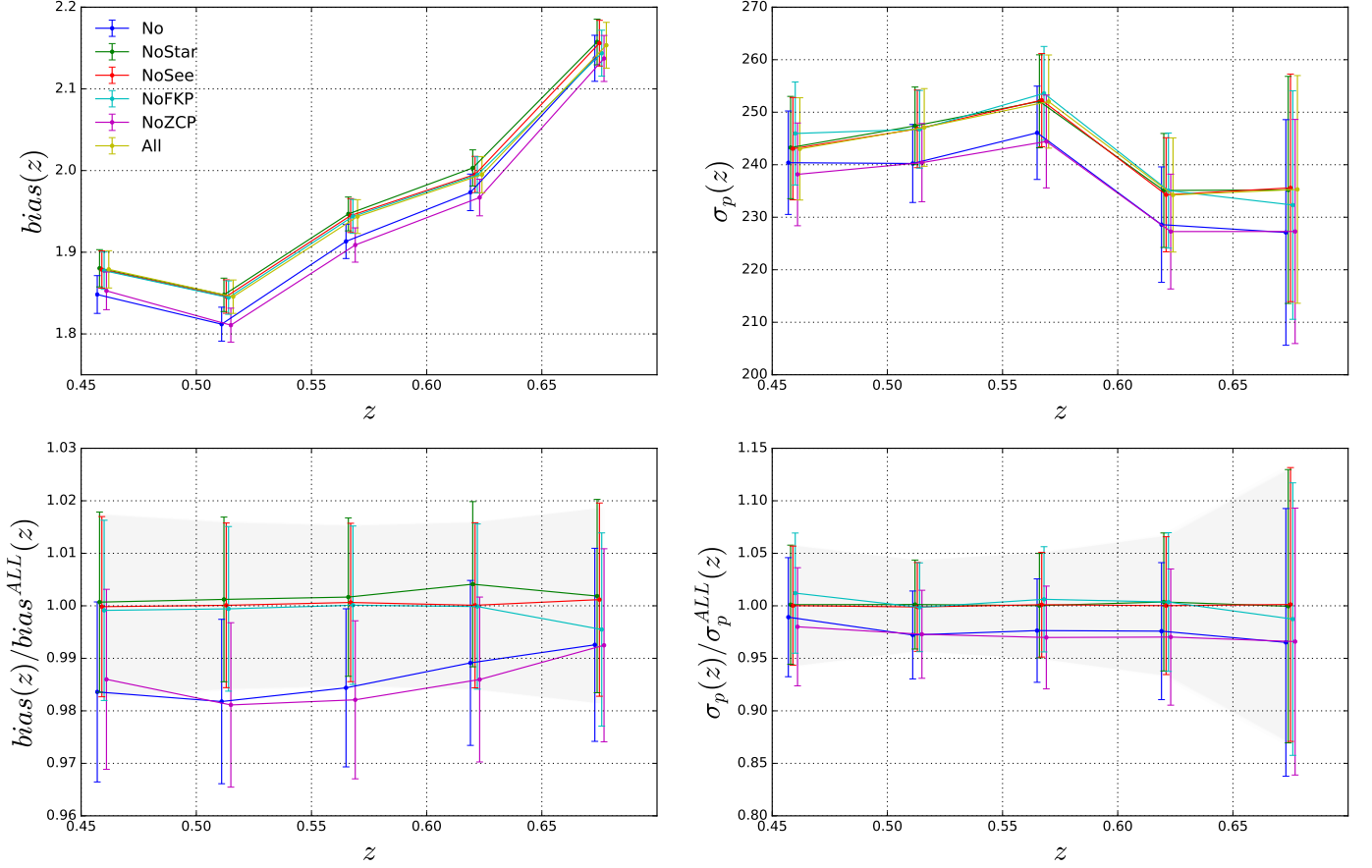
FIGURE 4.28: Systematic measurement of the bias, b and peculiar velocities, \sigma_p as a function of redshift bins, z for the North galactic cap. Different colors correspond to different weighting scheme. Top figures show the measurement and bottom figures show the percentage ratio from the measurement applying all the weights. Shaded regions shows the 1\sigma error of the measurement applying all the weights.
