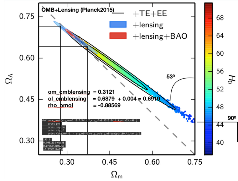
FIGURE 5.20: Extraction of the (\Omega_m, \Omega_\Lambda) prior information from CMB [Taken and remodified from Collaboration et al. [22]].
