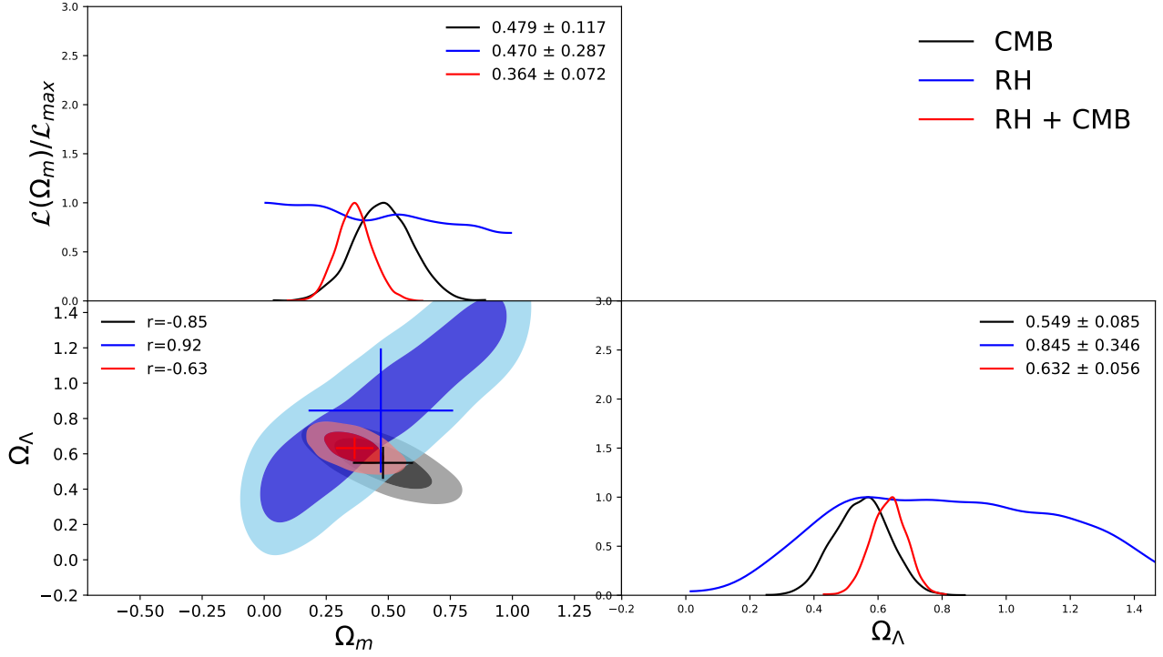
FIGURE 5.15: RH results. Contours of the cosmological parameters exploring, using the CMB (black), \mathcal{R}_H (blue), \mathcal{R}_H + \text{CMB} (red). See text for details.
