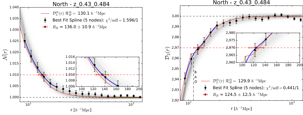
FIGURE 4.3: Scaled counts-in-spheres, \mathcal{N}(<r) , (left) and fractal correlation dimension, \mathcal{D}_2(r) , (right). The black points with error bars are the result for the galaxy distribution in the NGC in the 0.430 \leq z \leq 0.484 redshift bin. The blue lines are the best spline fit of the data. The green lines are the results for the 1000 QPM mock catalogs. The red continuous line is the \Lambda CDM prediction for b = 1.95 and \sigma_p = 252 km/s. The vertical dash line shows the BAO feature on the fractal correlation dimension computation.
