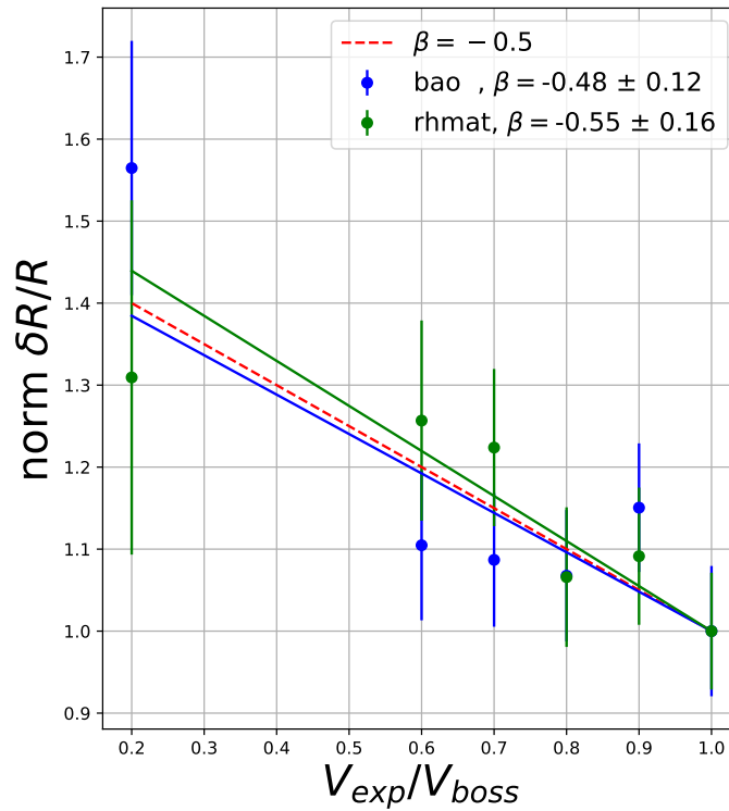
FIGURE 5.22: Normalized fractional error \delta R/R as a function of volume, V , for the bao scale (blue) and the homogeneity scale (green) for the the galaxy distribution. [See text for details.]
