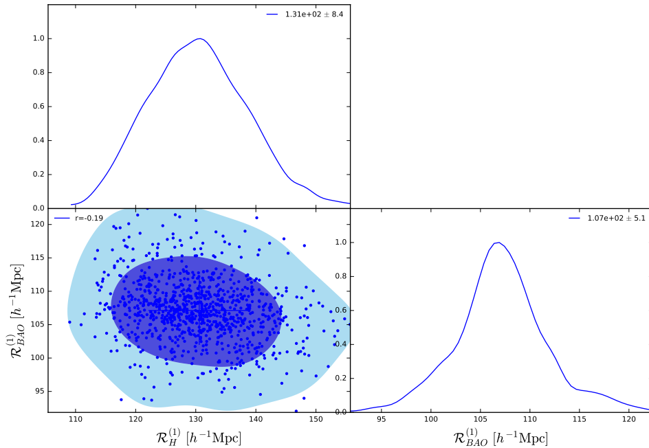
FIGURE 5.1: Contour plot with 1\sigma(2\sigma) in dark blue (light blue) for the Homogeneity scale versus the BAO scale for the 0.538 \leq z < 0.592 . See text for details.
