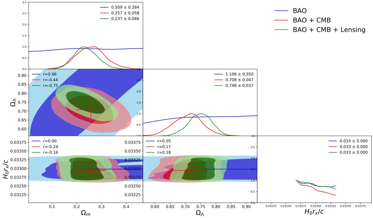
FIGURE 5.9: Estimation of cosmology [Contours of %68,%95 of (\Omega_m, \Omega_\Lambda) -plane] using BAO and CMB and BAO, CMB and CMB-Lensing data. [see text for details.]
