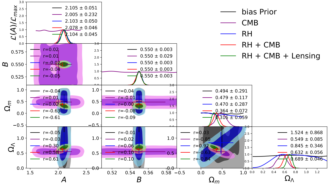
FIGURE 5.14: RH results for (A, B, \Omega_m, \Omega_\Lambda) . Contours of the cosmological parameters exploring, using the Prior- (A, B) determination (black), CMB (purple), \mathcal{R}_H (blue), \mathcal{R}_H + CMB (red), \mathcal{R}_H + CMB + Lensing (green). See text for details.
