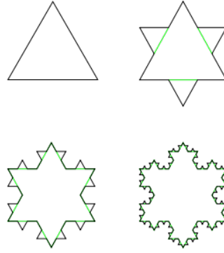
FIGURE 2.5: The first four iterations of the Kock snowflake.[Image taken from [15]]
