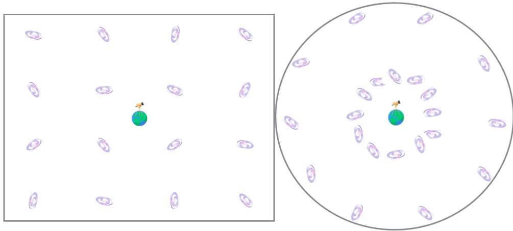
FIGURE 2.2: Left : 2D representation of homogeneous (and isotropic) galaxy distribution Right : 2D representation of an isotropic (but not homogeneous) galaxy distribution [See text for explanation][Credit on [13]]
