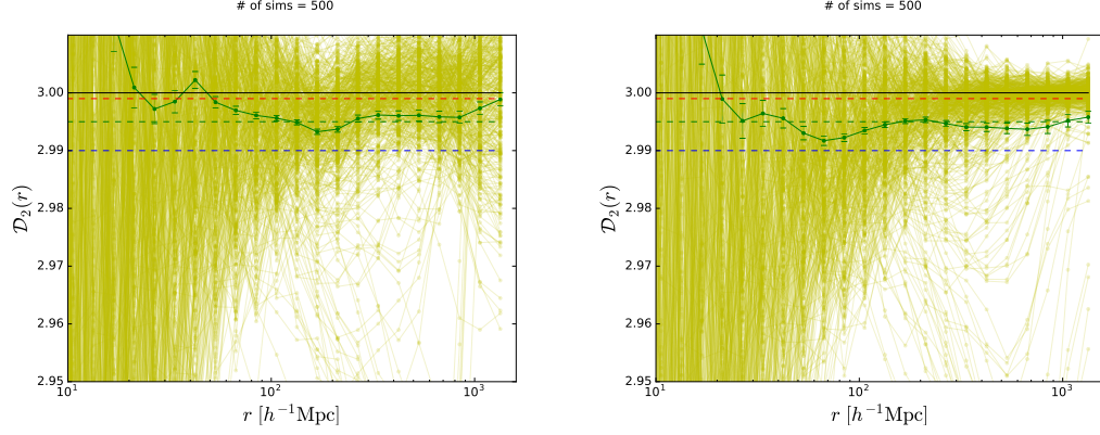
FIGURE 4.13: Reconstructed fractal correlation dimension, \mathcal{D}_2 , at the nominal value 2.995 (green dash line) in the redshift interval z = 0.538 - 0.592 . Yellow line represent each fractal simulation. Green line is the average and error over 500 simulations for str-estimator (left) and cor-estimator (right).
