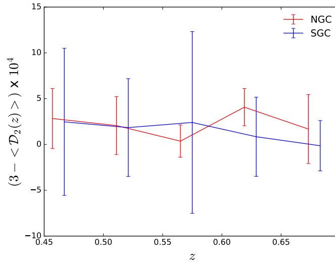
FIGURE 4.8: Fractal correlation dimension for the matter distribution, 3 - \langle \mathcal{D}_2 \rangle , averaged over 300 h^{-1} < r < 1300 h^{-1} Mpc, in the different redshift bins.
