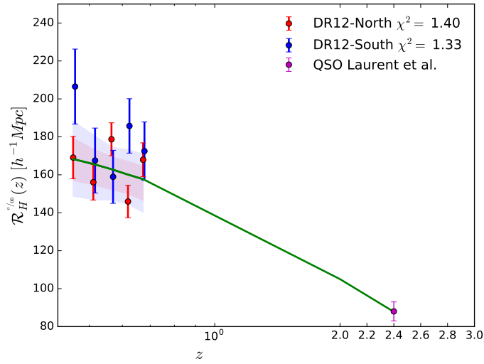
FIGURE 4.33: The homogeneity scale at 0.1% level, R_H^{D_2=2.997}(z) , measured in the NGC (red) and in the SGC (blue) as a function of redshift. The purple point is the result obtained with quasars in the NGC, in the redshift range 2.2 \leq z \leq 2.8 by Laurent et al. [21]. The green line is the \Lambda\text{CDM} model prediction. The shaded areas indicate the 1\sigma range for the 1000 QPM mock catalogs.
