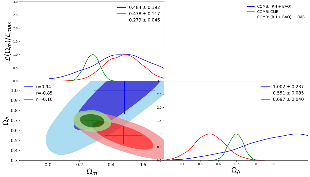
FIGURE 5.17: R_H + BAO combined with CMB. see text for details.
