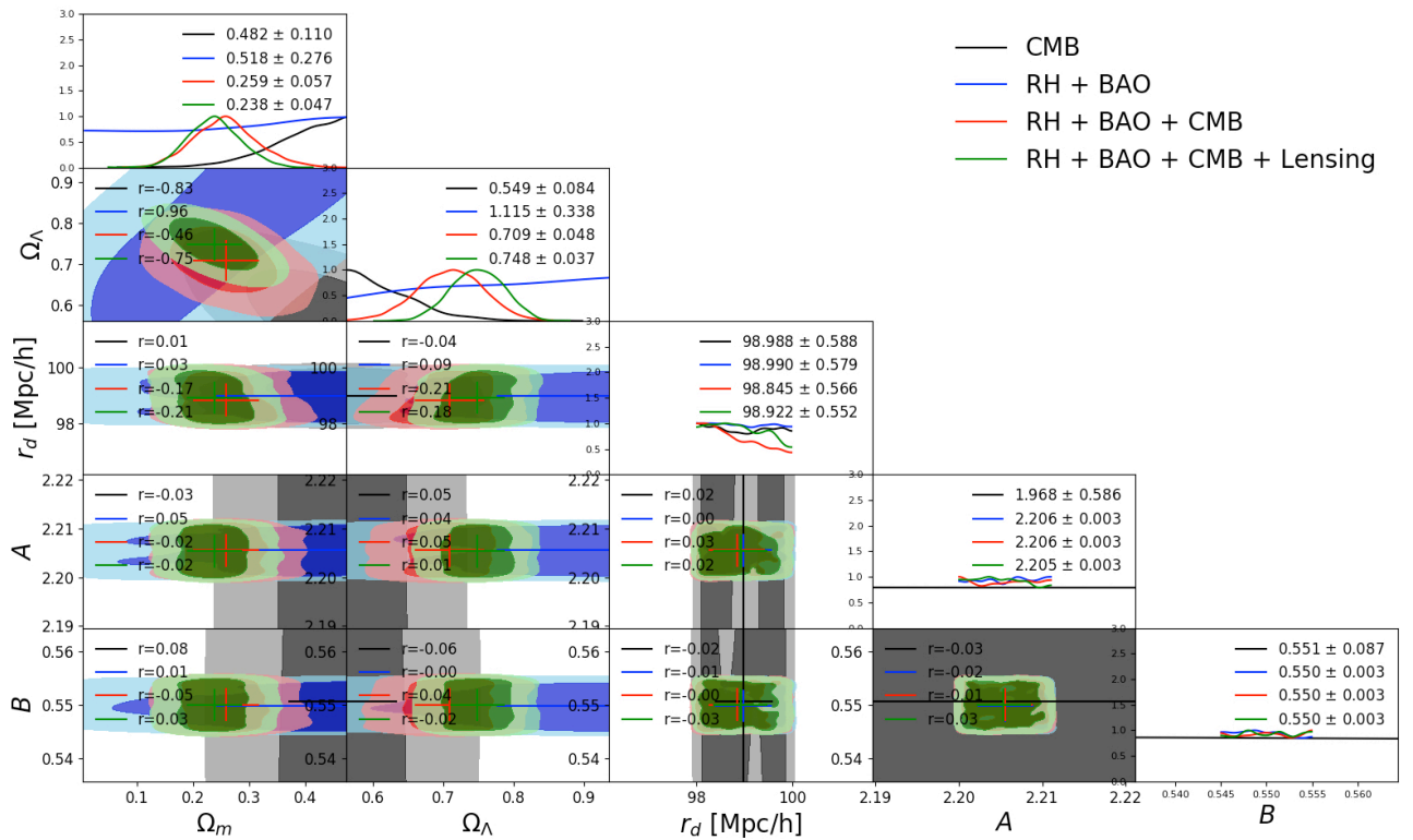
FIGURE 5.11: R_H + BAO combination results. see text for details.
