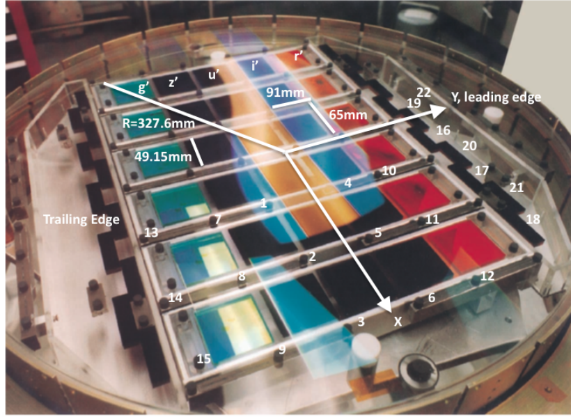
FIGURE 3.2: Photometric Camera Layout and its design overplotted. Optical layout of the focal plane of the SDSS camera. Field 22 (top and bottom) are focus CCDs; Fields 16-21 are astrometric chips, and 1-15 are the photometric array. The TDI drift scan direction is coming from the nose of Y-arrow to its tail, so a star-light traverses this array from right to left. [Image taken from [16] and modified to include the design]
