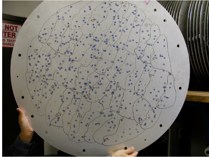
FIGURE 3.6: BOSS Aluminum plate. Bundles are separated by black bounded edges, and holes are marked in blue to reduce contamination between nearby emission line galaxies or quasars. Holes for guide star fibers are marked in black and denoted by the corresponding number ranging from 1 to 16.
