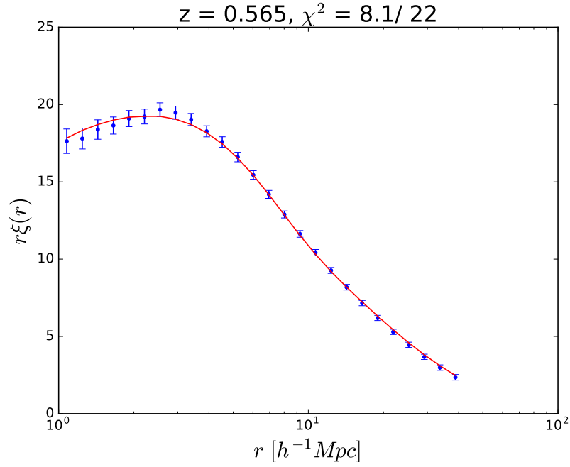
FIGURE 4.17: Empirical 2ptCF, \xi_{fit}(r; b, \sigma_p, \vec{p}_{cs}) , as a function of scales, r , for the best fit parameters, (b, \sigma_p, \vec{p}_{cs}) = (b^{fit}, \sigma_p^{fit}, \vec{p}_{cs}^{fit}) for the mean of the (0.538 \leq z \leq 0.592) -slice. [See text for details]
