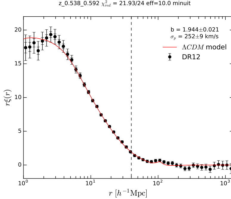
FIGURE 4.4: The correlation function of the CMASS galaxies in the [0.538 - 0.592] redshift range. Data points have both their original error bars and the error bars enlarged to take into account the uncertainty of the RSD model on small scales (see section 4.2.2 and appendix 4.3.7). The red line is the result of the fit performed over the range [1, 40] h^{-1}\text{Mpc} (up to the vertical black-dashed line).
