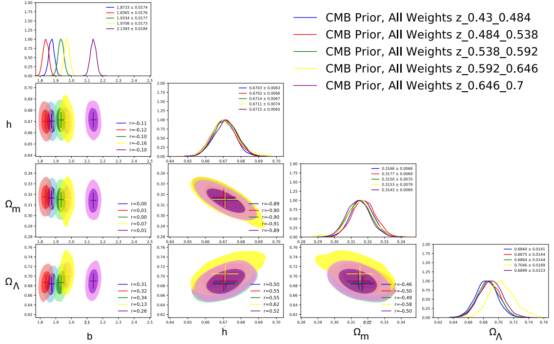
FIGURE 5.6: Contours of 68% (shaded) and 95% (light) C.L. of the homogeneity scale of the galaxy distribution for the 3 cosmological parameters of \Lambda CDM-model for the 5 redshift slices (color-coded) of the North Galactic Cap. [See text for details.]
