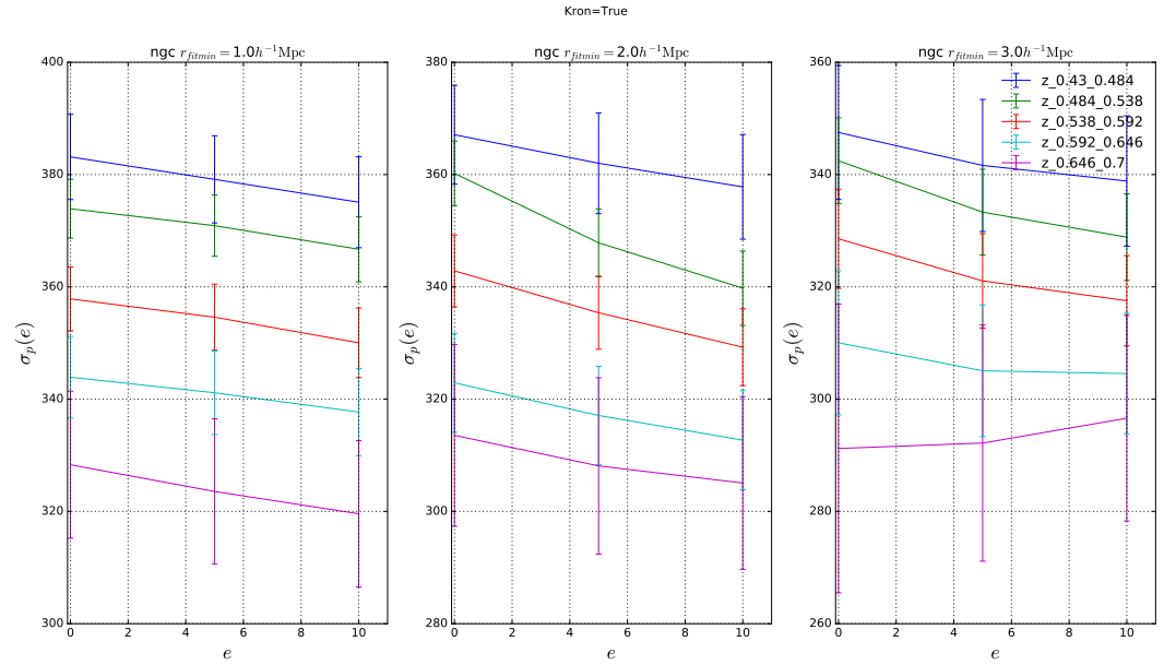
FIGURE 4.20: Same as Fig. 4.19 but for the peculiar velocities, \sigma_p . [See text for details]
