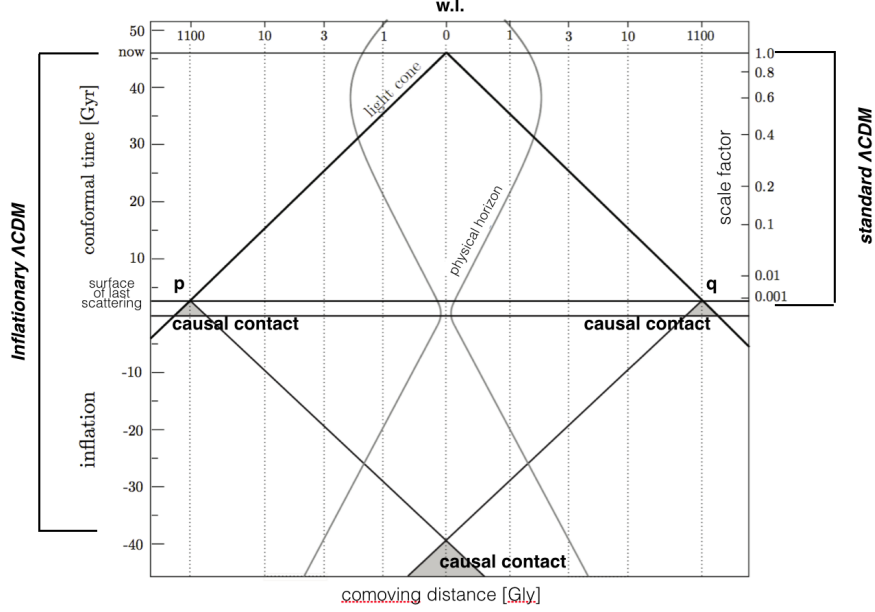
FIGURE 1.9: : Illustration of the inflationary solution to the horizon problem. The comoving physical horizon shrinks during inflationary epoch and expands during the standard \Lambda CDM-model evolution at least until later time at a > 0.5 . This allows all large physical fluctuations ( p, q points at the surface of last scattering which are outside the physical horizon) to be in causal contact with each other at initial times since in the past they were inside the physical horizon. [Diagram was taken by Baumann [8]]
