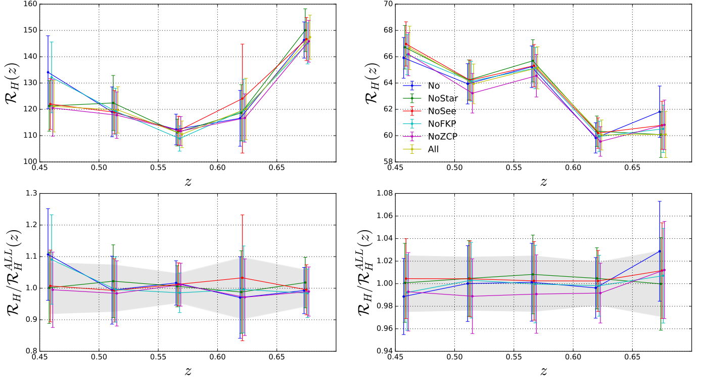
FIGURE 4.31: Same figure as Fig. 4.29 for the south galactic cap
