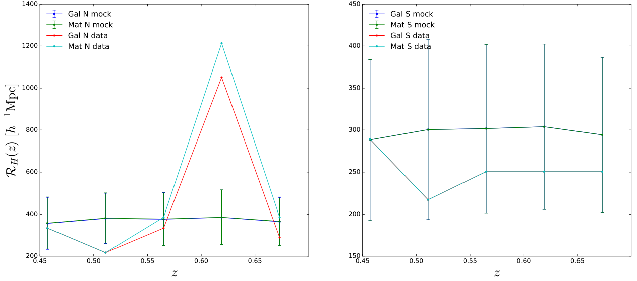
FIGURE 4.35: Mean and dispersion of \mathcal{R}_H^E -estimator for NGC and SGC.
