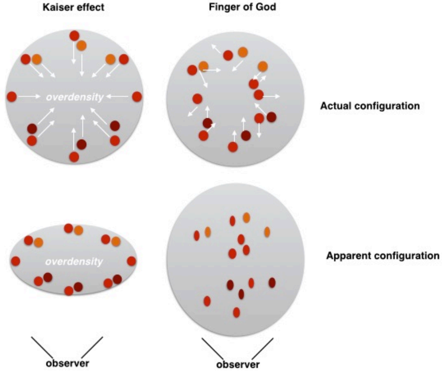
FIGURE 2.6: Schematic illustration of the Redshift Space Distortion effect. In the top the figures represent the actual position of the celestial objects and their velocities. On the left the motions are due to gravitational potential of the overdensity and on the right due to gravitational interaction among the objects. Bottom figures represent the apparent position of the objects and the apparent shape of the overdensity. [See text for details]
