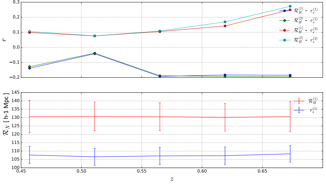
FIGURE 5.2: Upper: Correlation coefficient ( r ) as a function of z for methods measuring \mathcal{R}_H and r_s . Bottom: \mathcal{R}_H and r_s measurement as a function of z for 1000 QPM mock catalogues. See text for explanation.
