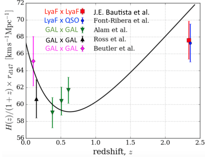
FIGURE 1.8: Large scale structure clustering measurements, revealing the accelerating nature of our universe with a combination of AP-tests [Image drag from [7]]
