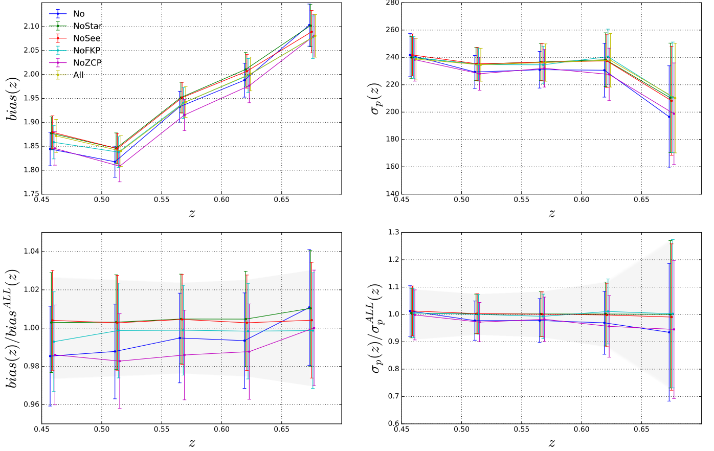
FIGURE 4.30: Same figure as Fig. 4.28 for the south galactic cap
