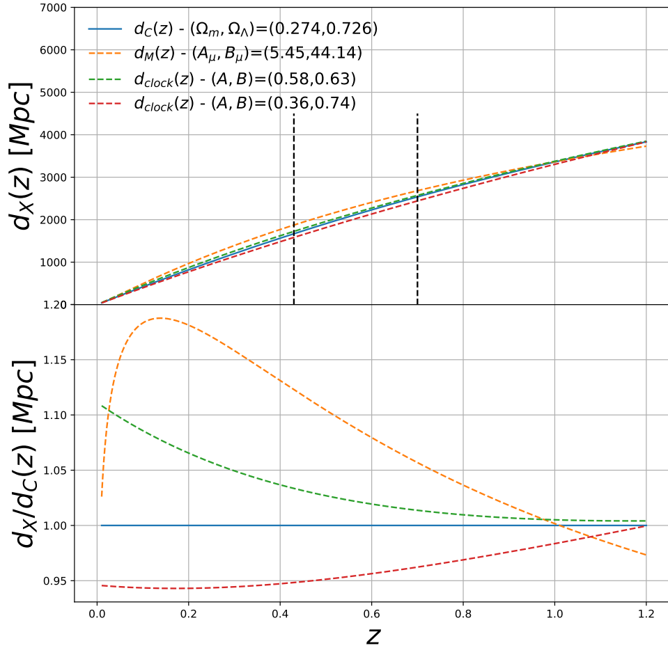
FIGURE 6.3: (Top) Cosmological distance versus redshift for the FLRW comoving distance, d_C (blue), model-independent transverse comoving distance, d_M (orange), and the two model independent cosmic clock comoving distances, d_{clock} (green and red). The black vertical lines indicate the redshift cuts of our survey. (Bottom) Different cosmological distances over comoving distance versus redshift.
