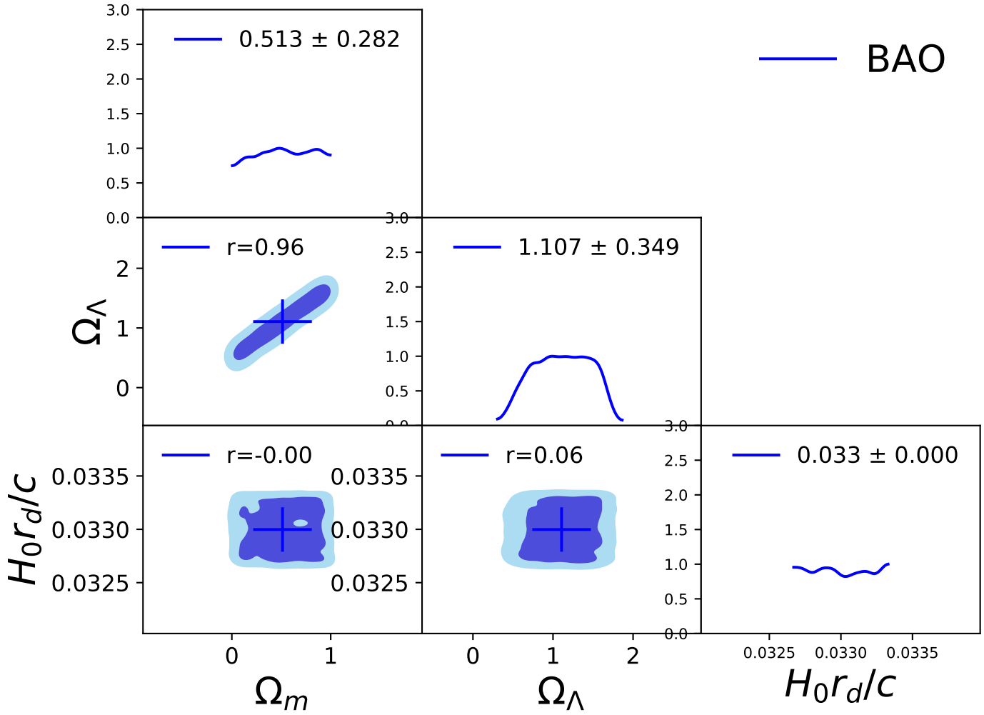
FIGURE 5.12: BAO results. see text for details.
