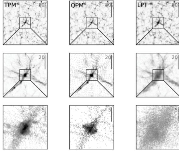
FIGURE 3.10: Qualitative comparison mock catalogues QPM and LPT with N-body simulations (TPM). The advantage of QPM against LPT is clear on the non linear regime.[image taken from White et al. [20]]
