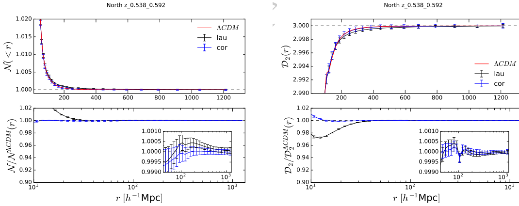
Figure 12. Top: the scaled counts-in-spheres, \mathcal{N}(< r) , (left) and the fractal correlation dimension, \mathcal{D}_2(r) , (right) for matter distribution, with lau (black) and cor (blue) estimators, compared to \Lambda CDM model (red). Bottom: the ratio to \Lambda CDM model for both estimator.
