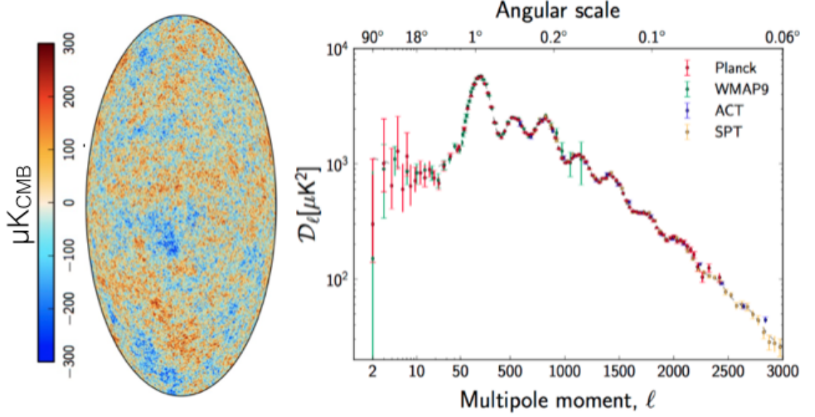
FIGURE 1.11: Left : CMB intensity map showing the temperature fluctuations as observed by PLANCK Satellite[10]. Right : Measured angular power spectra of a compilation of experiments denoted with different colours [11]. [See text for details]
