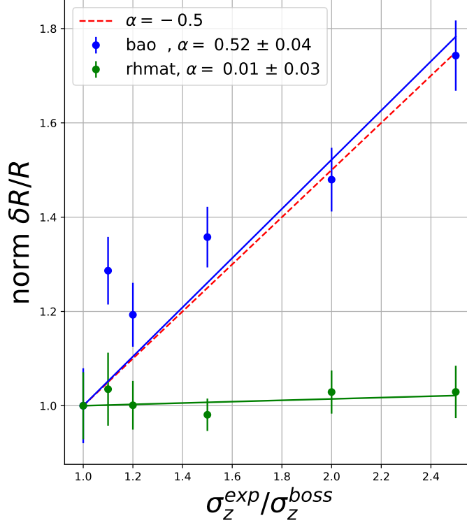
FIGURE 5.24: Normalized fractional error \delta R/R as a function of photometric redshift error, \sigma_z , for the bao scale (blue) and the homogeneity scale (green) for the the galaxy distribution. [See text for details.]
