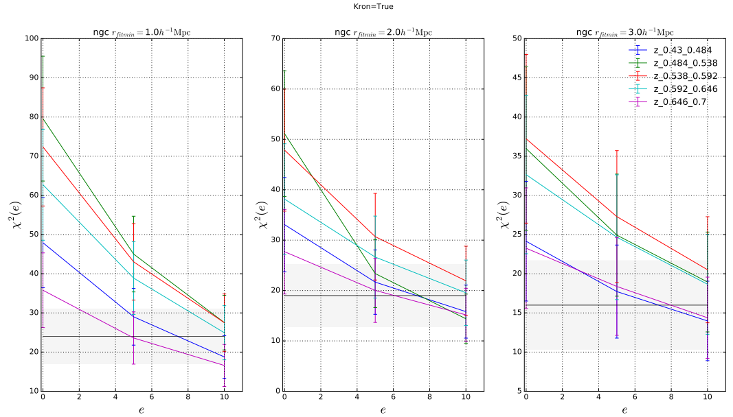
FIGURE 4.18: \chi^2 test for selection of best boosting error parametrized by e , for different fitting ranges from left to right and different redshift slices (different colors). See text for details]
