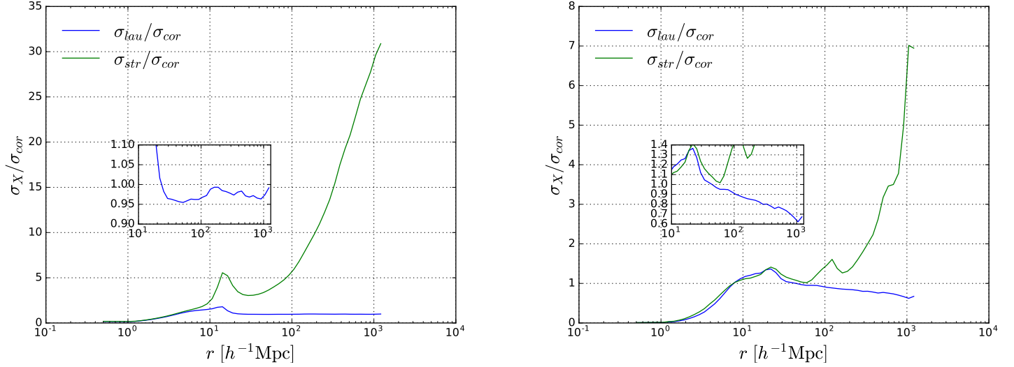
FIGURE 4.24: Ratio of the 1\sigma of the observables \mathcal{N} (left) and \mathcal{D}_2 (right) for estimators lau (blue) and str (green) against cor as defined in table 4.2 as a function of scales, r . We zoom in at scales r \in [10 - 1300]h^{-1}\text{Mpc} .
