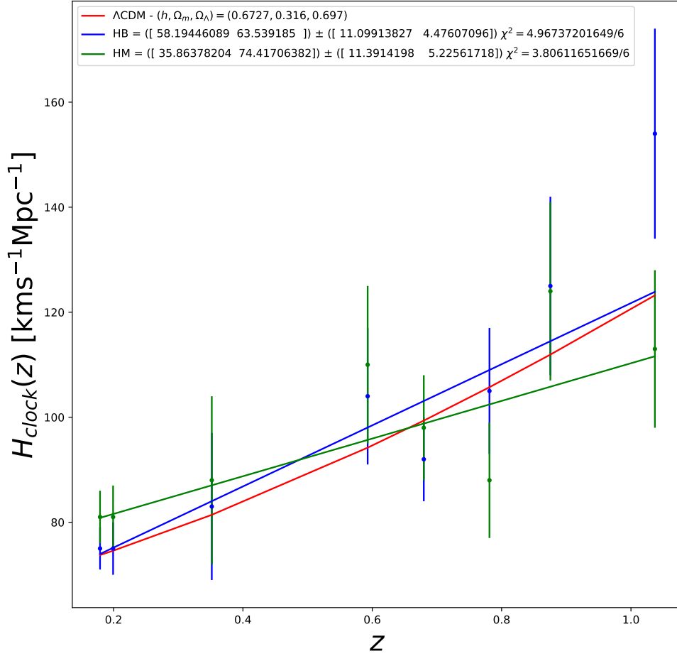
FIGURE 6.1: Left : Calibrating the Hubble expansion rate using cosmic chronometers. [See text for details]
