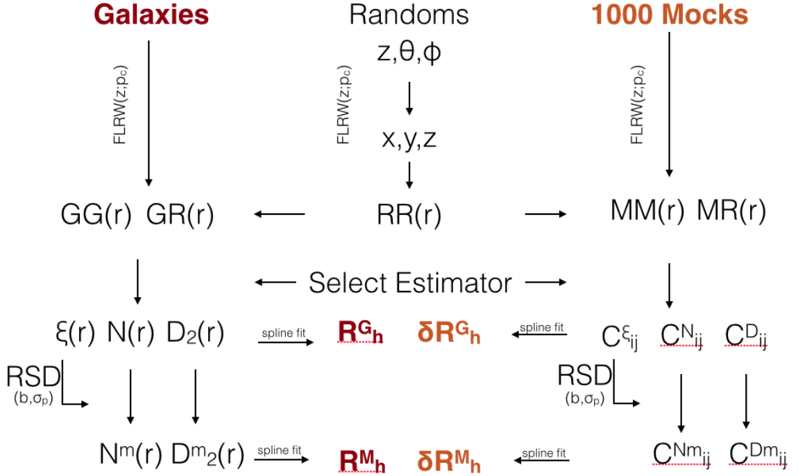
FIGURE 4.2: Core analysis pipeline procedure. See text for detailed explanation
