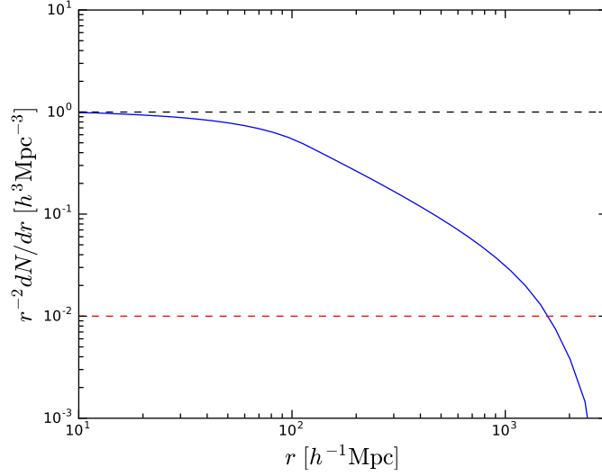
FIGURE 4.9: Scaled number density of random pairs, r^{-2}dN/dr , versus the comoving radius of spheres, r , normalized to be unity at small r .
