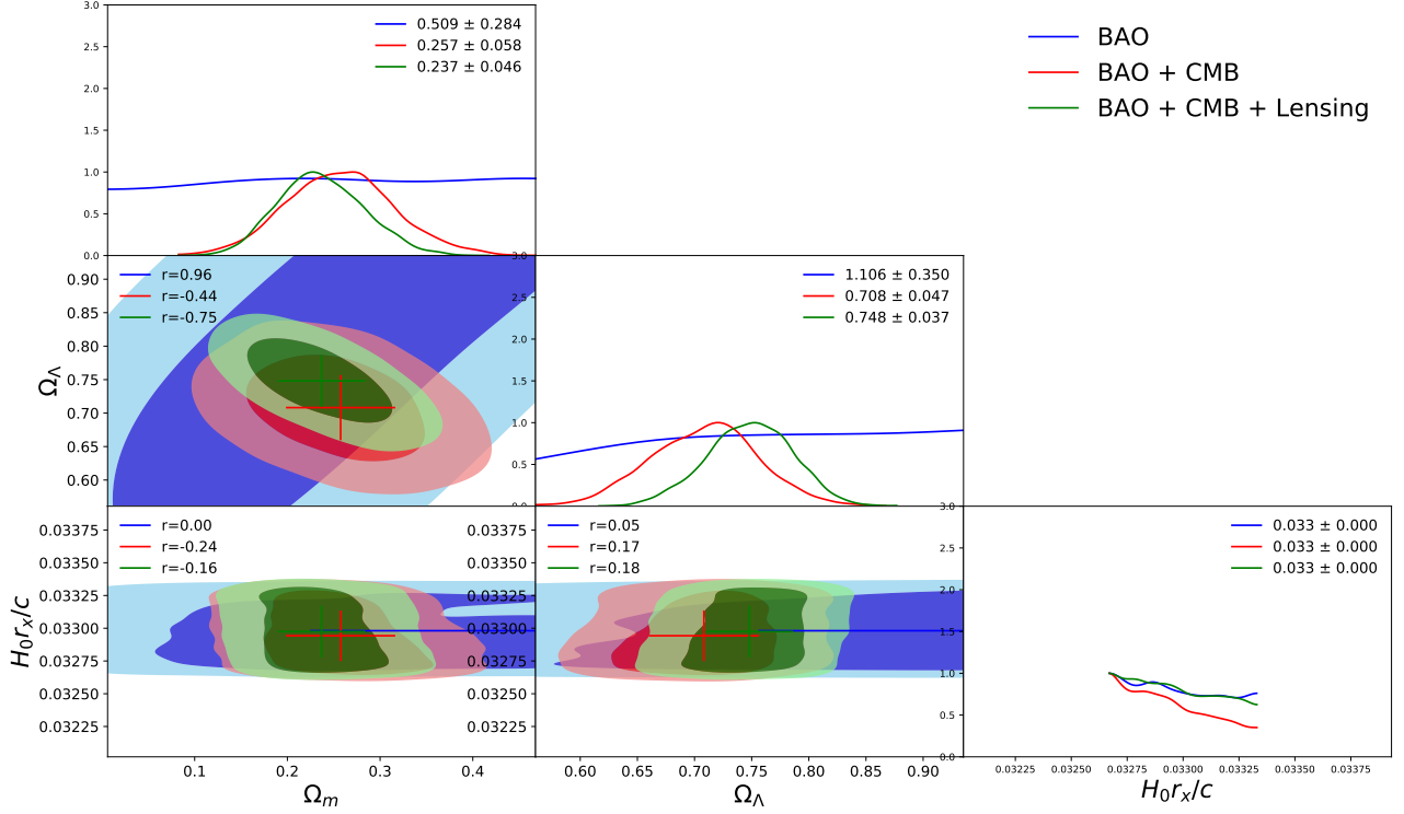
FIGURE 5.13: Estimation of cosmology [Contours of %68,%95 of (\Omega_m, \Omega_\Lambda) -plane] using BAO and CMB and BAO, CMB and CMB-Lensing data. [see text for details.]
