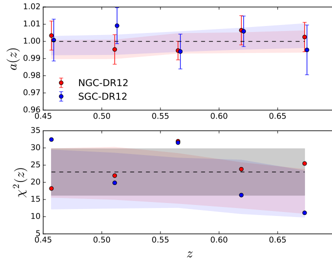
FIGURE 4.7: Top: value of the dilatation parameter a resulting from the fit of the NGC (red) and SGC (blue) \mathcal{D}_2(r) data with the model of equation 4.23, in different redshift bins. The shaded areas correspond to the 1\sigma region for the 1000 QPM mock catalogs. Bottom: The corresponding \chi^2 .
