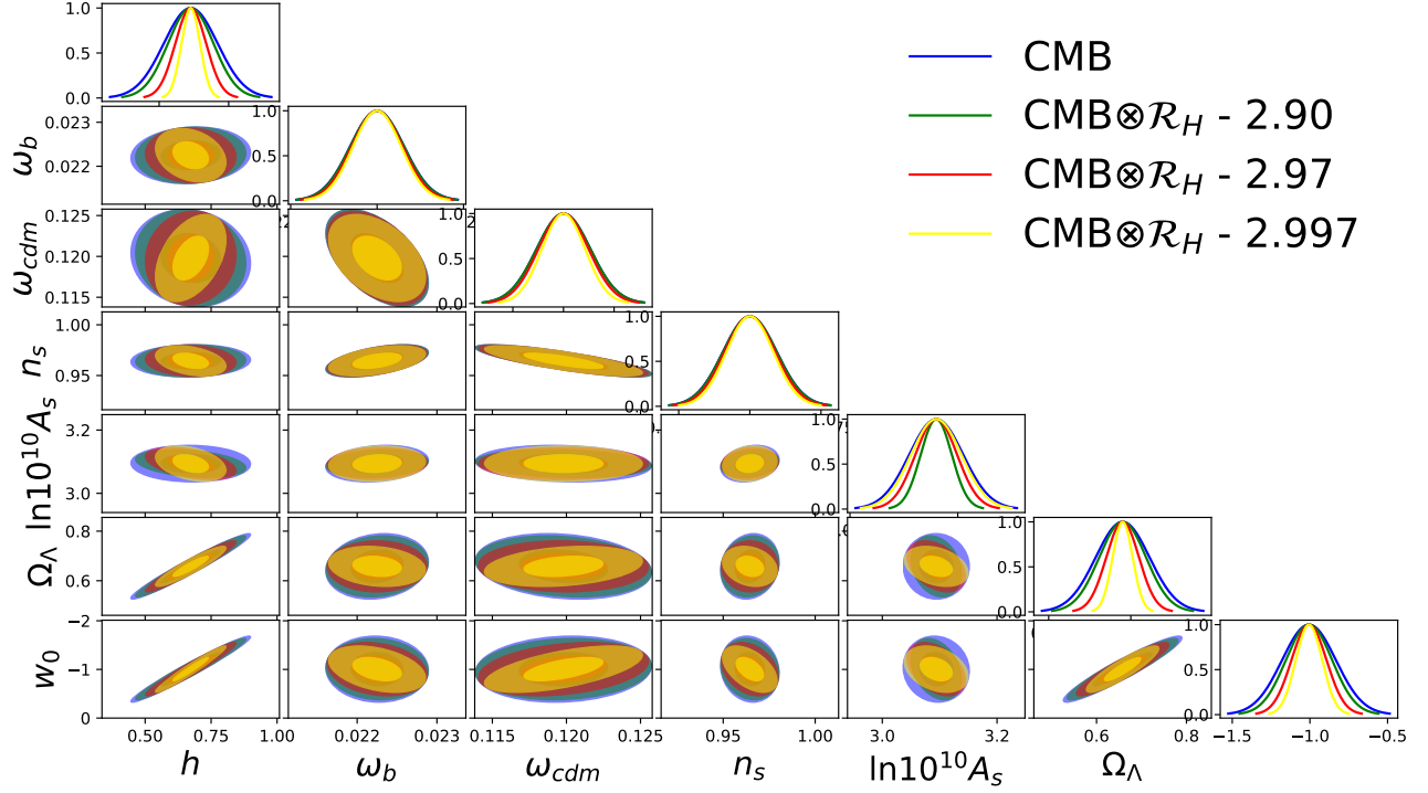
FIGURE 5.4: Fisher matrix showing the dependence of our estimation on the choice on the definition of the homogeneity scale. Different colors represent different combination of probes. The three different values correspond to the different thresholds on the definition of the Homogeneity scale, D_2(\mathcal{R}_H) = D_2^{nominal} , where D_2^{nominal} = 2.90, 2.97, 2.997
