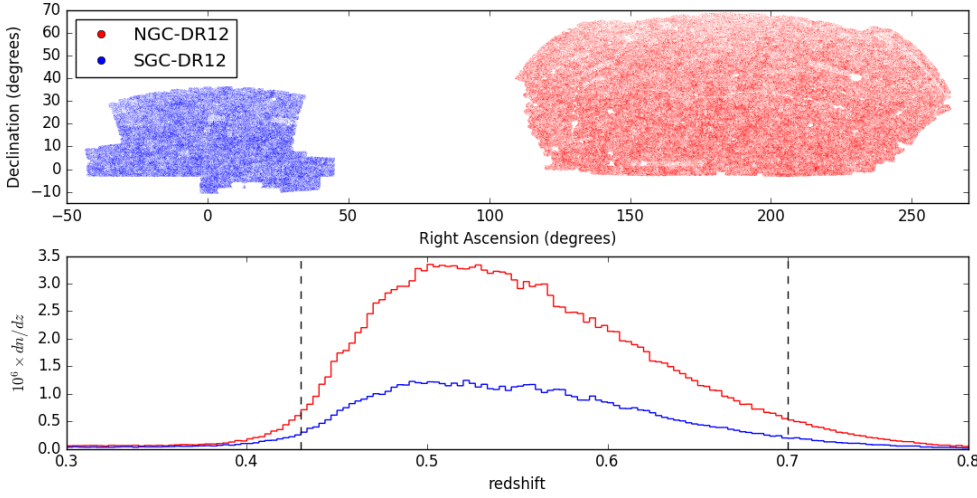
Figure 1. Right ascension and declination profiles (top) and redshift distribution (bottom) of the DR12 sample for the North (NGC) and South (SGC) Galactic Caps. The vertical dashed lines define the redshift interval used in our analysis.
