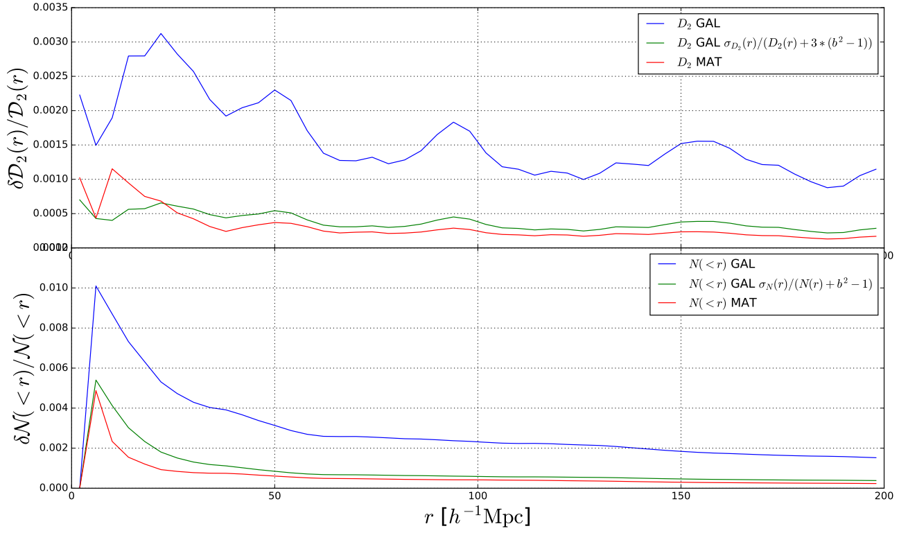
FIGURE 4.32: Top : D_2 -precision Bottom : N -precision for galaxy(blue) , matter(red) and the prediction-relation (green)
