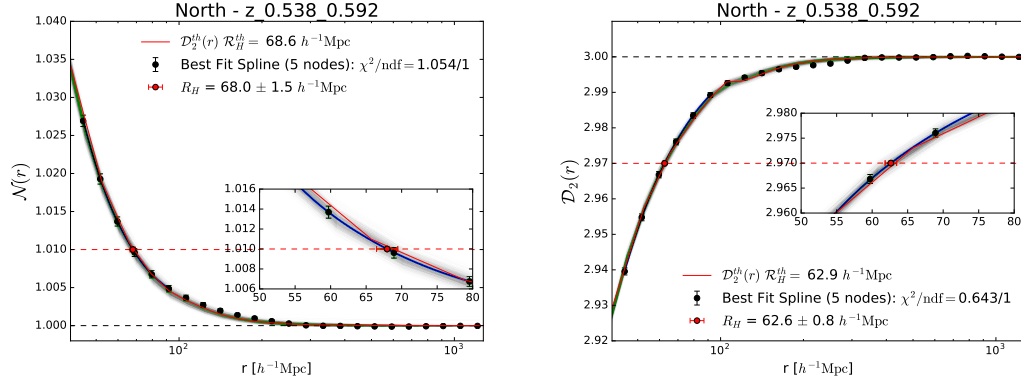
FIGURE 4.5: Same as figure 4.3 for matter distribution in the redshift interval 0.538 \leq z \leq 0.592 .
