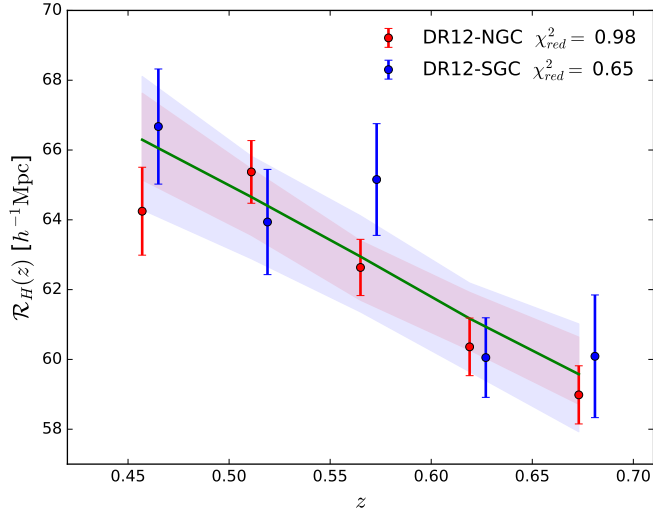
FIGURE 4.6: The homogeneity scale \mathcal{R}_H^{\mathcal{D}_2=2.97}(z) measured in the NGC (red) and in the SGC (blue) as a function of redshift. The green line is the \Lambda\text{CDM} model prediction. The shaded areas indicate the 1\sigma range for the 1000 QPM mock catalogs.
