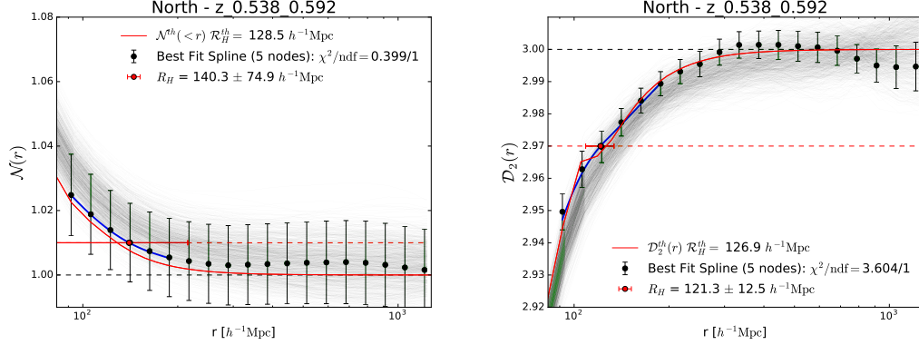
FIGURE 4.12: Same as figure 4.3 for the str-estimators in the redshift interval 0.538 \leq z \leq 0.592 .
