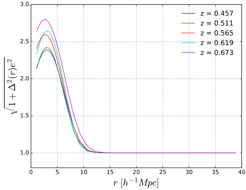
FIGURE 4.21: Boosting factor on the error in the correlation function as a function of scales, for all redshift bins (different colors).
