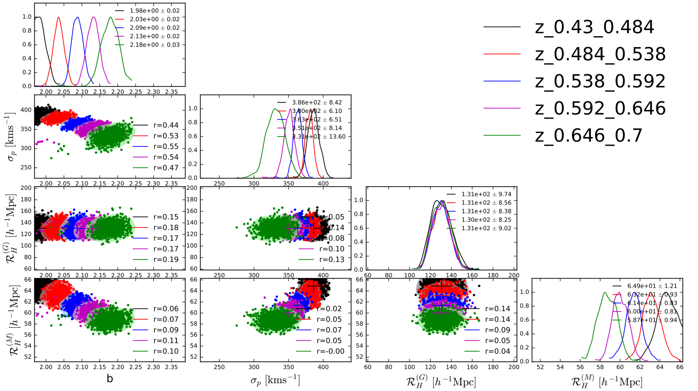
FIGURE 4.25: Homogeneity scale for the galaxy distribution measurement, \mathcal{R}_H^{(G)} or matter distribution, \mathcal{R}_H^{(M)} , versus bias, b , or peculiar velocities, \sigma_p , measurements for 1000 QPM mock catalogs on the North Galactic Cap for the different redshift bins color-coded. The contours show the 1\sigma and 2\sigma confidence regions. The normalised histograms with the mean and 1\sigma values are displayed for the two measurements. The correlation coefficient, r , is also displayed.
