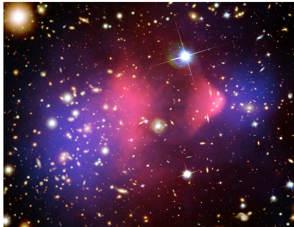
FIGURE 1.3: Composite image of the Bullet (star) Cluster observed by the Chandra X-ray Observatory [3]. We can see the X-ray(blue) and \gamma -ray (pink) radiation emitted by the collision of star cluster with another star cluster providing us with direct evidence of Dark Matter through gravitational lensing.
