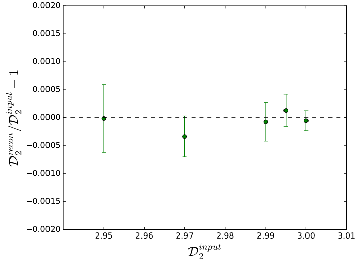
FIGURE 4.15: Reconstructed fractal correlation dimension, \mathcal{D}_2 , in the redshift interval z = 0.538 - 0.592 , averaged over r \in [15, 1300] h^{-1} \text{ Mpc} .
