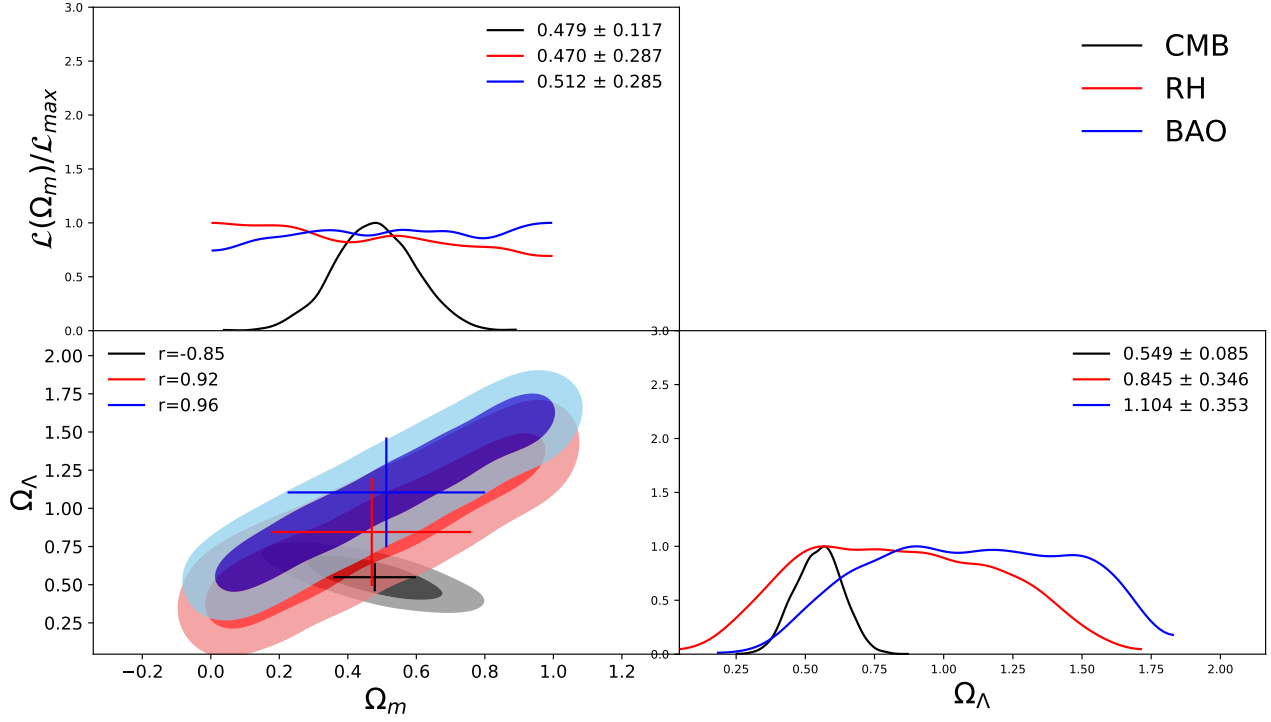
FIGURE 5.16: R_H + BAO combination results. see text for details.
