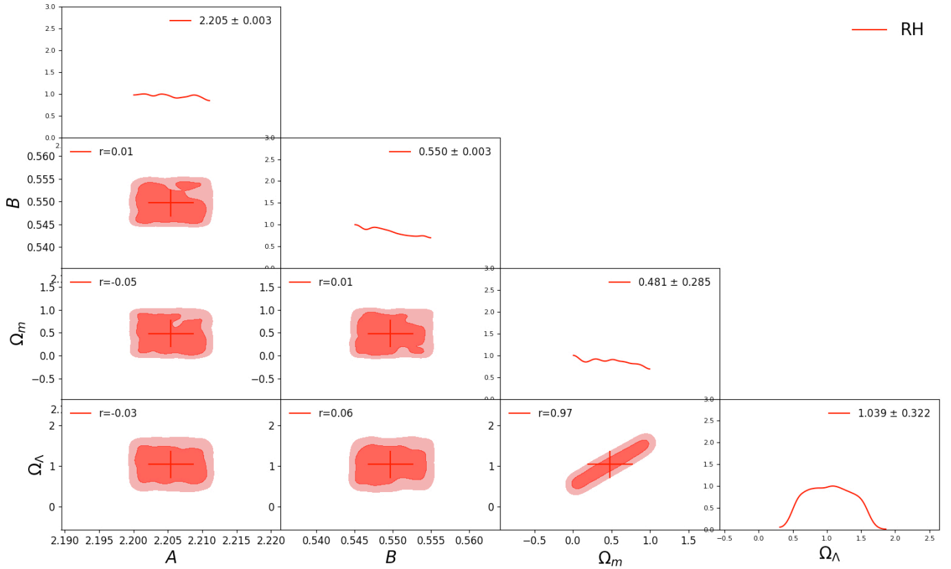
FIGURE 5.10: RH results. see text for details.
