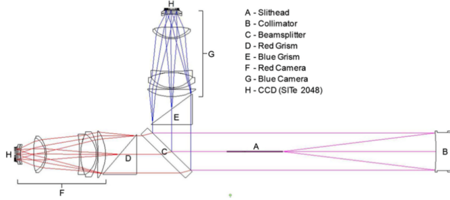
FIGURE 3.4: Optical layout of the SDSS spectrographs. Light enters each spectrograph through 320 fibers (180 \mu\text{m} diameter) terminating at a curved slit plate mounted inside the slithead. The slit plate positions the fiber ends on a radius concentric with the spherical collimating mirror (B). The 45 deg dichroic beamsplitter reflects the blue portion of the bandpass ( \lambda < 605 \text{ nm} ) and transmits the red wavelengths ( \lambda > 605 \text{ nm} ). Immediately after the beamsplitter in each channel is a grism (D,E), dispersing the light which exits the grisms and enters all-refractive, eight-element (F,G). Each camera contains a single 2^{11} \times 2^{11} CCD with 24\mu\text{m} pixels (H). [Image taken from Smee et al. [17]]
