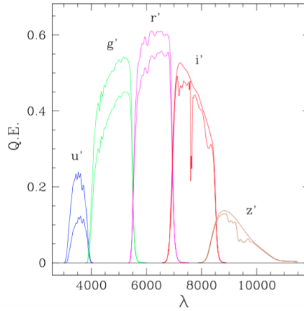
FIGURE 3.3: Quantum Efficiency of the telescope camera for the u,g,r,i,z photometric bands. The expected throughput of the optics is included; the lower of each pair of curves includes the expected atmospheric extinction. [Image taken from [16]]
