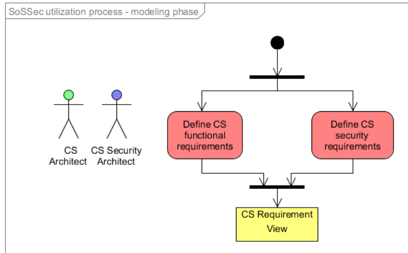
Fig. I.3.5 SoSSec utilization process - Modeling phase - Requirements definition
