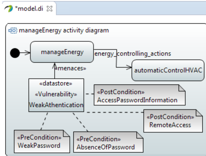
Fig. I.3.10 Smart Grid CS, manageEnergy activity diagram
