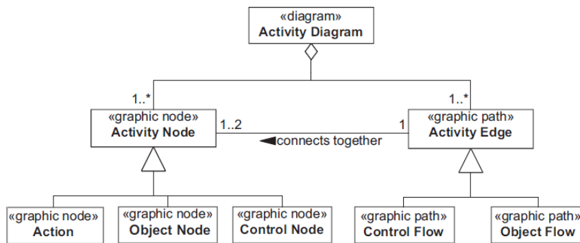
Fig. I.2.7 Part of the SysML activity diagram MetaModel, adapted from [97]
