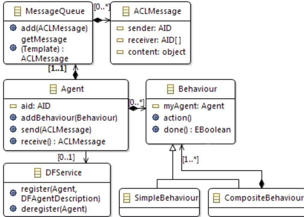
Fig. II.2.2 Part of the MAS MetaModel
