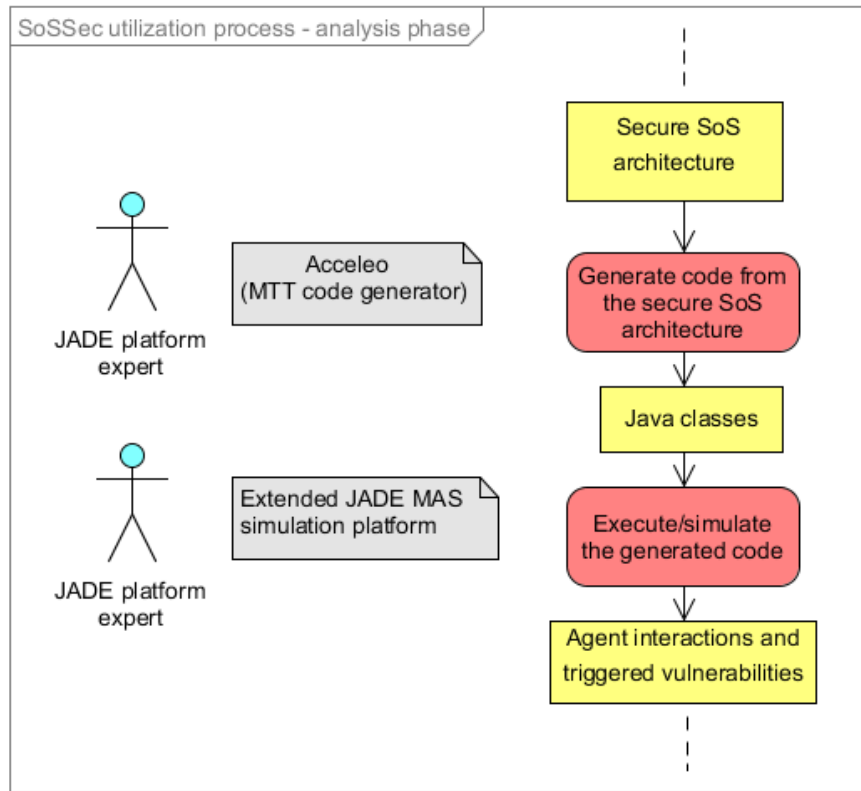
Fig. II.3.1 SoSSec Utilization Process - Analysis phase - Code Generation
