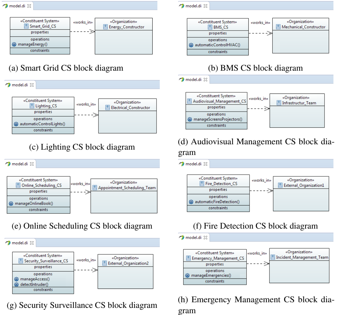
Fig. I.3.7 AHMS CS block diagrams
