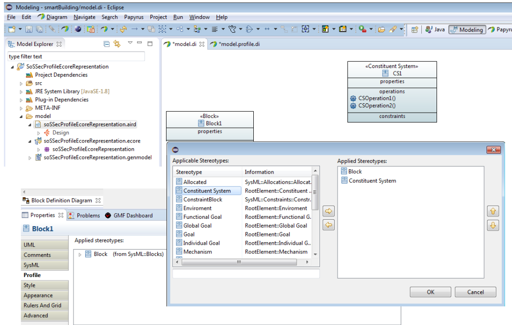
Fig. I.2.13 SoSSecML graphical editor defined as Papyrus extension
