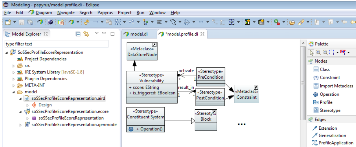
Fig. I.2.12 Part of the SoSSecML MetaModel implemented as Papyrus profile
