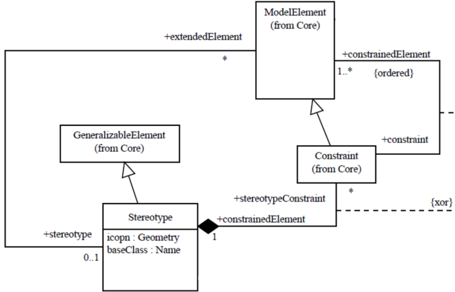
Fig. I.2.4 Profile definition mechanisms from [98]
