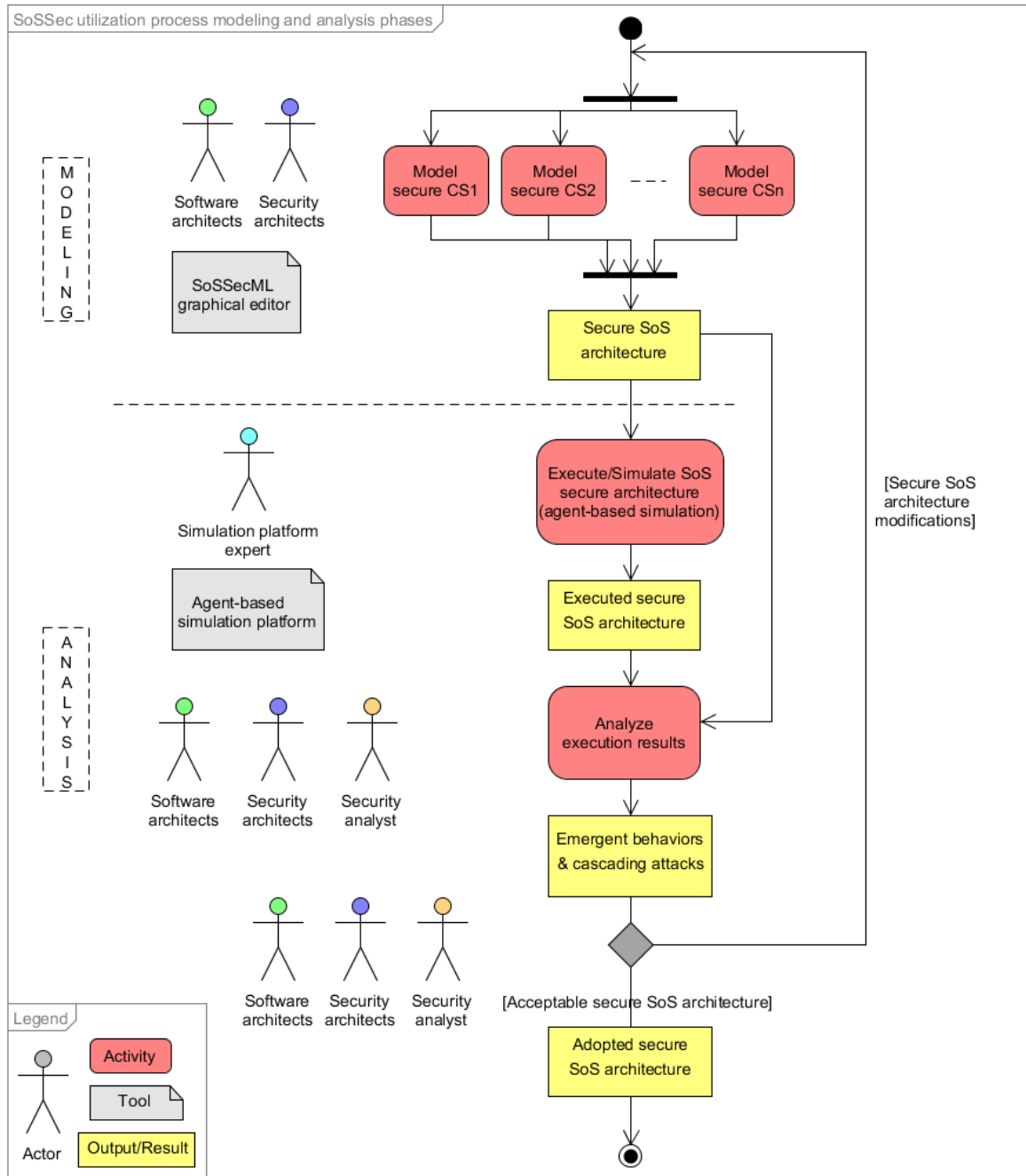
Fig. II.2.12 SoSSec utilization process - Modeling and Analysis phases
