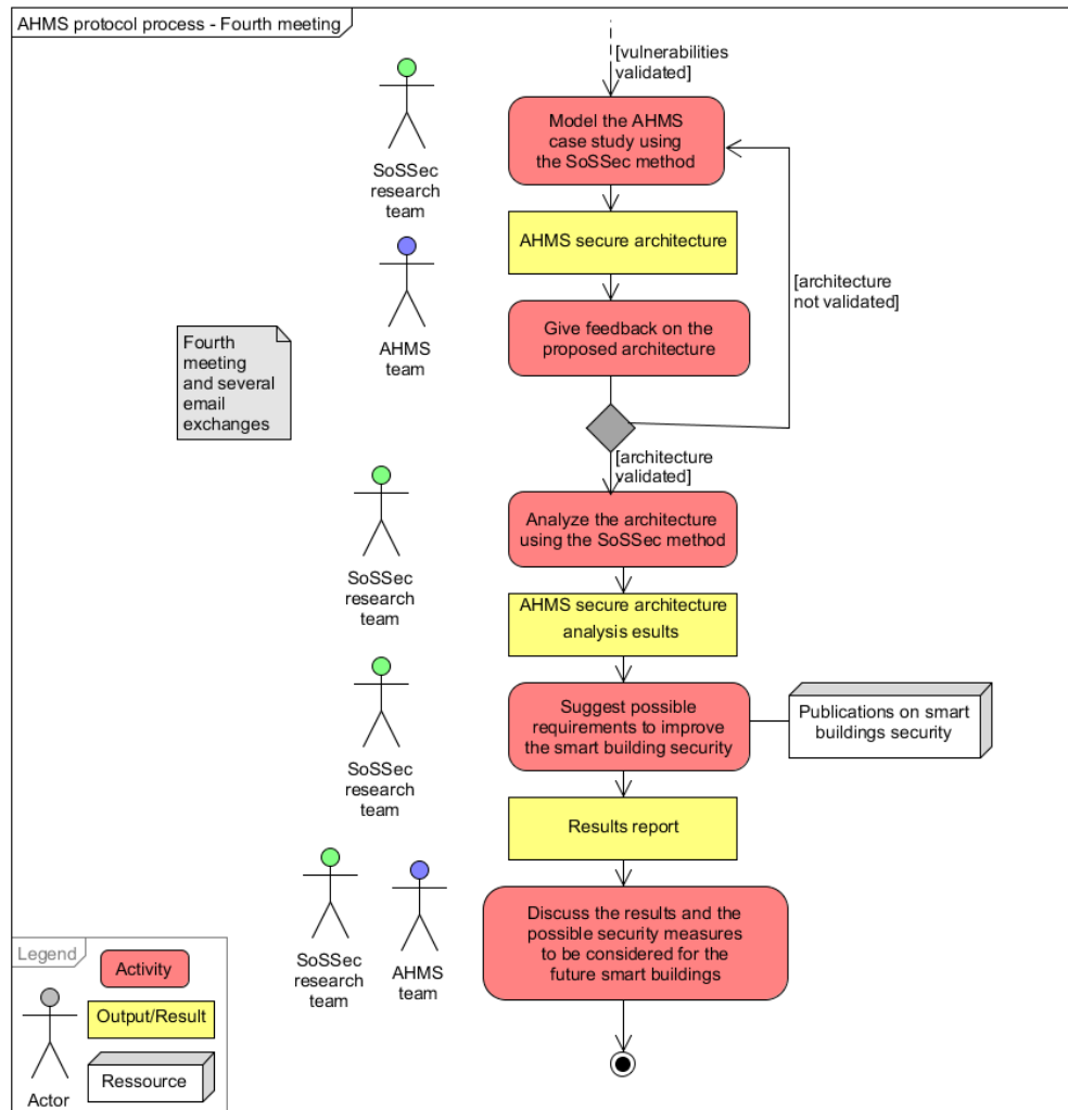
Fig. I.3.4 AHMS planning protocol - Fourth meeting
