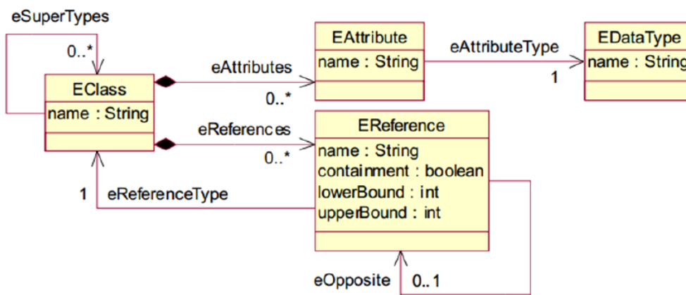
Fig. I.2.10 Part of the Ecore MetaMetaModel in EMF from [80]
