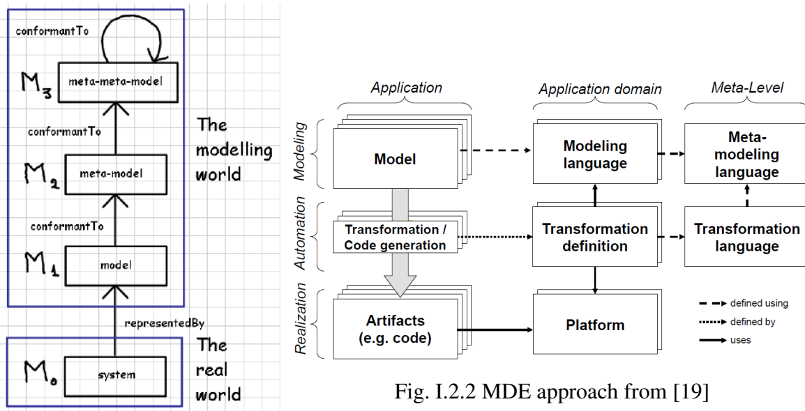
Fig. I.2.1 Model driven architecture levels from [15]
