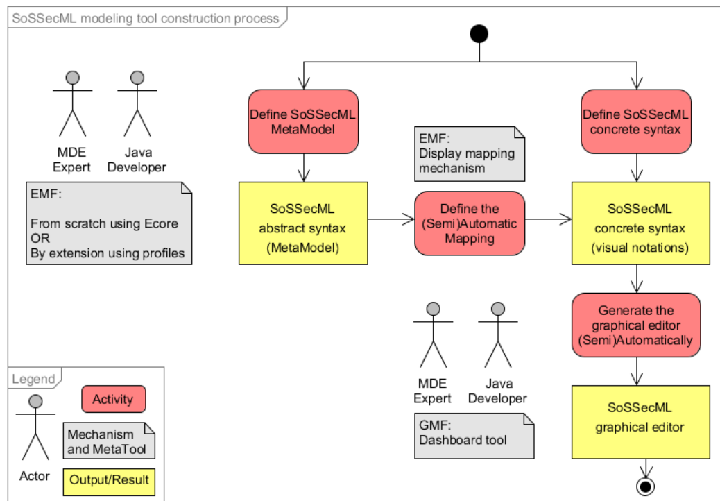
Fig. I.2.9 SoSSec modeling tools construction process
