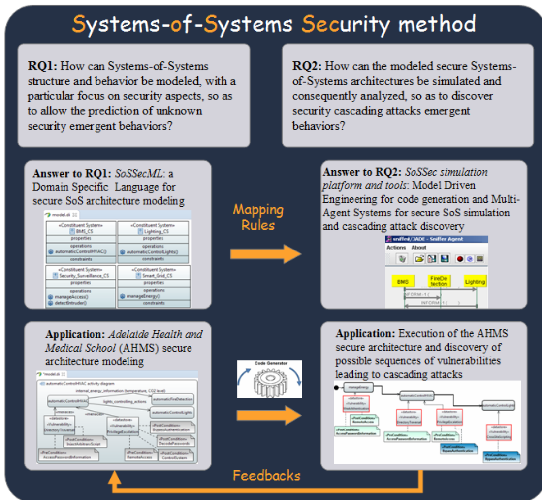
Fig. II.3.11 SoSSec method for secure SoS modeling and analysis
