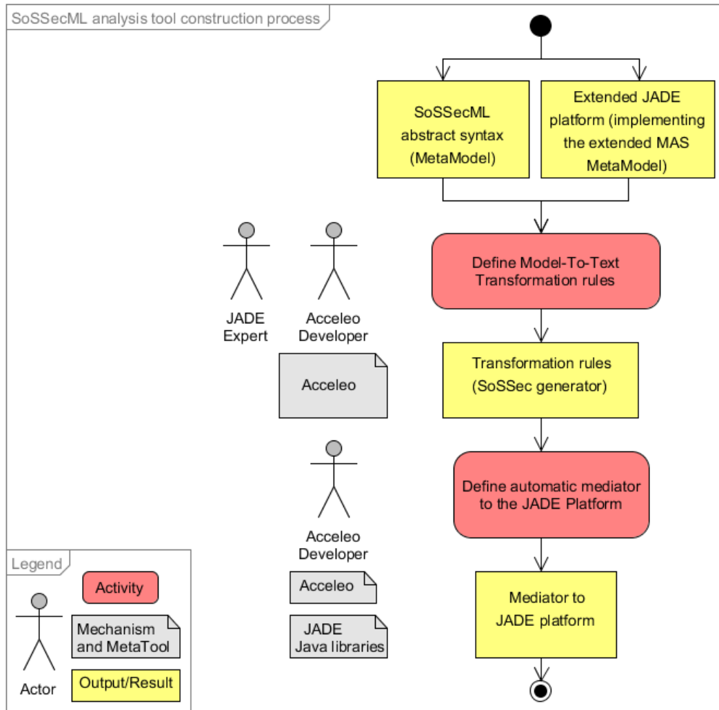
Fig. II.2.8 SoSSec analysis tool construction process
