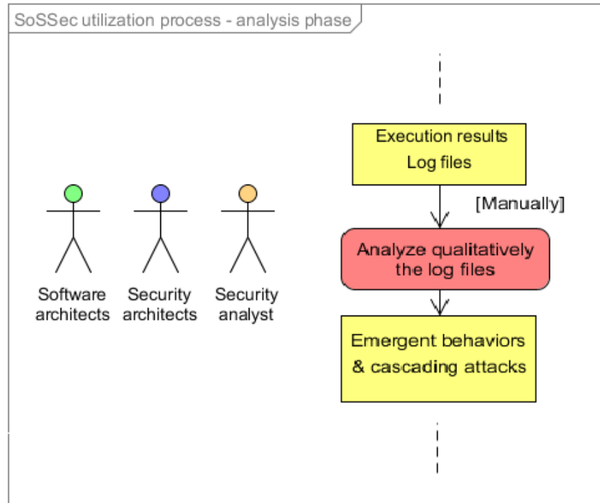
Fig. II.3.4 SoSSec Utilization Process - Analysis phase - Qualitative Analysis
