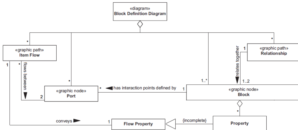
Fig. I.2.6 Part of the SysML block definition diagram MetaModel, adapted from [97]
