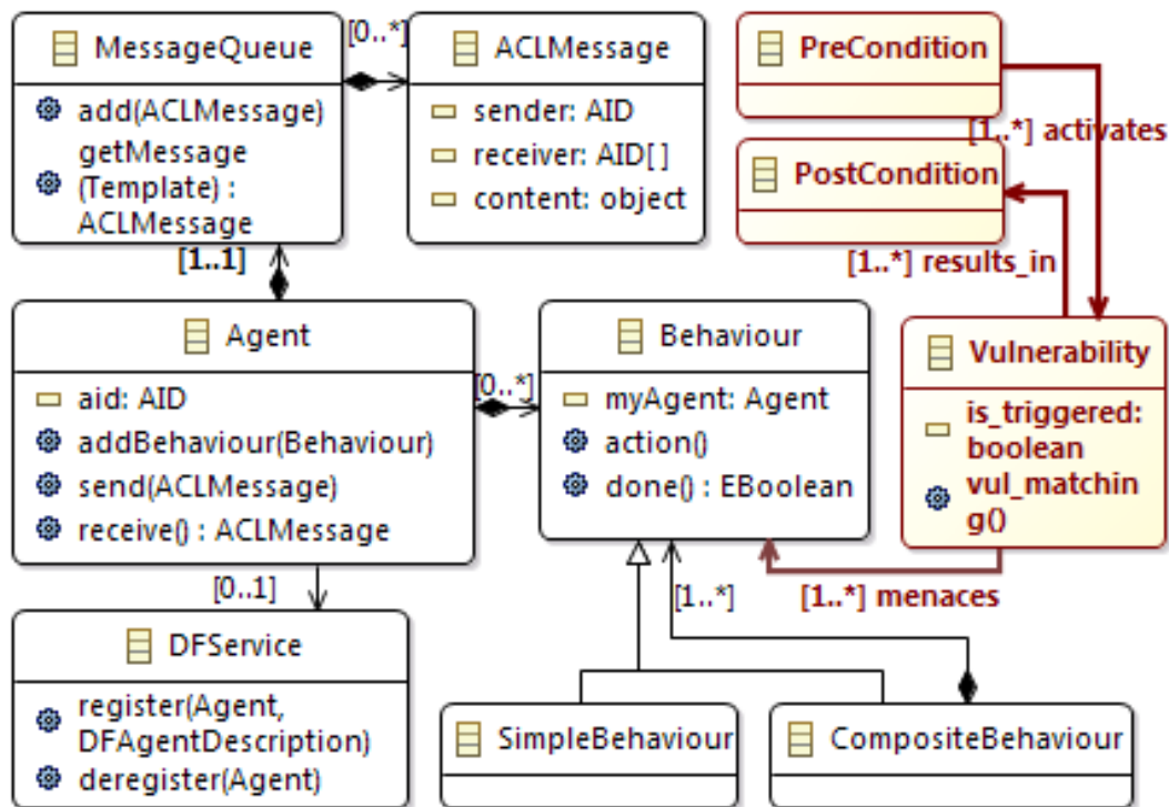
Fig. II.2.4 Part of the MAS MetaModel with the security extension
