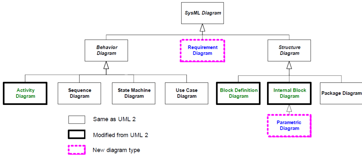
Fig. I.2.5 SysML Diagrams from [97]
