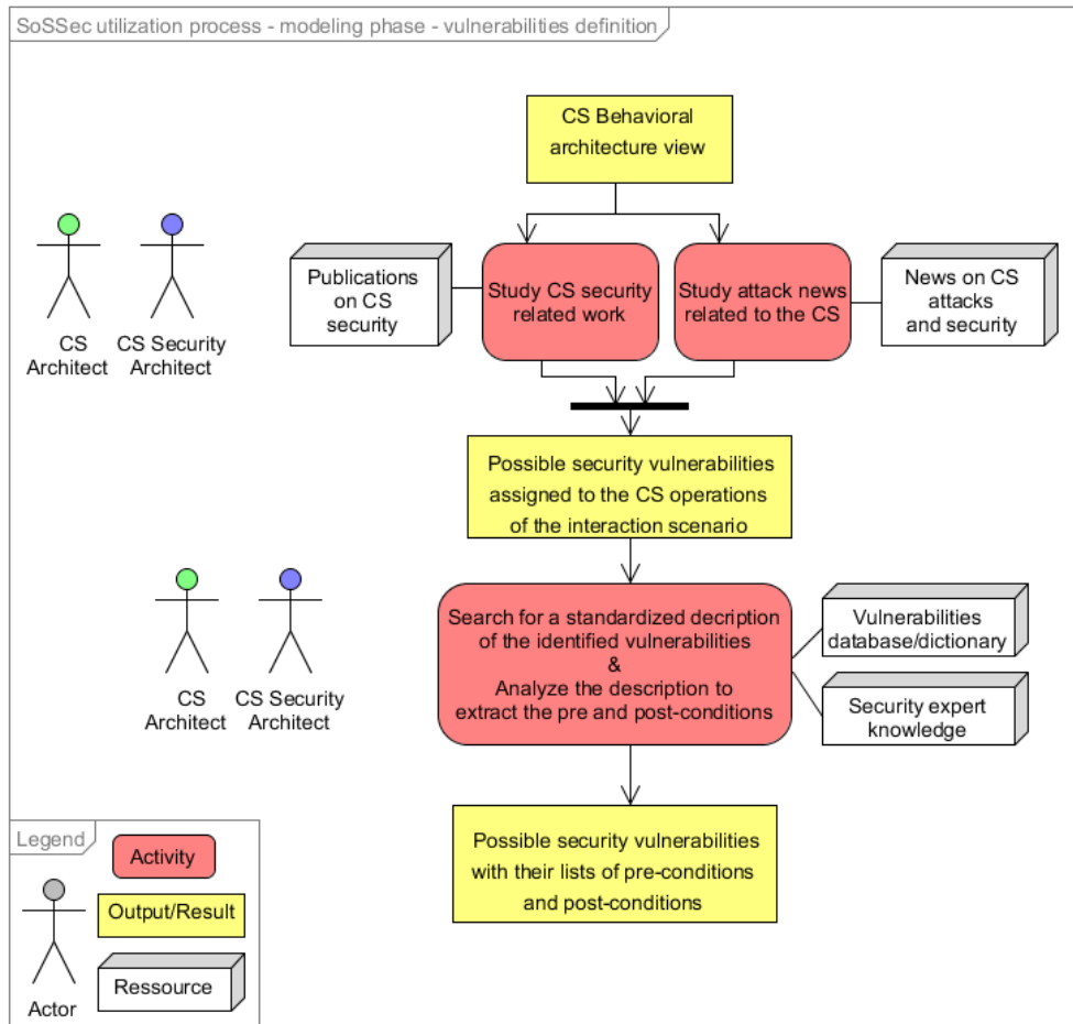
Fig. I.2.16 SoSSec utilization process - modeling phase - vulnerabilities definition
