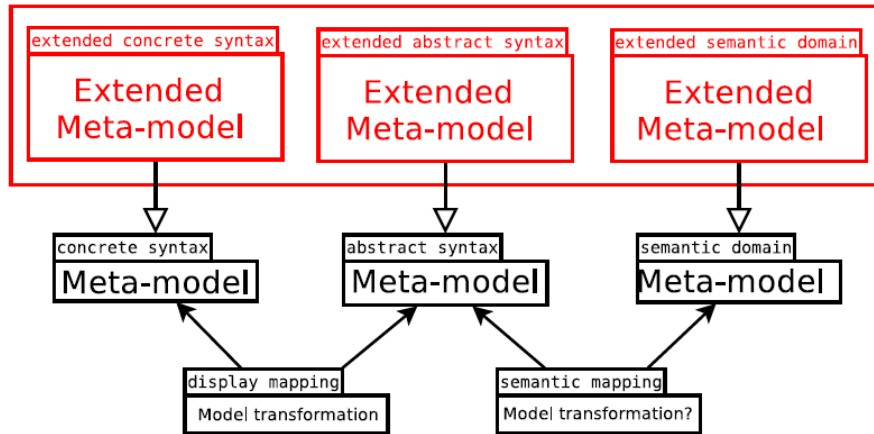
Fig. I.2.3 MetaModeling approach for DSL definition from [27]
