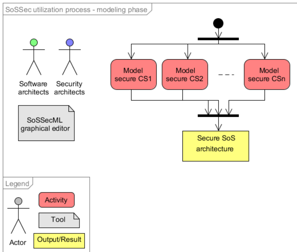
Fig. I.2.14 SoSSec utilization process - Modeling phase
