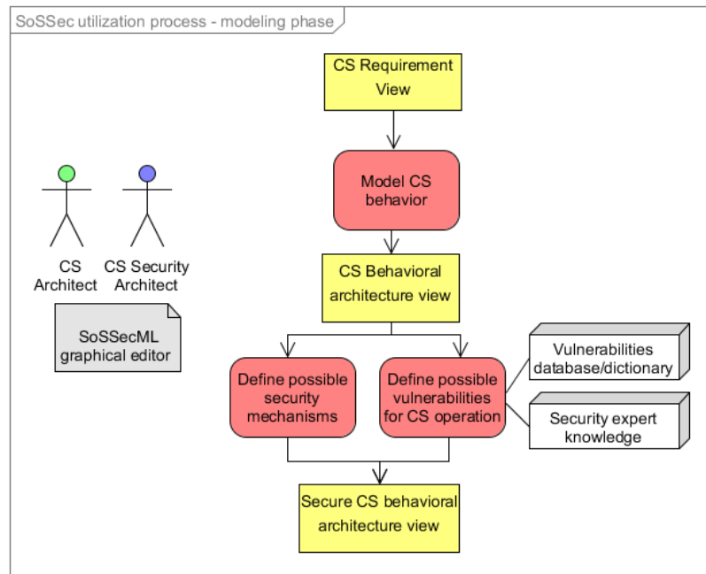
Fig. I.3.8 SoSSec utilization process - Modeling phase - Behavior Modeling
