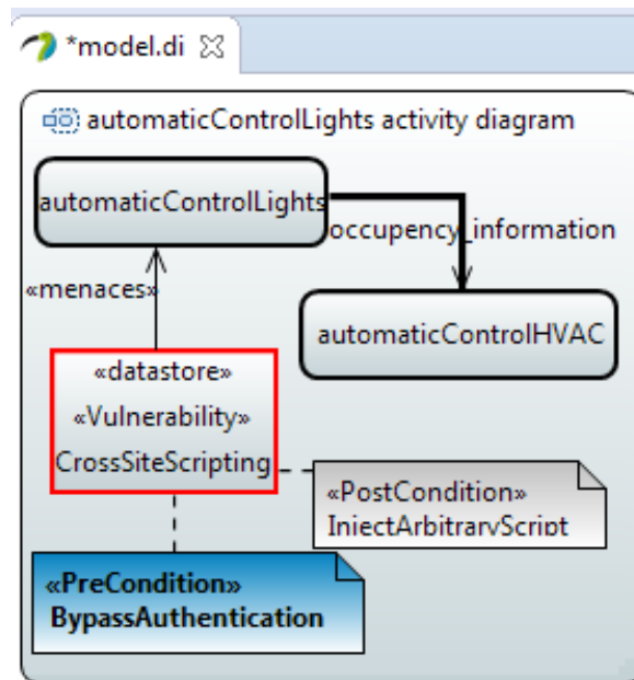
Fig. II.3.8 Lighting CS - triggered vulnerability on automaticControlLights operation
