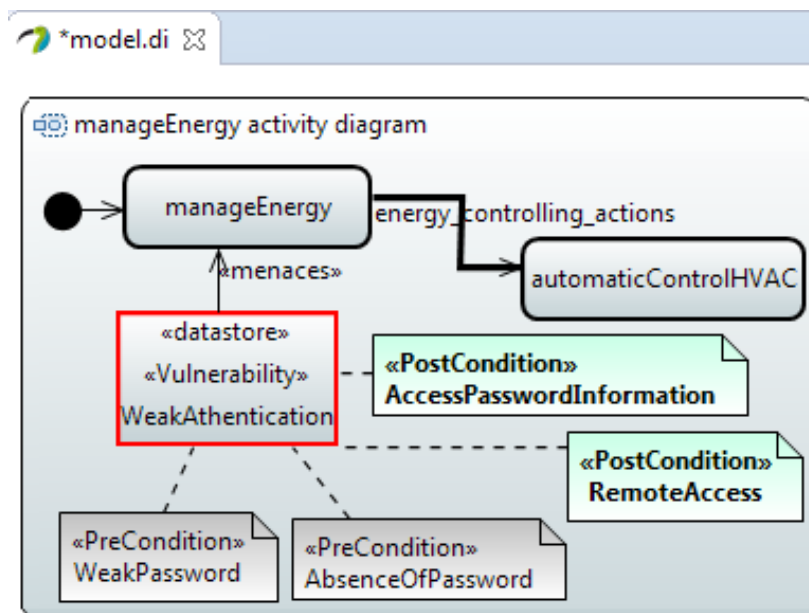
Fig. II.3.6 Smart Grid CS - triggered vulnerability on manageEnergy operation
