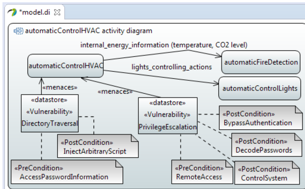
Fig. I.3.11 BMS CS, automaticControlHVAC activity diagram
