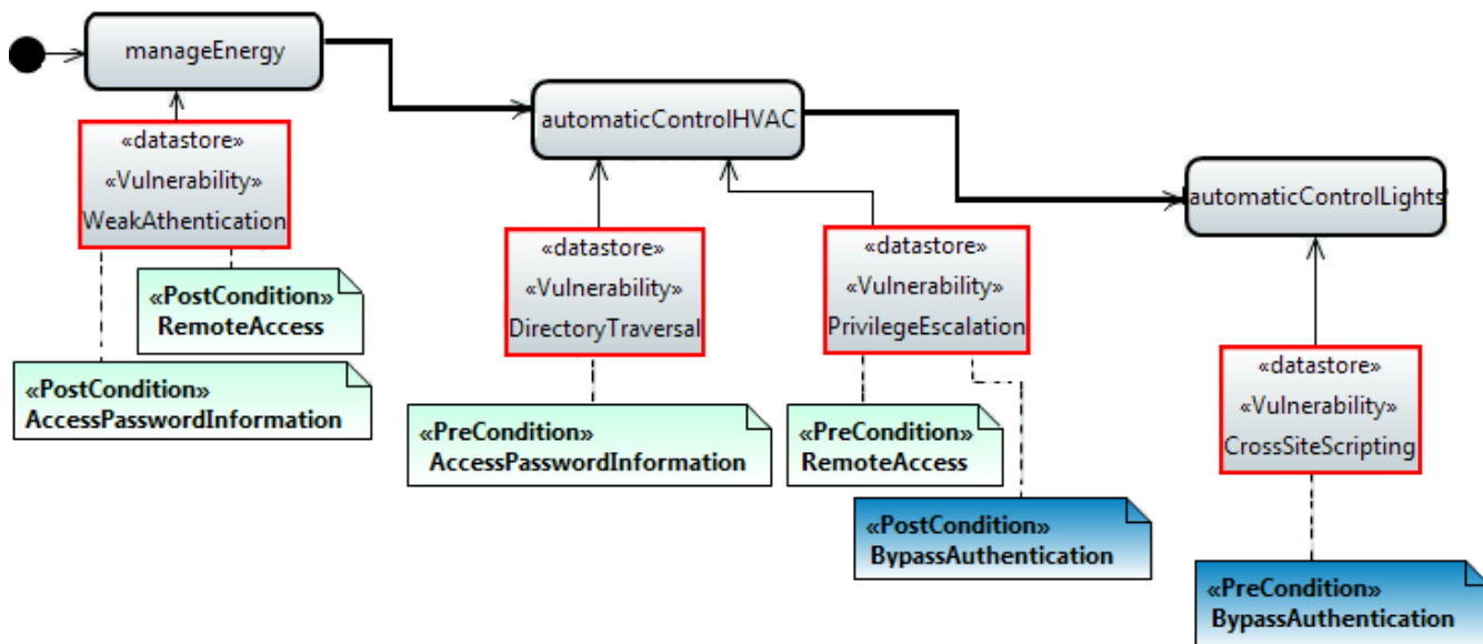
Fig. II.3.9 AHMS smart building cascading attack
