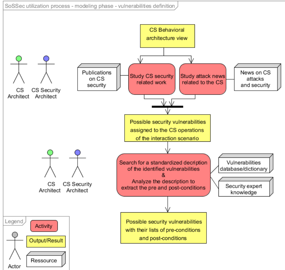
Fig. I.3.9 SoSSec utilization process - modeling phase - vulnerabilities definition
