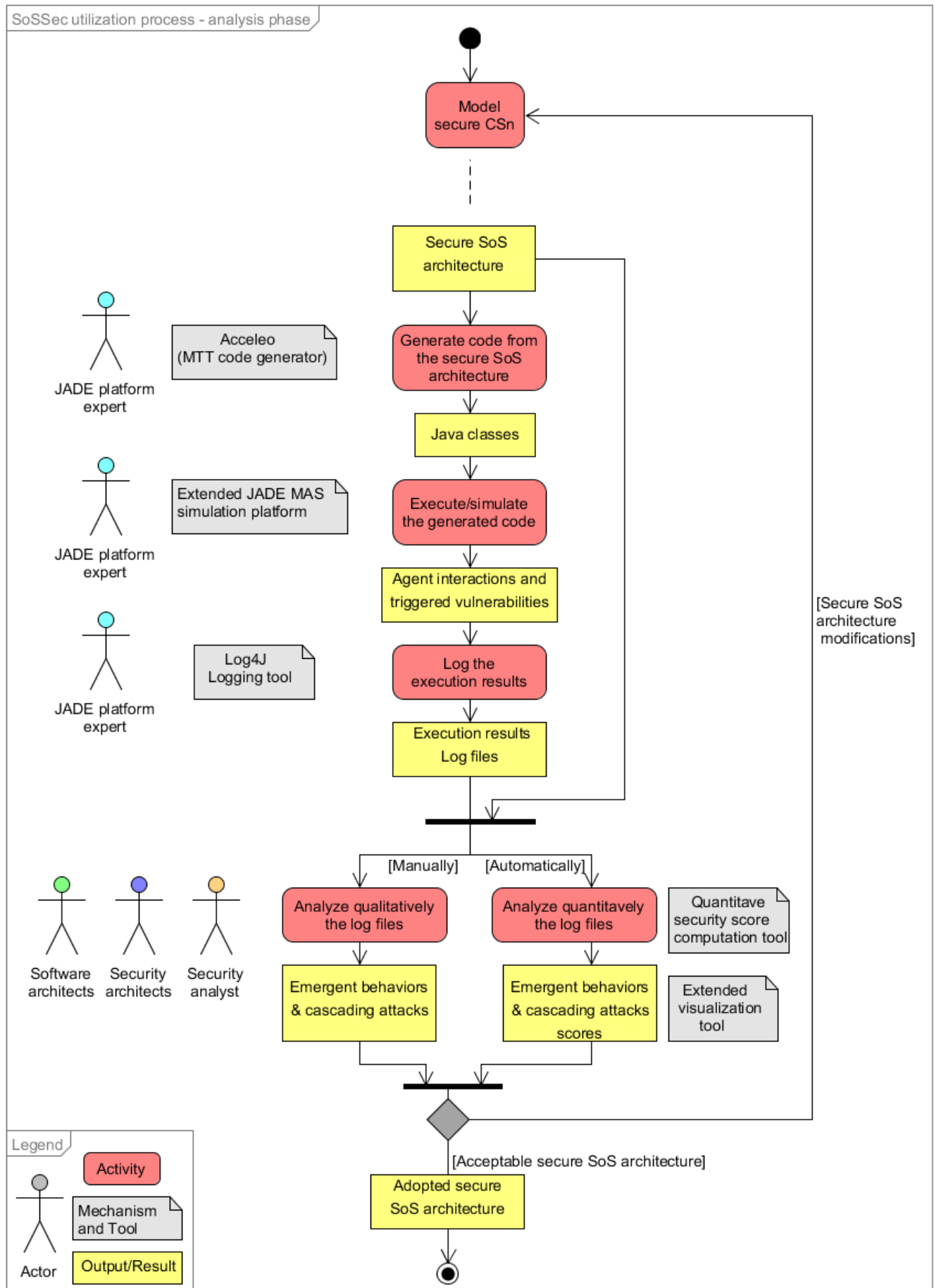
Fig. II.2.13 SoSSec utilization process - Analysis phase
