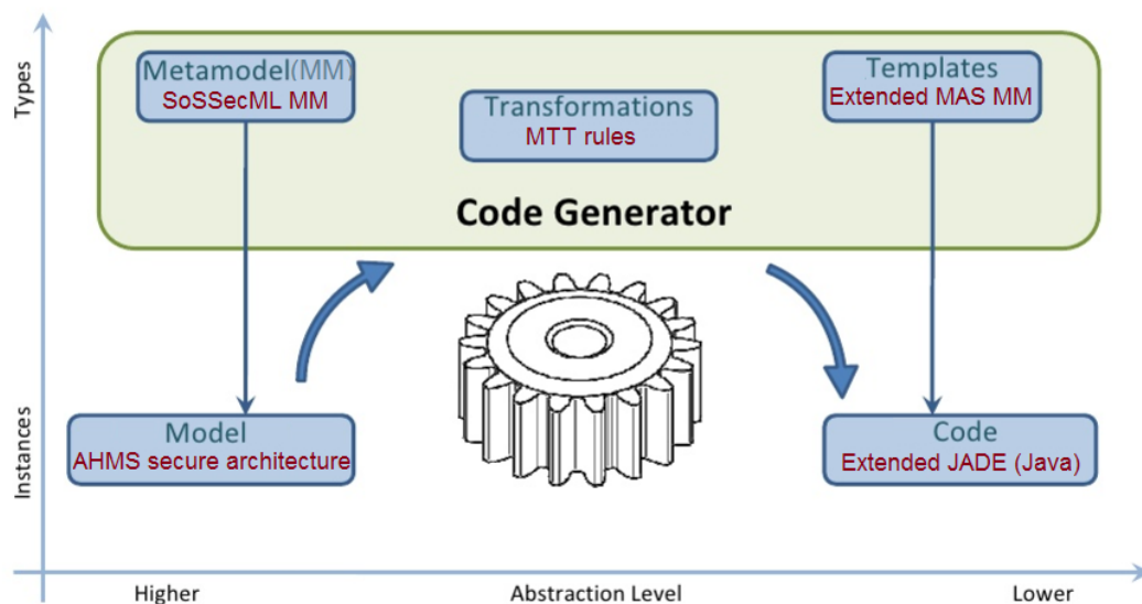
Fig. II.2.7 Conceptual map for code generation from [82]
