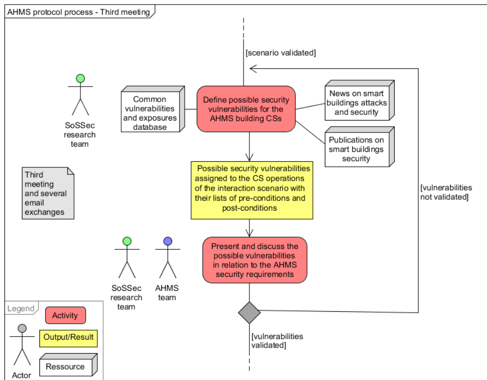
Fig. I.3.3 AHMS planning protocol - Third meeting
