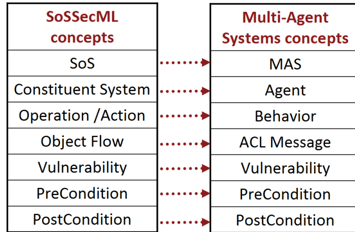
Fig. II.2.5 SoSSecML MetaModel and MAS MetaModel concepts alignment
