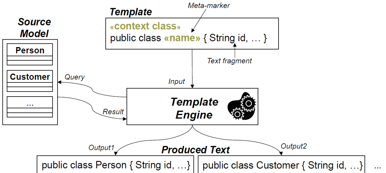
Fig. II.2.9 Template-based approaches from [19]
