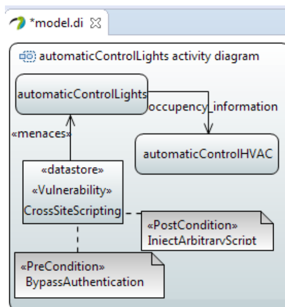
Fig. I.3.12 Lighting CS, automaticControlLights activity diagram
