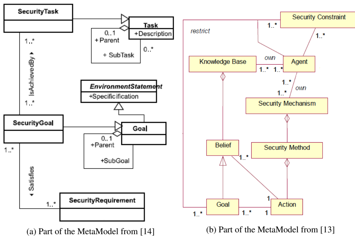
Fig. II.2.3 Security-aware MAS MetaModel proposed in [14][13]
