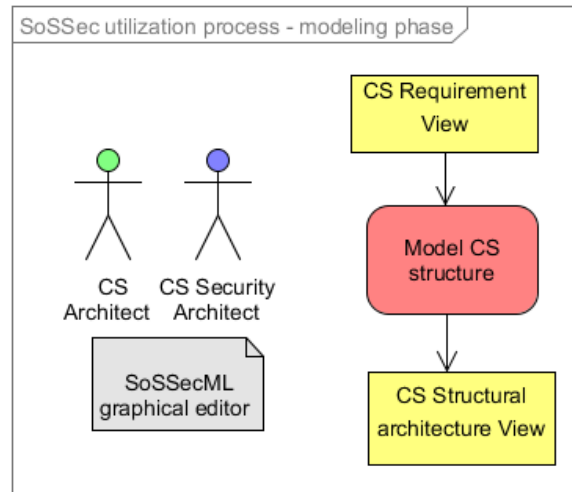
Fig. I.3.6 SoSSec utilization process - Modeling phase - Structure Modeling
