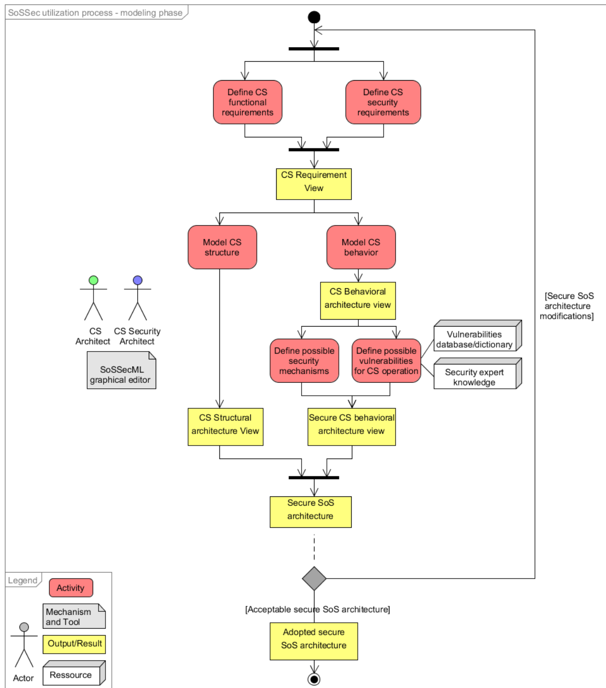
Fig. I.2.15 SoSSec utilization process - Detailed modeling phase
