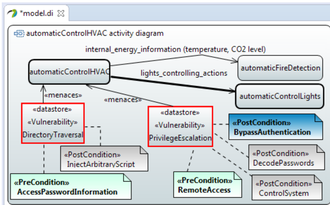
Fig. II.3.7 BMS CS - triggered vulnerability on automaticControlHVAC operation
