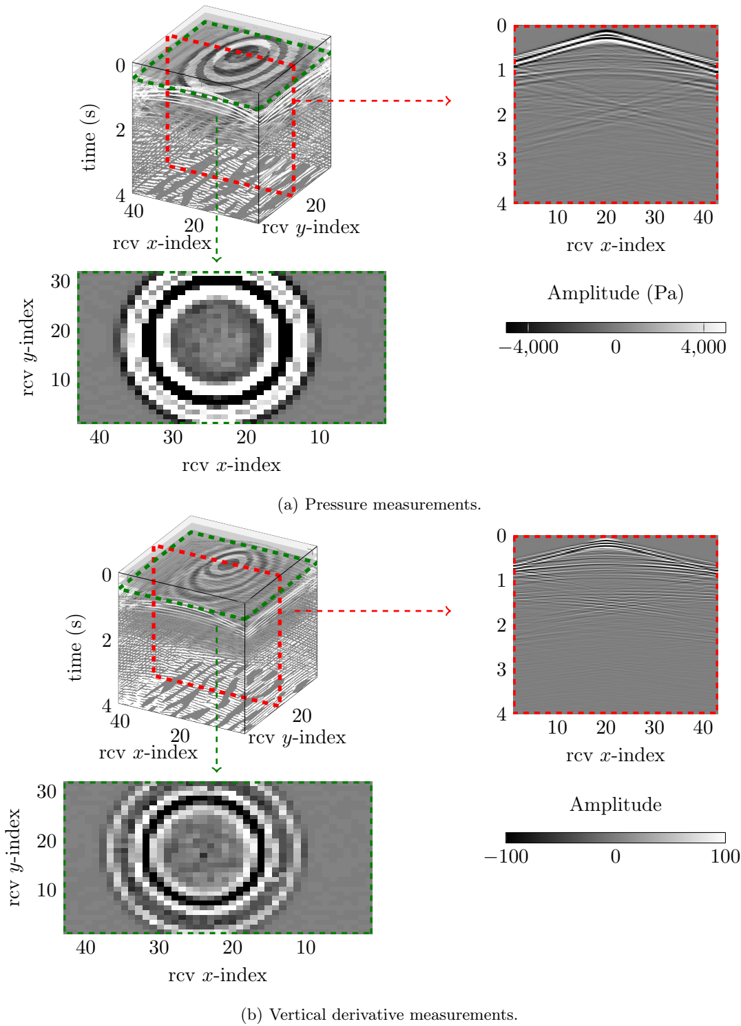
Figure 7.3: Three-dimensional trace associated with a centrally located source. A two-dimensional section at a fixed time t = 0.5 s is pictured in the bottom left of each figure, and is indicated in green in the 3D visualization. The upper right of each figure selects a fixed line receivers positioned at y = 695 m, which is indicated by the red dashed line in the 3D visualization.
