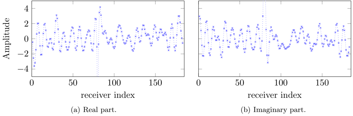
Figure 4.3: Discrete Fourier transform of the seismic trace Figure 4.2(b) at 5 Hz. For every receiver index k the Fourier domain complex value is given by \hat{S}_k , as indicated in Equation (4.1)
