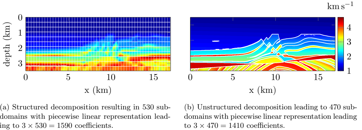
Figure 3.9: Piecewise linear decomposition of the model pictured Figure 3.8 from structured and unstructured decision resulting in about 0.25% of the original number of coefficients. The subdomains are indicated with the white lines.
