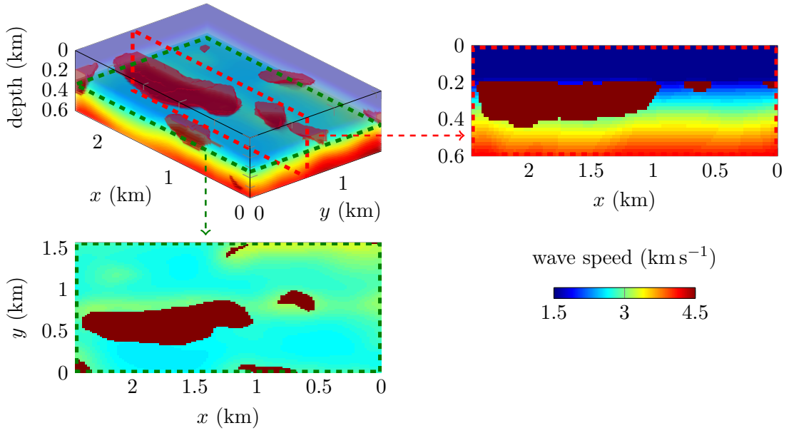
Figure 6.37: Wave speed for the three-dimensional acoustic Louro medium of size 2.46 \times 1.56 \times 0.6 km (courtesy of Total). The velocity varies between 1500 and 4500 \text{ m s}^{-1} . Vertical section at y = 680 m is indicated with the red dashed frame and plotted in the right. The horizontal section at fixed depth z = 340 m is indicated with the green frame and shown at the bottom.
