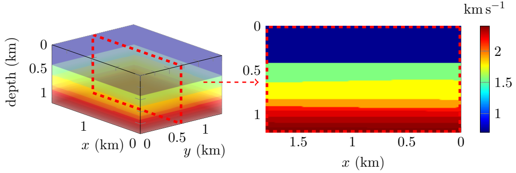
Figure 6.69: S-wave speed for the three-dimensional elastic Epati medium of size 1.8 \times 1.4 \times 1.2 km (courtesy of Total). The velocity varies between 700 and 2400 \text{ m s}^{-1} . Vertical section at y = 700 m is indicated with the red dashed frame and pictured in the right.
