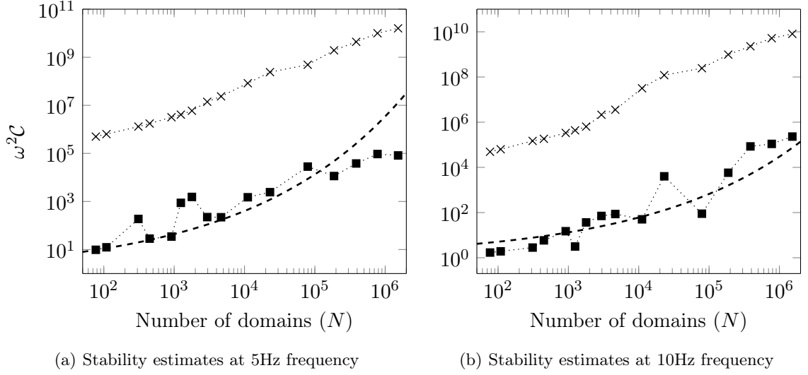
Figure A.7: Comparison of the computational stability estimates using partial data only located on the top boundary (·×·) and using the full boundary data (·■·). The dashed line (---) represents the analytical lower bound as found in Figure A.4.
