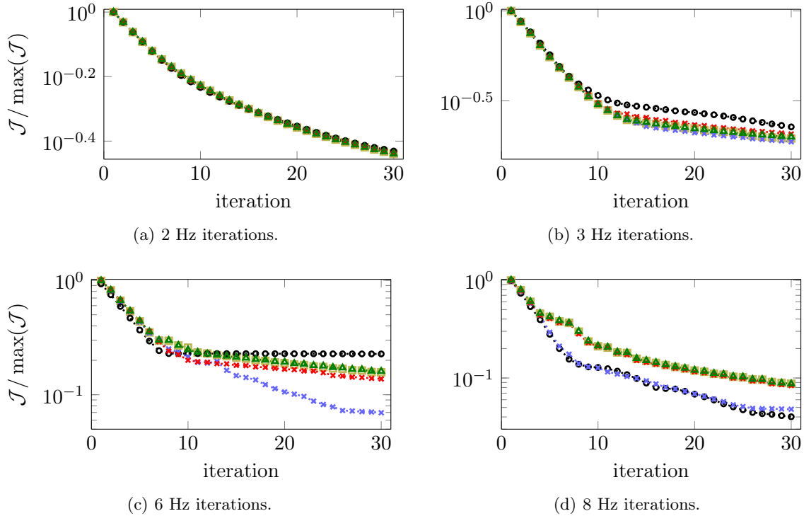
Figure 4.6: Evolution of the cost function for different frequencies using the nonlinear conjugate gradient method. The black circles ( \bullet\bullet\bullet ) use the Fletcher–Reeves (FR) formula, the blue crosses ( \times\times\times ) the Polak–Ribière (PR) formula, the red crosses ( \times\times\times ) the Hestenes–Stiefel (HS) formula and the green triangles ( \triangle\triangle\triangle ) the Dai–Yuan (DY) formula. The yellow squares ( \square\square\square ) uses the gradient descent algorithm. At every frequency, the cost function progression is scaled with the value of the first iteration.
