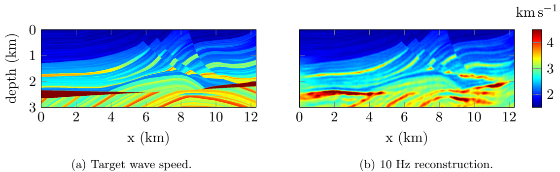
Figure 6.53: 2D reconstruction of the Marmousi wave speed with synthetic data covering frequencies from 1 to 10 Hz. The dimensions are artificially increased to the size 12.3 \times 3 km. The initial model used for the algorithm is given in Figure 6.4.
