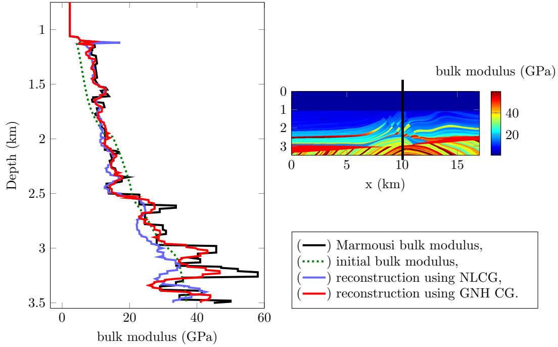
Figure 4.20: One-dimensional profile of the acoustic Marmousi bulk modulus for a fixed position x = 10 km. The position is indicated with the black line on the original Marmousi bulk modulus (right). The reconstructed profiles are extracted from the results presented Figure 4.19.
