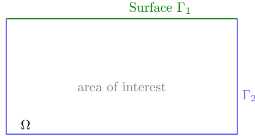
Figure 4.1: Notation for the domain of interest \Omega , \Gamma_1 denotes the upper boundary, \Gamma_2 = \Gamma/\Gamma_1 the others. The upper boundary usually consists in a free surface characterizing the interface between the air and the medium. On the other hand the lateral and bottom boundaries have to reflect the natural continuation of the Earth.
