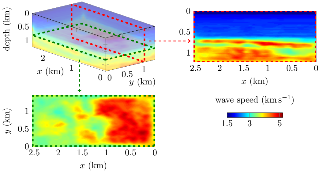
Figure 7.14: Application of a Gaussian smoothing filter (see Remark 7.3) onto the reconstruction of the acoustic 3D Statoil wave speed from Cauchy data using frequencies from 3 to 15 Hz, and the cost function \mathcal{J}_G (Equation (7.4)). The set of sources is different between the observations and the simulations, see Table 7.2.
