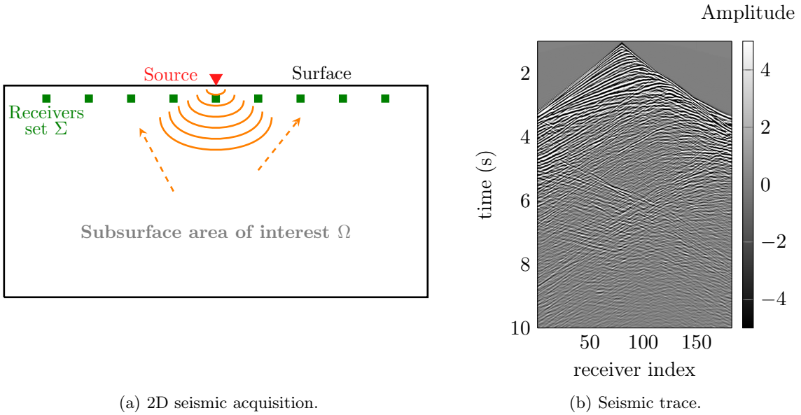
Figure 4.2: (a): Illustration of seismic acquisition for a two-dimensional domain for a single source positioned at the surface which is represented by the red triangle. The wave propagates through the area of interest, then subsurface structures reflect part of the wave (indicated with the dashed arrows). The receivers (represented by the squares) record the resulting signal (direct wave and reflections).
