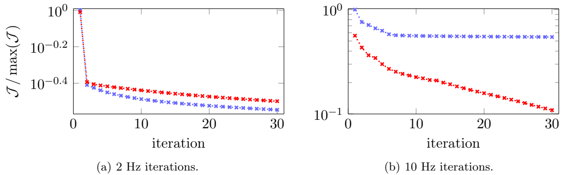
Figure 4.13: Evolution of the cost function for different frequencies. The blue crosses ( \cdots \times \cdots ) involve the Polak–Ribière (PR) formula, the red crosses ( \cdots \times \cdots ) use the Gauss-Newton Hessian with 10 conjugate gradient iterations and diagonal preconditioner with value 10^{-4}\beta (see Equation (4.42)).
