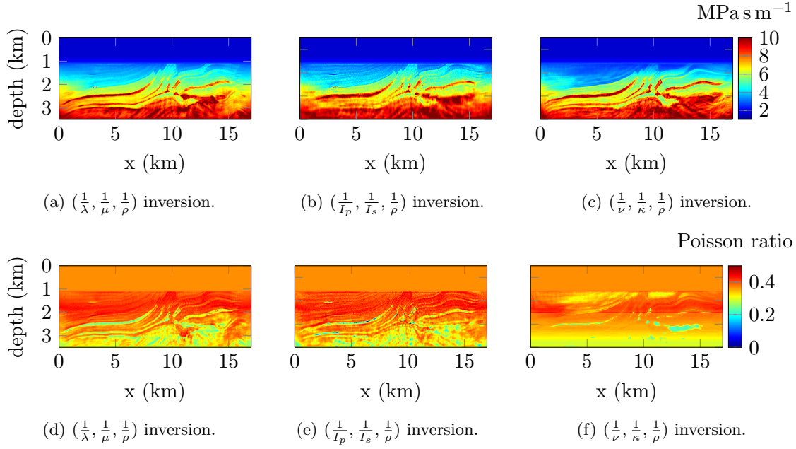
Figure 5.48: Final reconstruction after 10 Hz iterations of the Marmousi P-impedance (top) and Poisson ratio (bottom) using different parametrizations. The density is kept fixed with the iterations, to its initial representation.
