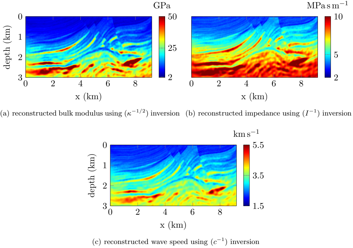
Figure 5.43: Final reconstruction after 10 Hz iterations of the Marmousi model using different parametrization and keeping the density fixed as its initial value pictured Figure 5.39(b).
