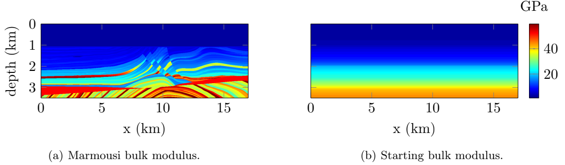
Figure 4.17: True and initial bulk modulus related to the acoustic Marmousi medium with variable density, the corresponding velocity and density have been shown in Figures 4.15 and 4.16.
