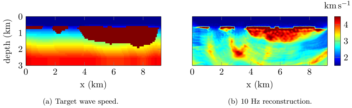
Figure 6.52: 2D reconstruction of wave speed including salt domes with data covering frequencies from 1 to 10 Hz. The models on the left represent the target model (from which the observations are acquired). The domain has size 9.225 \times 3 km. The larger salt dome is approximately located between 500 and 2000 m. The initial model used for the algorithm is given in Figure 6.47.
