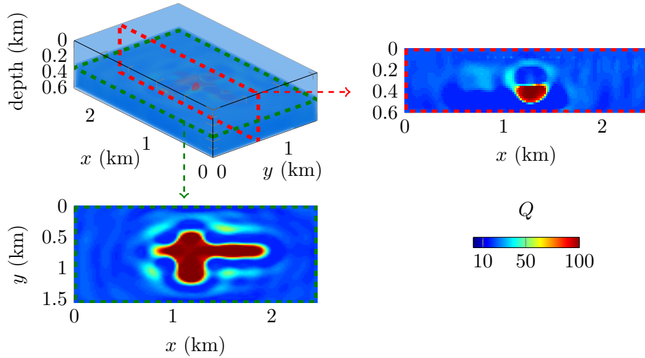
Figure 6.57: Reconstructed attenuation factor of the three-dimensional acoustic model with attenuation and the subsurface cross-shaped body. Vertical section at y = 680 m and horizontal section at fixed depth z = 400 m are detailed.
