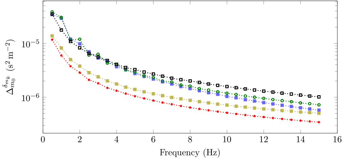
Figure 5.6: Evolution of the interval size verifying the deflection condition, quantity \Delta_{m_0}^{\delta_{m_k}} , with frequency using m_0 as a smooth velocity background and different directions \delta_{m_k} . The blue squares ( \cdots\blacksquare\cdots ) employ one reflector ( \delta_{m_1} , Figure 5.5(a)), the green circles ( \cdots\bullet\cdots ) two reflectors ( \delta_{m_2} , Figure 5.5(b)) the red stars ( \cdots\star\cdots ) one large reflector ( \delta_{m_3} , Figure 5.5(c)) and the black squares ( \cdots\blacksquare\cdots ) the reflectors extracted from the Marmousi model ( \delta_{m_m} , Figure 5.5(d)). The yellow squares ( \cdots\blacksquare\cdots ) represent the estimates using constant direction.
