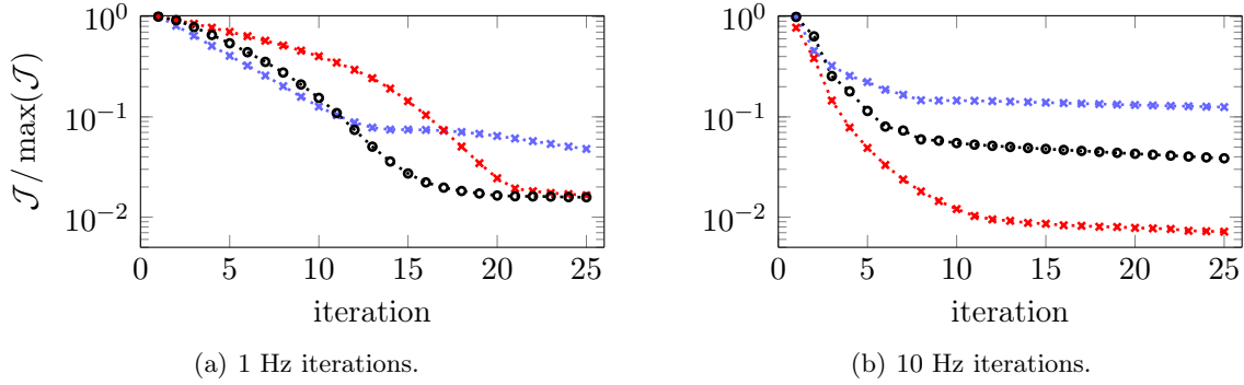
Figure 4.18: Evolution of the cost function for different frequencies using different methods for the model update. The blue crosses ( \cdots \times \cdots ) use the Fletcher–Reeves (FR) nonlinear conjugate gradient. The red crosses ( \cdots \times \cdots ) use the Gauss-Newton Hessian CG approximation. The black circles ( \cdots \bullet \cdots ) use the Gauss-Newton Hessian CG approximation with preconditioner. The number of iterations for the conjugate gradient is set to 10.
