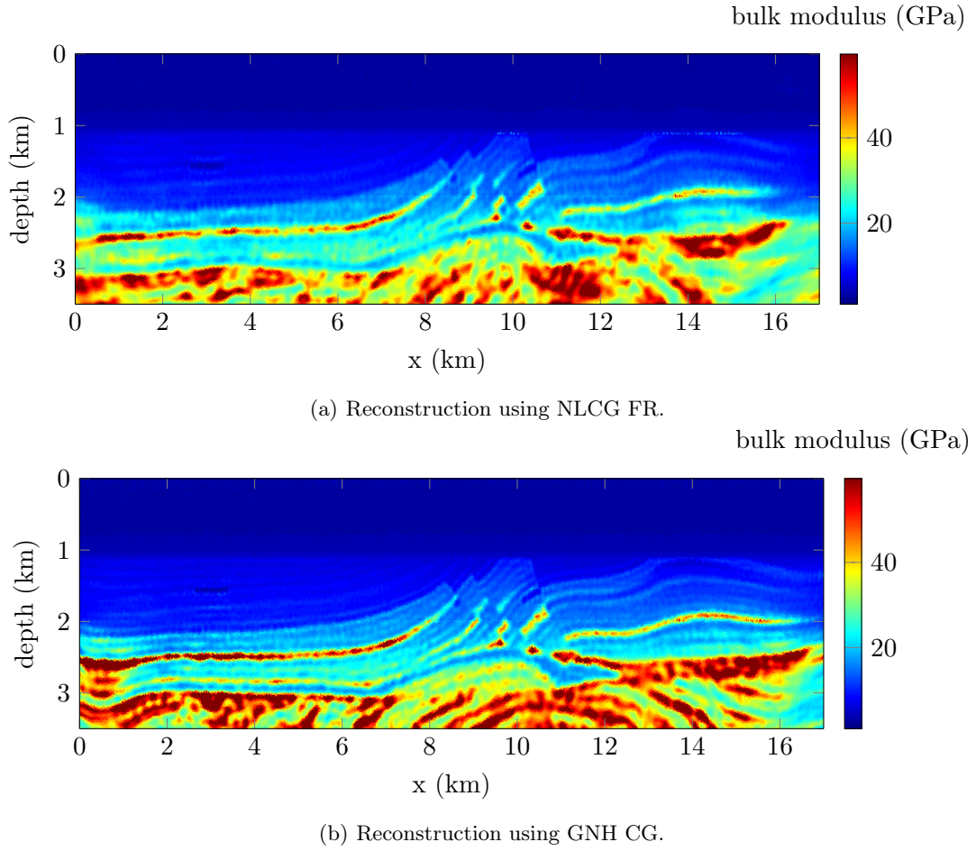
Figure 4.19: Final reconstruction of the acoustic Marmousi bulk modulus assuming variable density and using frequencies from 1 to 10 Hz. 25 iterations are performed per frequency (for a total of 250 iterations) and we compare the methods involving the gradient and the Gauss-Newton Hessian of the cost function.
