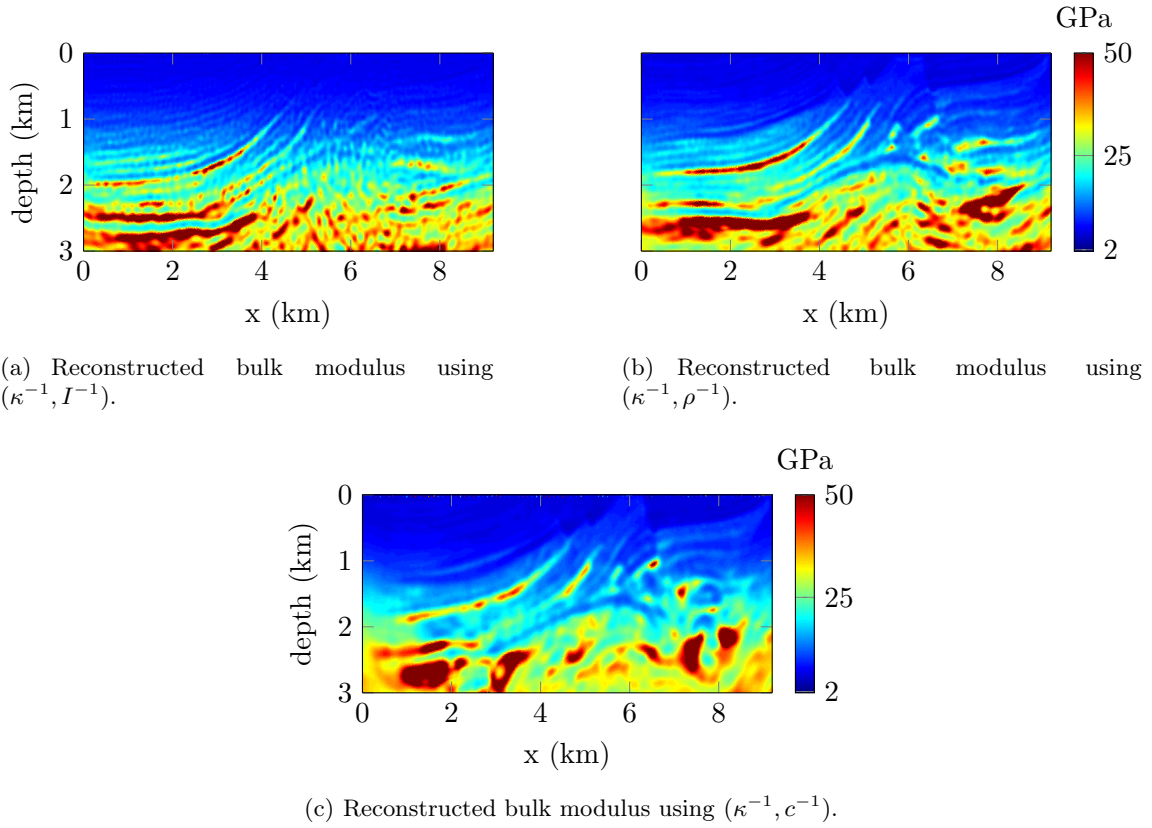
Figure 5.42: Final reconstruction after 10 Hz iterations of the Marmousi bulk modulus using different parametrizations.
