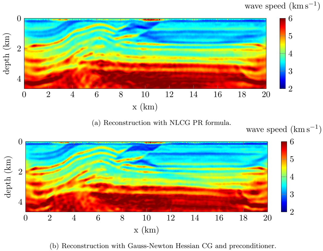
Figure 4.14: Final reconstruction of the acoustic OT wave speed assuming constant density and using frequencies from 1 to 10 Hz. 30 iterations are performed per frequency (for a total of 300 iterations) and we compare the methods involving the gradient and the Hessian of the cost function.
