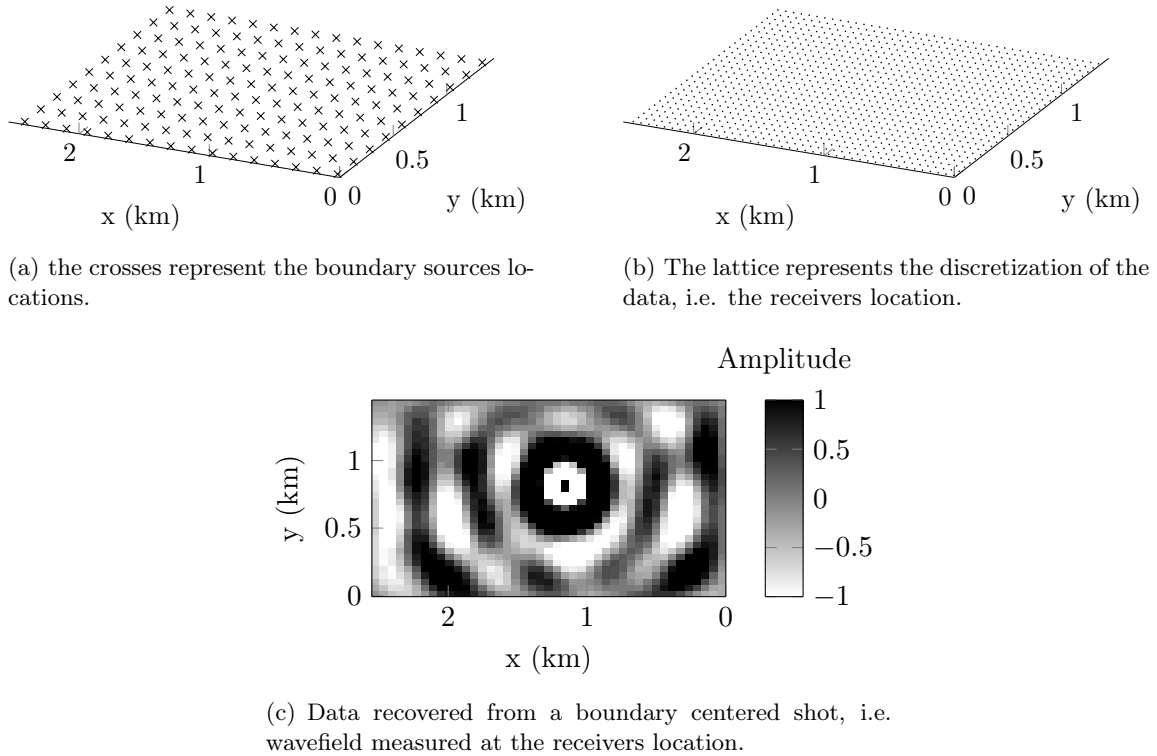
Figure A.6: Illustration of the seismic acquisition set.
