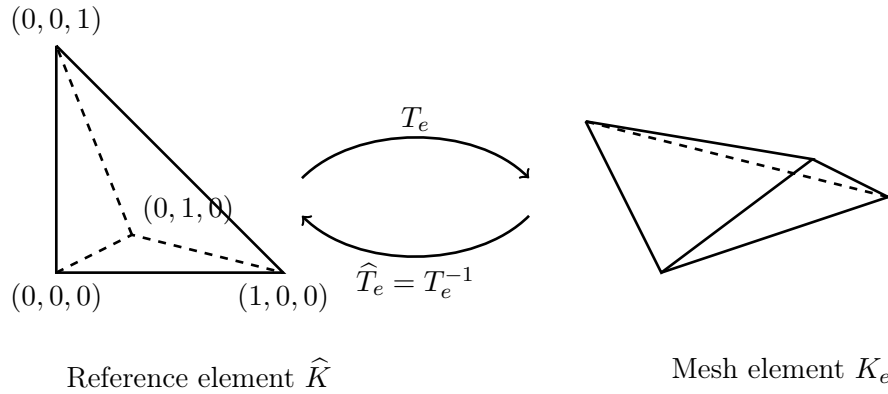
Figure 2.4: Illustration of the reference element. The tetrahedron K_e is mapped with the reference element \hat{K} with the transformation T_e .
