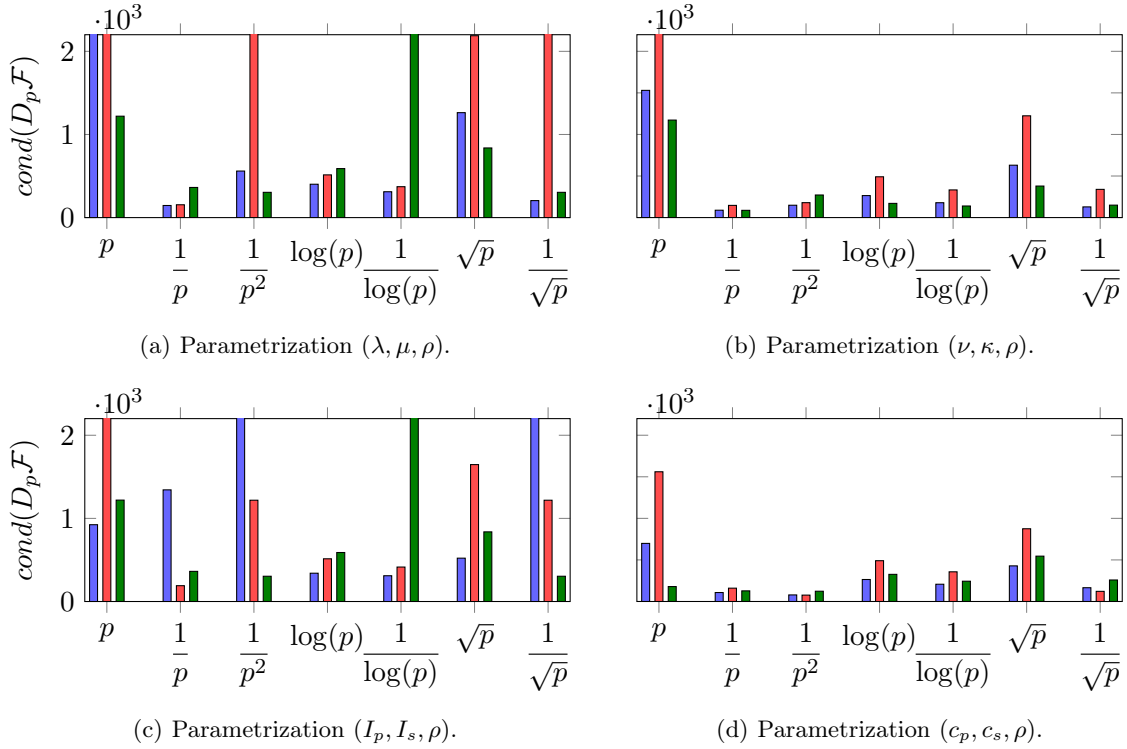
Figure 5.46: Comparison of the Fréchet derivative condition number for different parametrizations associated with the elastic Marmousi2 medium imposing the model partition N = 530 per parameter. The blue bars (■) represent the condition number of the Fréchet derivative of the first parameter of interest, the red bars of the second parameter and the green bars (■) of the last parameters. The parameters are indicated in the parenthesis.
