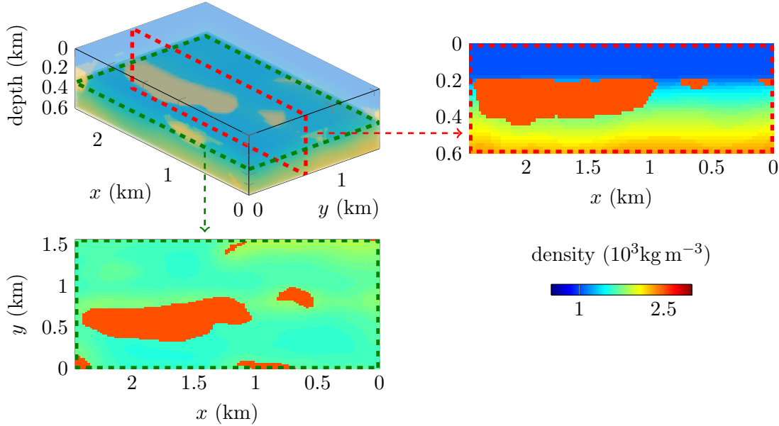
Figure 6.43: Density for the three-dimensional acoustic Louro medium of size 2.46 \times 1.56 \times 0.6 km. The density varies between 1000 and 2500 \text{ kg m}^{-3} . Vertical section at y = 680 \text{ m} is indicated with the red dashed frame and plotted in the right. The horizontal section at fixed depth z = 340 \text{ m} is indicated with the green frame and shown at the bottom.
