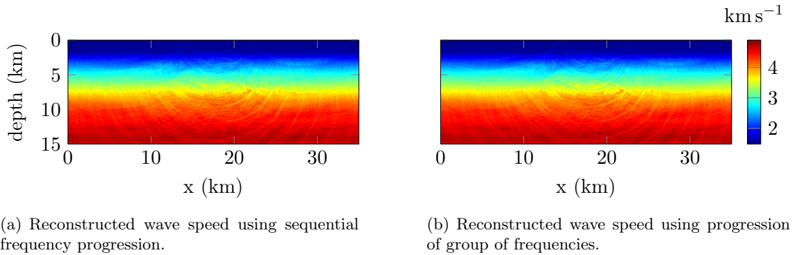
Figure 6.34: Reconstructions of the acoustic Seam wave speed using frequencies from 1 to 10 Hz. 20 iterations are performed per set of frequencies (for a total of 200 iterations).
