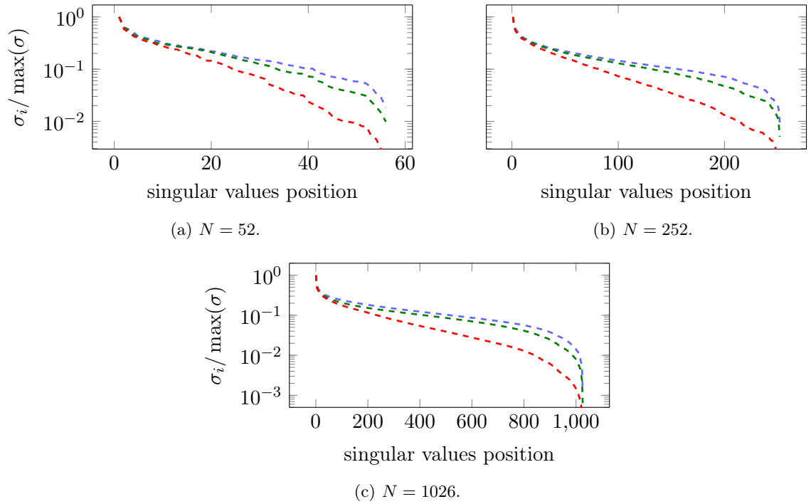
Figure 5.30: Evolution of the Fréchet derivative singular values for different partitioning. The blue dashed line (---) represents the slowness squared parametrization, the green dashed line (---) the slowness parametrization and the red dashed line (---) the velocity parametrization. This experiment uses the Marmousi velocity (of Figure 5.7(a)).
