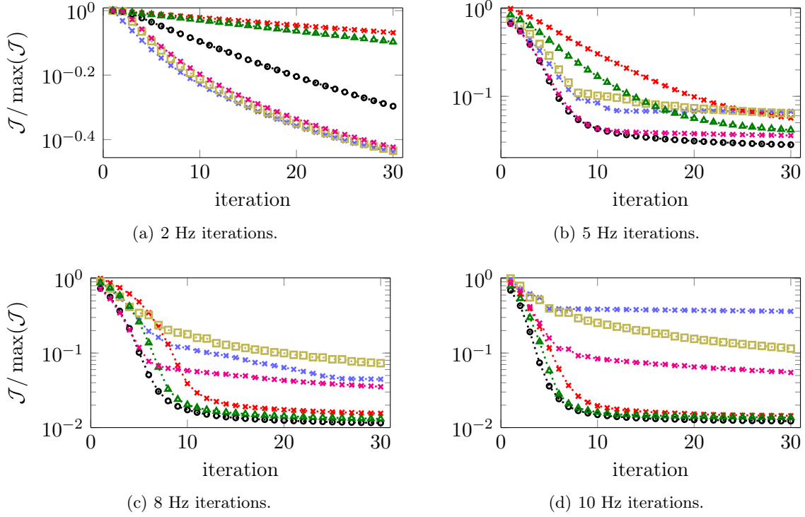
Figure 4.9: Evolution of the cost function for different frequencies using different methods. The blue crosses ( \cdots \times \cdots ) use the non-linear conjugate gradient Polak–Ribière formula. The red crosses ( \cdots \times \cdots ) use the Gauss-Newton Hessian and 10 conjugate gradient iterations. The yellow squares ( \cdots \square \cdots ) use a diagonal preconditioner with value \beta of Equation (4.42). The black circles ( \cdots \bullet \cdots ) use a diagonal preconditioner with value 10^{-3}\beta . The green triangles ( \cdots \blacktriangle \cdots ) use a diagonal preconditioner with value 10^{-4}\beta . The magenta crosses ( \cdots \times \cdots ) use a diagonal preconditioner with value 10^{-2}\beta . All methods using preconditioner use the Gauss-Newton Hessian and 10 conjugate gradient iterations.
