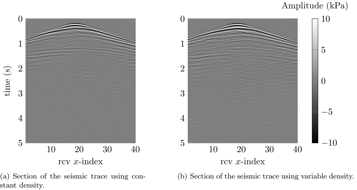
Figure 6.44: Comparison of two-dimensional sections of the trace for a centrally located source, it corresponds to a fixed line of receivers positioned at y = 855 m.
