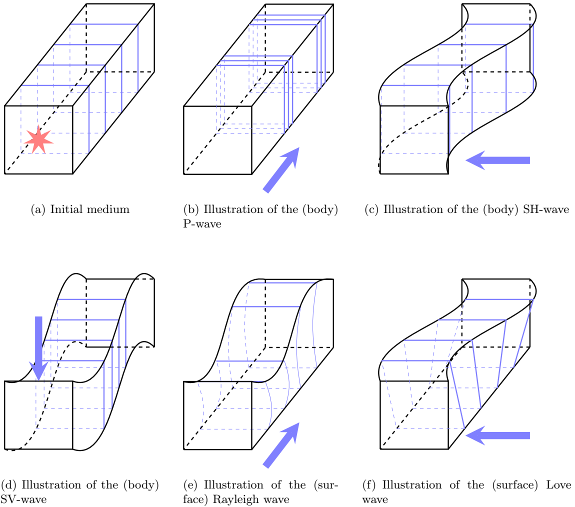
Figure 1.2: Illustration of the decomposition of a seismic wave into body (1.2(b), 1.2(c) and 1.2(d)) and surface (1.2(e) and 1.2(f)) waves. Figure 1.2(a) corresponds to the medium without perturbation, where the source is located at the center of the front face, marked with the red star. It is where the wave is generated from. The body wave is decomposed into the P- (1.2(b)), SH- (1.2(c)) and SV- (1.2(d)) waves. The P-wave component propagates along the longitudinal axis of the medium, normal to the front surface and introduces inner compression and dilatation of the medium as shown by the displacement of the blue sections. The S-wave corresponds to the part of the wave which is parallel to the surface and introduces the oscillations marked by the blue sections. Surface wave can further be decomposed into the Rayleigh (1.2(e)) and Love (1.2(f)) waves. The Rayleigh wave is along the longitudinal axis and the Love wave perpendicular. The blue arrows represents the direction of propagation of the wave components.
