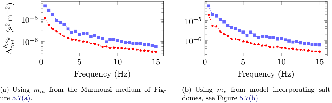
Figure 5.8: Evolution of the interval size verifying the deflection condition, quantity \Delta_{m_j}^{\delta_{m_k}} , with frequency where m_j is the Marmousi model or a model containing salt domes, see Figure 5.7. The blue squares ( \cdots \blacksquare \cdots ) employ one reflector ( \delta_{m_1} , Figure 5.5(a)) and the red stars ( \cdots \star \cdots ) one large reflector ( \delta_{m_3} , Figure 5.5(c)).
