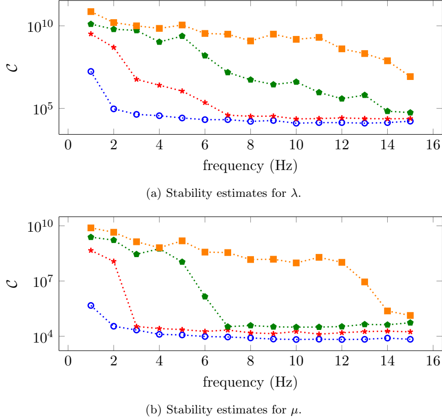
Figure 3.5: Evolution of the computational estimates of the stability constant depending on the frequency for elastic media. The models chosen for m_0 and m_1 are given Figure 3.4. We compare the evolution for the Lamé parameters \lambda and \mu . The blue circles ( \cdots\bullet\cdots ) employ the partition N = 530 . The red crosses ( \cdots\times\cdots ) employ the partition N = 2226 . The green pentagons ( \cdots\blacklozenge\cdots ) employ the partition N = 9116 . The orange squares ( \cdots\square\cdots ) employ the partition N = 36975 .
