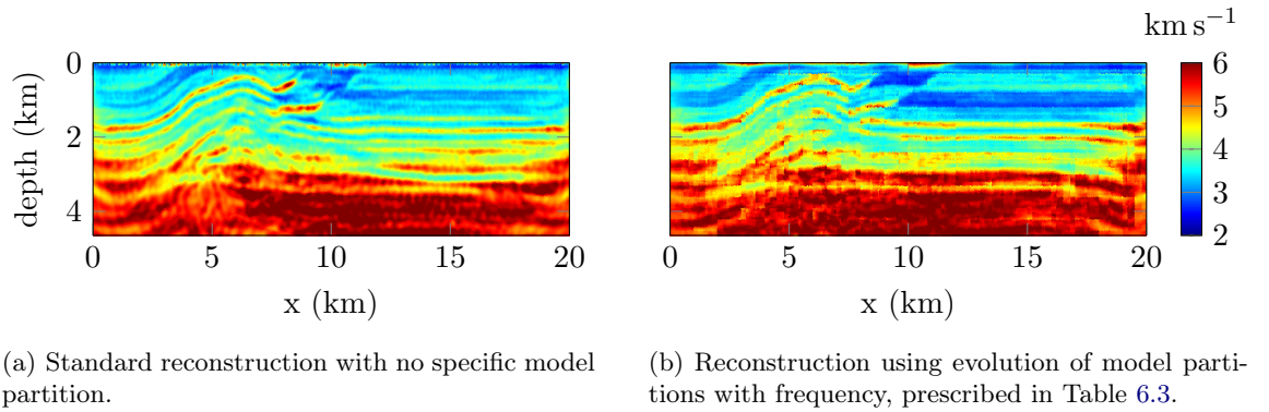
Figure 6.12: Reconstructions of the acoustic OT wave speed assuming constant density and using frequencies from 1 to 10 Hz. 20 iterations are performed per frequency (for a total of 200 iterations).
