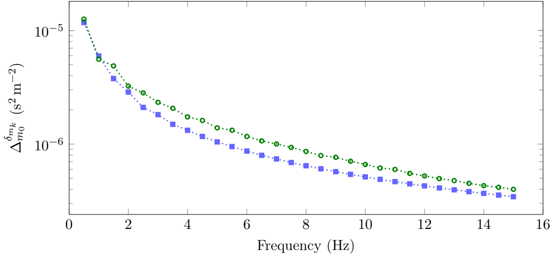
Figure 5.13: Evolution of the interval size verifying the deflection condition, quantity \Delta_{m_0}^{\delta_{m_k}} , with frequency using m_0 as smooth velocity background for direction \delta_{m_3} . The blue squares ( \cdots \blacksquare \cdots ) employ an acquisition of 19 sources and 183 receivers, which are only located at the top surface. the green circles ( \cdots \bullet \cdots ) employ 50 sources and 484 receivers, which are located all around the domain of interest.
