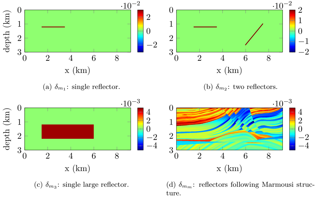
Figure 5.5: Four different directions for the estimation of the quantities of interest ( \hat{R}_{m_0}^{\delta_{m_k}} and \Delta_{m_0}^{\delta_{m_k}} ). The amplitude is determined so that \|\delta_{m_k}\| = 1 . The values of \delta_{m_k} are given in (\text{m s}^{-1})^{-2} = \text{s}^2 \text{m}^{-2} .
