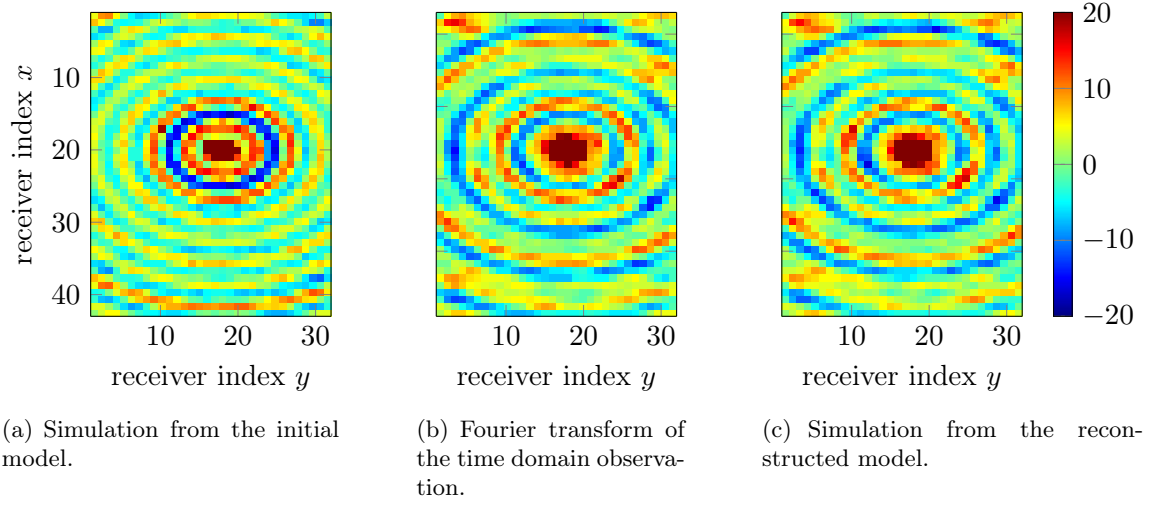
Figure 7.7: Comparison of the real part of the 10 Hz frequency vertical data for a centrally located source.
