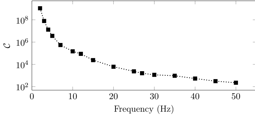
Figure 3.1: The black squares represent the computational estimates of the stability constant ( \cdots \blacksquare \cdots ) depending on the frequency at selected partition N = 4\,597\,248 . The model chosen for c_0 and c_1 are given Figures A.3 and A.2.
