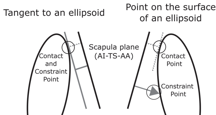
Figure 54 : Difference between constraint and contact points for the “tangent to an ellipsoid” and “contact point” kinematic constraints
