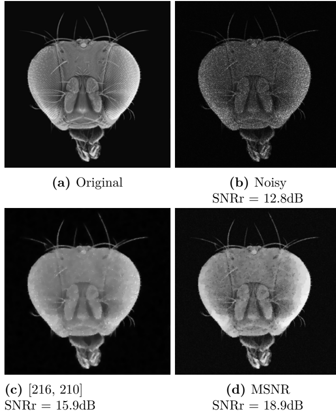
Figure 6.5 – Denoising experiment for image formation model \mathbf{u}_0 = \mathbf{u} \oslash \boldsymbol{\eta} , where \boldsymbol{\eta} is a gamma distributed white noise with \boldsymbol{\eta}[1] \sim \text{Gamma}(20, 20) . The SNRr for MSNR is stable after 50 iterations. Computing time MATLAB - CPU: 0.15s.
