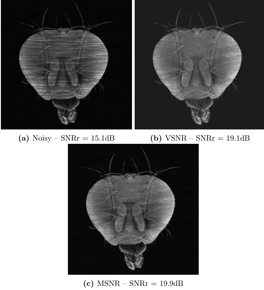
Figure 6.6 – Denoising simulation with structured noise. The image is corrupted with \psi a segment and a = 1.1 see Figure 6.3 bottom-left. The SNRr is stable after 50 iterations. Computing time GPU: 0.03s.
