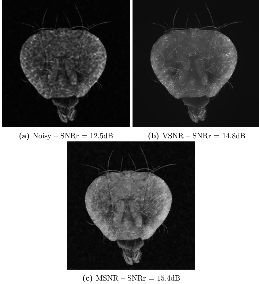
Figure 6.7 – Denoising simulation with structured noise. The image is corrupted with \psi the indicator function 4 \times 4 square and a = 1.1 see Figure 6.3 bottom-right. The SNRr is stable after 40 iterations. Computing time GPU: 0.025s.
