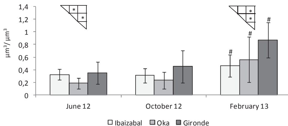
Figure 5: Mean values ( \pm standard deviations) of annual CTD values for oysters at three sampling points. Statistically significant differences ( p < 0.05 ) between sampling points from the same month are expressed in (*) while differences between same sampling points at different months are expressed in (#).
