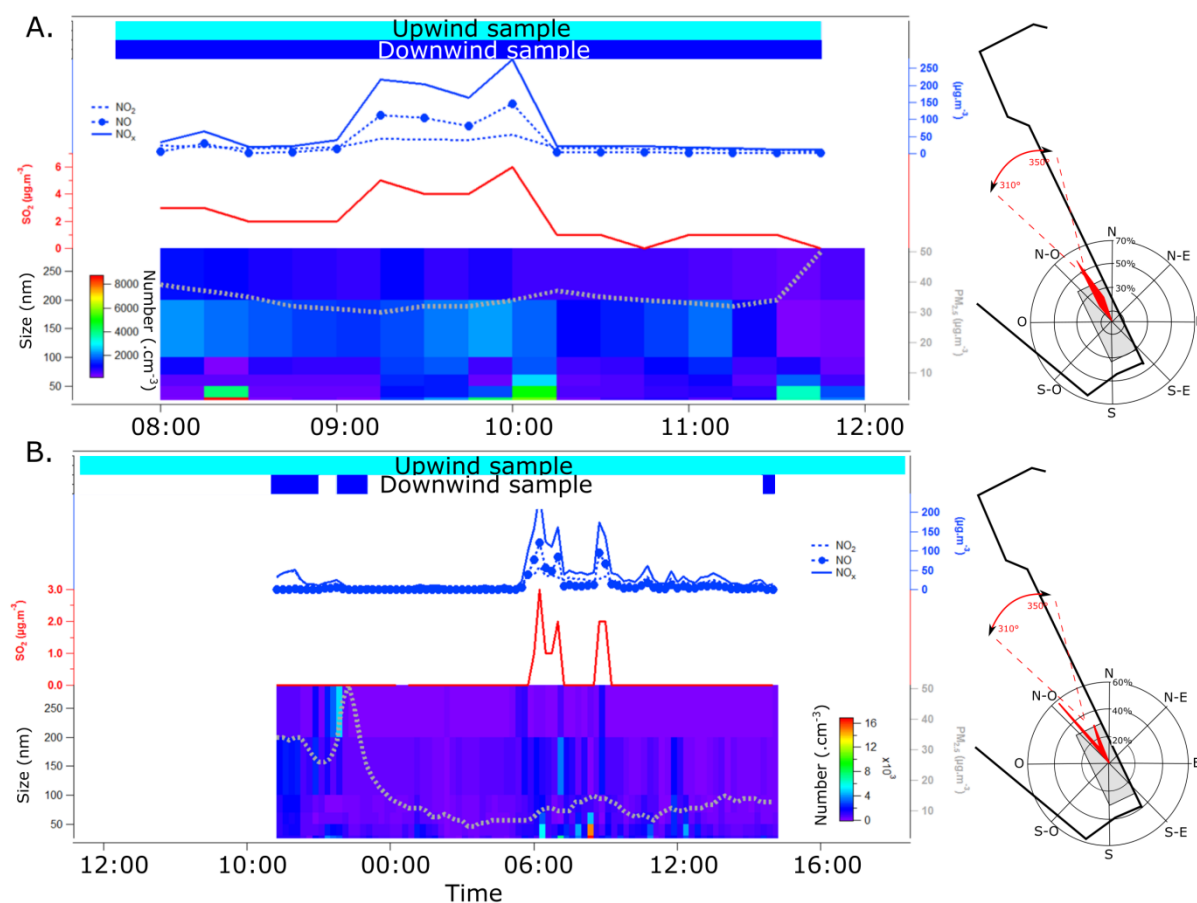
Figure A.1: A. Example of pair of samples selected and analyzed: Downwind and upwind samples were collected simultaneously. Peaks of concentration going up to 250\mu\text{g}\cdot\text{m}^{-3} for NO x , 150\mu\text{g}\cdot\text{m}^{-3} for NO, 50\mu\text{g}\cdot\text{m}^{-3} for NO 2 and 7\mu\text{g}\cdot\text{m}^{-3} for SO 2 were observed on the downwind site when samples were collected. A high and constant PM 2.5 concentration (between 30 and 50\mu\text{g}\cdot\text{m}^{-3} ) was observed with some episode with fine particle (20-50nm, going up to 8000\text{particles}\cdot\text{cm}^{-3} ). These couple of sample was selected. B. Example of pair of samples not selected for further analysis.
