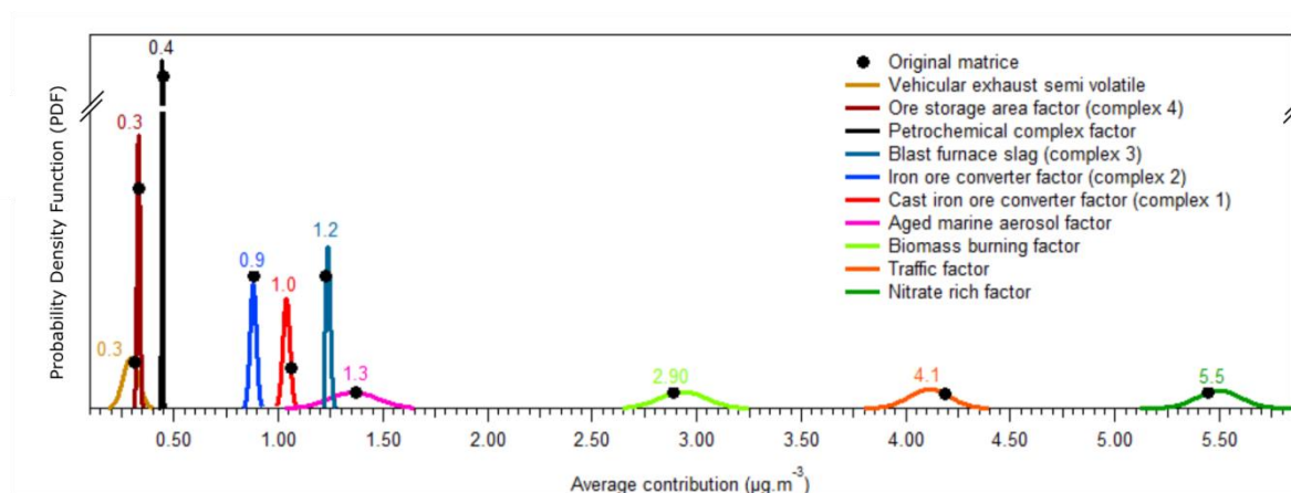
Figure 3: Probability Density Function (PDF) of the average factor contribution obtained for 30 different matrix of concentrations. The ambient data matrix modifications consist of random changes of the concentrations of all the variables (elements, organic makers and major fractions) for all the samples within their analytical uncertainty ranges.
