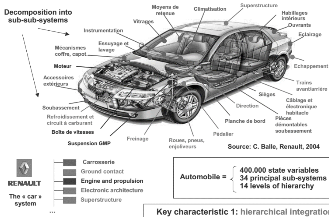
Figure 2-1 Vehicle decomposition
