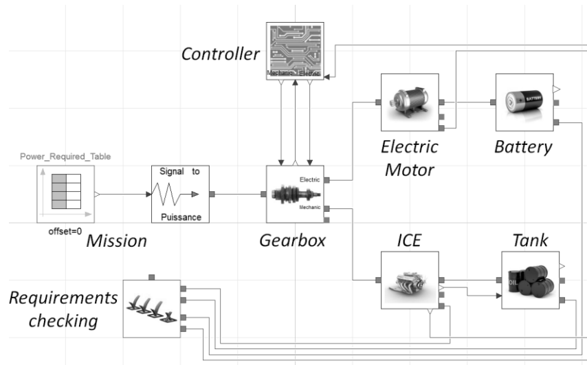
Fig. 4-14. Global model including electric motor and battery blank models
