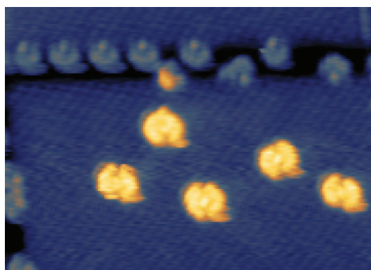
Figure B.4. – Fe-phen molecules on a CuN-rich surface. The Fe-phen molecules are either adsorbed on plain CuN surfaces or on trenches' edges. Image size is 14.3\text{ nm} \times 11.8\text{ nm} ( V=0.5\text{ V}, I=50\text{ pA} ).
