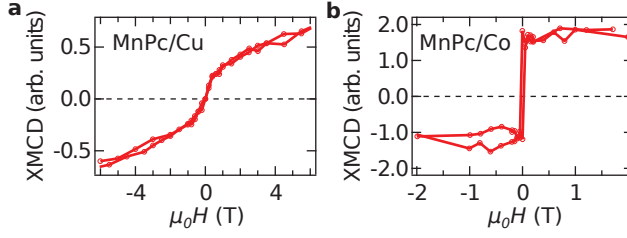
Figure 8.8. – Magnetic hysteresis loop of the central Mn ion of MnPc molecules on Cu(100) and Co/Cu(100). Evolution of the XMCD intensity of the Mn L_3 edge (photon energy: 640 eV) as a function of the external magnetic field for MnPc molecules on a , Cu(100) and b , Co/Cu(100) substrates. The hysteresis loop of a and b were acquired at a temperature of 8 K and 300 K on a MnPc coverage of 2.5 ML and 1 ML, respectively.
