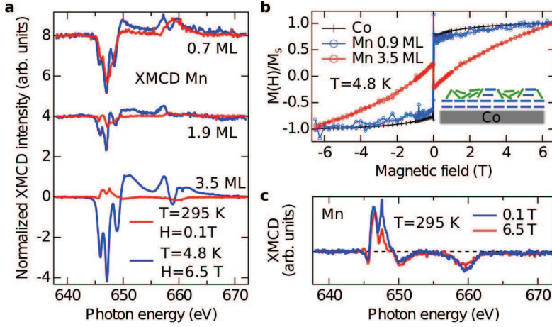
Figure 9.5. – AF ordering of MnPc molecules onto Co. a , XMCD at Mn L_{3,2} edges for MnPc coverages of 0.7 ML, 1.9 ML and 3.5 ML; and normalized by the quantity of probed MnPc, i.e. by its white line integral. For every coverage a pair of XMCD is represented, one at 295 K in a magnetic field of 0.1 T to probe the robustness of the magnetization and one at 4.8 K in a field of 6.5 T to align the uncoupled paramagnetic moments. b , Normalized magnetization of Co and Mn as a function of the external magnetic field at 4.8 K. The magnetization is deduced from the XMCD intensity at 786.8 eV and 647.0 eV for Co and Mn, respectively. The inset schematizes the stacking of 3.5 ML MnPc on Co where only a few proportion of third- and fourth-ML molecules are forming molecular columns with the underlying molecules. c , XMCD of MnPc at a molecular coverage of 3.5 ML at RT for two different magnetic fields demonstrating the robustness of the effect.
