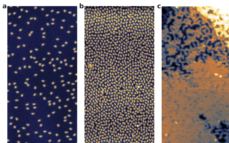
Figure 13.6. – Layer-by-layer growth of Fe-phen on Cu(111). Large-scale STM topography of Fe-phen molecules on Cu(111) at different coverages: a , 0.1 ML ( V=0.3 V, I=30 pA), b , 0.6 ML ( V=1.0 V, I=50 pA) and c , approximately 1.8 ML ( V=0.85 V, I=230 pA). The topographies indicate a layer-by-layer and contamination-free growth of Fe-phen on Cu(111). Image sizes are 55 nm \times 110 nm.
