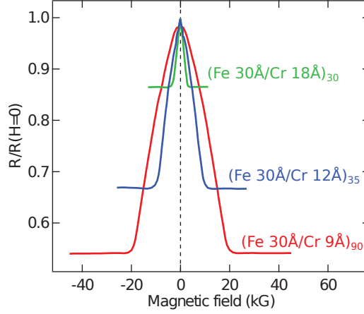
Figure 7.1. – Giant magnetoresistance in Fe/Cr superlattices. Variation of the normalized resistance as a function of the external in-plane magnetic field for three different superlattices at 4.2 K. The data are taken from Ref. 143.
