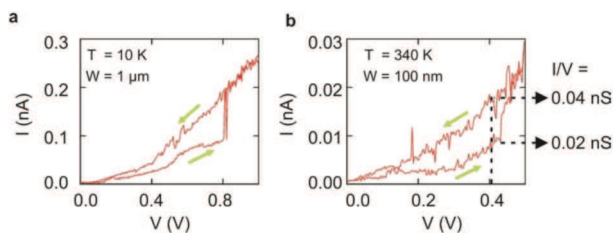
Figure 12.13. – I-V characteristics on a single nanoparticle. a , Current-voltage curve acquired at low temperature ( T = 10 K) on Fe-based SCO nanoparticles bridged between two 1\text{ }\mu\text{m} -width gold electrodes. b , Same measurements performed at T = 340 K on a single nanoparticle sandwiched between two 100\text{ nm} -width gold electrodes. In both panels, we observe a conductance jump ascribed by the authors to a transition from the LS to the HS state when increasing the voltage. The figure is taken from Ref. 341.
