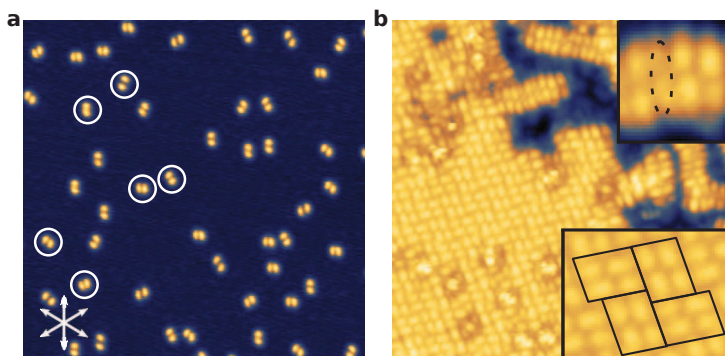
Figure 13.7. – Adsorption geometry of first- and second-ML Fe-phen on Cu(111). Topographies of a a , 0.1 ML sample revealing 6 different orientations of the molecules (molecules in the 6 different orientations are encircled in white), b , 1.8 ML showing ordered densely-packed areas (lower inset) in contrast to chain-like structures of the molecules in less dense-areas (upper inset). For clarity, a single molecule is encircled in the upper inset, and pairs of molecules are surrounded by a parallelogram in the lower inset. Image sizes are a , 45 nm \times 45 nm ( V=0.15 V, I=150 pA), b , 18 nm \times 18 nm ( V=0.6 V, I=200 pA), (upper inset) 2.0 nm \times 2.1 nm, (lower inset) 3.9 nm \times 3.1 nm.
