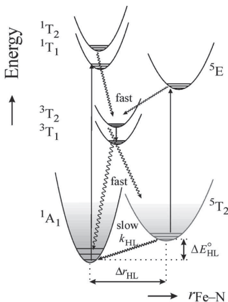
Figure 12.7. – Scheme of the electronic states of a \text{Fe}^{2+} ion of a SCO complex. The ^1A_1 ( ^5T_2 ) state corresponds to the LS (HS) state. The figure is taken from Ref. 257.
