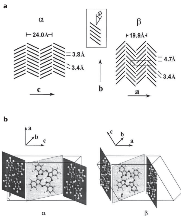
Figure 8.2. — \alpha and \beta phases of \text{H}_2\text{Pc} . a , Schematic of the staking of \text{H}_2\text{Pc} molecules along the b axis in the \alpha (left) and \beta (right) phases. The stacking angles defined as the angle between the normal of the molecular plane and the b axis (see inset) are 26^\circ and 45^\circ for the \alpha and \beta phases, respectively. b , Schematic of molecular arrangement within the unit cell for \alpha - (left) and \beta -phase (right) \text{H}_2\text{Pc} . For clarity, only half of the \alpha -phase unit cell is represented. The figure is taken from Ref. 195.
