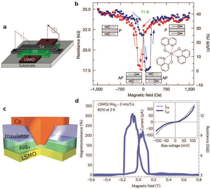
Figure 7.4. – Magnetoresistance in Alq 3 -based organic spin valves.
