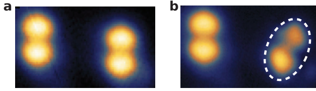
Figure 14.7. – Lateral tip manipulation on a LS Fe-phen molecule on Cu(100). Topographies a before and b after a tip induced lateral manipulation of a LS Fe-phen molecule. For clarity, the manipulated molecule is encircled in b . Image sizes are 4.8 \text{ nm} \times 2.8 \text{ nm} .
