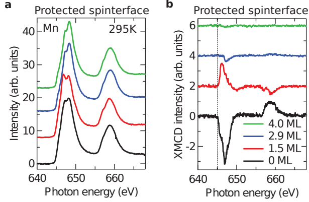
Figure 10.3. – XAS and XMCD at the Mn L_{3,2} edges of MnPc on \text{Cu}(d_{\text{Cu}})/\text{Co}(100) for different Cu thicknesses. a , White line spectra at the Mn L_{3,2} edges of MnPc on \text{Cu}(d_{\text{Cu}})/\text{Co}(100) for d_{\text{Cu}} = 0 ML, 1.5 ML, 2.9 ML and 4.0 ML. b , XMCD spectra at the Mn L_{3,2} edges of MnPc on \text{Cu}(d_{\text{Cu}})/\text{Co}(100) for the Cu thicknesses enumerated in a . The spectra were acquired at 295 K in 0.1 T, and are vertically shifted for clarity.
