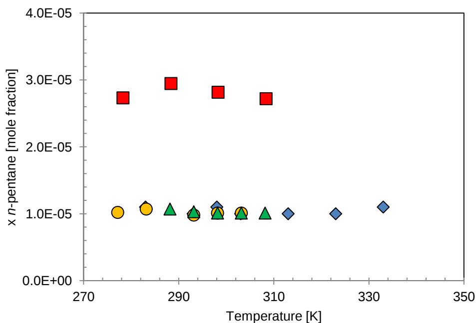
Figure 2.1: n -Pentane solubility in water at atmospheric pressure. Comparison of data from the literature ( \diamond ) [2.3], ( \blacktriangle ) [2.4], ( \bullet ) [2.5] and ( \blacksquare ) [2.6].
