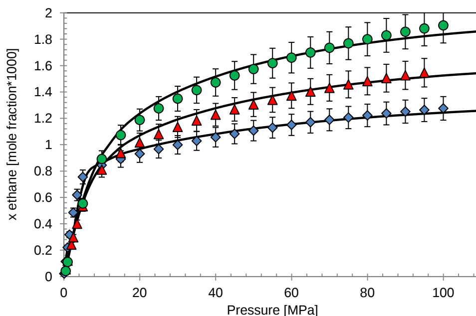
Figure 5.1: Ethane solubility in water at 313.15 K (♦), 373.15 K (▲) and 393.15 K (●) [5.6]. (–) GC-PR-CPA model. Error bar: \pm 7\%
