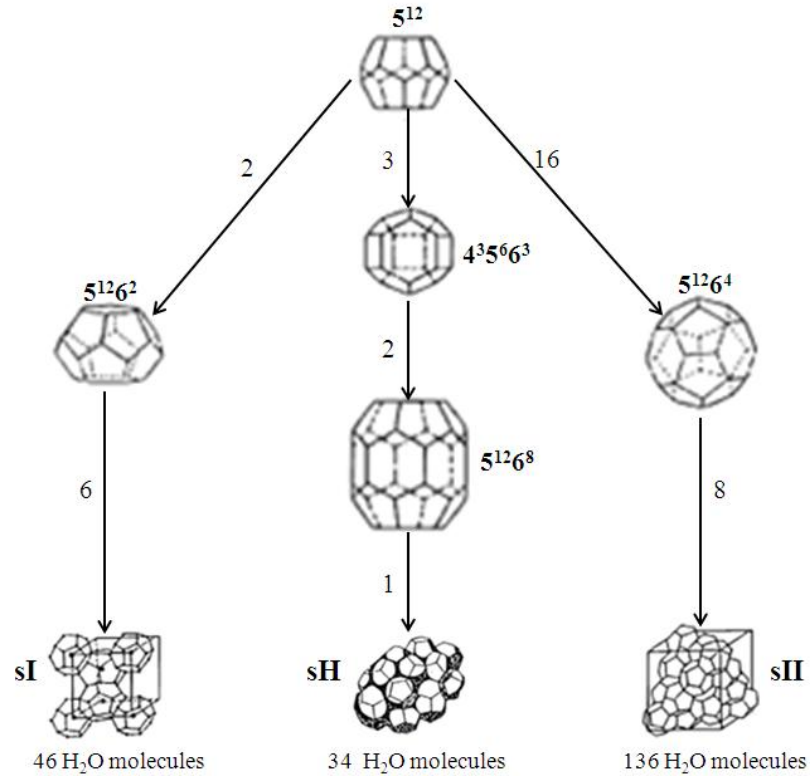
Figure 1.16: Hydrates structures [1.40]
