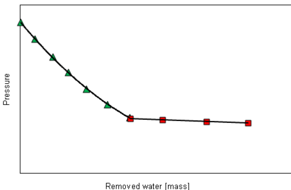
Figure 2.6: Pressure – mass diagram to determine the bubble point at constant temperature. ▲ above the bubble point. ■ bubble line.
