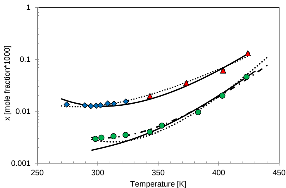
Figure 5.6: Cyclohexane (♦) [5.12] and (▲) [5.13], and Methylcyclohexane (●) [5.14] solubilities in water at atmospheric pressure. (–) GC-PR-CPA model. (.....) Tsionopoulos correlation. (– · –) Readjusted Tsionopoulos correlation. Error bar: \pm 5\%
