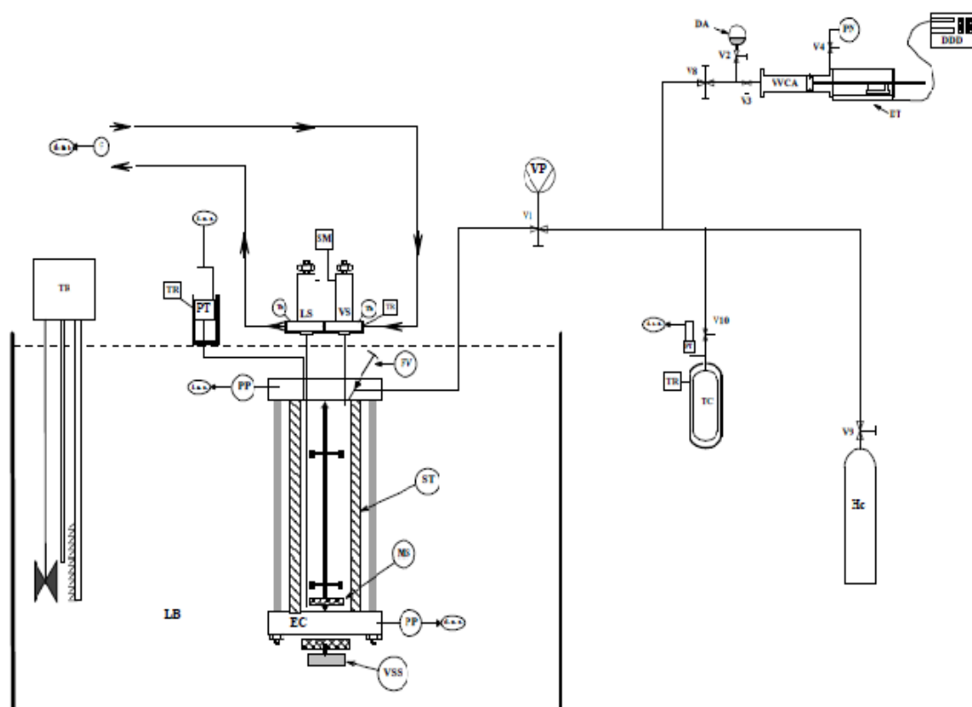
Figure 2.3: Flow diagram of the equipment used for VLE measurements. EC: equilibrium cell; PT: pressure transducer; LB: liquid bath; PP: platinum probe; SD: stirring device; TR: temperature regulator; VP: vacuum pump.
