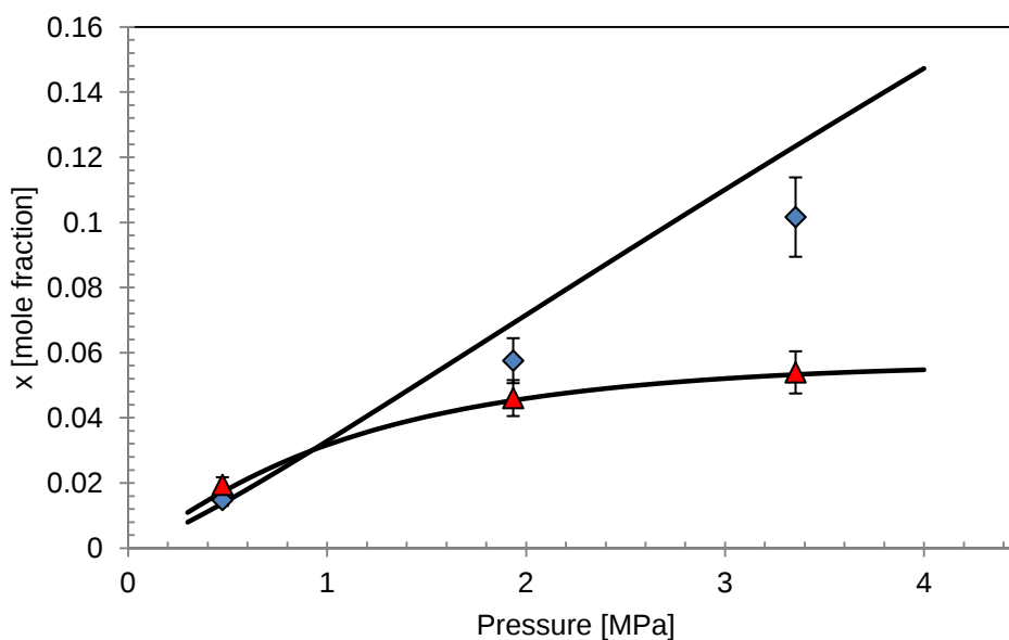
Figure 5.21: Compositions of methane (♦) and ethane (▲) in organic phase of MIX 10 at 298.1 K. (–) GC-PR-CPA model. Error bar from [5.37]: \pm 12\%
