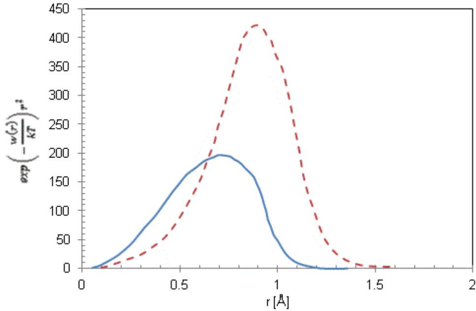
Figure 3.2: Boltzmann probability factor versus r . — N_2 hydrate. - - C_2H_6 hydrate. [3.12]
