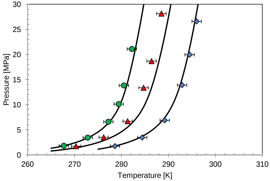
Figure 5.27: Hydrate dissociation points of MIX 5 with deionised water (♦), 25% wt ethanol (▲) and 25% wt methanol (●). (–) GC-PR-CPA model. Error bar: \pm 0.5 K.
