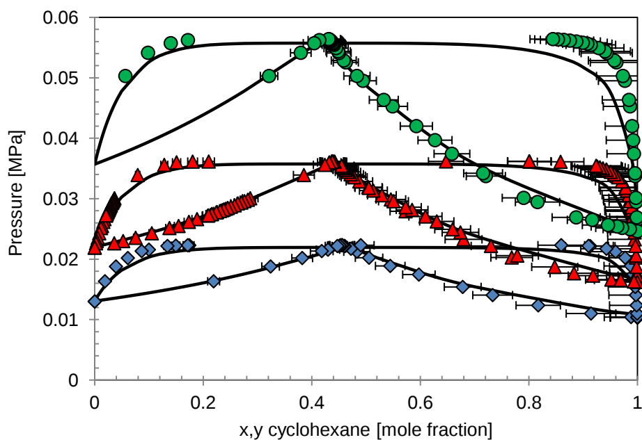
Figure 5.16: Phase equilibria of the binary system cyclohexane – methanol at 293.15 K ( \blacklozenge ), 303.15 K ( \blacktriangle ) [5.26] and 313.15 K ( \bullet ) [5.27]. (–) GC-PR-CPA model. Error bar: \pm 5\%
