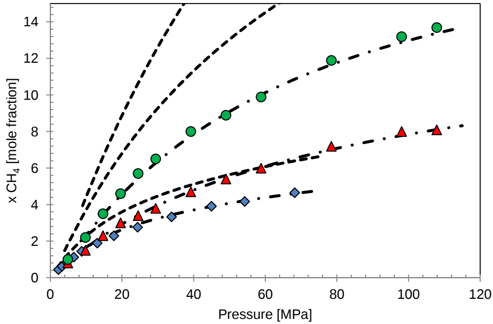
Figure 4.1: \text{CH}_4 solubility in water at 310.93 K ( \blacklozenge ) [4.4], 423.15 K ( \blacktriangle ) and 473.15 K ( \bullet ) [4.5]. — — SRK-CPA EoS with k_{ij}=0 . — · SRK-CPA EoS with adjusted k_{ij} .
