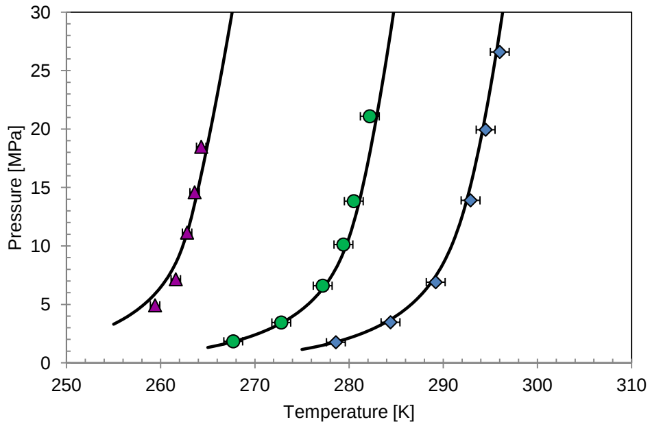
Figure 5.28: Hydrate dissociation points of MIX 5 with deionised water (♦), 25% wt methanol (●) and 50% wt methanol (▲). (–) GC-PR-CPA model. Error bar: \pm 0.5 K.
