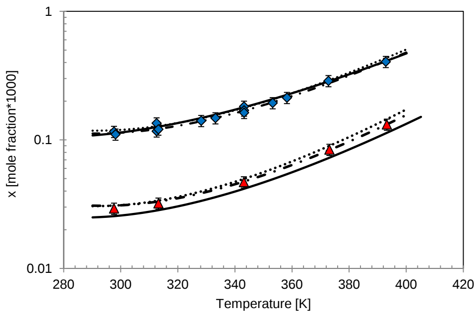
Figure 5.8: Toluene (♦) and Ethylbenzene (▲) solubilities in water at 0.5 MPa [5.17]. (-) GC-PR-CPA model. (.....) Tsonopoulos correlation. (- . .) Readjusted Tsonopoulos correlation. Error bar: \pm 10\%
