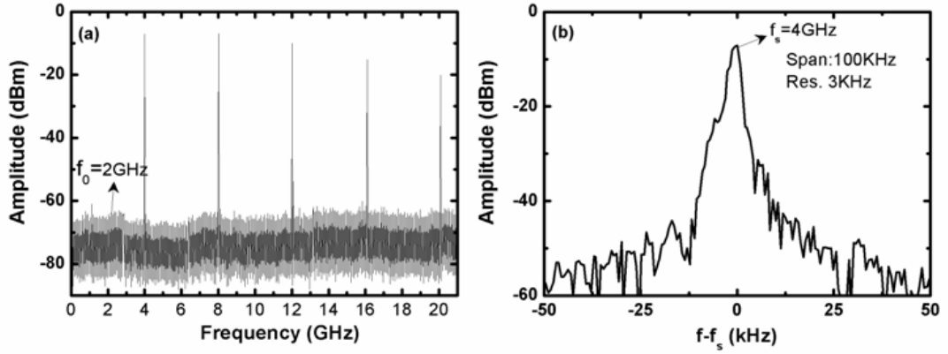
Figure 4.11 Second harmonic mode-locking results. (a) RF spectrum of the mode-locked pulse obtained for ACR54-A SESAM on a 21 GHz span. (b) Fundamental component of RF spectrum, taken at a 100 kHz span and 3 kHz resolution bandwidth
