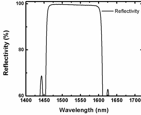
Figure 3.5 Measured reflectivity curves of an anti-reonant SESAM with a 35-pair AlAs/GaAs DBR
