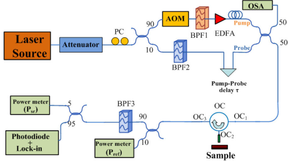
Figure 3.12 Schematic overview of the nonlinear reflectivity measurement setup. PC: Polarization Controller; AOM: Acousto-Optic Modulator; BPF: Band Pass Filter; EDFA: Erbium Doped Fiber Amplifier; OSA: Optical Spectrum Analyzer; OC: Optical Circulator.
