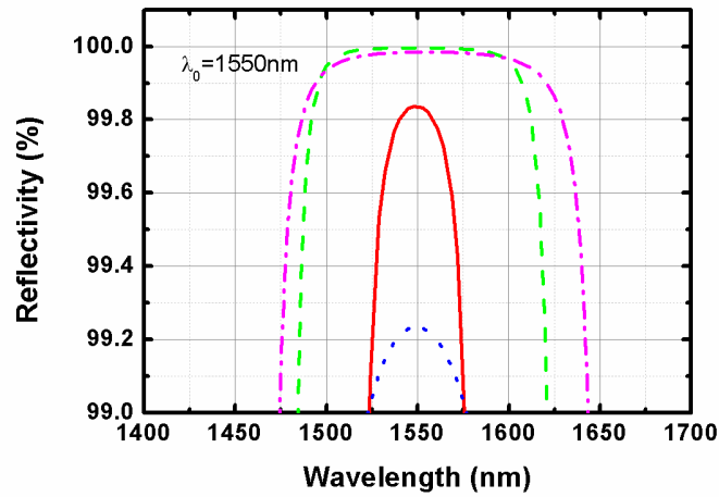
Figure 2.6 Calculated reflectivity of various DBR mirrors at 1550 nm. 48-pair InP/InGaAsP DBR mirror on InP substrate (red solid), 35-pair AlAs/GaAs DBR mirror on GaAs substrate (magnetic dash dot), 17-pair AlAs/GaAs DBR mirror on GaAs substrate (blue dot) and hybrid mirror consisting of 17-pair AlAs/GaAs DBR plus a gold mirror (green dash).
