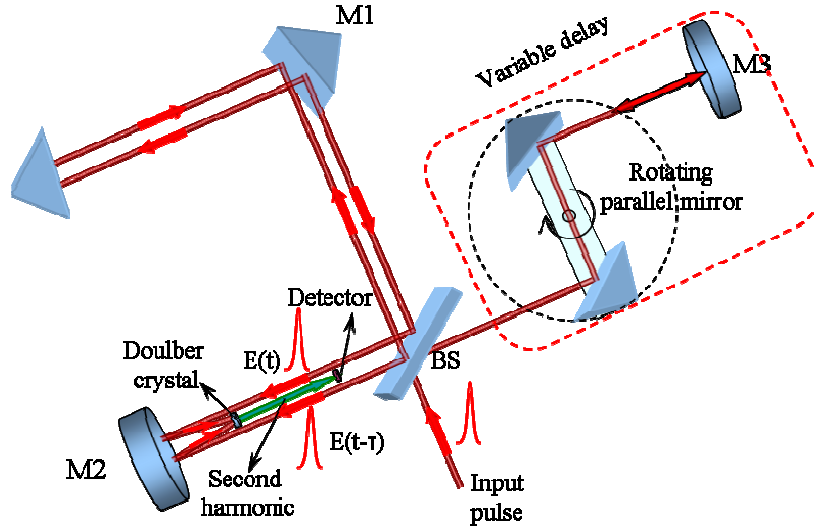
Figure 4.3 Second-harmonic generation geometry for measurement of the intensity autocorrelation function
