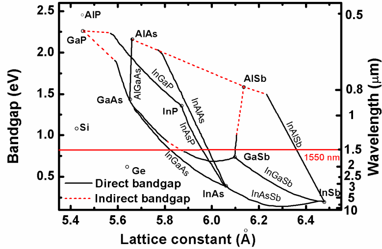
Figure 1.2 Bandgap energy as a function of lattice constant for different III-V semiconductor alloys at room temperature. The solid lines indicate a direct bandgap, whereas the dashed lines indicate an indirect bandgap (Si and Ge are also added to the figure).
