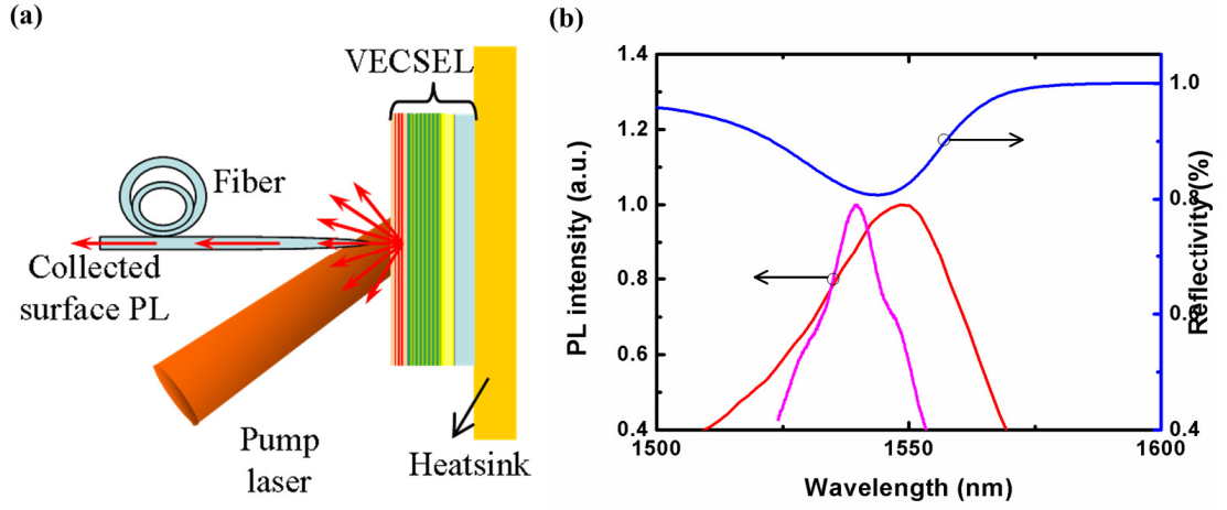
Fig 2.20 (a) Simplified experimental setup for collecting the surface PL signal from the VECSEL chip excited by a 980 nm pump laser. (b) Normalized QW PL (red line) and surface PL of VECSEL chip (magenta line) at room temperature. The cavity mode (reflectivity spectrum, blue line) indicates the strong cavity effect of VECSEL chip.
