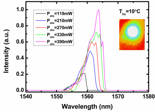
Figure 2.32 Laser spectra of VECSEL with electroplated copper substrate at various absorbed pump power for heatsink temperature of 10 °C. The inset shows the intensity profile of the output beam at an absorbed pump power of 390 mW.
