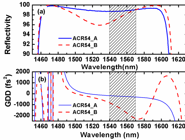
Figure 3.21 (a): Experimental reflectivity of ACR54-A SESAM (blue curve) and ACR54-B SESAM (red dash). (b): Corresponding calculated GDD value of the two SESAMs.
