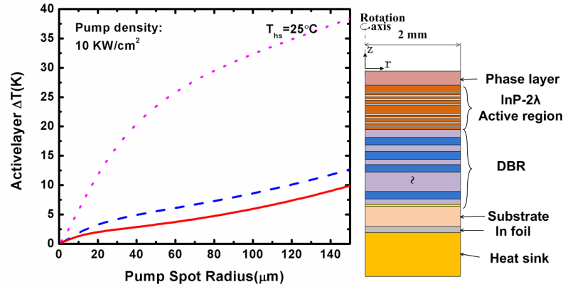
Figure 2.13: Temperature rise in the active region calculated versus pump spot radius for different DBR mirrors with 300- \mu\text{m} thick CVD diamond substrates: 17-pair GaAs/AlGaAs –Au hybrid mirror (red solid), 35-pair GaAs/AlGaAs DBR mirror (blue dash), 48-pair InP/InGaAsP DBR mirror (magenta dot).
