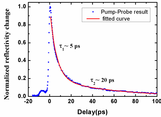
Figure 3.14 Normalized instantaneous reflectivity of a SESAM as function of the time delay between the pump and the probe pulse. The measurement is shown as blue dots, the solid red line is a fitting curve.
