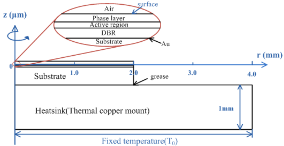
Figure 2.11. Simplified geometry for Multilayer VECSEL structure
