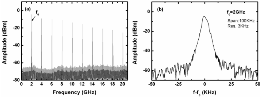
Figure 4.8 (a) RF spectrum of the mode-locked pulse obtained for ACR54-A SESAM on a 21 GHz span. (b) Fundamental component of RF spectrum, taken at a 100 kHz span and 3 kHz resolution bandwidth
