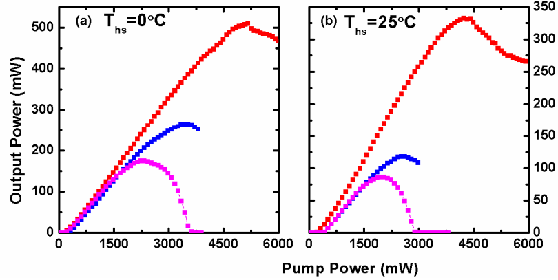
Figure 2.26 Continuous-wave emitted power of VECSELs with different host substrates. CVD diamond (red square), electroplated copper (blue square) and electroplated gold (magenta square) versus incident pump power at different temperatures. (a) Heatsink temperature is fixed at 0^\circ\text{C} . (b) Heatsink temperature is fixed at 25^\circ\text{C} .
