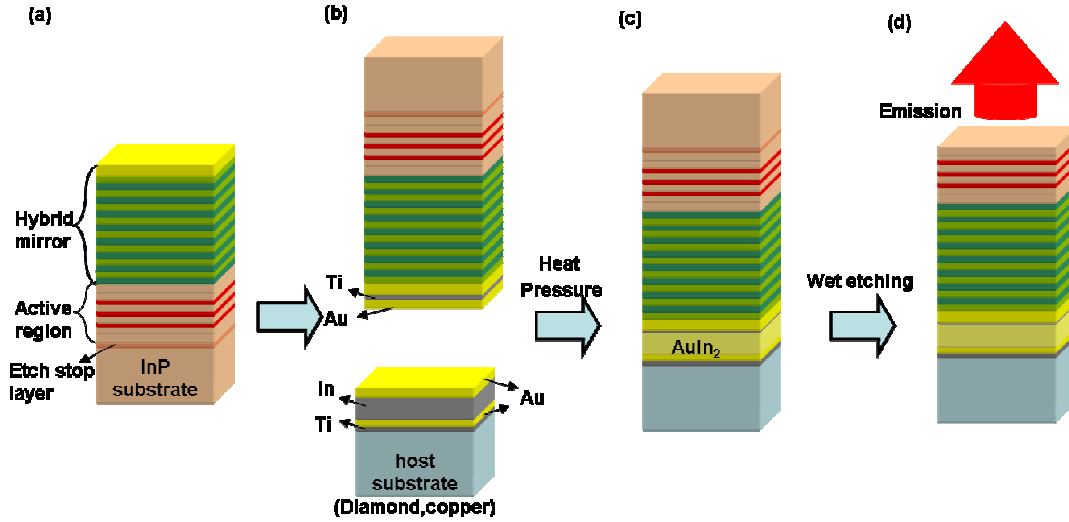
Fig 2.17 Description of the eutectic \text{AuIn}_2 bonding process of the VECSEL structure onto a host substrate
