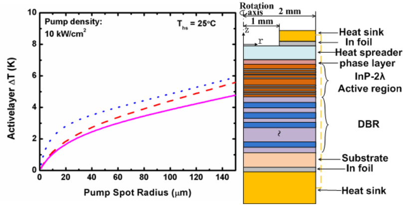
Figure 2.12: Temperature rise in active layer calculated versus pump spot radius for a 300\text{-}\mu\text{m} thick diamond heat spreader and with different DBRs and substrates: 35-pair GaAs/AlGaAs DBR mirror on GaAs substrate (red dash), and 48-pair InP/InGaAsP DBR mirror on InP substrate (blue dot). The limit case of the active region directly bonded onto the same heat spreader is a reference (magenta line).
