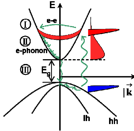
Figure 3.2 Schematic representation of the carrier dynamics in a bulk semiconductor material [7]. Three time scales can be distinguished. I. Coherent carrier dynamics, which at room temperature may last \sim few tens of femtoseconds depending on excitation density. II. Thermalization between the carriers due to carrier-carrier scattering and cooling to the lattice temperature by e-Phonon emission. III. Carrier-trapping or recombination.
