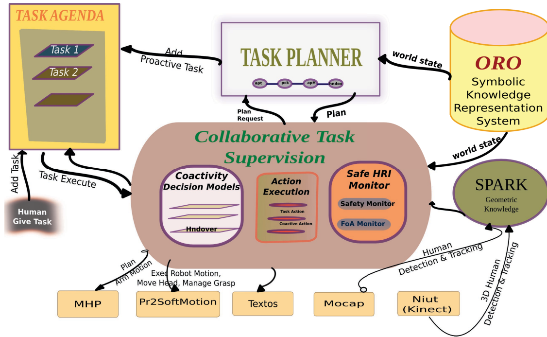
Figure 6.2: System Architecture
