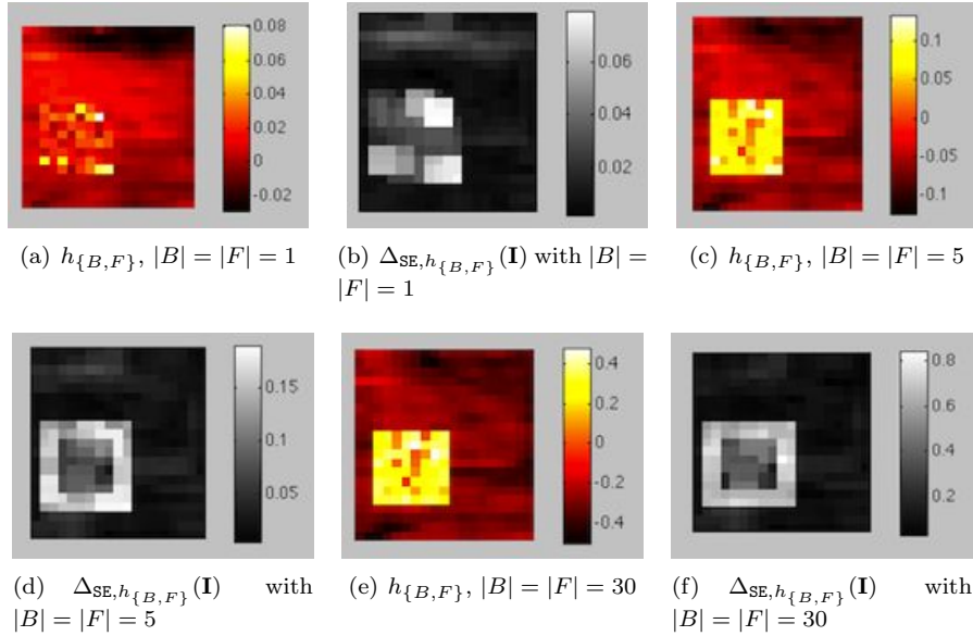
Figure 4.9: Comparison of h function, ordering and morphological gradient using different size of training set in the Toy example of Fig. 4.8. The experiment shows as the gradient is higher when the training size increases. We remark that the scale gradient in (f) is larger than (d) and (b).
