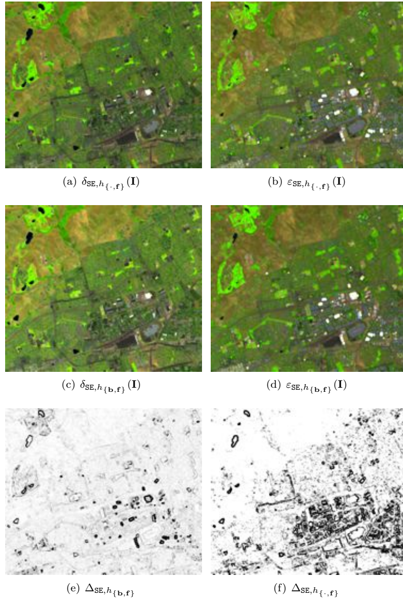
Figure 4.16: Comparison of different supervised morphological operators for h_{\{\cdot, f\}} and h_{\{b, f\}} . Spectra are shown using bands \{115, 70, 30\} . Both h -orderings are calculated using (4.9) with a polynomial kernel of degree two.
