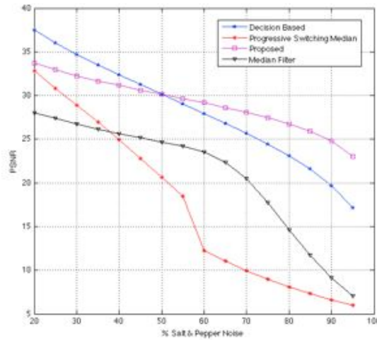
(a) Lena Grey
