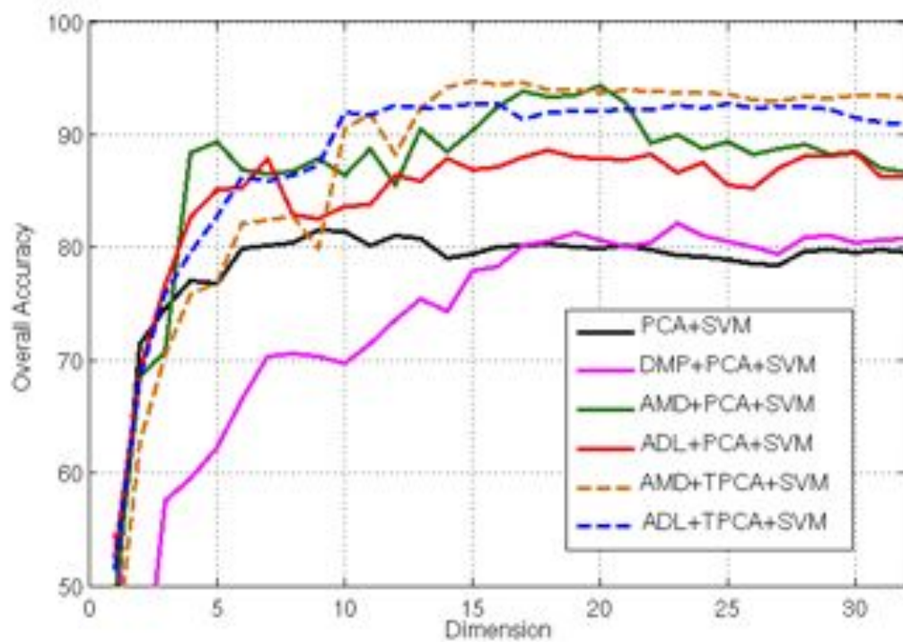
Figure 7.11: Behaviour of the overall accuracy in the Pavia University dataset for different morphological decompositions and dimensional reduction approach.
