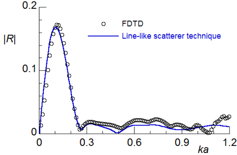
Fig. 6.17 Reflection coefficient modulus versus nondimensional frequency for a non-uniform (Gaussian) crack distribution. The solid line presents the theoretical result obtained by the line-like scatterer technique; the circles present the numerical data obtained from FDTD.
