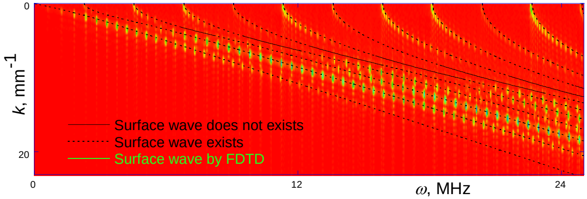
Fig. 5.9 The intensity picture of the FDTD-simulated wave field superposed on the analytically predicted dispersion curves for SHSW in the periodic semi-infinite strip with the unit-cell profile (5.4).
