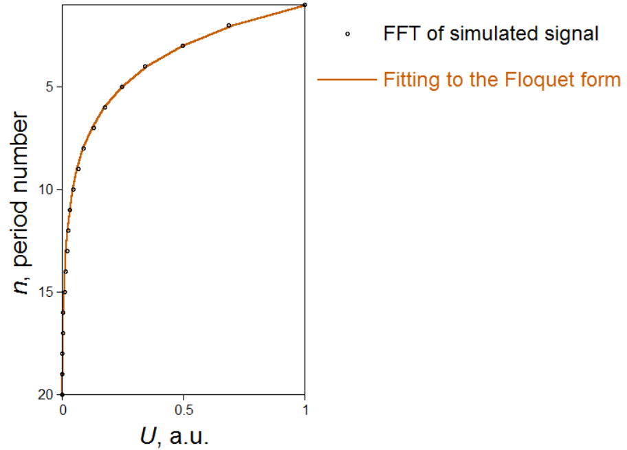
Fig. 5.6 Depth dependence of the particle velocity |v_3(\omega_0, k_0, y_n)| of the SHSW mode, extracted from FDTD simulation at (\omega_0, k_0) = (20.39, 0.98) , and its fitting to the Floquet form \exp(-K''y) with K'' = 0.35 \text{ mm}^{-1} .
