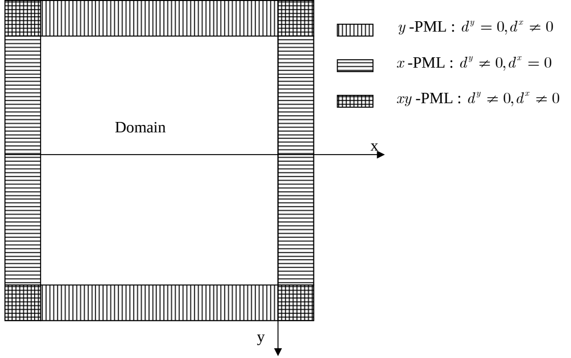
Fig. 3.9 Perfectly Matched Layers (PMLs)
