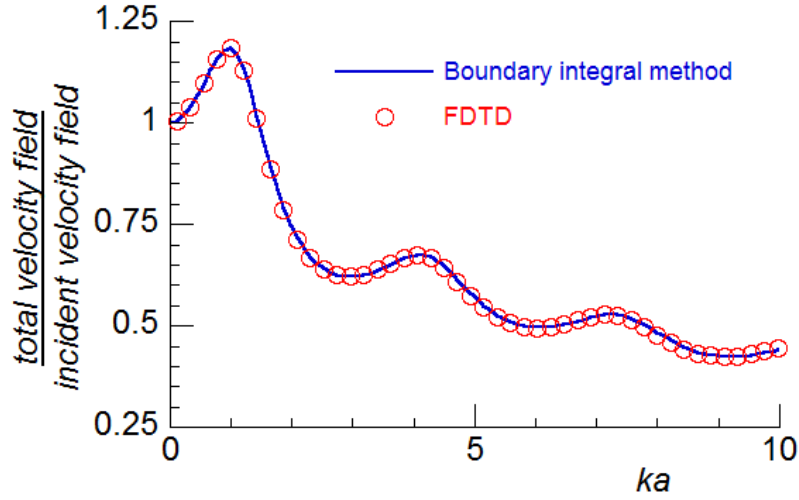
Fig. 6.1 Normalised velocity field v_s versus dimensionless frequency for a single crack of 2-mm length. The solid line presents the theoretical results; the empty circles present the numerical data extracted from the FDTD.
