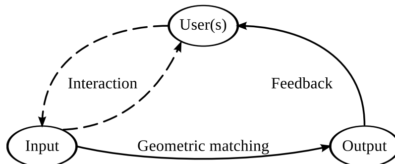
Figure 5.3: The semi-automatic interaction loop. We propose to enforce the standard interaction loop (dashed lines) by adding a real-time geometric matching whose input is defined by the user via the interaction technique, and whose output is the feedback to the user.
