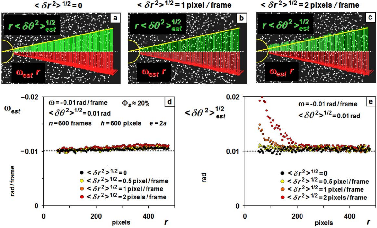
Fig. C.18 (a,b,c) Uniform circular motion of disks with both angular fluctuations \langle \delta \theta^2 \rangle^{1/2} = 0.01 \text{ rad} and radial fluctuations \langle \delta r^2 \rangle^{1/2} . Estimated angular velocity \omega_{\text{est}}(r) (d) and estimated rms angular fluctuation \langle \delta \theta^2 \rangle_{\text{est}}^{1/2} (e) versus radius 50 \text{ pixels} < r < 480 \text{ pixels} . Least squares fits of Eqs. C.12. Simulation parameters : \omega(r) = 0.01 \text{ rad/frame} , \langle \delta \theta^2 \rangle^{1/2} = 0.01 \text{ rad} , n = 600 \text{ frames} , h = 400 \text{ pixels} and 2a = 5 \text{ pixels} . \Phi_s = 20\% , \langle I \rangle = 125 and \langle \delta I^2 \rangle^{1/2} = 50 .
