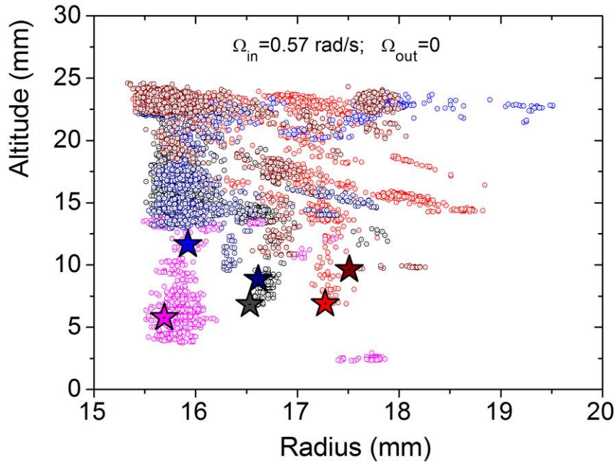
Fig.F.12 Meridian motions of a 100 \mu m tracer, recorded in passive SPT mode. Data with different colours come from different experiments. Stars represents initial position in each experiment.
