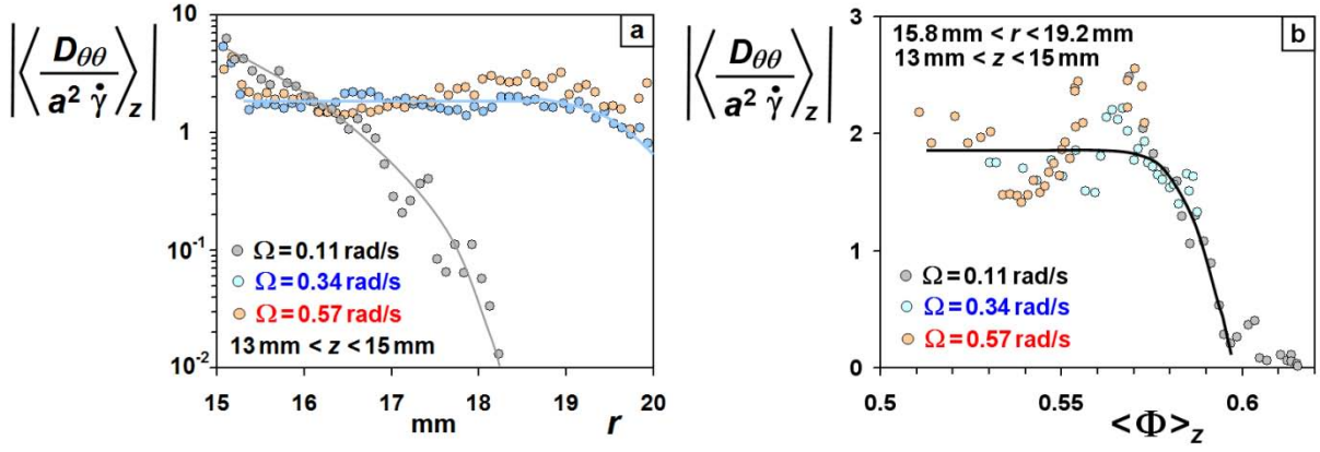
Fig. C.38 Dimensionless z averaged diffusion coefficient \left\langle D_{\theta\theta}(r, \Omega) / a^2 \dot{\gamma} \right\rangle_z in the non density-matched suspension versus the radial distance r (a) or the z averaged particle concentration \langle \Phi \rangle_z (b) for inner cylinder angular velocity \Omega = 0.114 \text{ rad/s} , \Omega = 0.342 \text{ rad/s} and \Omega = 0.57 \text{ rad/s} . Altitudes 13 \text{ mm} < z < 15 \text{ mm} and H \approx 30 \text{ mm} .
