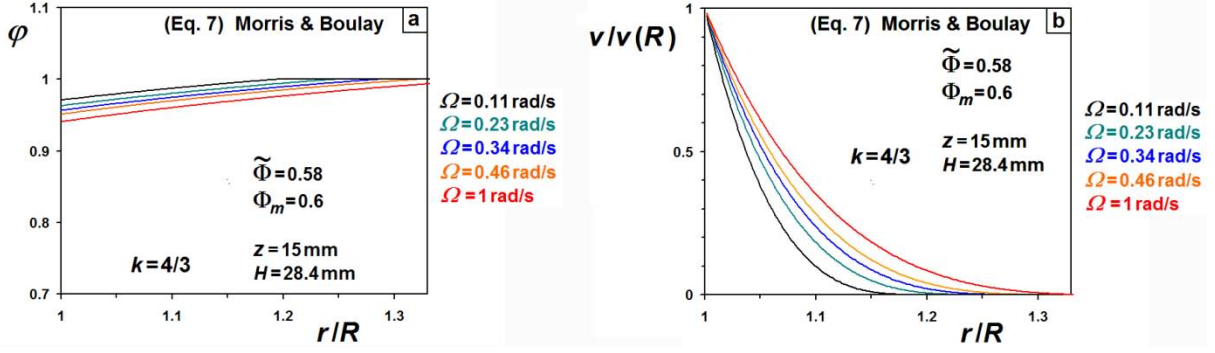
Fig. E.22 Shear induced re-suspension of non buoyant particles in a viscous fluid ( \tilde{\Phi} = 0.58 , \Phi_m = 0.6 , h_o = 27.5 \text{ mm} , H = 28.4 \text{ mm} , \Delta\rho = 0.3 \text{ g/cm}^3 ). Stationary concentration profile \phi(r, \Omega) and dimensionless velocity profile v(r, \Omega)/v(R, \Omega) versus dimensionless radius r/R for z = 15 \text{ mm} and angular velocity 0.11 \text{ rad/s} < \Omega < 0.57 \text{ rad/s} . Predictions of the force balance model using the Morris & Boulay viscometric function f_{MB}(\phi) (Eq.7) with \Phi_m = 0.6 , \lambda_2 = 0.85 , \lambda_3 = 0.5 and k = 4/3 .
