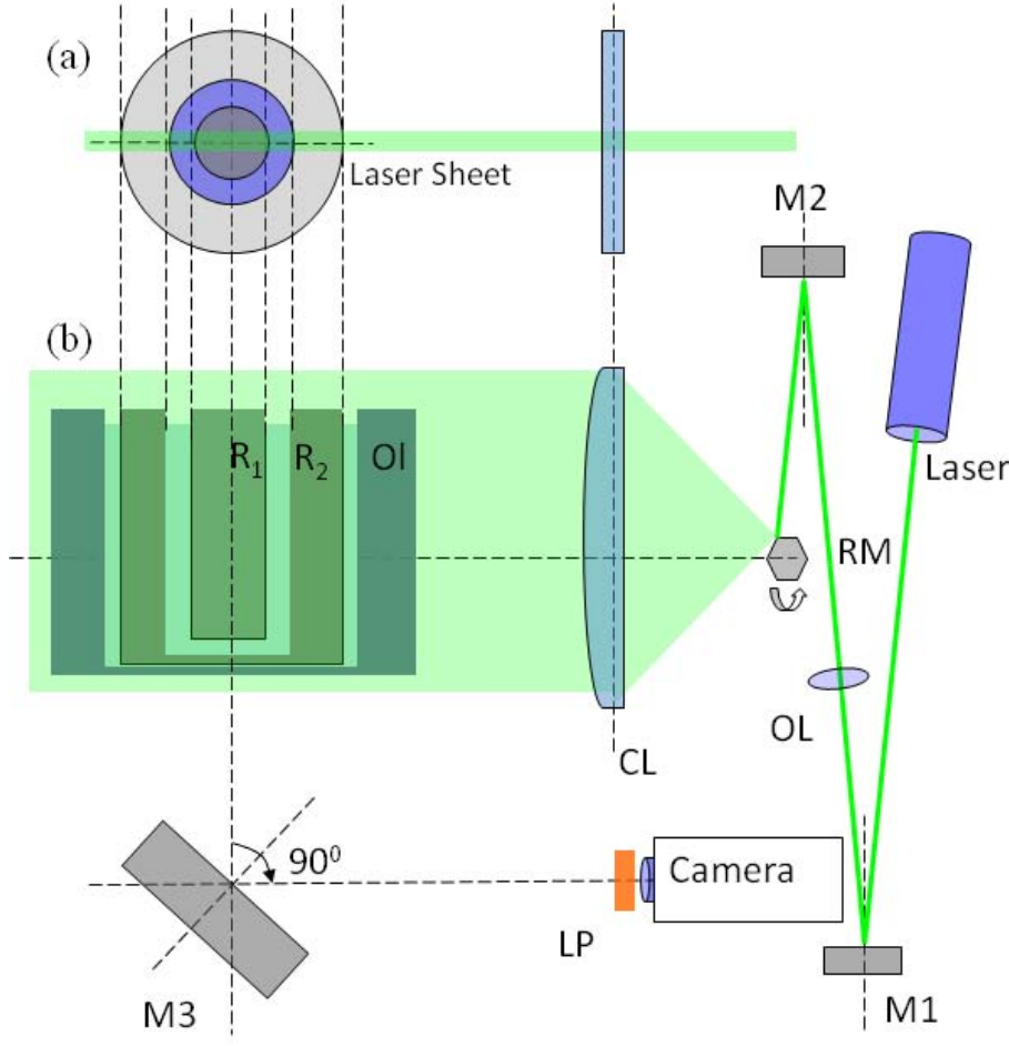
Fig.D.2 Top (a) and side view (b) of experimental setup and components. M1, M2, M3 : mirrors; RM : rotating mirror; CL: cylindrical lens (focal length: 240 mm); Ol : olearium; OL: spherical lens ( f=800\text{mm} ); LP: long pass filter; R_1, R_2 : inner and outer cylinder radii.
