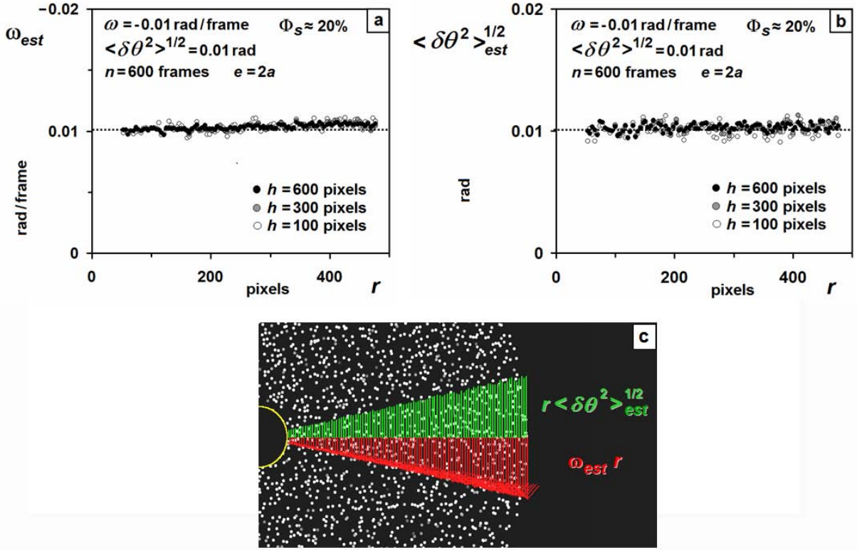
Fig. C.17 Estimated angular velocity \omega_{\text{est}}(r) (a) and rms angular fluctuation \langle \delta\theta^2 \rangle_{\text{est}}^{1/2} (b) of disks with circular motion as a function of radius 50\text{ pixels} < r < 480\text{ pixels} . (c) Estimated velocity profile \omega_{\text{est}} r (red arrows) and rms angular fluctuation profile r \langle \delta\theta^2 \rangle_{\text{est}}^{1/2} (green arrows). Least squares fits of Eqs. C.12. Simulation parameters : \omega(r) = 0.01\text{ rad/frame} , \langle \delta\theta^2 \rangle^{1/2} = 0.01\text{ rad} , n = 600\text{ frames} , h = 400\text{ pixels} and 2a = 5\text{ pixels} . \Phi_s = 20\% , \langle I \rangle = 125 and \langle \delta I^2 \rangle^{1/2} = 50 .
