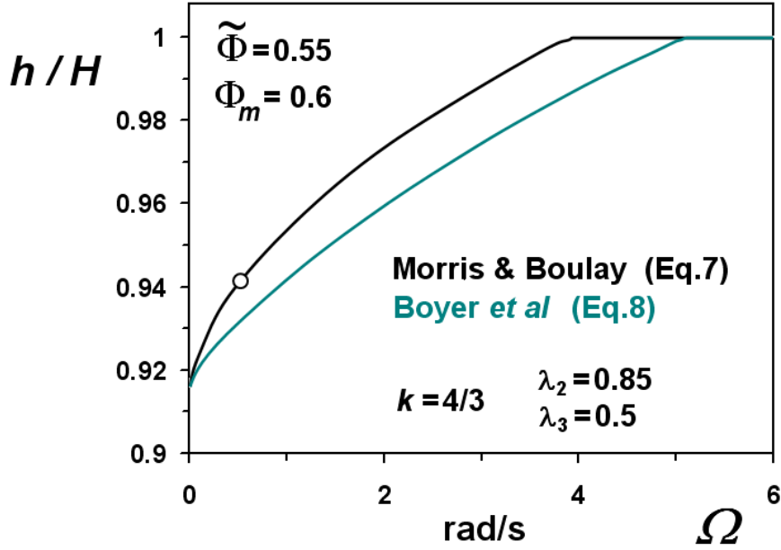
Fig. E.17 Shear induced re-suspension of non buoyant particles in a viscous fluid ( \tilde{\Phi} = 0.55 , \Phi_m = 0.6 , H = 30\text{mm} , \Delta\rho = 0.3\text{g/cm}^3 ). Reduced height h(\Omega)/H of the suspension versus angular velocity \Omega of the inner cylinder for Morris & Boulay f_{MB}(\varphi) (a) (Eq.E.7) or Boyer viscometric function f_{BPG}(\varphi) (b) (Eq.E.8) with \lambda_2 = 0.85 , \lambda_3 = 0.5 , \varphi_c = 0.22/\Phi_m and k = 4/3 . The open symbol indicates the full fluidization of the suspension in the case of Morris & Boulay viscometric function while shear banding is always present for the Boyer et al function.
