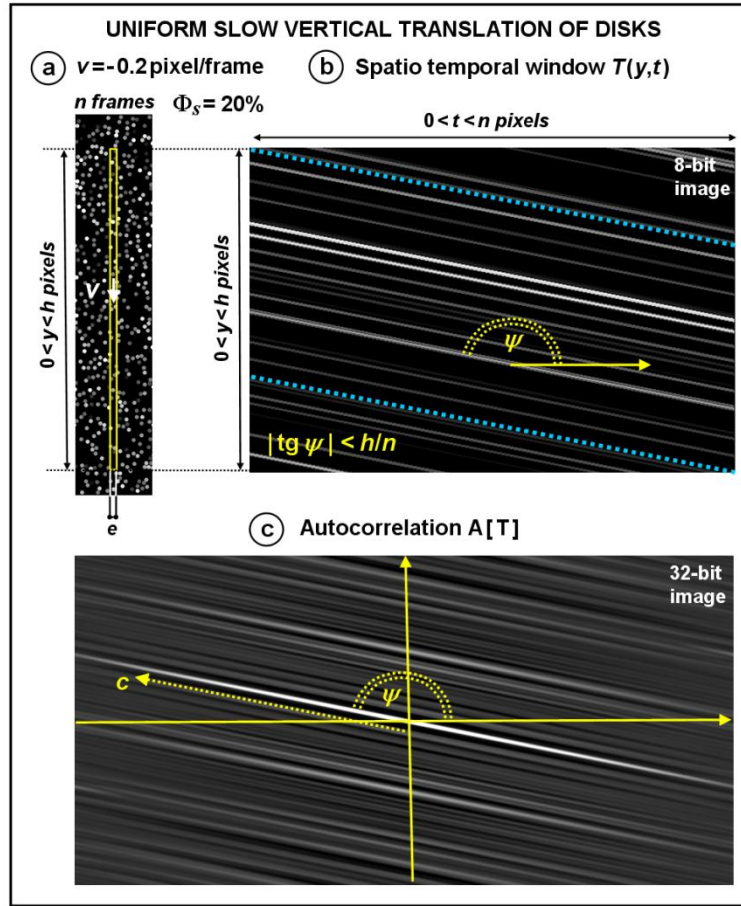
Fig. C.5 (a) Uniform slow vertical translation of disks (diameter 2a=5 pixels, v=-0.2 pixel/frame, surface density \Phi_s=20\% ) within a rectangular ROI (height h=400 pixels and width e=8 pixels). (b) Tilt angle \psi of disk trajectories in the spatiotemporal window T(y,t) . (c) Autocorrelation image A[T(y,t)] and bright ridge line along the \Psi direction. n=600 frames. \langle I \rangle = 125 and \langle \delta I^2 \rangle^{1/2} = 50 .
