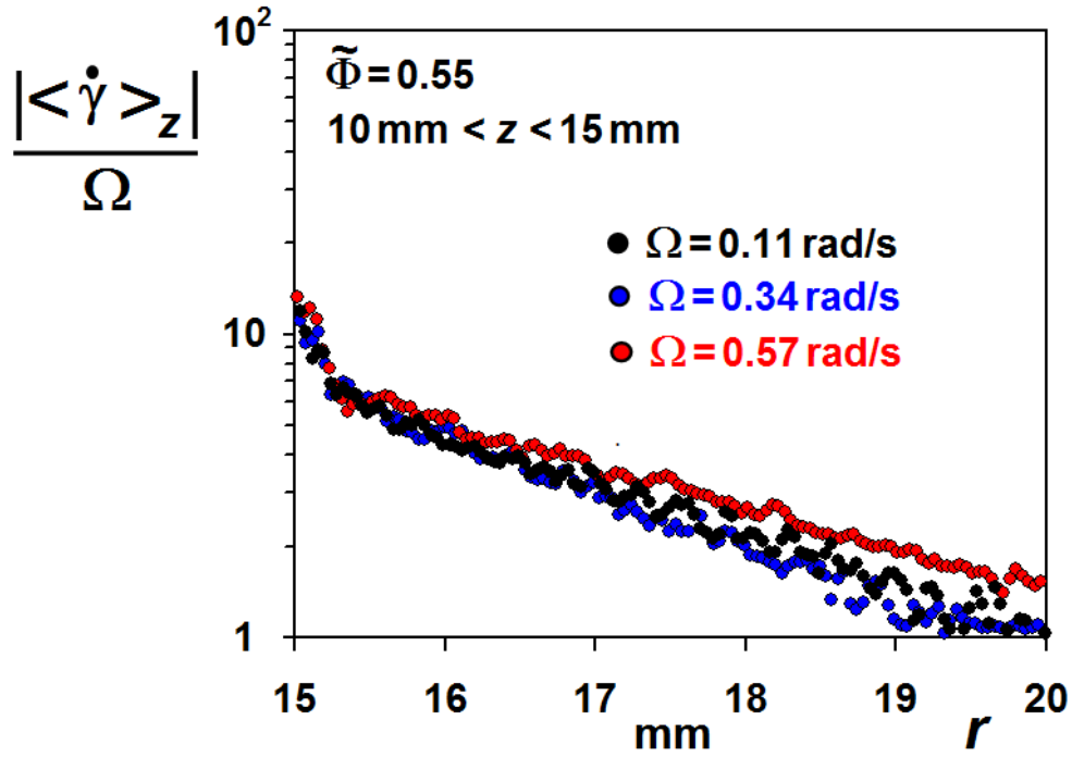
Fig. C.29 Dimensionless z averaged shear rate profile |\langle \dot{\gamma}(r, \Omega) \rangle_z| / \Omega in the 55% density-matched suspension for \Omega = 0.114 , 0.342 and 0.57 \text{ rad/s} . Altitudes 10 \text{ mm} < z < 15 \text{ mm} and H \approx 30 \text{ mm} .
