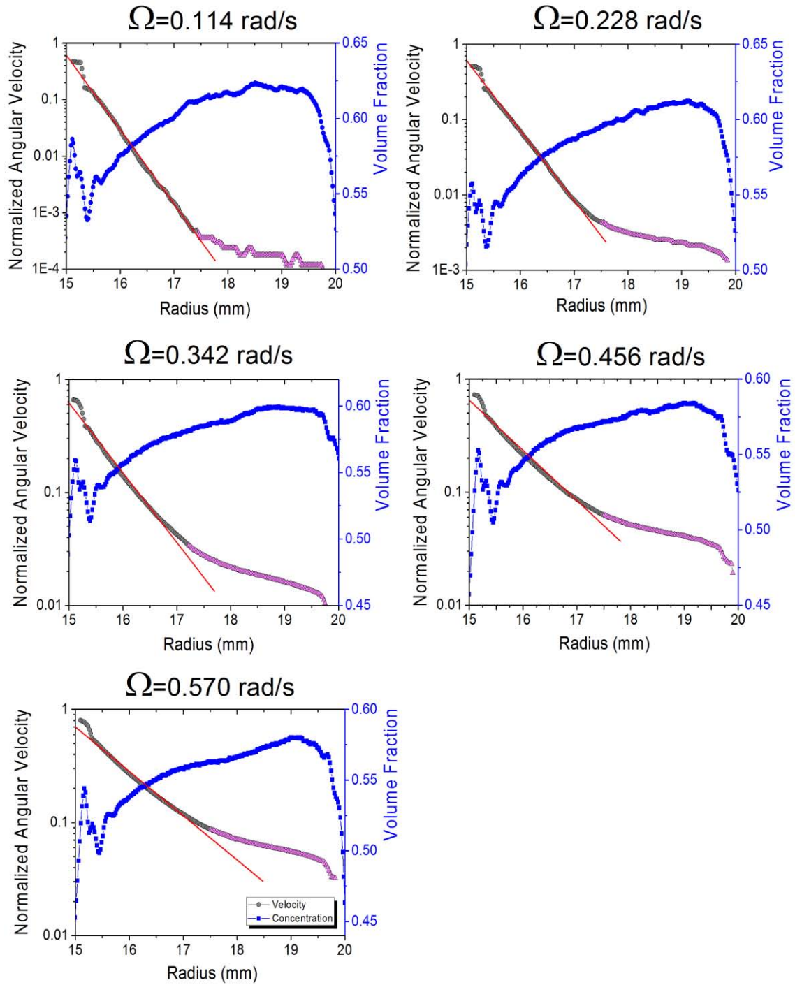
Fig.D.13 Combining velocity and concentration data for the C16-S150 system ( \Delta\rho > 0 ), at z = 15 mm. Velocity is plotted in semi-log scale, to show the transition between “active”(in gray) and “arrested”(in magenta) zones. Straight lines (in red) along the velocity profiles are guides to the eye.
