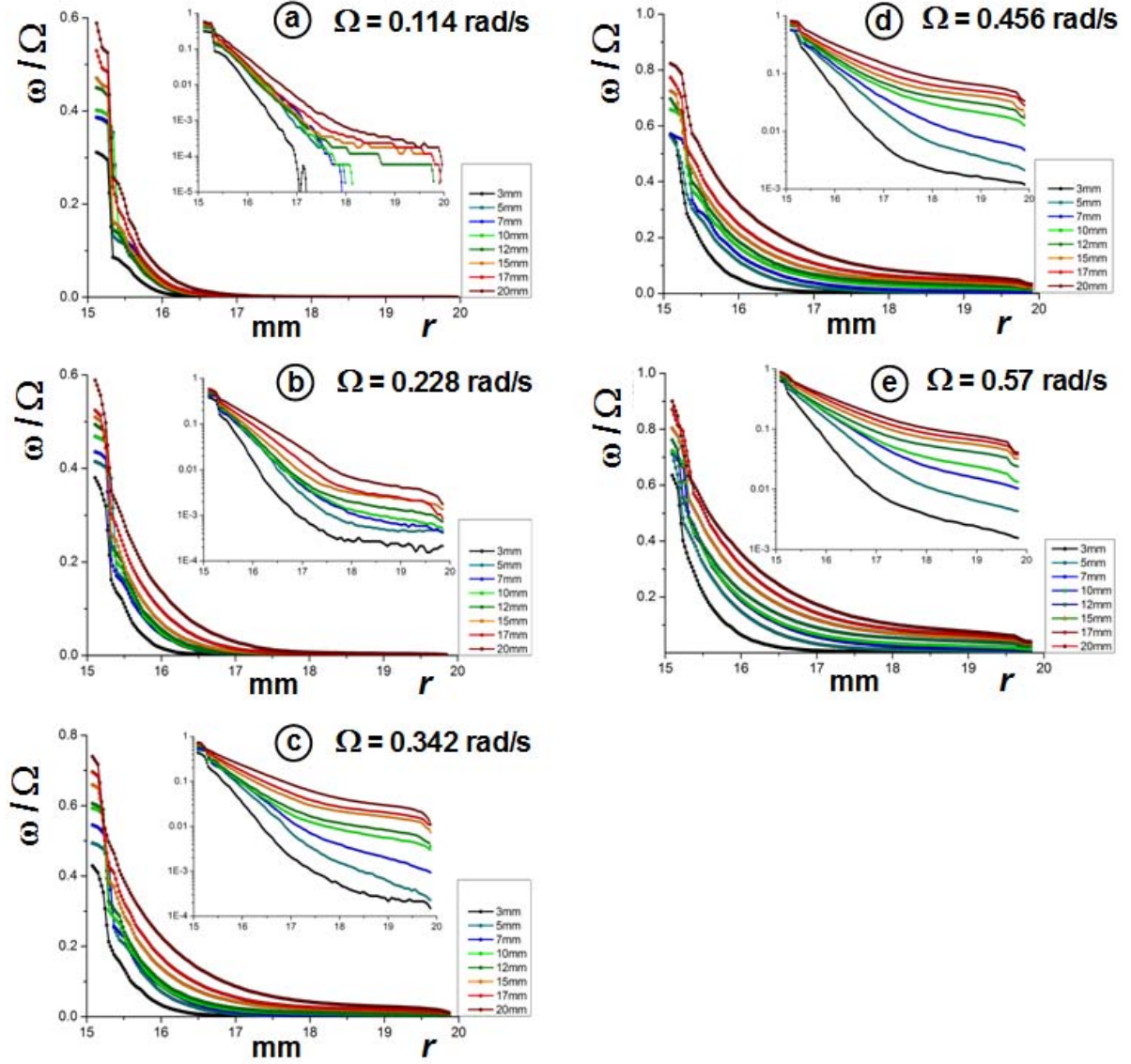
Fig. C.34 Dimensionless angular velocity profile \omega(r, z)/\Omega of the non density-matched suspension for inner cylinder angular velocity \Omega = 0.114 rad/s (a), \Omega = 0.228 rad/s (b), \Omega = 0.342 rad/s (c), \Omega = 0.456 rad/s (d), and \Omega = 0.57 rad/s (e). Altitudes 3 \text{ mm} < z < 20 \text{ mm} and H \approx 30 \text{ mm} .
