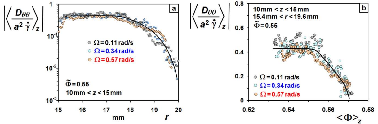
Fig. C.30 Dimensionless z -averaged diffusion coefficient \left\langle \frac{D_{\theta\theta}(r, \Omega)}{a^2 \dot{\gamma}} \right\rangle_z in the 55% density -matched suspension versus the radial distance r (a-panel) or the z averaged particle concentration \langle \Phi \rangle_z (b-panel) for \Omega = 0.114, 0.342 and 0.57 \text{ rad/s} . Altitudes 10 \text{ mm} < z < 15 \text{ mm} and H \approx 30 \text{ mm} .
