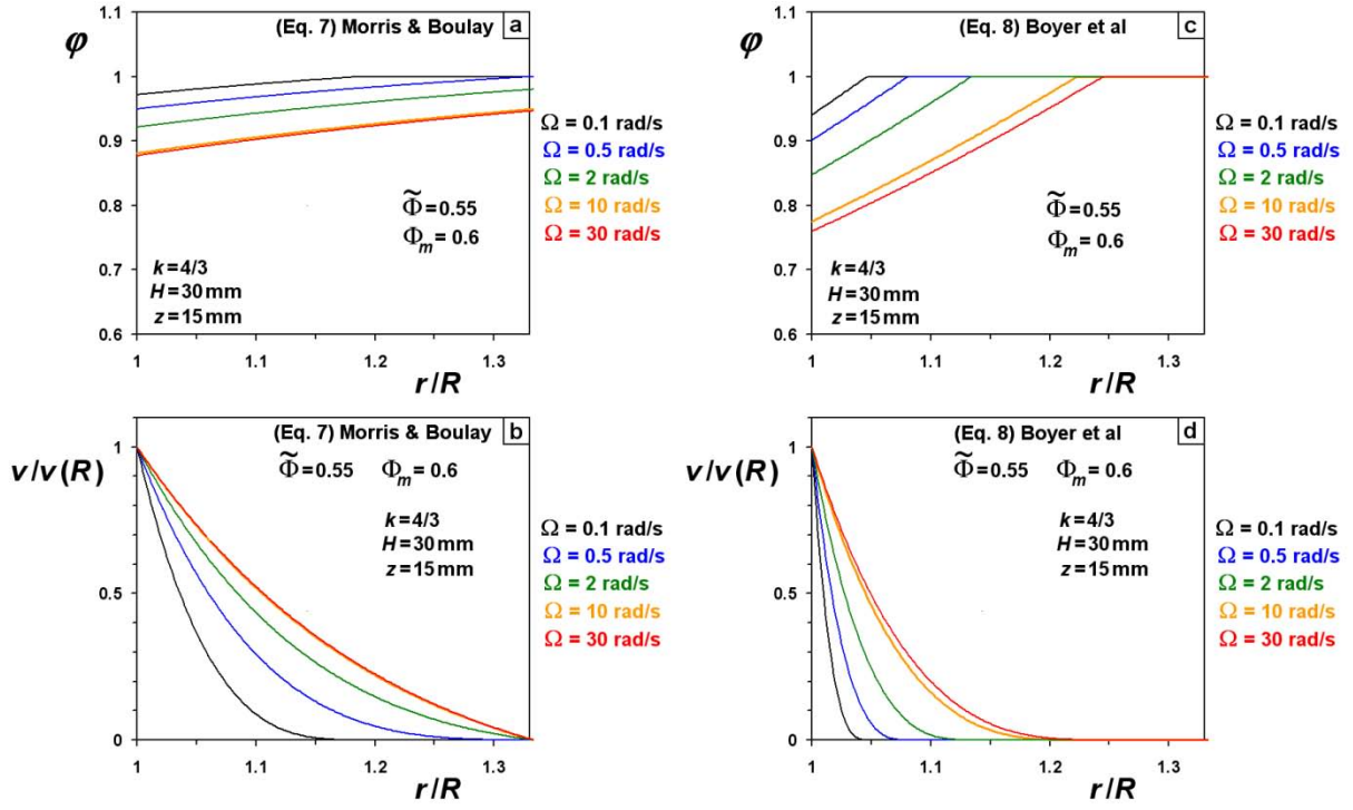
Fig. E.16 Shear induced re-suspension of non buoyant particles in a viscous fluid ( \tilde{\Phi} = 0.55 , \Phi_m = 0.6 , H = 30 \text{ mm} , \Delta\rho = 0.3 \text{ g/cm}^3 ). Stationary concentration profile \phi(r, \Omega) and dimensionless velocity profile v(r, \Omega)/v(R, \Omega) versus dimensionless radius r/R either for the Morris & Boulay f_{MB}(\phi) (a,b) (Eq.7) or the Boyer viscometric function f_{BPG}(\phi) (c,d) (Eq.8) at altitude z = H/2 with \lambda_2 = 0.85 , \lambda_3 = 0.5 and k = 4/3 .
