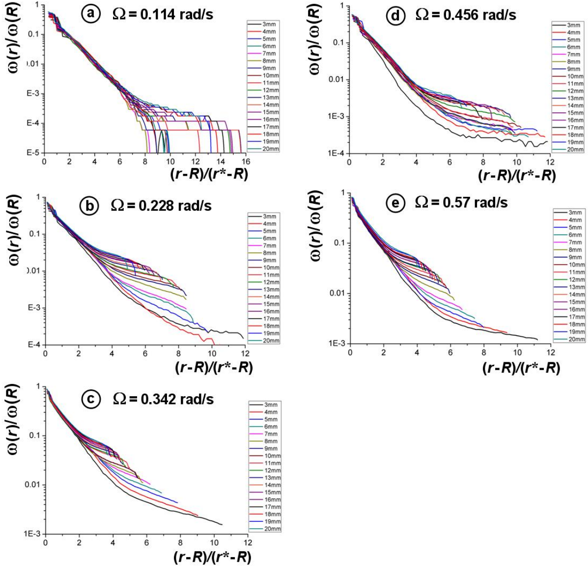
Fig. C.36 Dimensionless angular velocity profile \omega(r,z)/\omega(R,z) of the non density-matched suspension versus rescaled distance (r-R)/(r^*-R) for \Omega=0.114 \text{ rad/s} (a), \Omega=0.228 \text{ rad/s} (b), \Omega=0.342 \text{ rad/s} (c), \Omega=0.456 \text{ rad/s} (d), and \Omega=0.57 \text{ rad/s} (e). Altitudes 3 < z < 20 \text{ mm} and H \approx 30 \text{ mm} .
