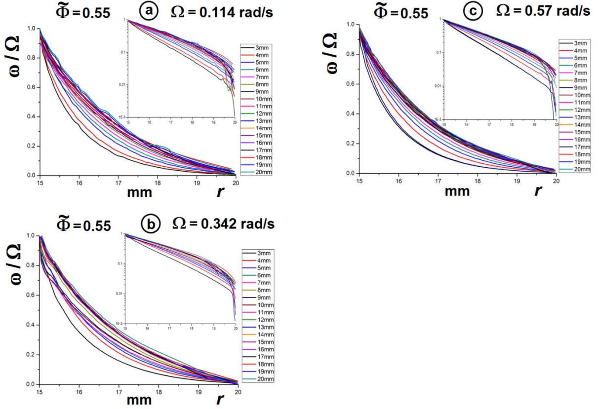
Fig. C.27 Dimensionless angular velocity profile \omega(r, z)/\Omega of the 55% density-matched suspension for inner cylinder angular velocity \Omega=0.114\text{rad/s} (a), \Omega=0.342\text{rad/s} (b) and \Omega=0.57\text{rad/s} (c). Altitudes 3\text{ mm} < z < 20\text{ mm} and H \approx 30\text{mm} .
