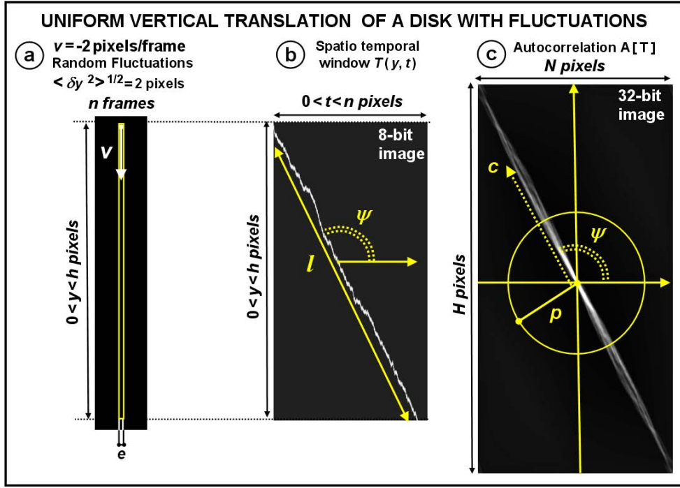
Fig. C.3 (a) Uniform vertical translation of a disk with longitudinal random fluctuations (diameter 2a=9 \text{ pixels} , v=-2 \text{ pixels/frame} , \langle \delta y^2 \rangle^{1/2}=2 \text{ pixels} ) within a rectangular ROI ( h = 550 \text{ pixels} and e=2a ). (b) Tilt angle \psi of the disk trajectory with length l in the spatiotemporal window T(y,t) . (c) Autocorrelation image A[T(y,t)] and ridge line in \Psi direction. n = 290 \text{ frames} .
