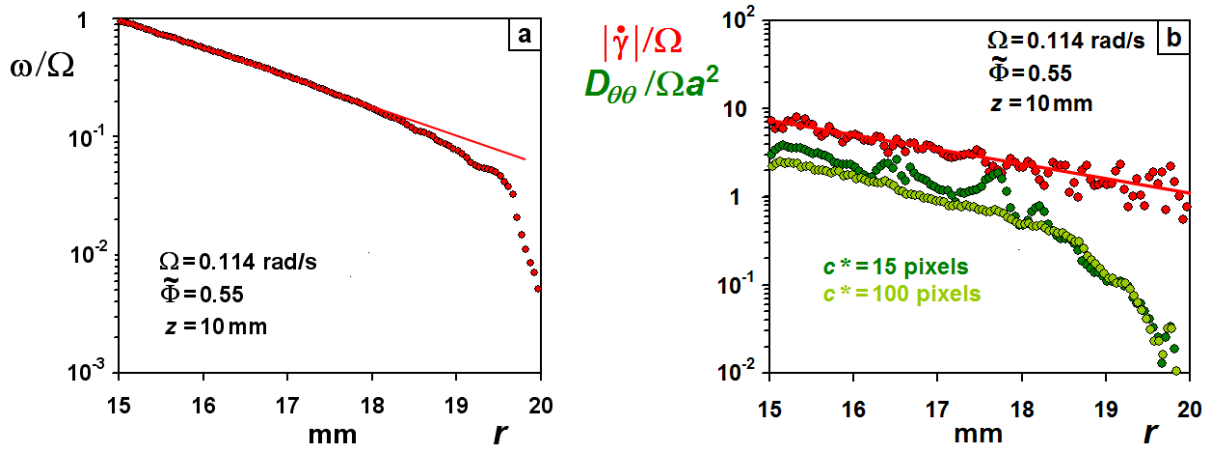
Fig. C.26 (a) Semi-log plot of the dimensionless angular velocity profile \omega(r)/\Omega of the 55% density-matched suspension (angular velocity of the inner cylinder \Omega = 0.114 \text{ rad/s} , altitude z = 10 \text{ mm} and H \approx 30 \text{ mm} ). (b) Semi-log of the dimensionless shear rate profile |\dot{\gamma}(r)|/\Omega = (r/\Omega)\partial\omega(r)/\partial r and dimensionless diffusion coefficient D_{\theta\theta}(r)/\Omega a^2 ( c^* = 15 \text{ pixels} or c^* = 100 \text{ pixels} ).
