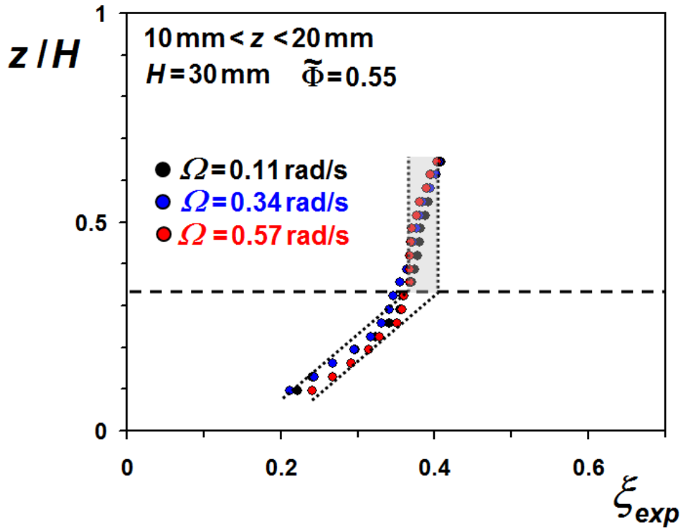
Fig. C.28 Dimensionless decay length \xi_{exp}(z, \Omega) = (r^* - R)/(R_{out} - R) versus the reduced altitude z/H in the 55% density-matched suspension for \Omega = 0.114, 0.342 and 0.57\text{rad/s} .
