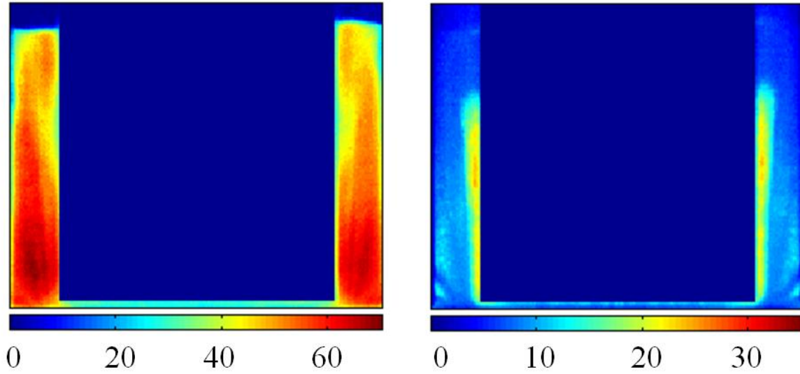
Fig. F.14 Shear-induced segregation in Couette cell (courtesy: Marie Lenoble-Eloy). Mixture of large ( 180\ \mu\text{m} ) and small ( 20\ \mu\text{m} ) particles in C16S150 ( \Delta\rho > 0 ), in 16/84 % proportion. The figure shows concentrations maps in stationary regime, for \Omega = 0.31\ \text{rad/s} : small particles at left, and large ones at right. Values of concentration follow the colour codes at bottom. Here concentrations were obtained from colored tracers.
