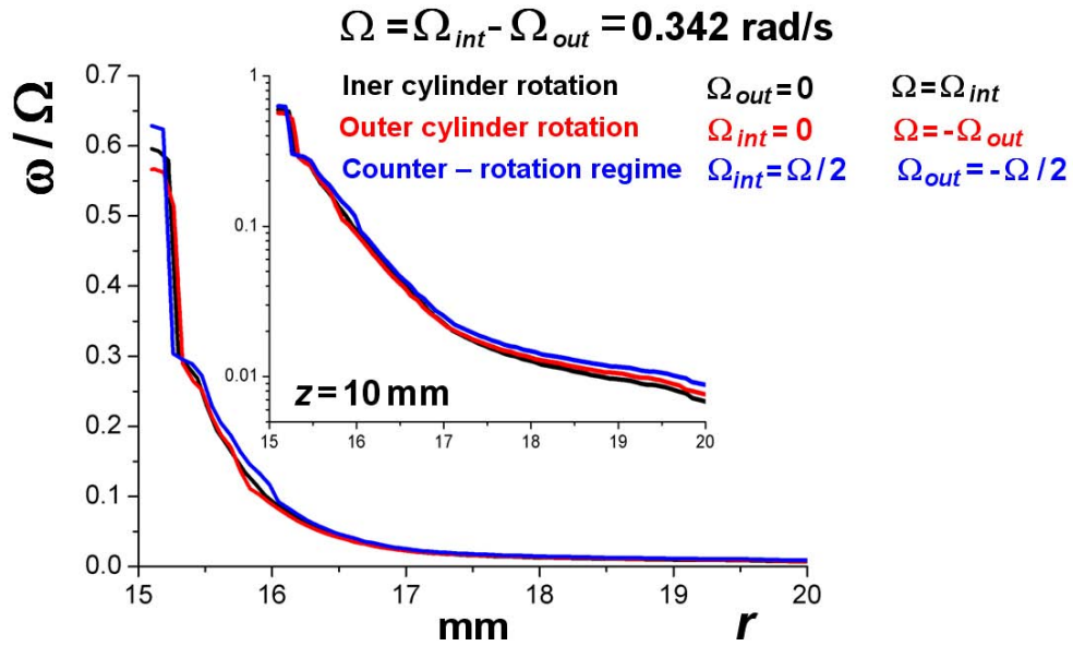
Fig. C.39 Steady state angular velocity profiles \omega(r)/\Omega of the non density-matched suspension for a constant differential angular velocity \Omega = \Omega_{int} - \Omega_{out} = 0.342 \text{ rad/s} between inner and outer cylinders : rotation of the inner cylinder only (black solid curves), rotation of the outer cylinder only (red solid curves) or counter-rotation mode (blue solid curves). The insert shows a semi-log plot. Altitude z = 10 \text{ mm} and H \approx 30 \text{ mm} .
