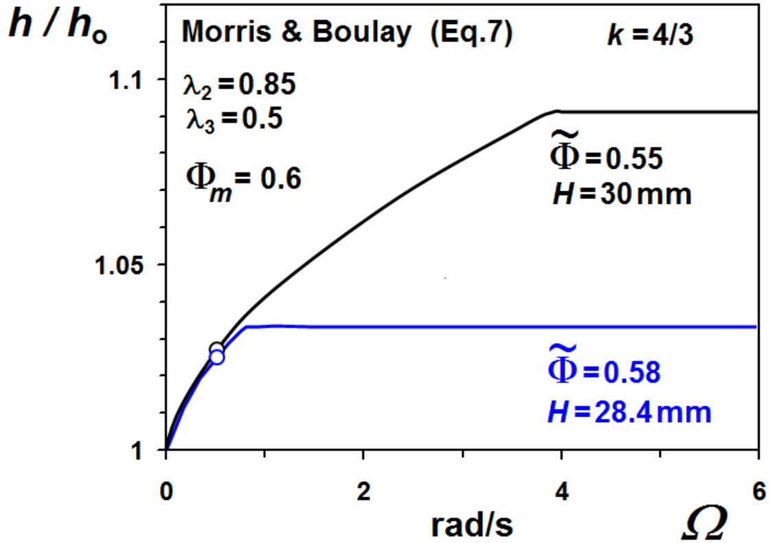
Fig. E.21 Shear induced re-suspension of non buoyant particles in a viscous fluid ( \Phi_m = 0.6 , h_0 = 27.5 mm, \Delta\rho = 0.3 g/cm 3 ). Reduced height h(\Omega)/h_0(\Omega=0) of the suspension versus angular velocity \Omega of the inner cylinder for a volume averaged concentration \tilde{\Phi} = 0.55 ( H = 30 mm) or \tilde{\Phi} = 0.58 ( H = 28.4 mm). Morris and Boulay viscometric function f_{MB}(\varphi) with \lambda_2 = 0.85 , \lambda_3 = 0.5 , \varphi_c = 0.22/\Phi_m and k = 4/3 . The open symbols indicate the full fluidization of the suspension.
