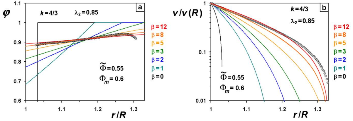
Fig. E.6 (a) Stationary concentration profile \phi(r) ; (b) velocity profile v(r)/v(R) , versus dimensionless radius r/R for different integral values of the \beta exponent, with k = 4/3 , \lambda_2 = 0.85 , \tilde{\Phi} = 0.55 and \Phi_m = 0.6 . Grey circles are experimental data (see Fig. E.7 and chapters C and D).
