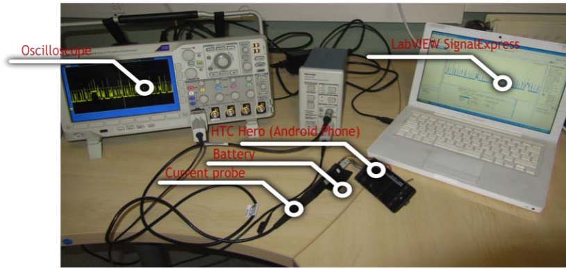
Figure 28: Our measurement platform for power monitoring
