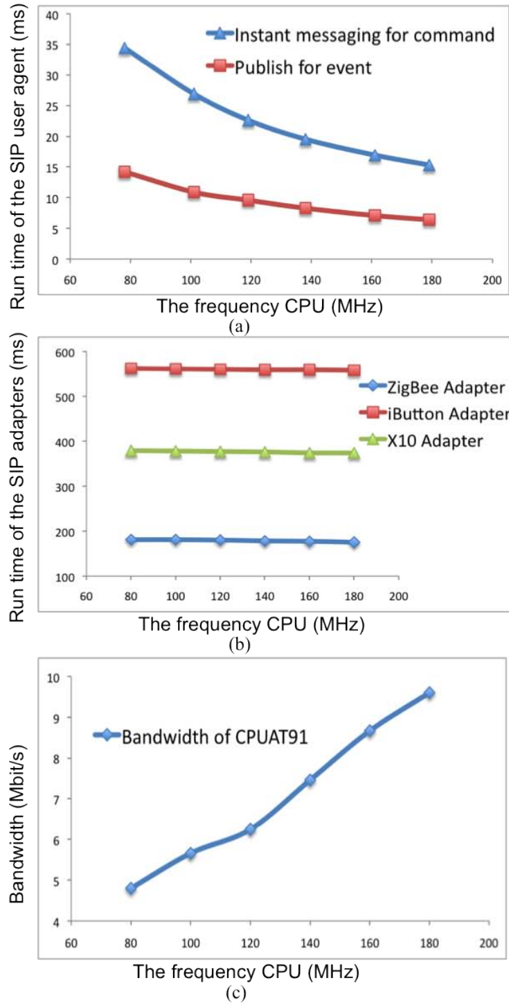
Figure 19: Performances as a function of CPU frequency: (a) Variation of run time of two interaction modes of the SIP user agent with varying the frequency CPU (b) Variation of run time of read or write operations of the SIP adapters with varying the frequency CPU (c) Variation of bandwidth for our SBC board with varying the frequency CPU
