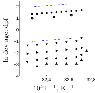
Figure 2.5: Ln developmental (dev) age as a function of inverse temperature ( T ). Model predictions for birth ( \blacksquare ) and data: protruding mouth stage ( \circ , from Kimmel et al. (1995) ), 8 cell stage ( \blacktriangle ), late cleavage ( \blacktriangleleft ), very late blastula ( \blacktriangleright ), and blastoderme 3/4 yolk sphere ( \blacktriangledown ), all from Shirone and Gross (1968) . The slope of the dashed lines gives an Arrhenius temperature of 3000 K.
