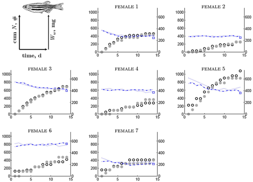
Figure I.1: DEB model fit to individual control females. Data kindly provided by S. Bourrachot from her thesis (Bourrachot, 2009). Parameters can be found in tables 5.4 and 5.3. Left y-axis: empty circles (black) represent observed cumulated (cum) number N of eggs spawned ( \# ) and full circles (grey) represent model predictions. Right y-axis: dotted line represents predicted wet mass using buffer handling rules, mg (eq. 5.8). Dot-dashed line represents predicted wet mass without buffer handling rules, mg (eq. 5.9). The square represents final observed wet mass for that individual.
