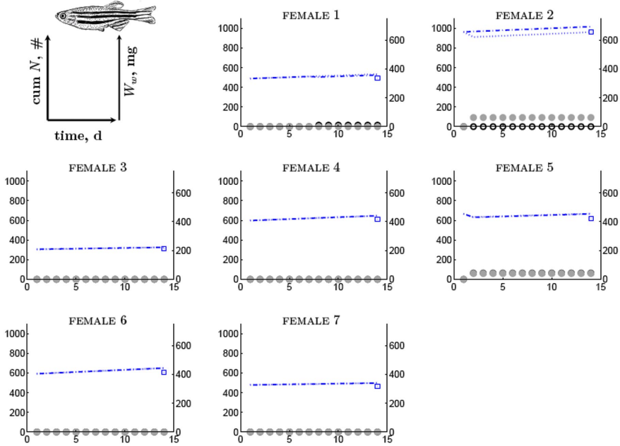
Figure I.3: DEB model fit to individual females exposed to 1054 nmol U l -1 for 20d prior to the reproduction trial. Data kindly provided by S. Bourrachot from her thesis (Bourrachot, 2009). The model assumes U increases volume-linked somatic maintenance. Parameters can be found in tables 5.4 and 5.3. Left y-axis: empty circles (black) represent observed cumulated (cum) number N of eggs spawned (#) and full circles (grey) represent model predictions. Right y-axis: dotted line represents predicted wet mass using buffer handling rules, mg (eq. 5.8). Dot-dashed line represents predicted wet mass without buffer handling rules, mg (eq. 5.9). The square represents final observed wet mass for that individual.
