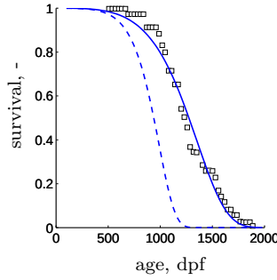
Figure 2.4: Survival probability in relation to nutritional status as predicted by the DEB ageing module. ( \square ) data from Gerhard et al. (2002) outbred tank 2; solid line: model prediction for f = 0.8 . Dashed line: predicted survival for f = 1 . T = 26^\circ\text{C} .
