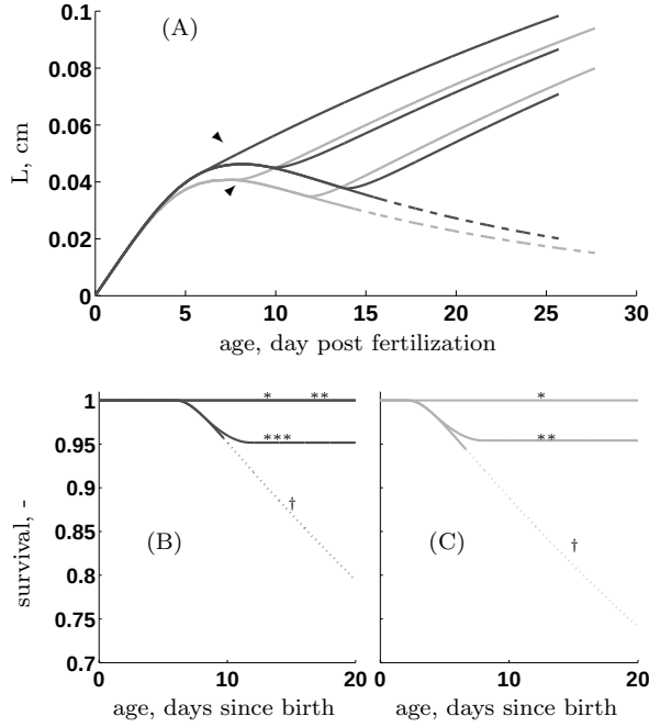
Figure 3.2: Impact of delays in first feeding on growth at reference temperature ( 20^{\circ}\text{C} ). s_H = 2 ; k'_J = 2.4 ; f = 1 (see table 3.2). (A) structural length ( L ) against age for E_0 = 1.7 (black lines) and E_0 = 1.1 (grey lines); arrowheads: birth; dashed lines: instantaneous death by shrinking. E_0 = 1.7 : feeding is never initiated (negative growth till death by shrinking) and feeding is delayed 0, 4 and 8 days after birth. E_0 = 1.1 : feeding feeding is never initiated and feeding is delayed 0 and 4 days after birth. Survival probability for E_0 = 1.67 (B) and E_0 = 1.1 (C). Survival for delays in initial feeding of 0 days after birth (*), 4 days after birth (**), 8 days after birth (***) and feeding is never initiated (†). Dotted line: all organisms have died from shrinking.
