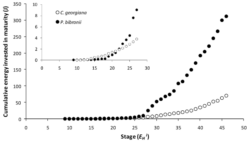
Figure 4.5: Cumulated energy invested in maturity against stage of development for Crinia georgiana and Pseudophryne bibronii until metamorphosis. Insert shows cumulative energy invested in maturity against stage until birth. Each stage is represented by E_H^i where i refers to stage 1 - 46 (Gosner, 1960). Hatch occurs at E_H^{27} and birth at E_H^{27} in C. georgiana . Hatch and birth both correspond with E_H^{27} in P. bibronii .
