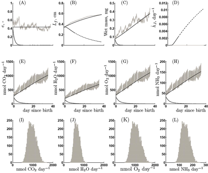
Figure 3.4: Model outputs computed at 20°C. s_H = 2 and k'_J = 0.024 \text{ day}^{-1} . First row: an example of scaled reserve density ( e_i ), observed length ( L_f ), wet mass, rejuvenation hazard ( \dot{h}_J ) for an individual sampled randomly from the Monte Carlo simulation study. Second row: an example of fluxes of \text{CO}_2 , \text{H}_2\text{O} , \text{O}_2 and \text{NH}_3 against age since birth from the same individual sampled randomly from the Monte Carlo simulation study. Black: stochastic mineral fluxes for that individual ( x = 0.75 , E_0 = 1.67 \text{ J} , f alternates between 0 and 1) are compared to deterministic predictions (smooth lines) for f = x/(1+x) and f = 0 ( E_0 = 1.67 \text{ J} ). When f = 0 the deterministic mineral fluxes go to 0 and the dotted line is when structure reaches a fraction \delta_X = 0.75 of the maximum structure (instantaneous death is assumed at this point). Bottom row: distribution of each mineral flux at age 30 since birth for 5000 Monte Carlo trials ( x = 0.75 , E_0 = 1.67 \text{ J} , f alternates between 0 and 1). Please note that the x and y axis of fluxes of \text{NH}_3 differ.
