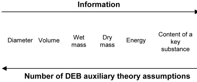
Figure 3.1: Modified from Kamler (2005). Egg size is measured in many different ways. Assumptions of auxiliary theory link these measurements to amounts of reserve and structure (egg size to initial amount of energy in reserve), which comes with some parameters (see table 3.2, auxiliary parameters).
