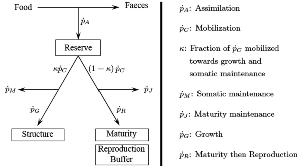
Figure 2.1: Conceptual organisation of animal metabolism as defined by DEB theory (Kooijman, 2010). Arrows: energy fluxes ( \text{J d}^{-1} ); boxes: state variables of the system. Embryo: \dot{p}_A = 0 ; birth: assimilation is switched on; puberty: allocation to maturity stops and allocation to reproduction starts. Energy allocated to reproduction accumulates in the reproduction buffer and is emptied at spawning.
