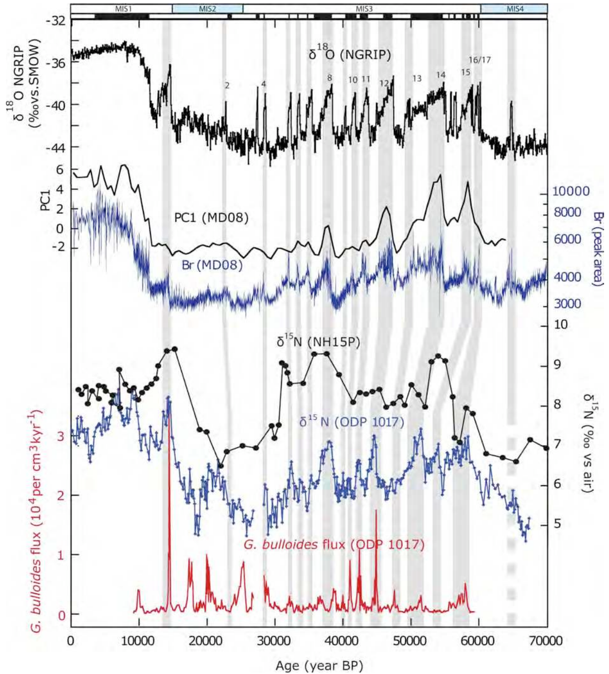
Figure Article 1.6. : The isotopic composition of the north GRIP ice core ( \delta^{18}\text{O}\text{‰}/\text{SMOW} ) based on the SS09sea time scale [Johnsen et al., 2001], the PC1 and Br counts (this study), the \delta^{15}\text{N} of the NH15P and ODP1017 cores, and the G. bulloides flux in ODP1017 [Hendy et al., 2004]. Gray vertical bars indicate DO warm periods; blue vertical bars indicate H events.
