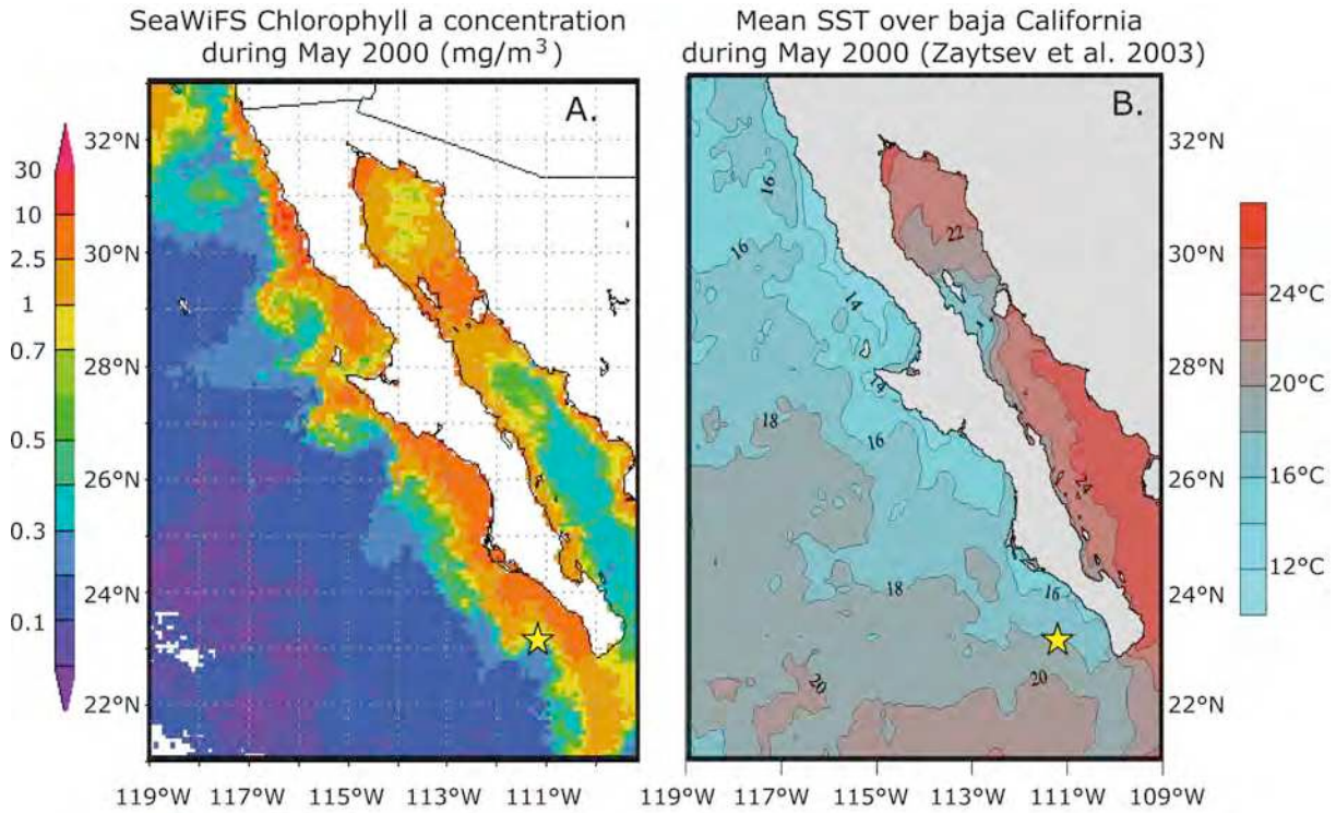
Figure Article 1. 2: A: The Seawifs chlorophyll-a concentration ( \text{mg}/\text{m}^3 ) estimation for May 2000 for Baja California ( http://reason.gsfc.nasa.gov/Giovanni/ ). The analyses and visualizations provided in Figure 2A were produced using the Giovanni online data system, developed and maintained by the NASA GES DISC [Acker and Leptoukh, 2007]. B: The mean SST for Baja California during May 2000 [Zaytsev et al. , 2003]. The core MD02-2508 site is indicated with a yellow star.
