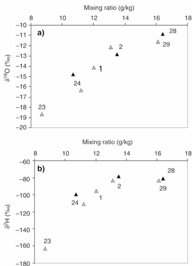
Figure 3. Vapour trap data ( \delta_{VT} ) plotted as a function of average mixing ratio of the sampling period of the day, for \delta^{18}\text{O} (a) and \delta^2\text{H} (b). The vapour is sampled at 2 cm above the evaporation surface (black triangles) and at 1.5 m high (grey triangles). The dates of sampling are indicating (days of August) two samples have been taken on 2 and 24 August. Correlation coefficient with the mixing ratio are r^2 = 0.87 and r^2 = 0.64 for \delta^{18}\text{O} and \delta^2\text{H} , respectively.
