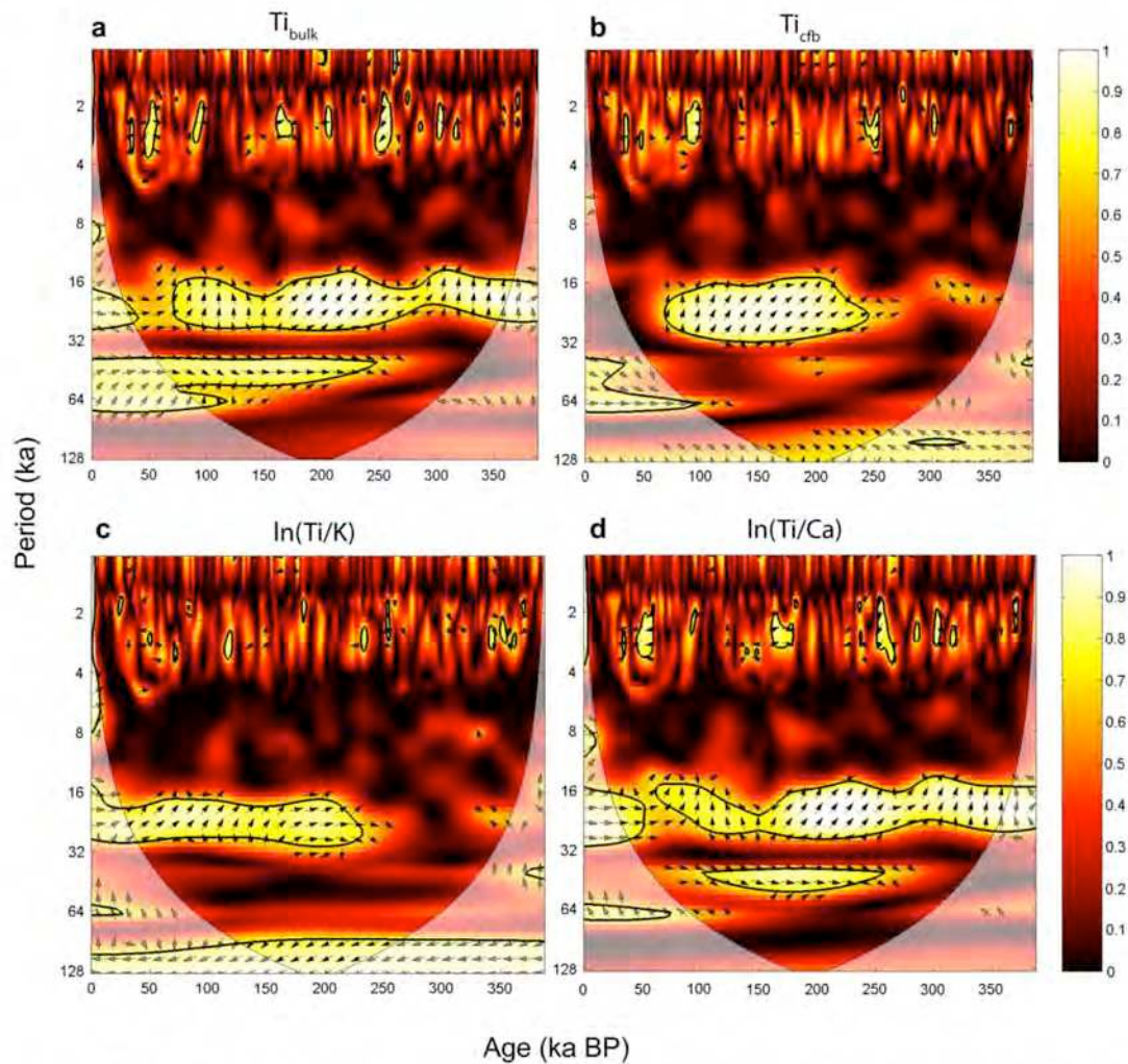
Fig. 7. The wavelet cross coherence and the phase spectra between local summer insolation (3°S, January) and the elemental records obtained from this study. The x-axis is the age (ka) and the y-axis is the period (ka). The right bars indicate the colour code of the coherency, whereas the vectors in the plots indicate phase lags. (a) The Ti_{bulk} concentration, (b) the Ti_{cfb} concentration, (c) the \ln(Ti/K) , and (d) the \ln(Ti/Ca) . The confidential part of the spectrum is included in the cone of influence and marked as statistically significant. The black thick line of statistical significance denotes the 5% significance level against the red noise background. In general, statistically significant patches in the spectrum plots are presented in the form of small or large “islands” or “bands”. Only when the entire “island” is located outside of the cone, should it be considered a result of a boundary effect. Vectors surrounding and inside the islands/bands indicate the phase relationship between the elemental records and insolation: rightward horizontal vectors present in-phase relationships and anti-clockwise rotations of vectors present larger lags.
