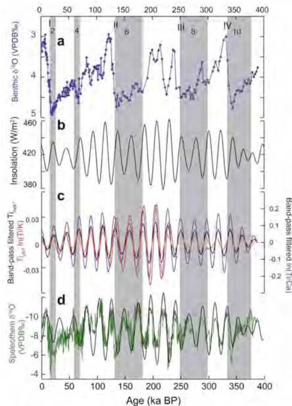
Fig. 8. The orbital-scale precipitation pattern over the past 400 ka. (a) The benthic foraminiferal \delta^{18}\text{O} record ( U. peregrina ) of core MD05-2920. (b) Local summer insolation (3°S, January) (Paillard et al., 1996; Laskar et al., 2004). (c) The precession band-pass filtered elemental records of core MD05-2920. The T_{\text{bulk}} (black), T_{\text{Hulu}} (orange), \ln(T_{\text{Hulu}}) (red), and \ln(T_{\text{Ca}}) (blue). Thin curves indicate areas corresponding to a very low coherency with local insolation. (d) The speleothem \delta^{18}\text{O} record from the Sanbao, the Hulu, and the Linzu Caves (110°26'E, 31°40'N, 119°10'E, 32°30'N and 110°19'E, 31°31'N, respectively) from China (Wang et al., 2001; Wang et al., 2008; Cheng et al., 2009). The black curve indicates the precession band-pass filtered record. Vertical bars indicate glacial marine isotope stages 2, 4, 6, 8, and 10. Terminations I, II, III, and IV are also indicated. Band-pass filter with central frequency of 0.0454 \text{ ka}^{-1} and bandwidth of 0.01 \text{ ka}^{-1} . (For interpretation of the references to colour in this figure legend, the reader is referred to the web version of this article.)
