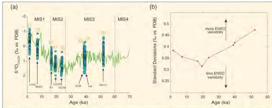
Figure 2: a ) Multiple-specimen (green curve) and individual specimen (blue circles) \delta^{18}\text{O}_{\text{COC2}} measurements performed on N. dutertrei planktonic foraminifera. Orange numbers indicate the number of individual foraminifer tests measured from each interval. Marine Isotopic Stages (MIS) are labeled. LHOL = Late Holocene, EHOL = Early Holocene, H1 and H4 = Heinrich events 1 and 4, LGM = Late Last Glacial Maximum, ELGM = Early Last Glacial Maximum, DOB and DO14 = Dansgaard-Oeschger interstadials 8 and 14. b ) Standard deviations of the individual \delta^{18}\text{O} measurements for each time slice, interpreted as thermocline variability induced by ENSO activity. Figures modified from Leduc et al., 2009a.
