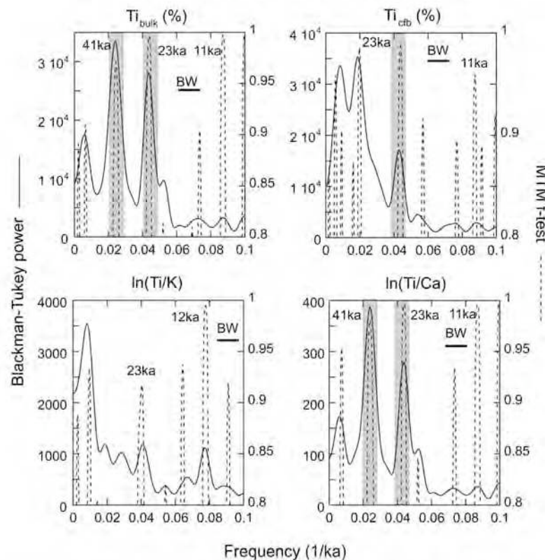
Fig. 6. The spectral analysis (multitaper method, MTM and Blackmann–Tukey) of bulk Ti concentrations ( Ti_{bulk} ), the CaCO_3 -free basis Ti concentrations ( Ti_{cfb} ) and the XRF intensity ratio, and the \ln(Ti/K) and the \ln(Ti/Ca) of core MD05-2920 performed with the AnalySeries 2.0 software (Paillard et al., 1996). The power spectra (solid lines, Blackmann–Tukey) and the significance value of the peaks (dashed lines, MTM F-Test) are shown. Vertical bands correspond to statistically significant cycles that correspond to the obliquity (41 ka), and the precession (23 ka).
