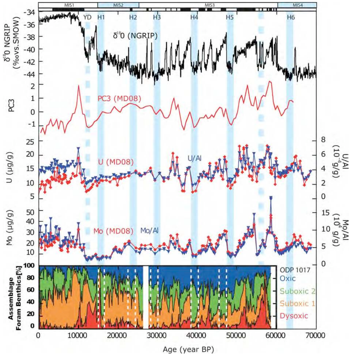
Figure Article 1.7 : The isotopic composition of the north GRIP ice core ( \delta^{18}\text{O}\text{‰/SMOW} ) based on the SS09sea time scale [Johnsen et al., 2001], PC3 in MD08 core, and the benthic foraminiferal assemblages within the ODP1017 core [Cannariato and Kennett, 1999]. Oxic assemblages indicate bottom water [\text{O}_2] > 1.5\text{ml/l} , suboxic corresponds to 0.3 < [\text{O}_2] < 1.5\text{ml/l} , and dysoxic assemblages to [\text{O}_2] < 0.3\text{ml/l} .
