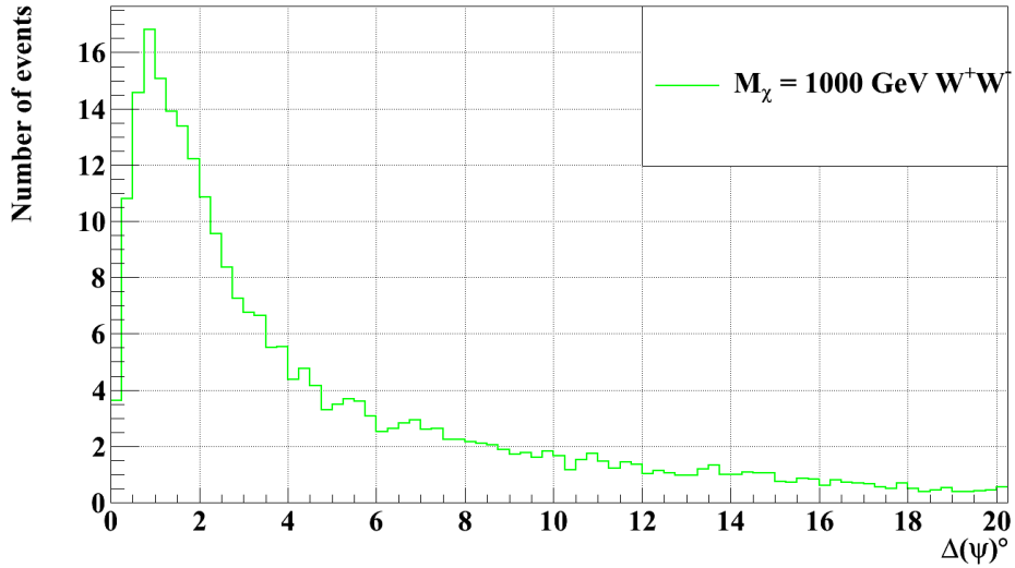
Figure 5.17: The differential distribution of number of events as a function of \Delta(\Psi) which is the angle between the neutrino trajectory and reconstructed muon track for one dark matter spectrum. A cut of 1.6 on \chi^2 was applied for this distribution.
