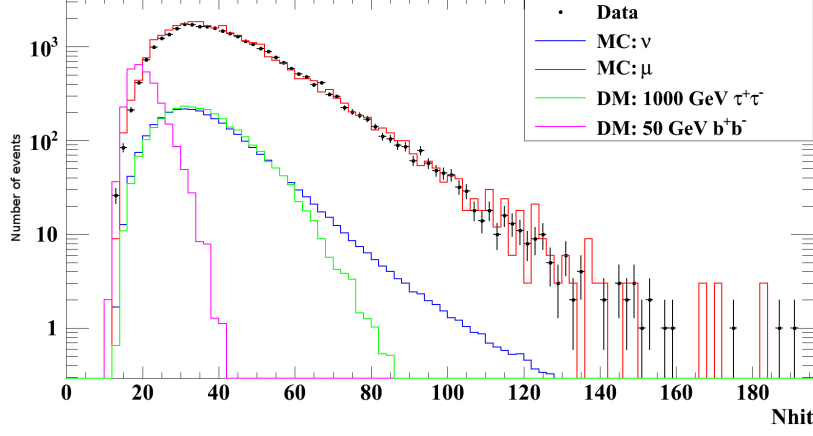
Figure 6.30: Comparison of the N_{hit} distribution of data, MC: atm_{\mu} & atm_{\nu} , and two dark matter models ( 50 GeV b^+b^- & 1000 GeV \tau^+\tau^- ) which were normalized to the number of events of atm_{\nu} . A cut of \Lambda > -5.6 was applied here. The muon and neutrino Monte Carlo are normalized to the lifetime of the data taking.XS
