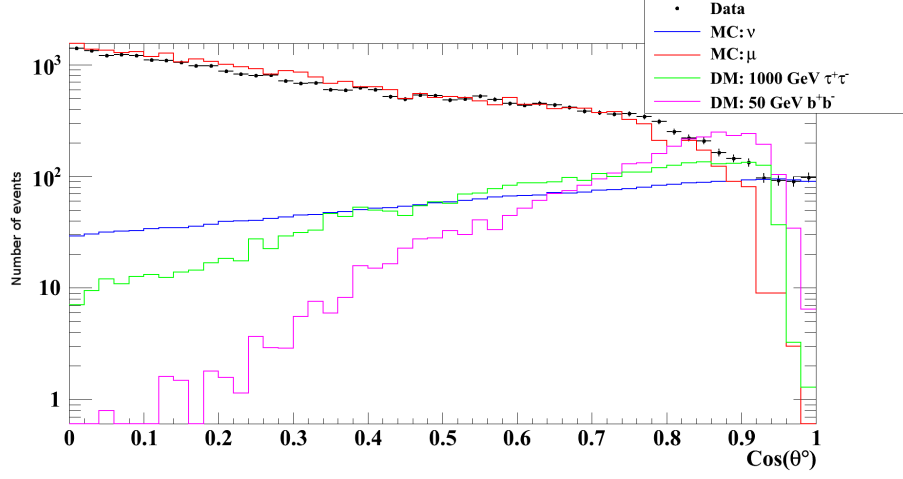
Figure 6.31: Comparison of the \cos(\theta) distribution of data, MC: \text{atm}_\mu & \text{atm}_\nu , and two dark matter models ( 50 GeV b^+b^- & 1000 GeV \tau^+\tau^- ) which were normalized to the number of events of \text{atm}_\nu . A cut of \Lambda > -5.6 was applied here. The muon and neutrino Monte Carlo are normalized to the lifetime of the data taking.
