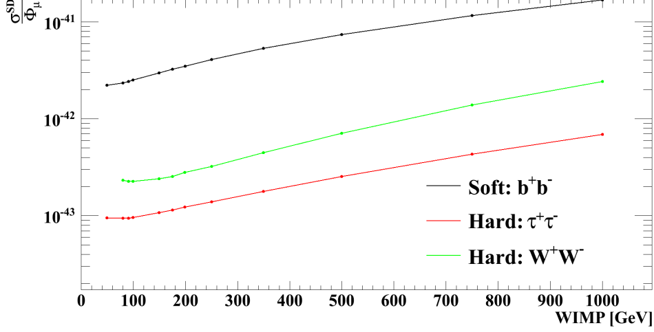
Figure 2.17: Conversion factor from muon flux [ km^{-2}[year^{-1}] ] to spin-dependent cross-section [pb] as a function of the annihilation channel and WIMP mass.
