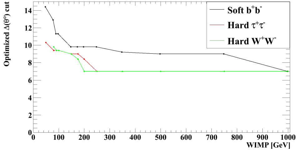
Figure 6.21: Comparison of the optimized \Delta(\theta^\circ) cut as a function of the WIMP mass and the annihilation channel .
