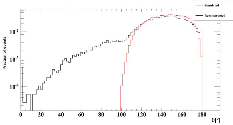
Figure 4.5: Percentage of muons simulated/reconstructed as function of the zenith angle \theta . \theta = 0^\circ is the nadir, \theta = 90^\circ is the horizontal and \theta = 180^\circ is the zenith. This distribution is before any cuts, and reconstructed using the BBFit reconstruction method.
