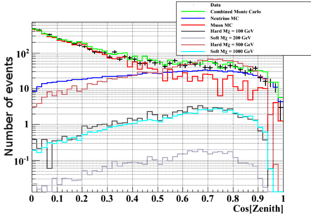
Figure 5.10: Distribution of \text{Cos}[\text{Zenith}] after a cut on T_{\text{chi}2} < 2 for data, atmospheric neutrinos/muons and several Dark Matter models. The muon and neutrino Monte Carlo are normalized to the lifetime of the data taking. The absolute normalization of the Dark Matter distributions are arbitrary.
