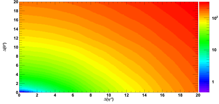
Figure 6.25: Estimation of our background in the direction of the Sun as a function of \Delta(\Psi) & \Delta(\theta) . The cuts used \chi^2_{multi} < 1.6 , \chi^2_{single} < 0.8
