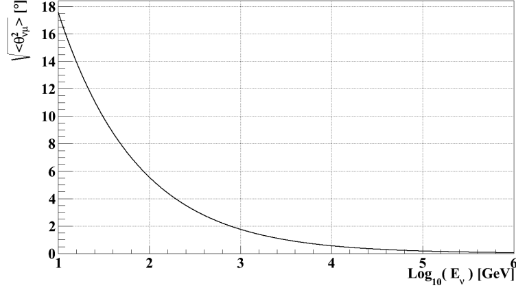
Figure 3.5: Mean kinematic angle between the neutrino and the muon as a function of energy of the neutrino.
