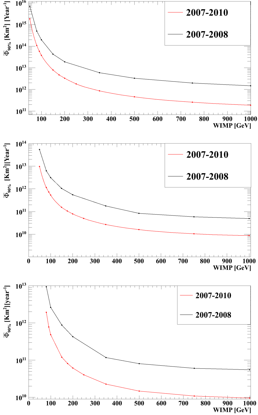
Figure 6.12: Comparison of sensitivities to neutrino flux coming from dark matter annihilation inside the Sun as a function of WIMP mass between the 2007-2008 and 2007-2010 analysis. Top plot is for b^+b^- , middle is for \tau^+\tau^- , and the bottom is for W^+W^- .
