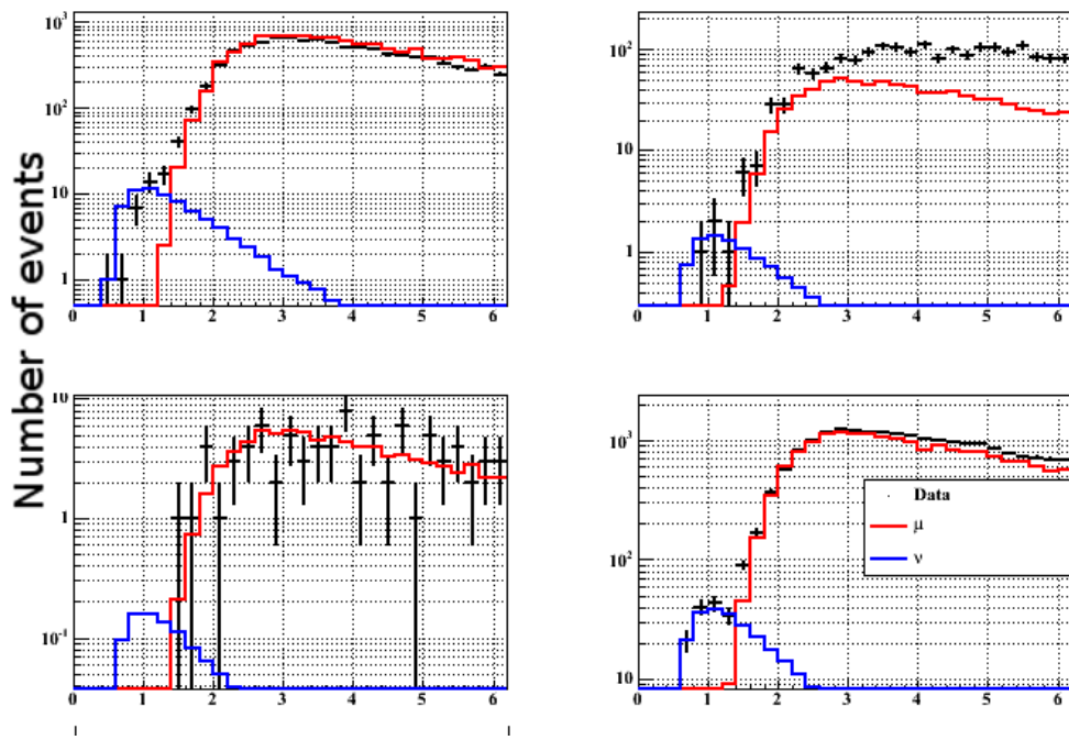
Figure 5.8: Tchi2 distribution for data and atmospheric neutrinos/muons for only the 10pe threshold of the 5,9,10,12 Lines detector periods. Upper left plot is for the 5 lines detector, upper right is for 9 lines, bottom left is for the 10 lines, and bottom right is for 12 lines. The Monte Carlo is normalized to the lifetime of the data taking.
