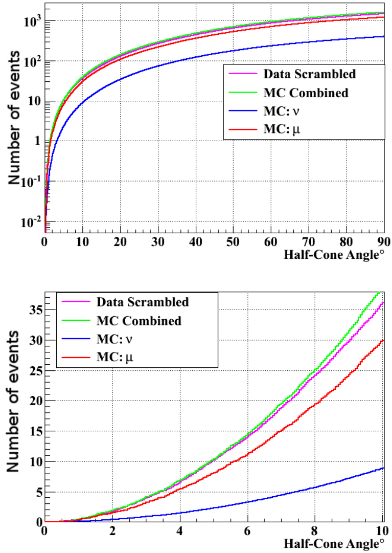
Figure 5.15: Estimation of the background distribution in the direction of the Sun, i.e the number of events inside a cone centered around the Sun as a function of the cone's half opening angle, with a quality cut of T_{chi2} < 2 .
