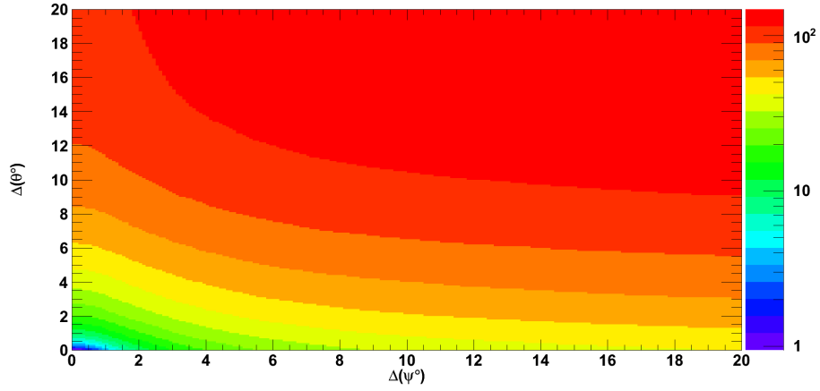
Figure 6.26: Estimation of the signal of 50 GeV \tau^+\tau^- dark matter model as a function of \Delta(\Psi) & \Delta(\theta) . The cuts used \chi^2_{multi} < 1.6 , \chi^2_{single} < 0.8
