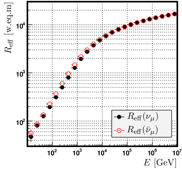
Figure 5.30: Effective range of \bar{\mu}/\mu as a function of its neutrino energy [108] .
