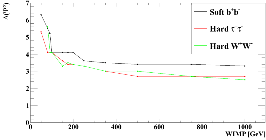
Figure 6.10: Comparison of the optimized \Delta(\Psi^0) cut as a function of the WIMP mass and the annihilation channel .
