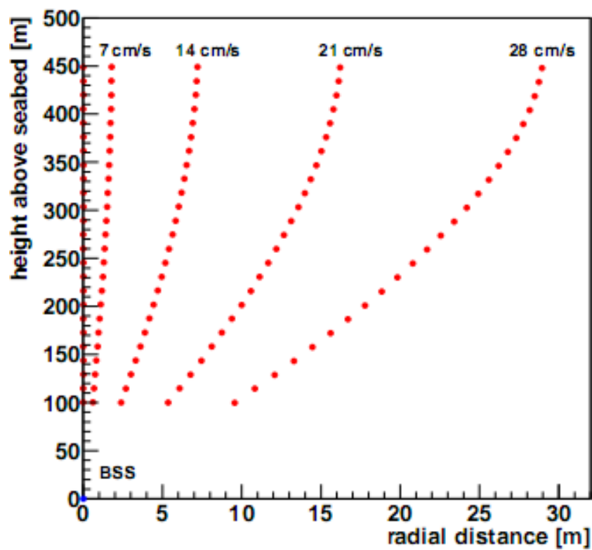
Figure 3.20: Height and radial displacement of each and every stories of a line for different sea current velocities.
