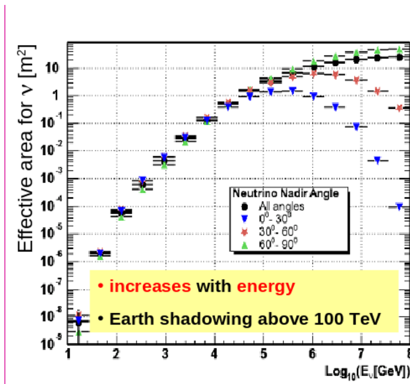
Figure 3.30: Effective area at trigger level for the neutrinos as a function of \text{Log}_{10}(\text{neutrino energy}) .
