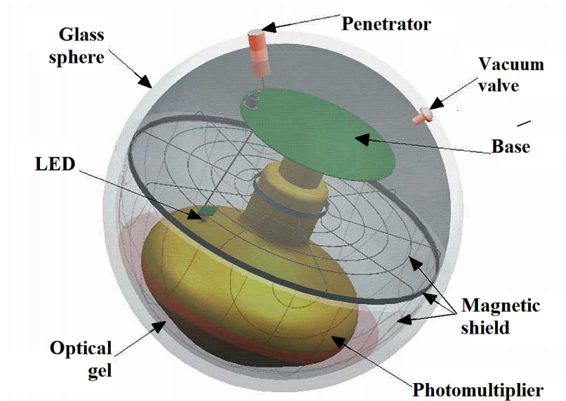
Figure 3.12: ANTARES Optical Module
