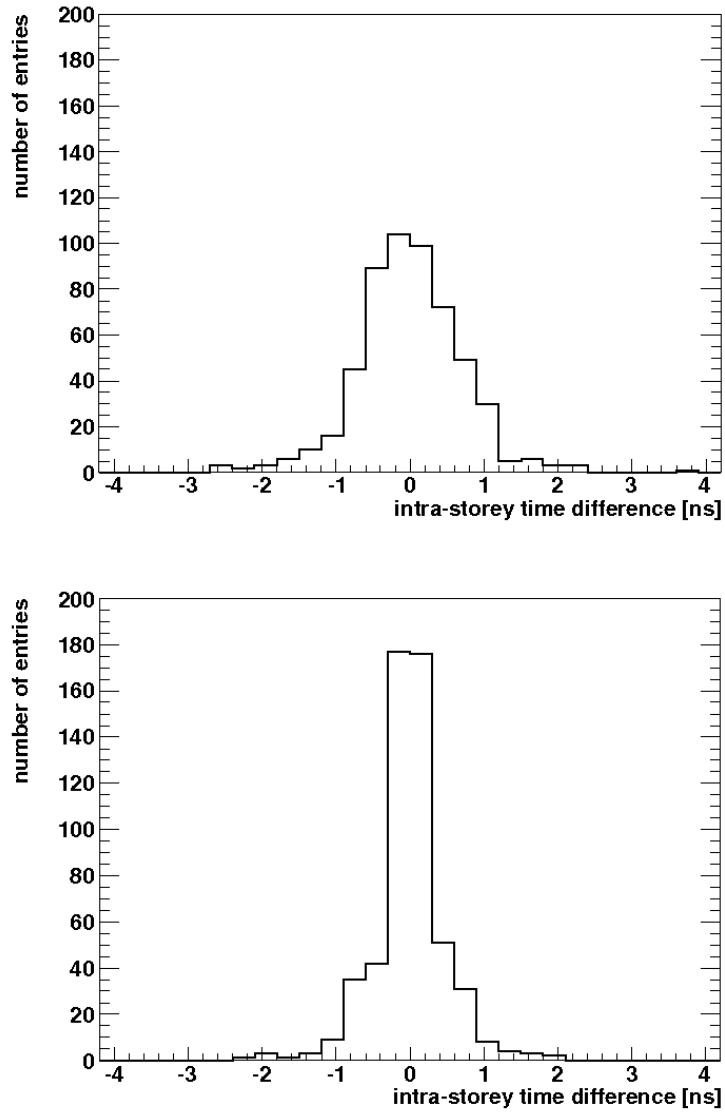
Figure 3.24: Time offset among OMs in the same storey for one of the lines using the time offsets measured onshore (up) and in situ (down).
