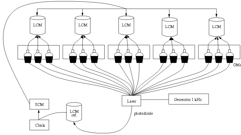
Figure 3.23: OM time offset calibration setup as done in a dark room.
