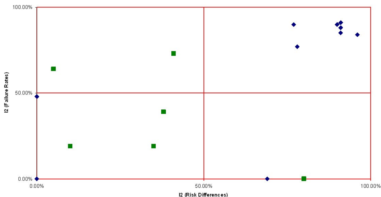
Figure 4. I^2 of RDs versus I^2 of FRs for studies from the ASAQ meta-analysis database ( \diamond ) and the virtual studies ( \square )
