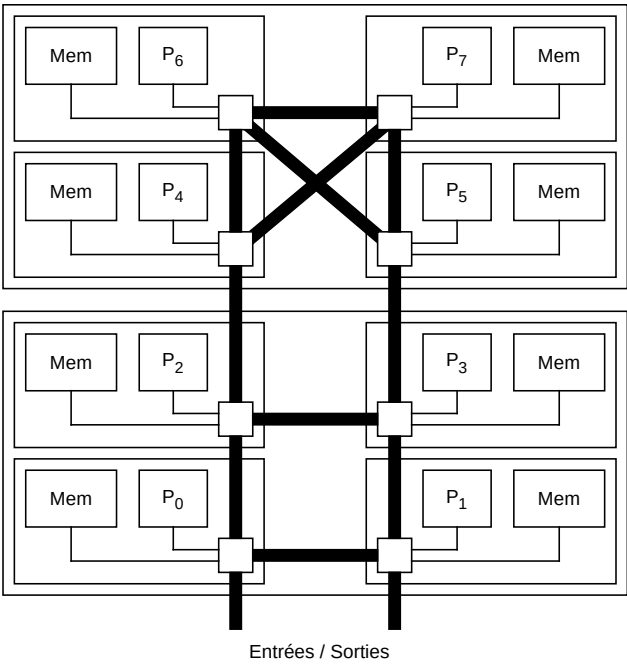
FIG. 5.2 – Architecture de la machine Hagrid.
