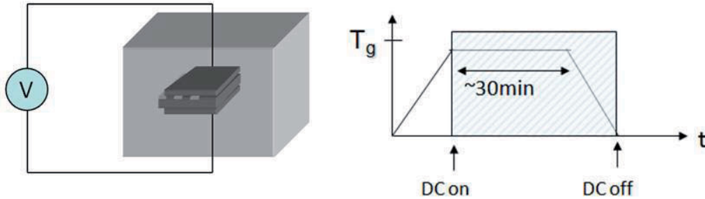
Figure 7.2 Thermal poling of glass
