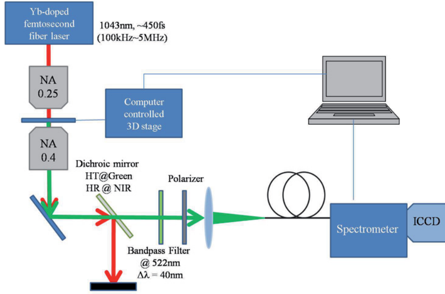
Figure 7.7 SHG measurement setup
