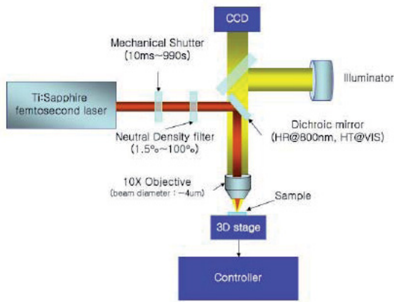
Figure 3.17 Schematic diagram of a laser direct writing system
