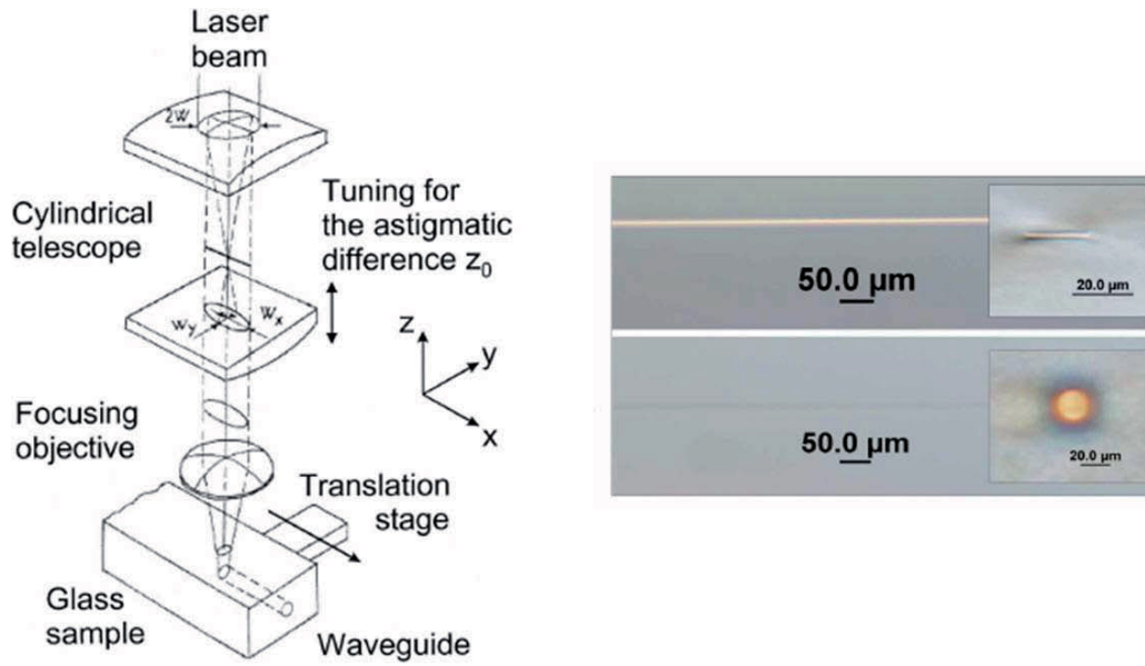
Figure 3.6 Astigmatic beam shaping using a cylindrical lens (left, From [50]) and a waveguide written in a phosphate glass with/without a slit with width of 500 \mu\text{m} (right, From [51])
