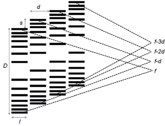
Figure 6.3 Schematic diagram of a stack of spread FZPs
