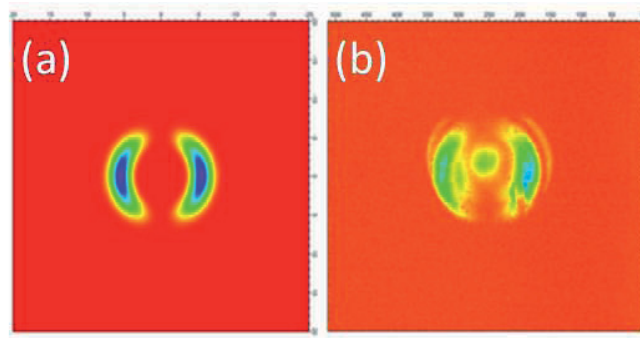
Figure 7.12 SHG distribution at horizontal polarization of probe and analyzer, (a) theoretical (b) experimental
