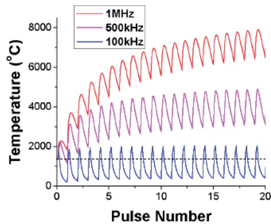
Figure 2.10 Heat accumulation effect. Finite-difference model of glass temperature at a radial position of 2 \mu\text{m} from the center of the laser pulse. From [46]
