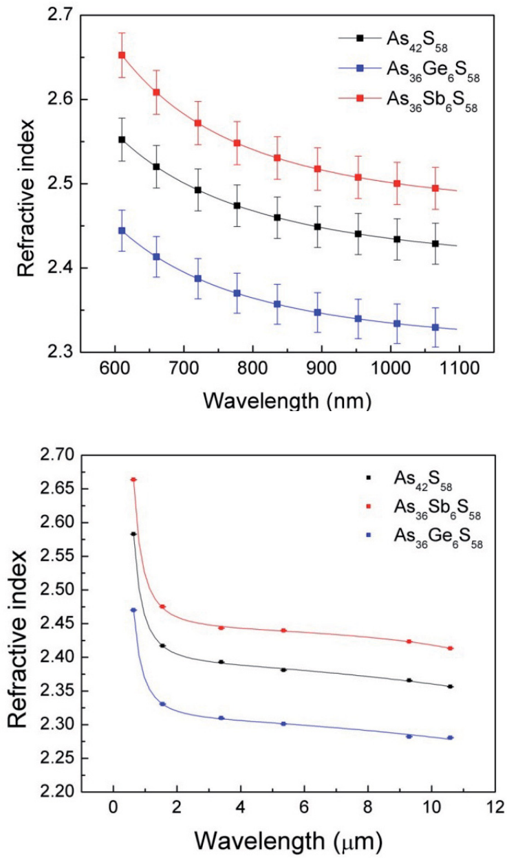
Figure 4.2 Refractive index of given materials (top) in NIR region (bottom) in MIR region. From [84] 4
