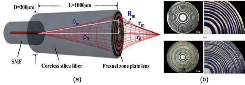
Figure 5.4 Binary FZP created on a coreless silica fiber attached on to a single mode fiber. From [115].
