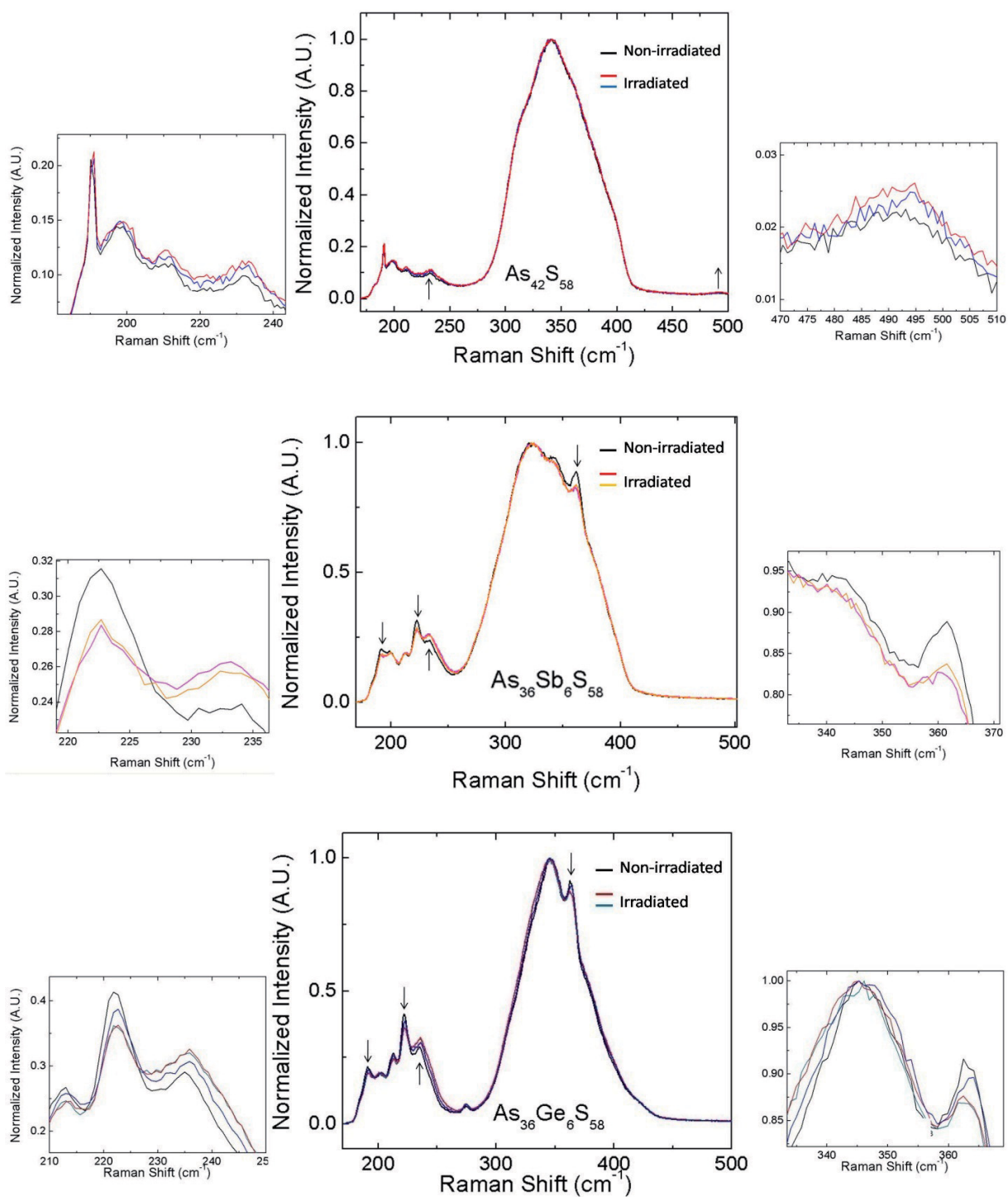
Figure 8.2 Raman shift of irradiated and non-irradiated \text{As}_{42}\text{S}_{58} , \text{As}_{36}\text{Sb}_6\text{S}_{58} and \text{As}_{36}\text{Ge}_6\text{S}_{58} after annealing
