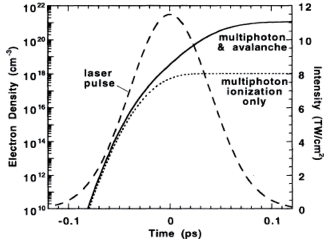
Figure 2.6 Electron density of the material irradiated by a ultrashort pulse with/without a participation of avalanche ionization. From [32].
