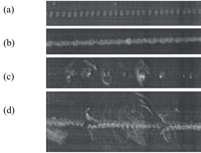
Figure 2.4 Comparison of micro drilling of PET plastic with different pulse widths at 800 nm. (a),(b) 80 fs, 5 \mu\text{J}/\text{pulse} , with translation speed at 20 mm/s, 8 mm/s (c),(d) 200 ps. 20 \mu\text{J}/\text{pulse} , 15 mm/s and 150 \mu\text{J}/\text{pulse} , 20 mm/s. 80 fs pulses shows regularly ablated dots compared to 200 ps. From [37]
