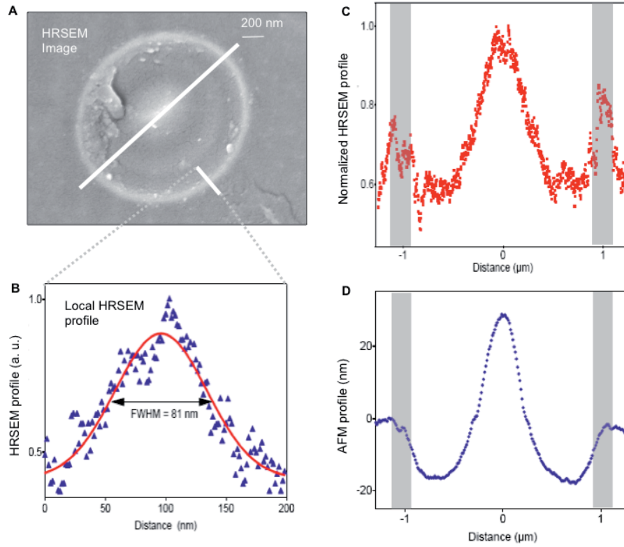
Figure 7.4 HRSEM and AFM characterization of the nanostructures. (a) HRSEM (b) the transversal profile of the rim (c,d) profiles across the ring. From [131]
