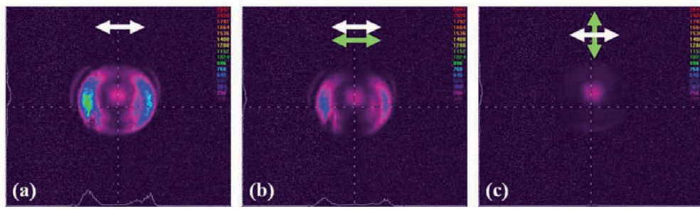
Figure 7.11 Intensity map of the SHG of Ag micro-structure (a) no analyzer, the direction of the analyzer (b) parallel (HH) and (c) perpendicular (HV) to the polarization of the laser
