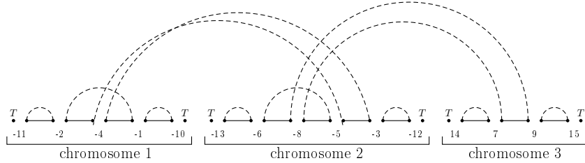
Figure 2.11: Application of the algorithm Proper_Flip_Left to genomes \Pi and \Gamma . (a) Entry data. (b) Graph G(\Pi^*, \Gamma^*) obtained from optimal cappings \Pi^* = \hat{\Pi} and \Gamma^* = \hat{\Gamma} . There are two interchromosomal and unoriented components: chromosomes 1 and 2 are those to flip. (c) Proper flipping of chromosome 2. (d) Proper flipping of chromosome 1. Obtained graph is properly flipped.
