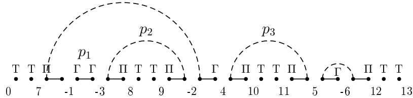
Figure 7.3: Counterexample to Ozery-Flato and Shamir's algorithm [OFS03] for building an optimal capping. Breakpoint graph G(\Pi, \Gamma) with \Pi = \{-1 \ -3, \ -2 \ 4, \ 5 \ -6\} and \Gamma = \{1 \ 2 \ 3, \ 4 \ 5 \ 6\} .
